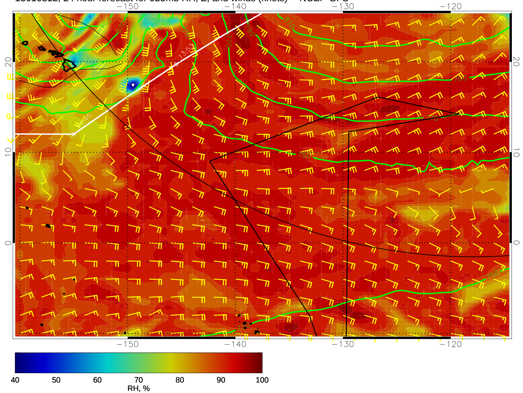
15010312, 24 hour forecast for 925mb RH, Z, and winds (knots) -- NCEP GFS
