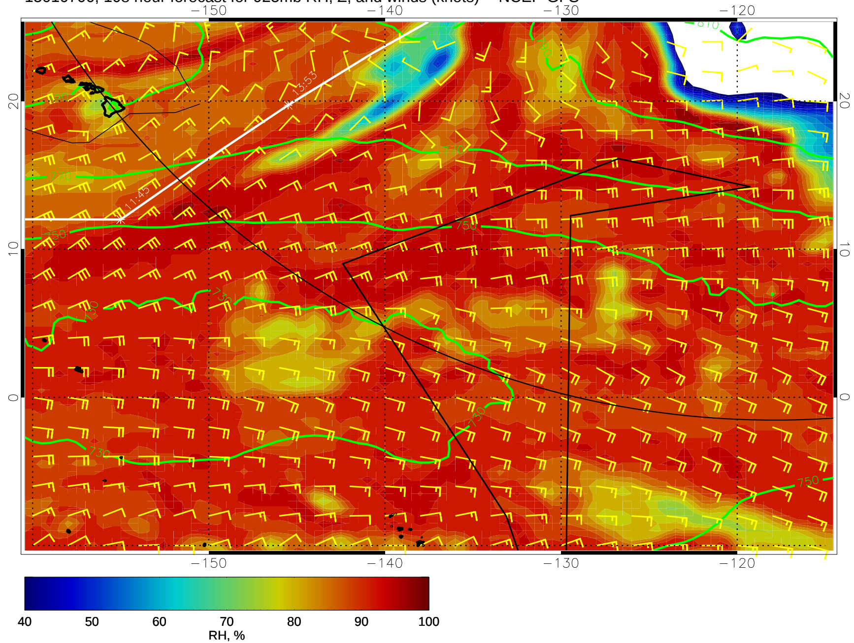
15010700, 108 hour forecast for 925mb RH, Z, and winds (knots) -- NCEP GFS
