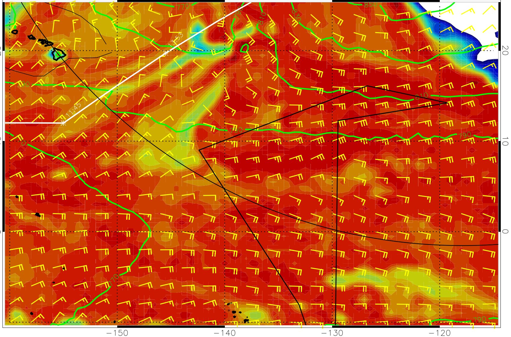
10010010, 10-hour forecast for elements T1H, U, and winds (knots) 10010010 10010010 10010010 10010010 -150 -140 -130 -120
