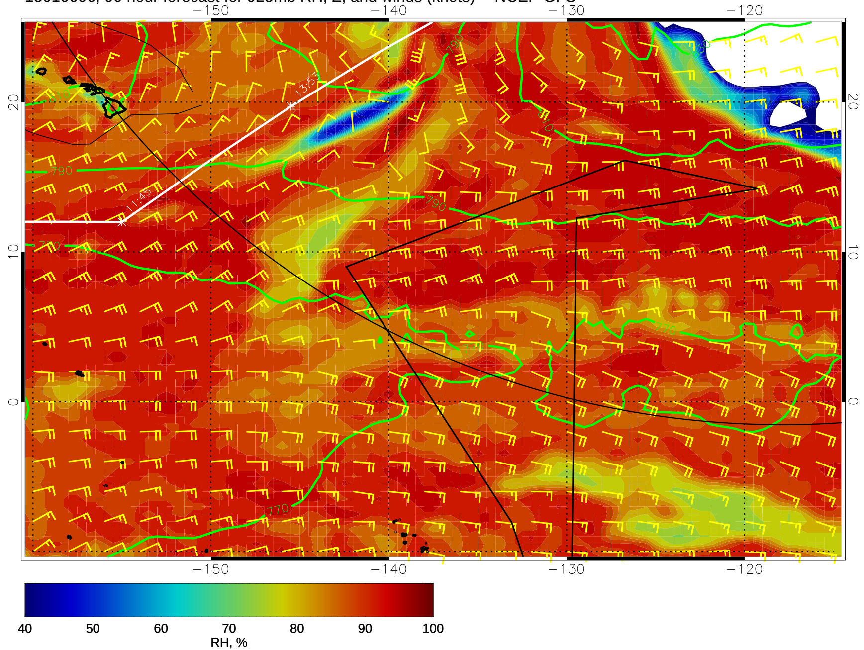
15010606, 90 hour forecast for 925mb RH, Z, and winds (knots) -- NCEP GFS
