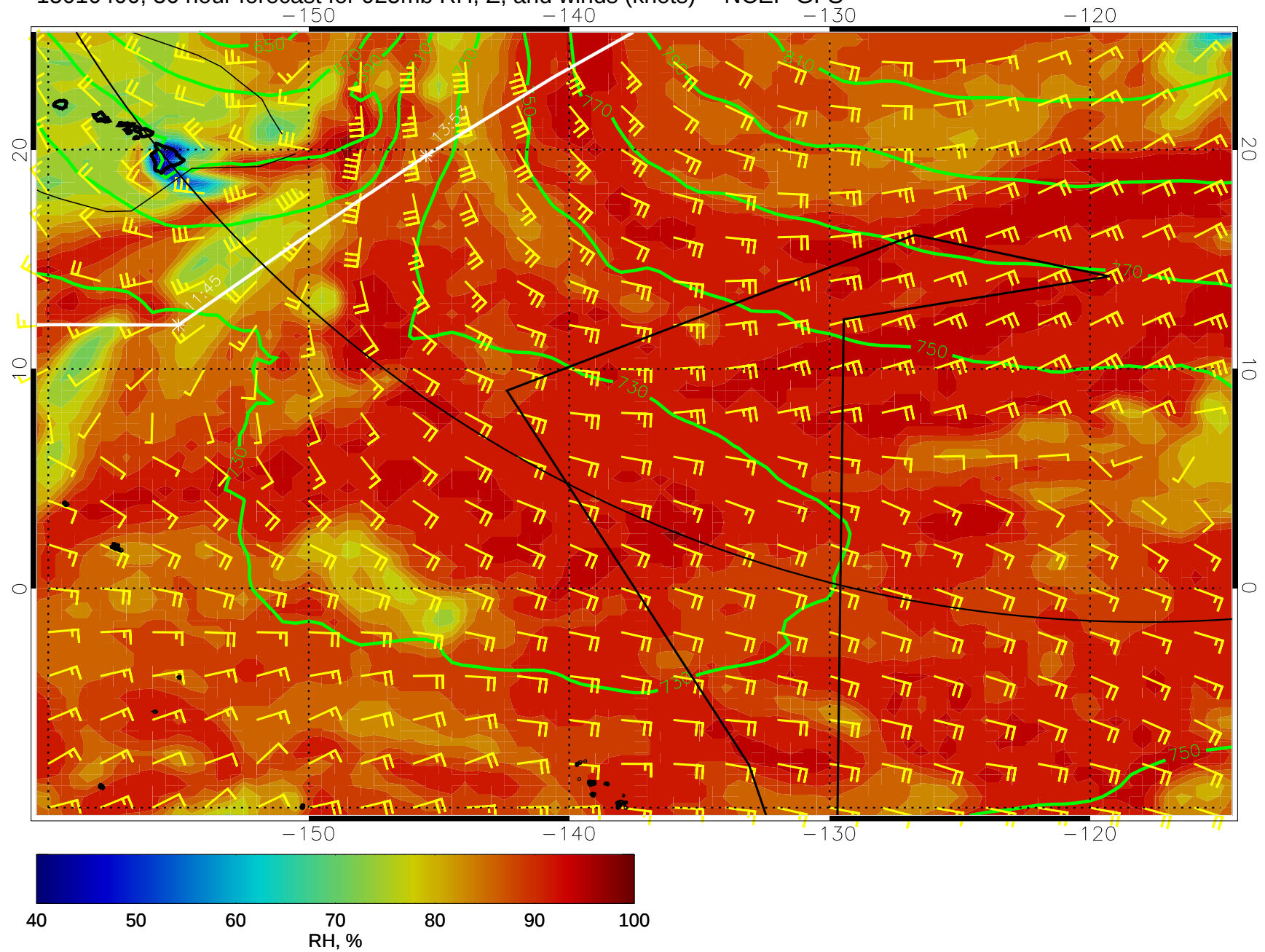
15010400, 36 hour forecast for 925mb RH, Z, and winds (knots) -- NCEP GFS
