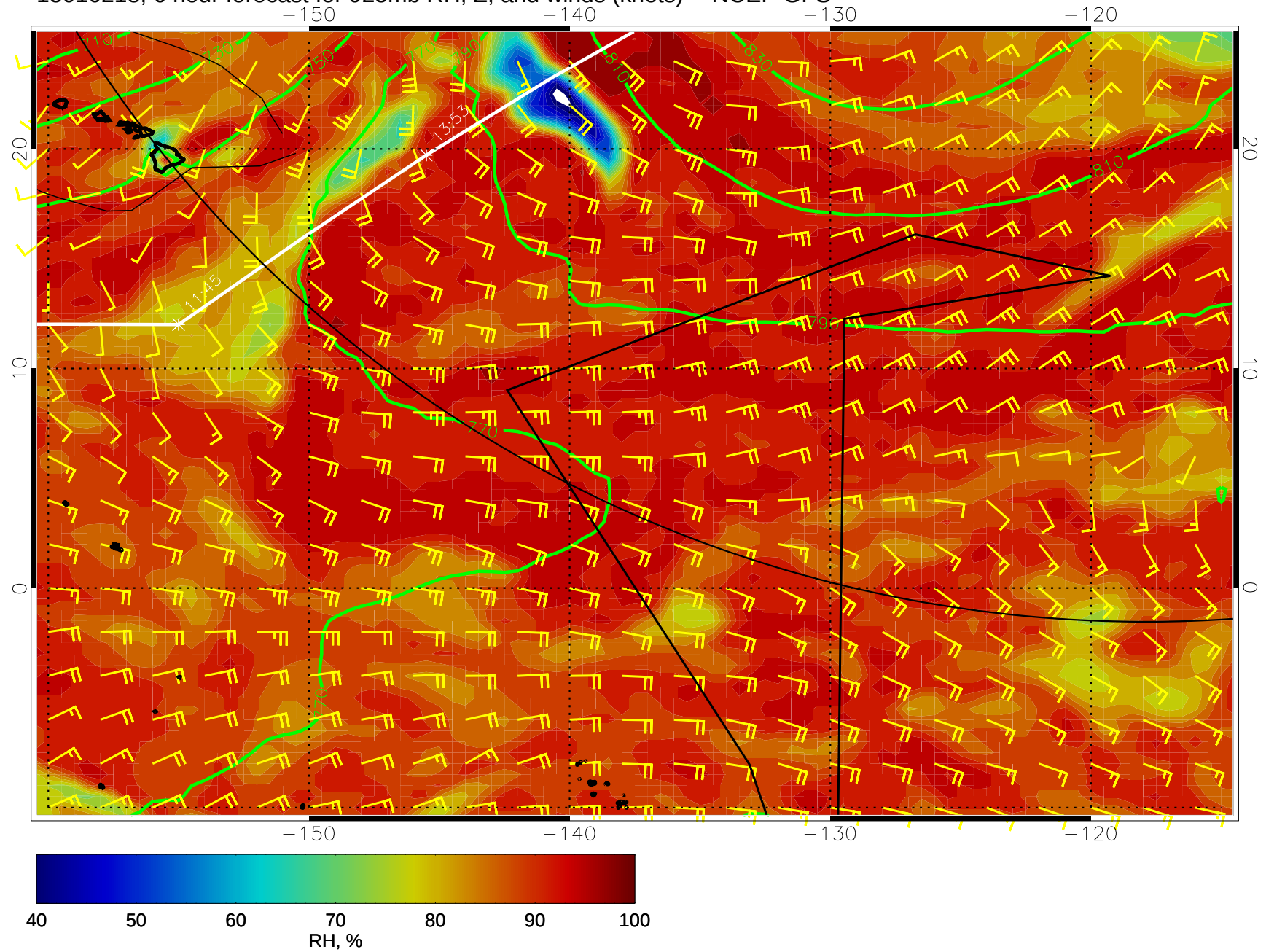
15010218, 6 hour forecast for 925mb RH, Z, and winds (knots) -- NCEP GFS
