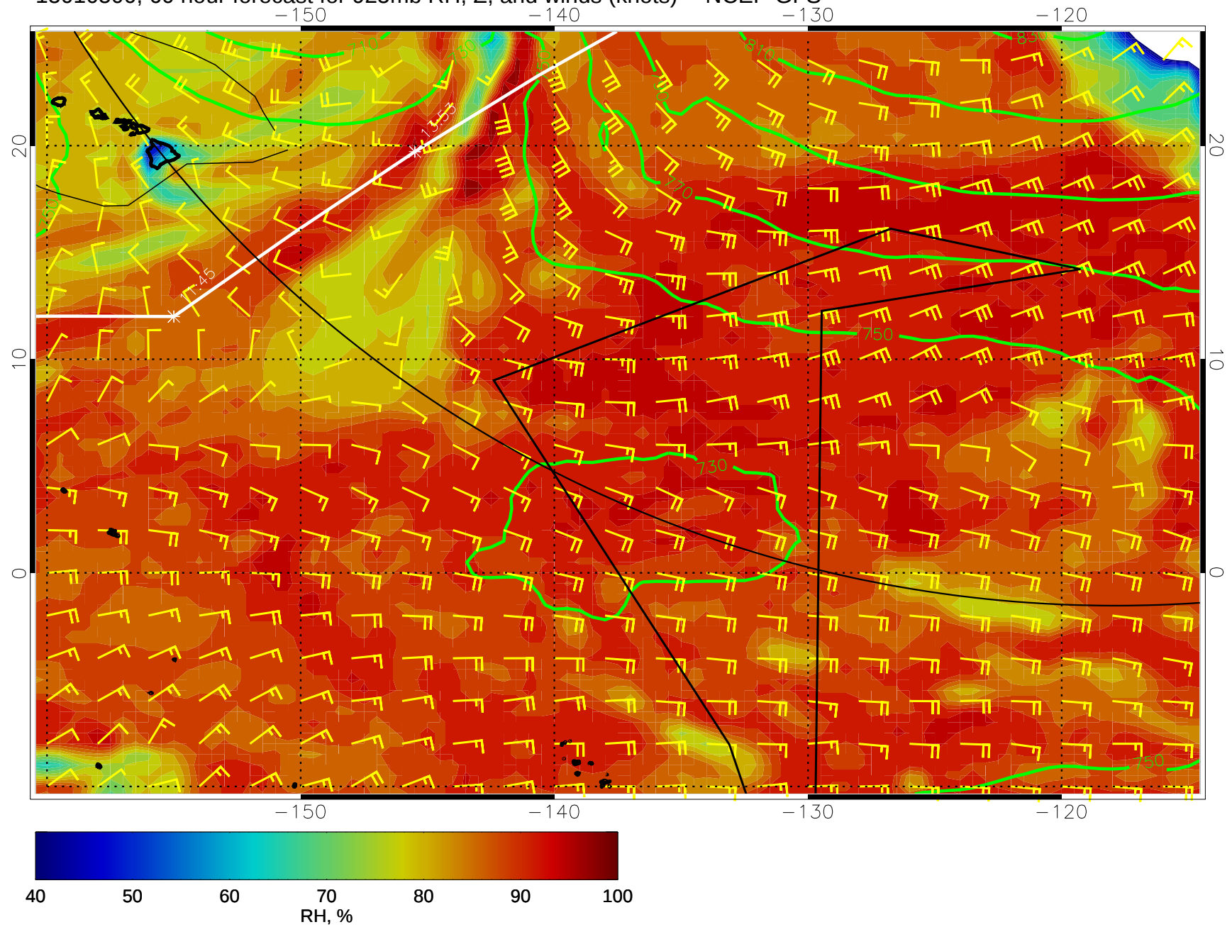
15010500, 60 hour forecast for 925mb RH, Z, and winds (knots) -- NCEP GFS
