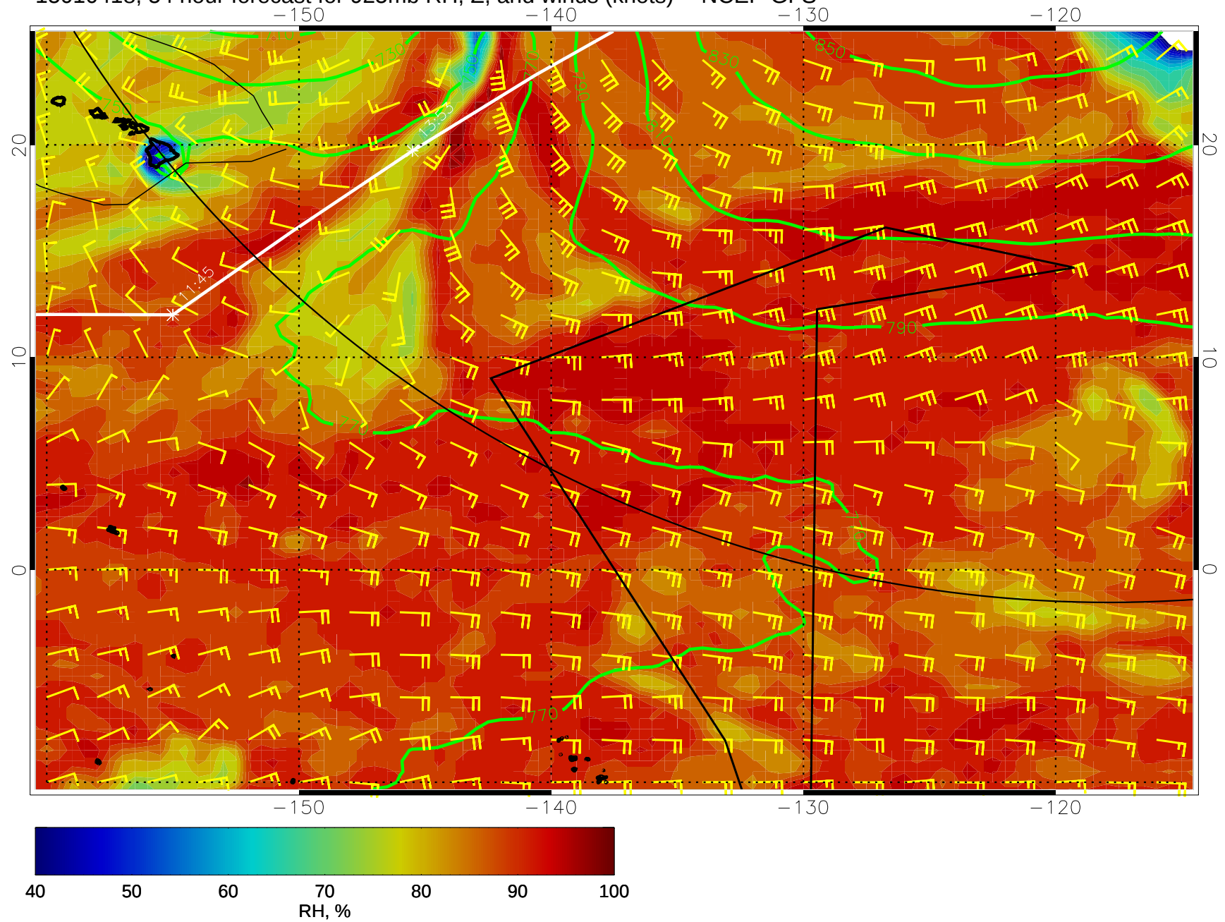
15010418, 54 hour forecast for 925mb RH, Z, and winds (knots) -- NCEP GFS
