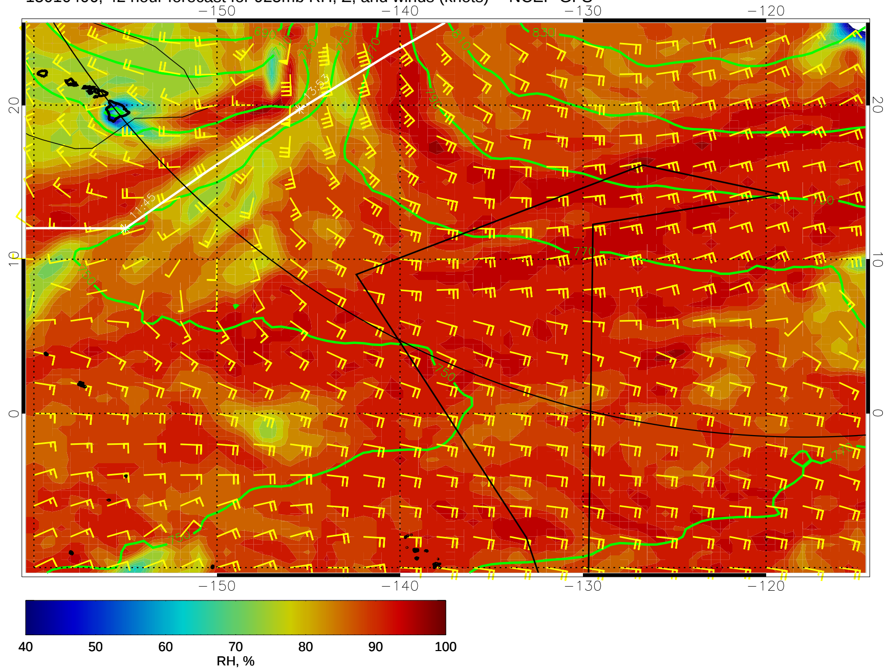
15010406, 42 hour forecast for 925mb RH, Z, and winds (knots) -- NCEP GFS
