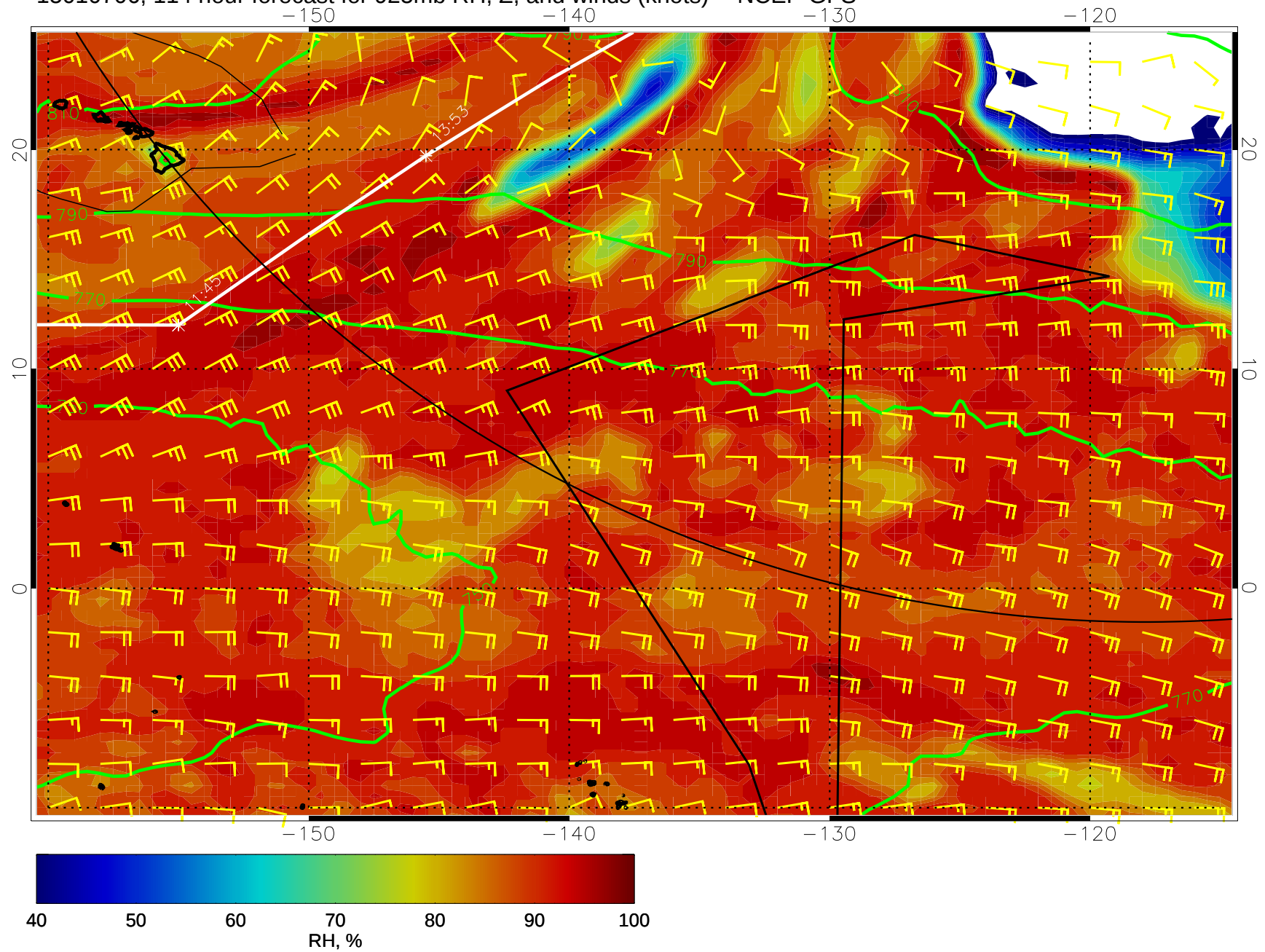
15010706, 114 hour forecast for 925mb RH, Z, and winds (knots) -- NCEP GFS
