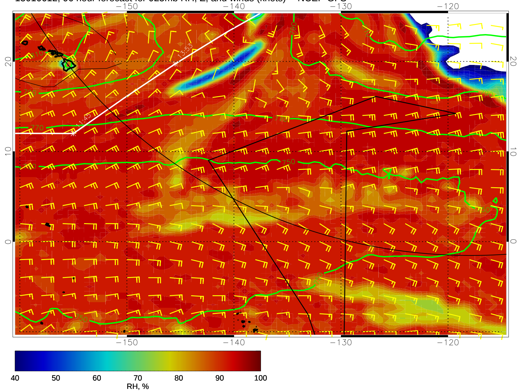
15010612, 96 hour forecast for 925mb RH, Z, and winds (knots) -- NCEP GFS
