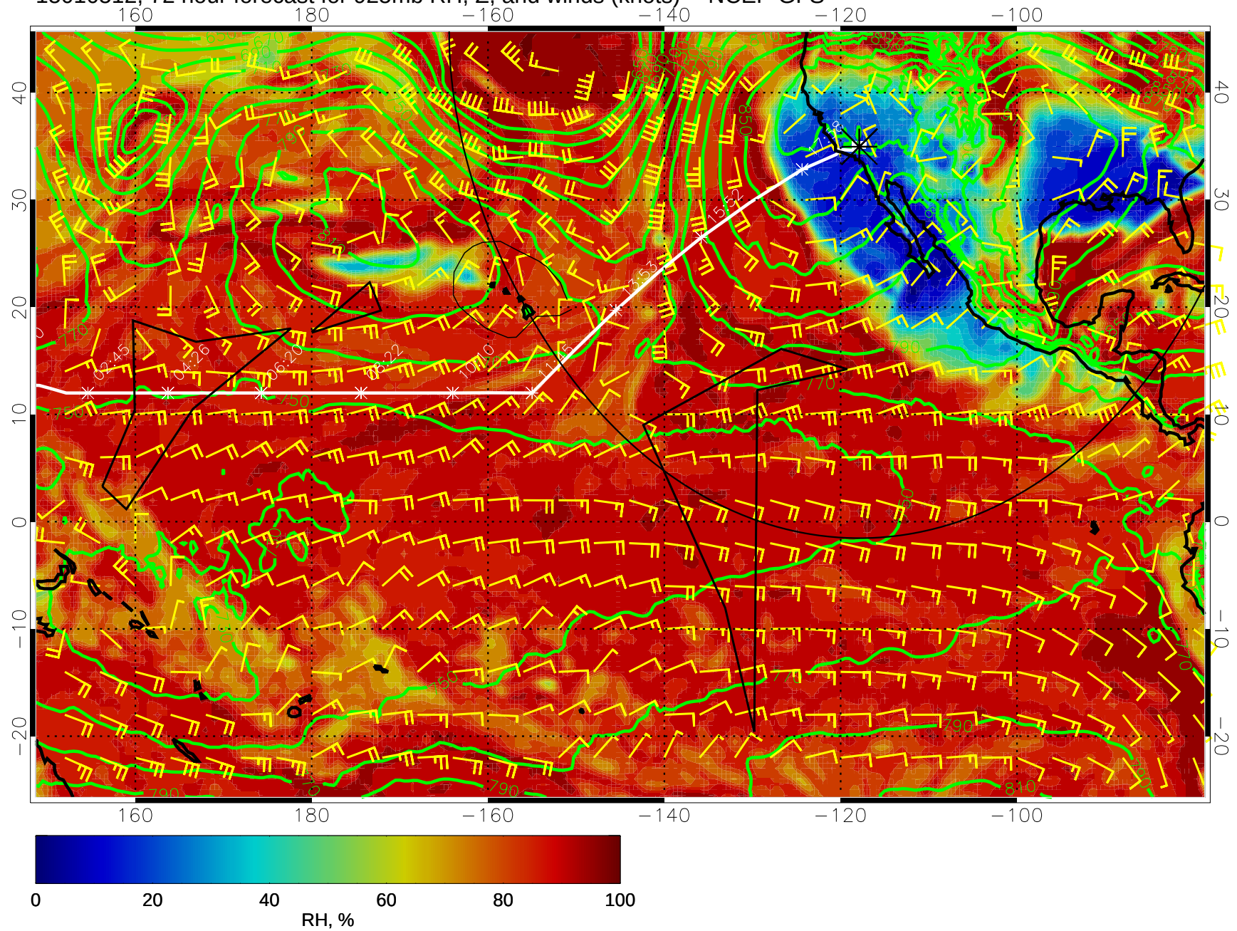
15010512, 72 hour forecast for 925mb RH, Z, and winds (knots) -- NCEP GFS
