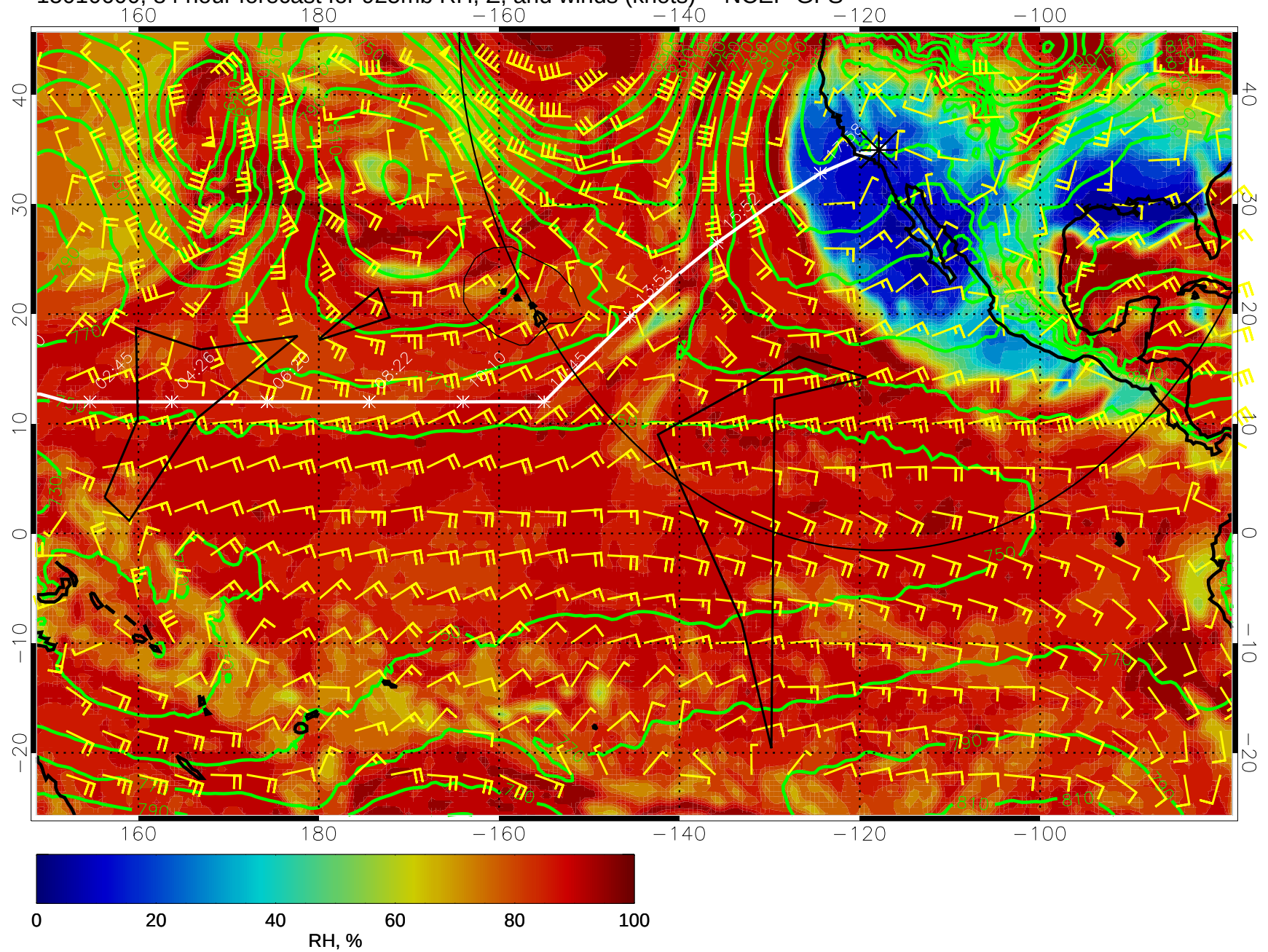
15010600, 84 hour forecast for 925mb RH, Z, and winds (knots) -- NCEP GFS
