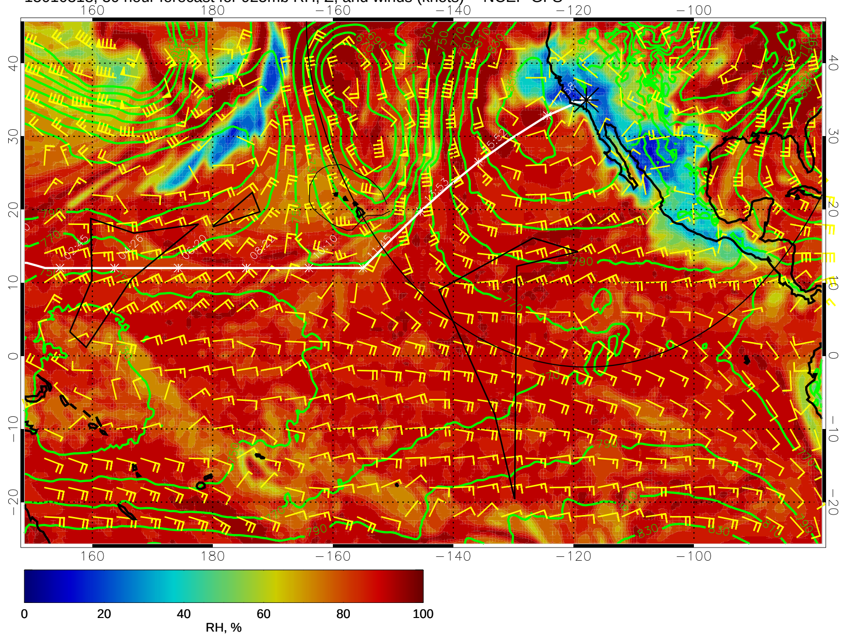
15010318, 30 hour forecast for 925mb RH, Z, and winds (knots) -- NCEP GFS
