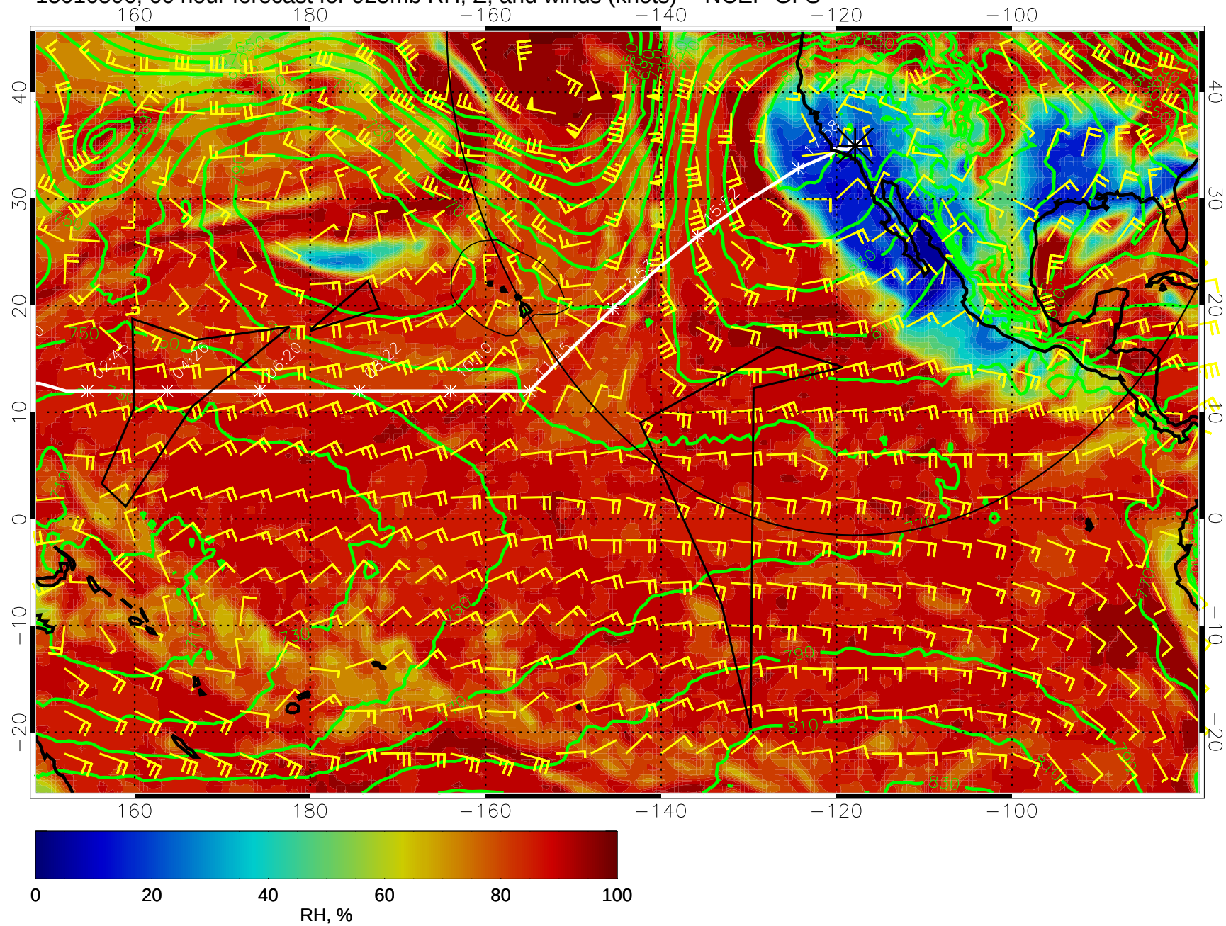
15010506, 66 hour forecast for 925mb RH, Z, and winds (knots) -- NCEP GFS
