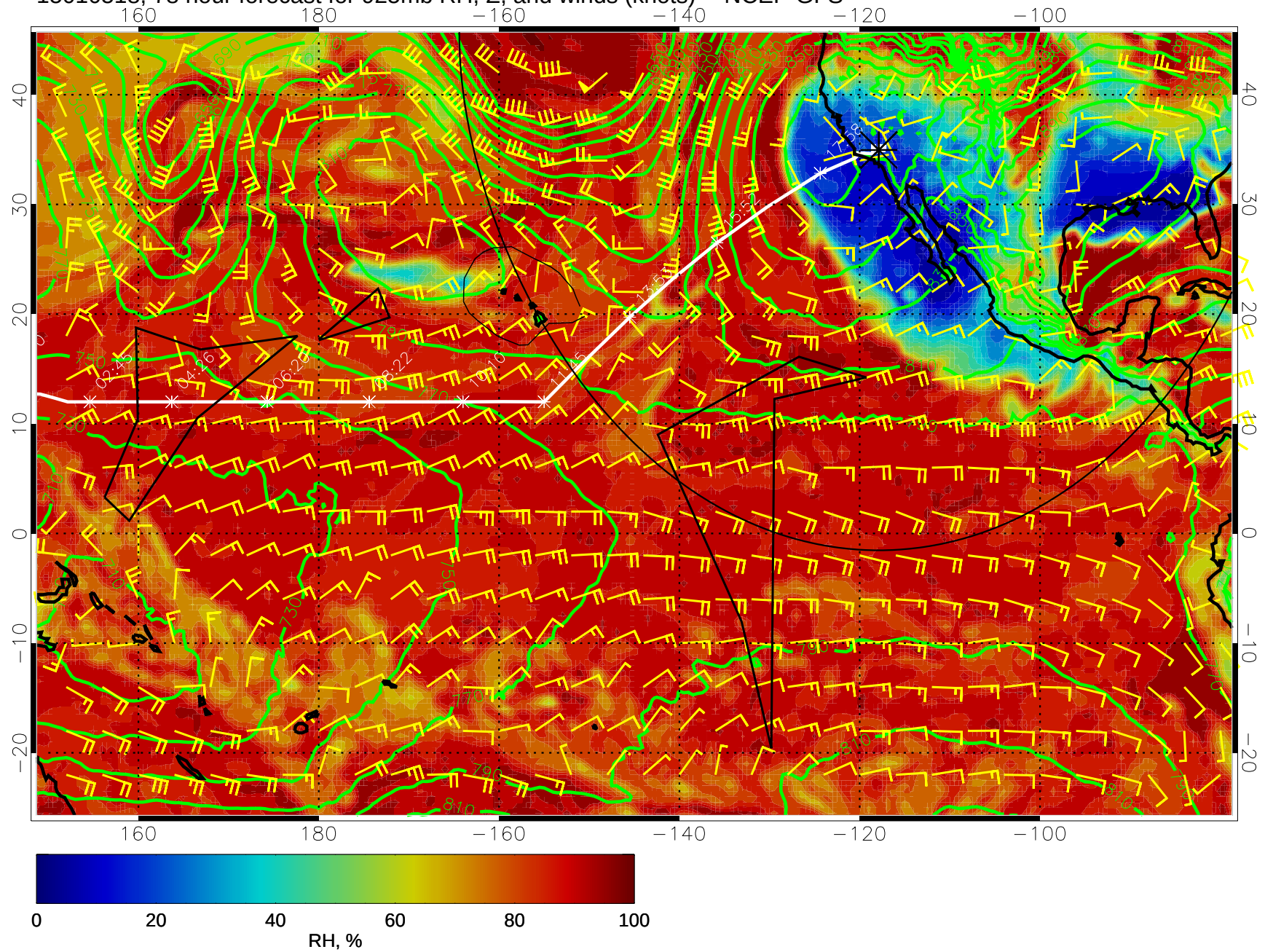
15010518, 78 hour forecast for 925mb RH, Z, and winds (knots) -- NCEP GFS
