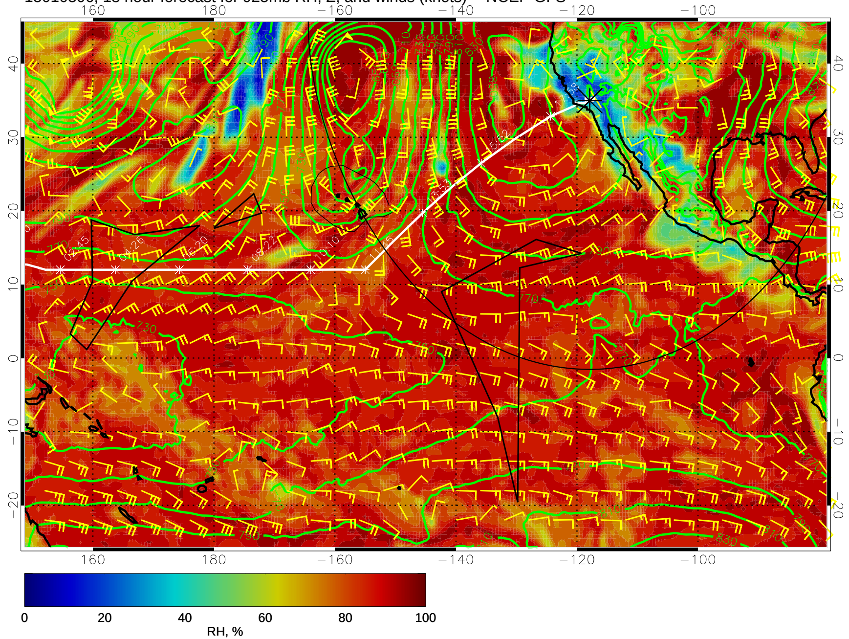
15010306, 18 hour forecast for 925mb RH, Z, and winds (knots) -- NCEP GFS
