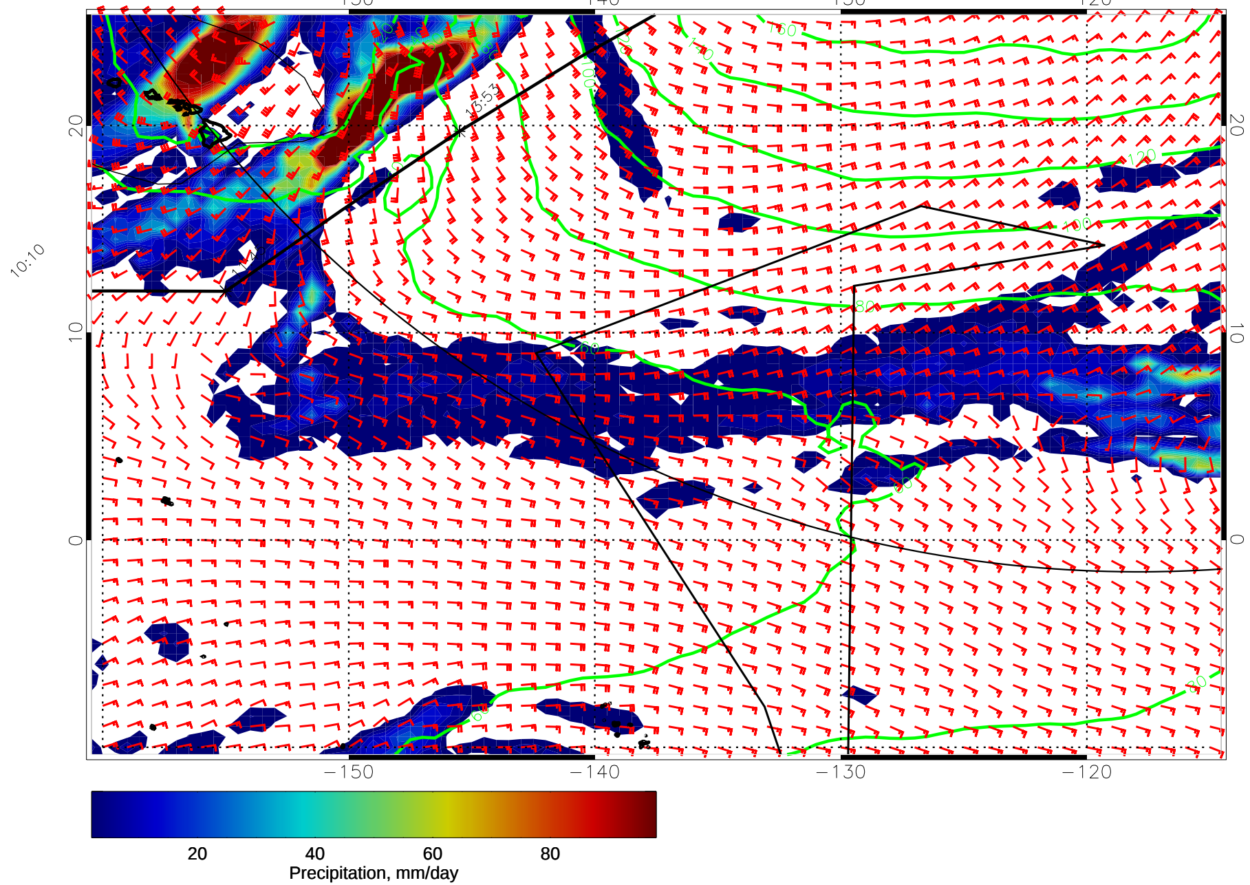
15010312, 24 hour forecast for precip, 1000mb Z, and winds (knots) -- NCEP GFS
