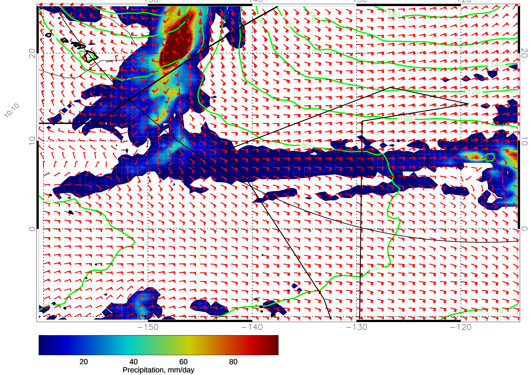
15010406, 42 hour forecast for precip, 1000mb Z, and winds (knots) -- NCEP GFS
