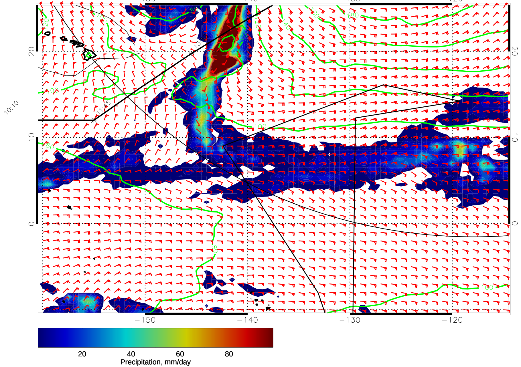
15010506, 66 hour forecast for precip, 1000mb Z, and winds (knots) -- NCEP GFS
