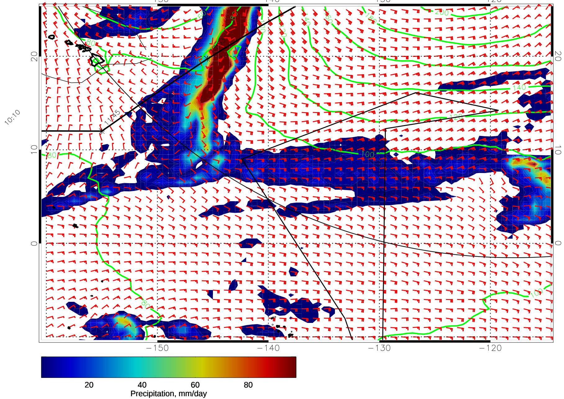
15010418, 54 hour forecast for precip, 1000mb Z, and winds (knots) -- NCEP GFS
