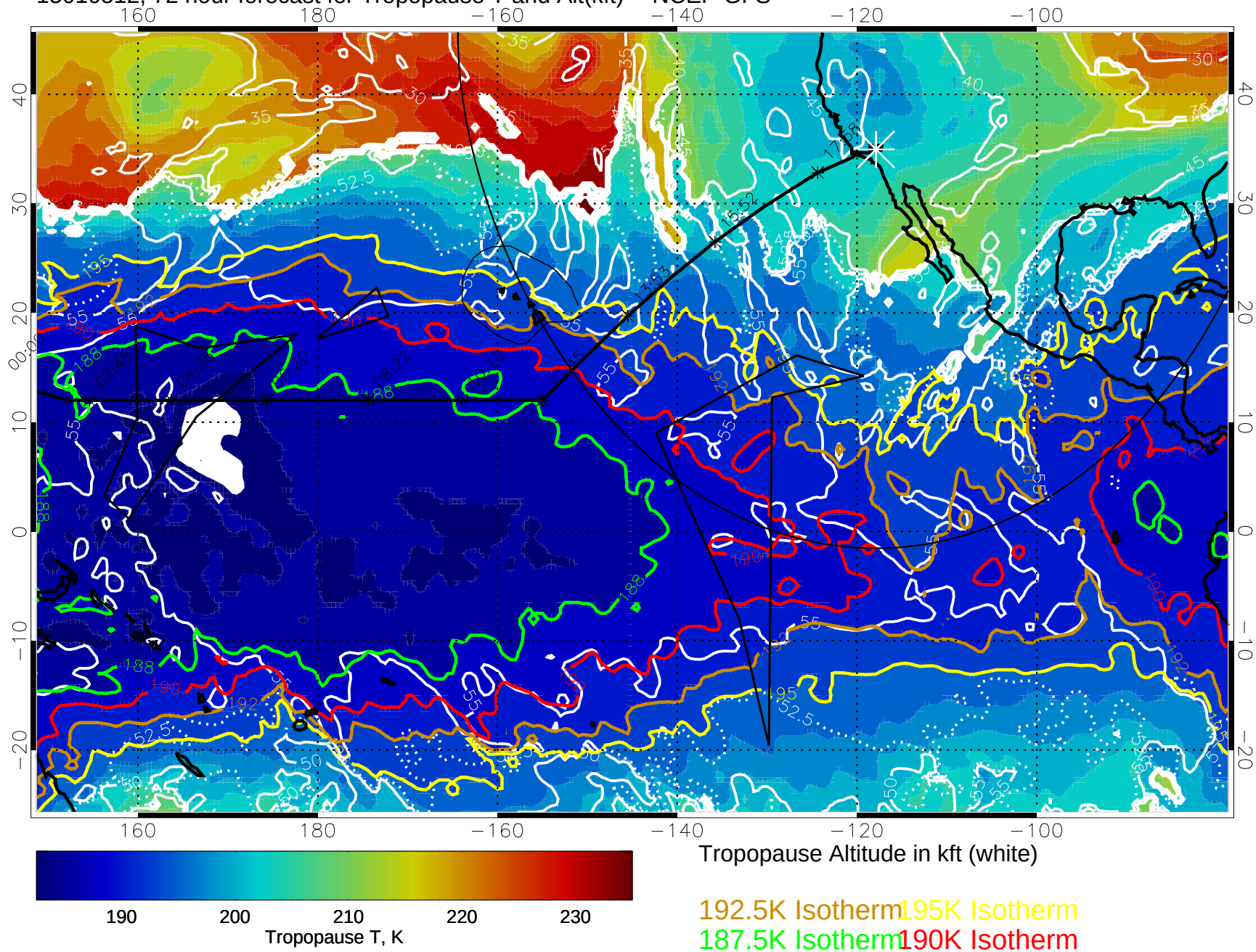
15010512, 72 hour forecast for Tropopause T and Alt(kft) -- NCEP GFS
