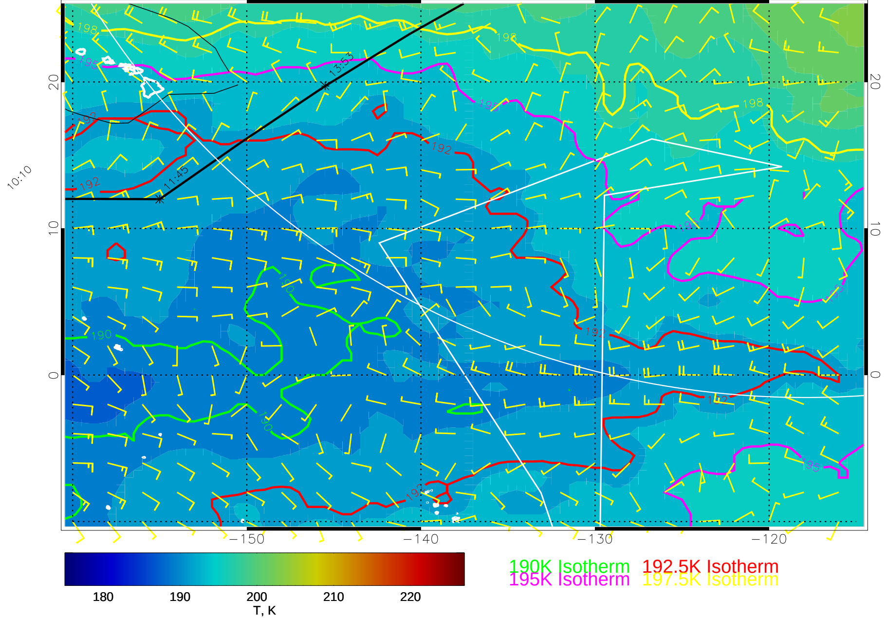
15010706, 114 hour forecast for 70mb T and winds (knots) -- NCEP GFS
