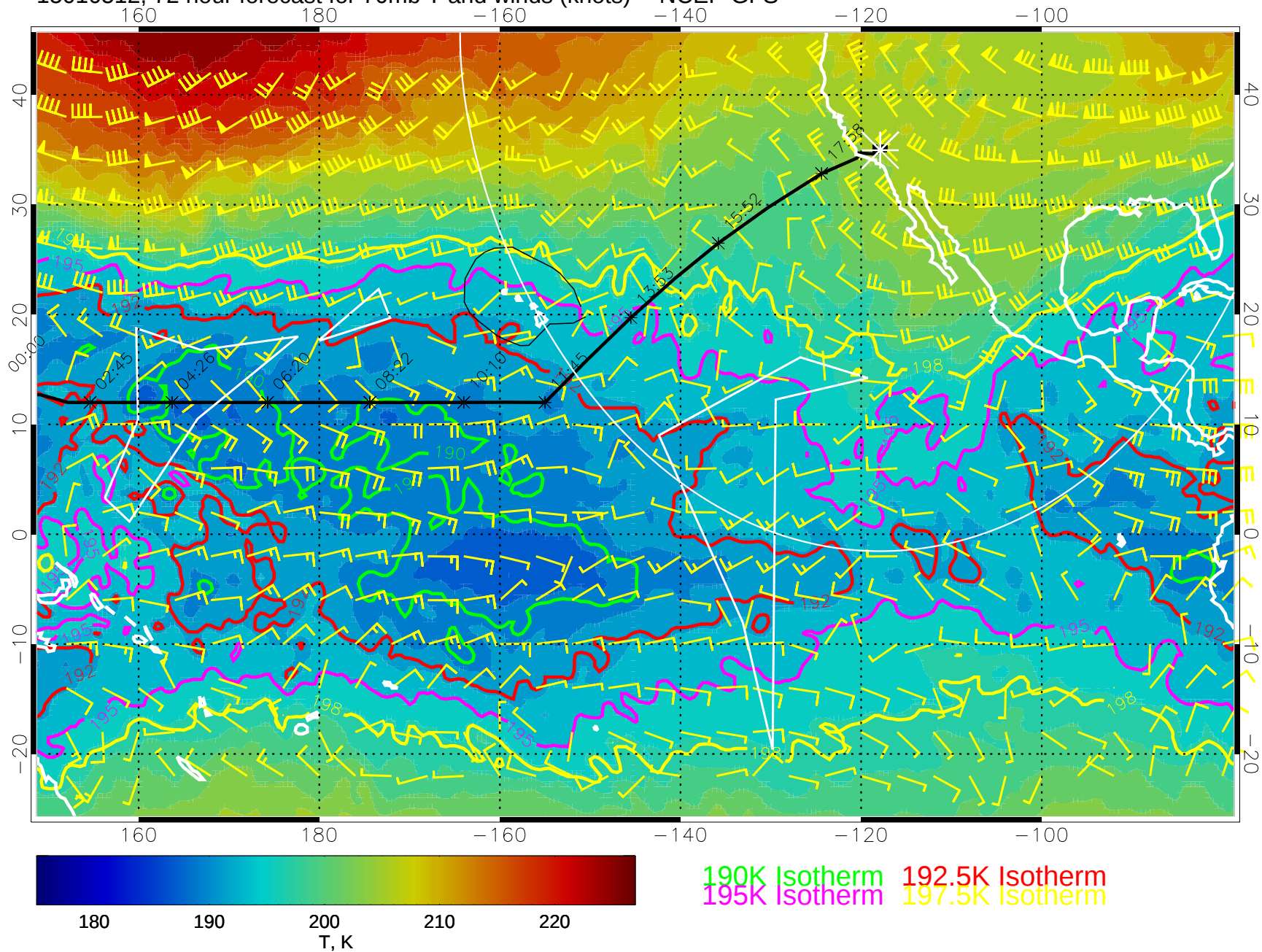
15010512, 72 hour forecast for 70mb T and winds (knots) -- NCEP GFS
