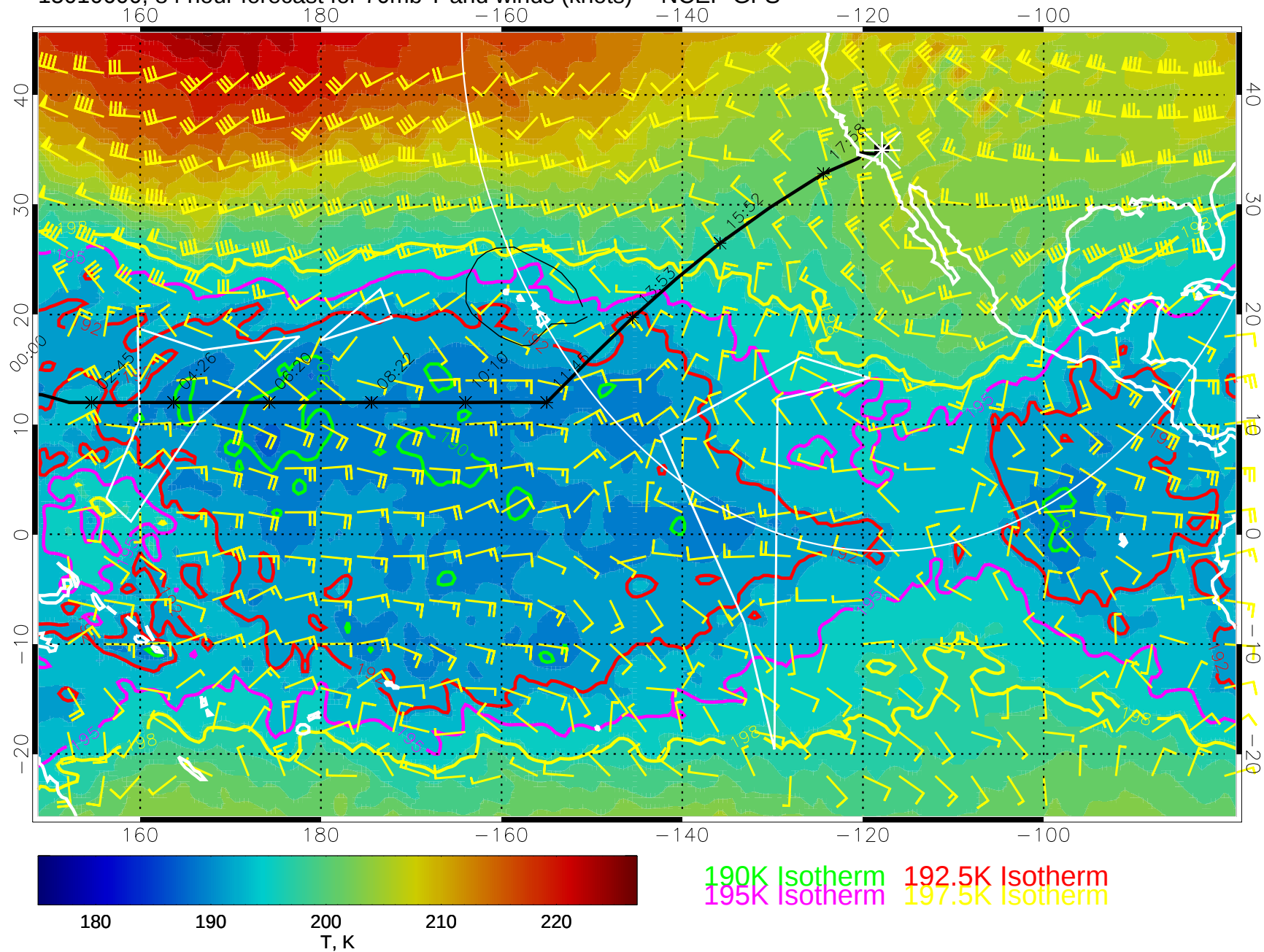
15010600, 84 hour forecast for 70mb T and winds (knots) -- NCEP GFS
