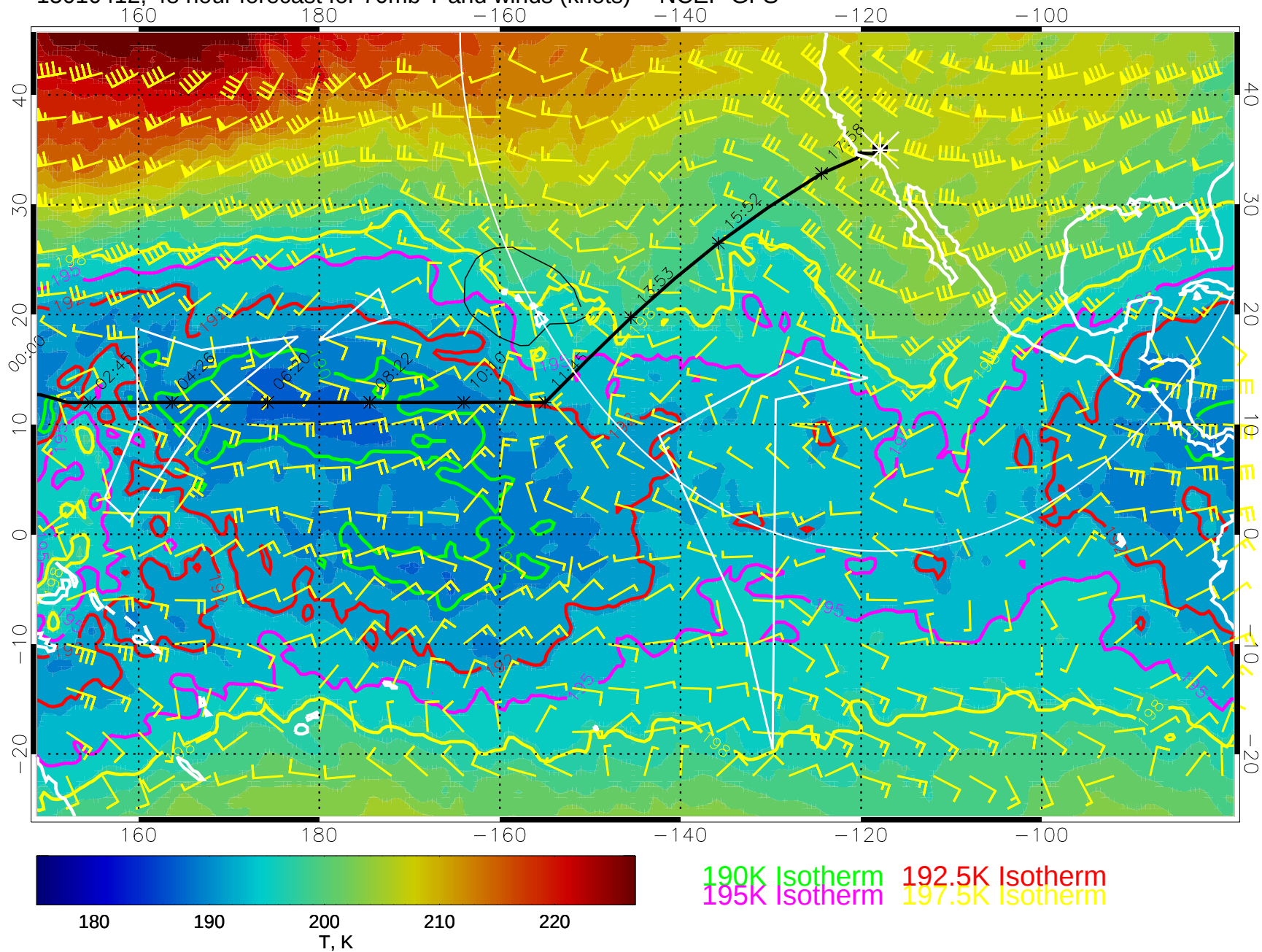
15010412, 48 hour forecast for 70mb T and winds (knots) -- NCEP GFS
