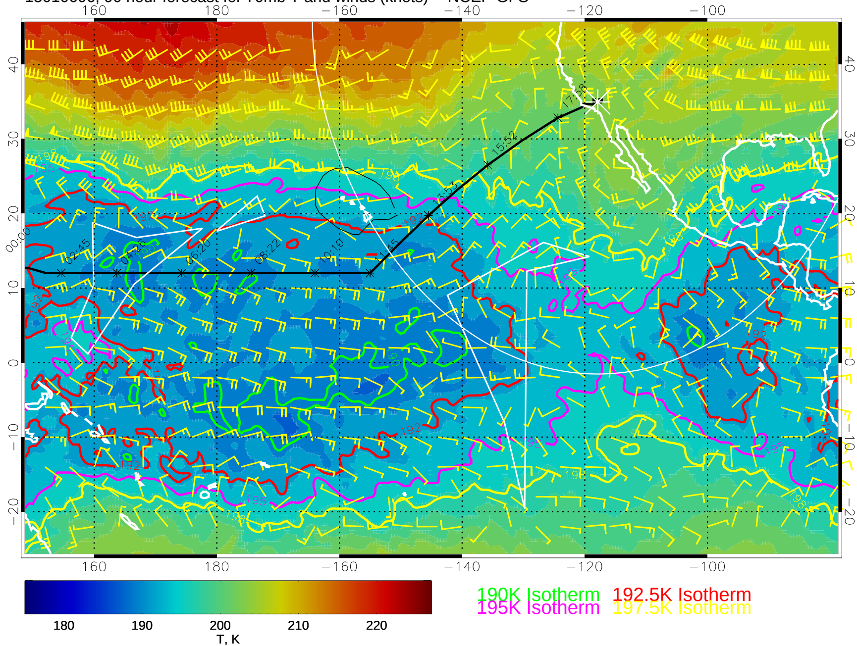
15010606, 90 hour forecast for 70mb T and winds (knots) -- NCEP GFS
