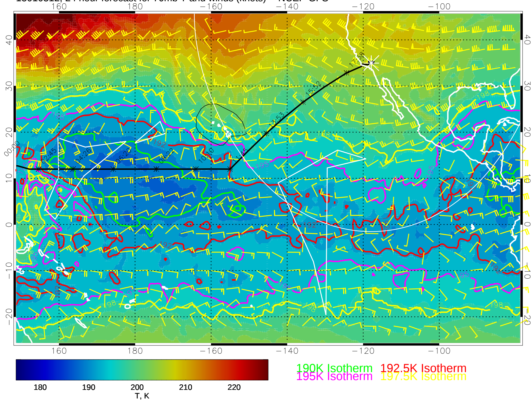
15010312, 24 hour forecast for 70mb T and winds (knots) -- NCEP GFS
