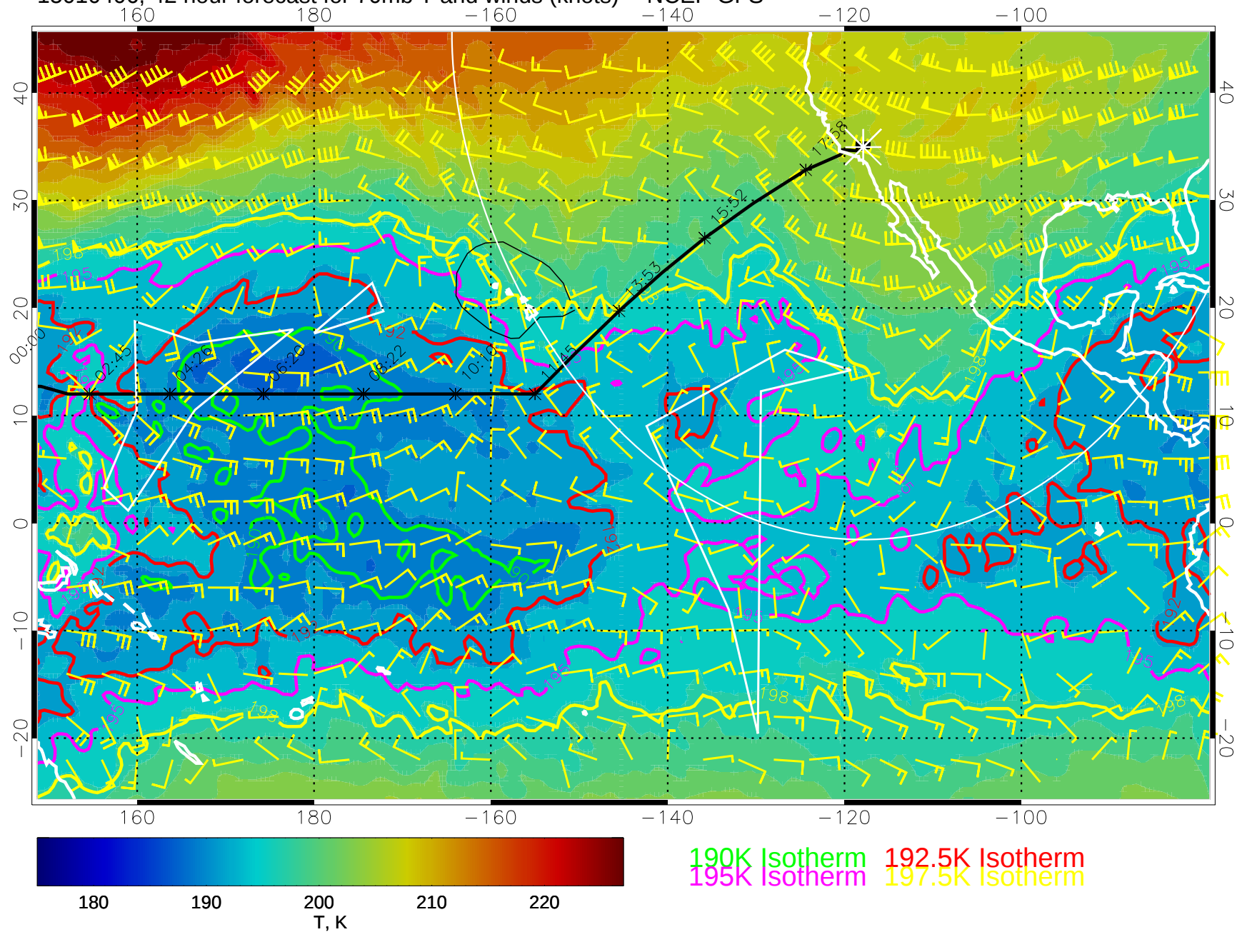
15010406, 42 hour forecast for 70mb T and winds (knots) -- NCEP GFS
