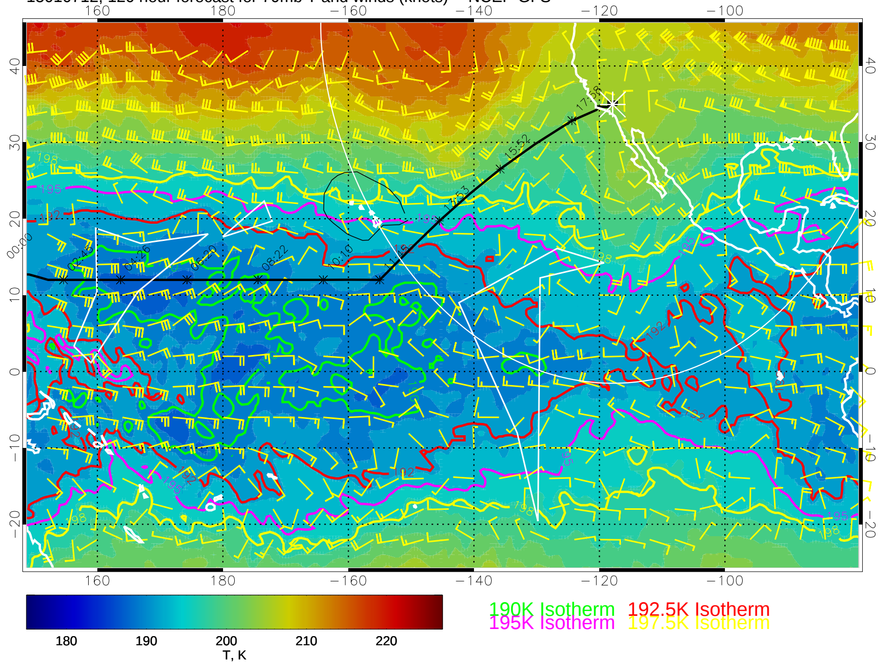
15010712, 120 hour forecast for 70mb T and winds (knots) -- NCEP GFS
