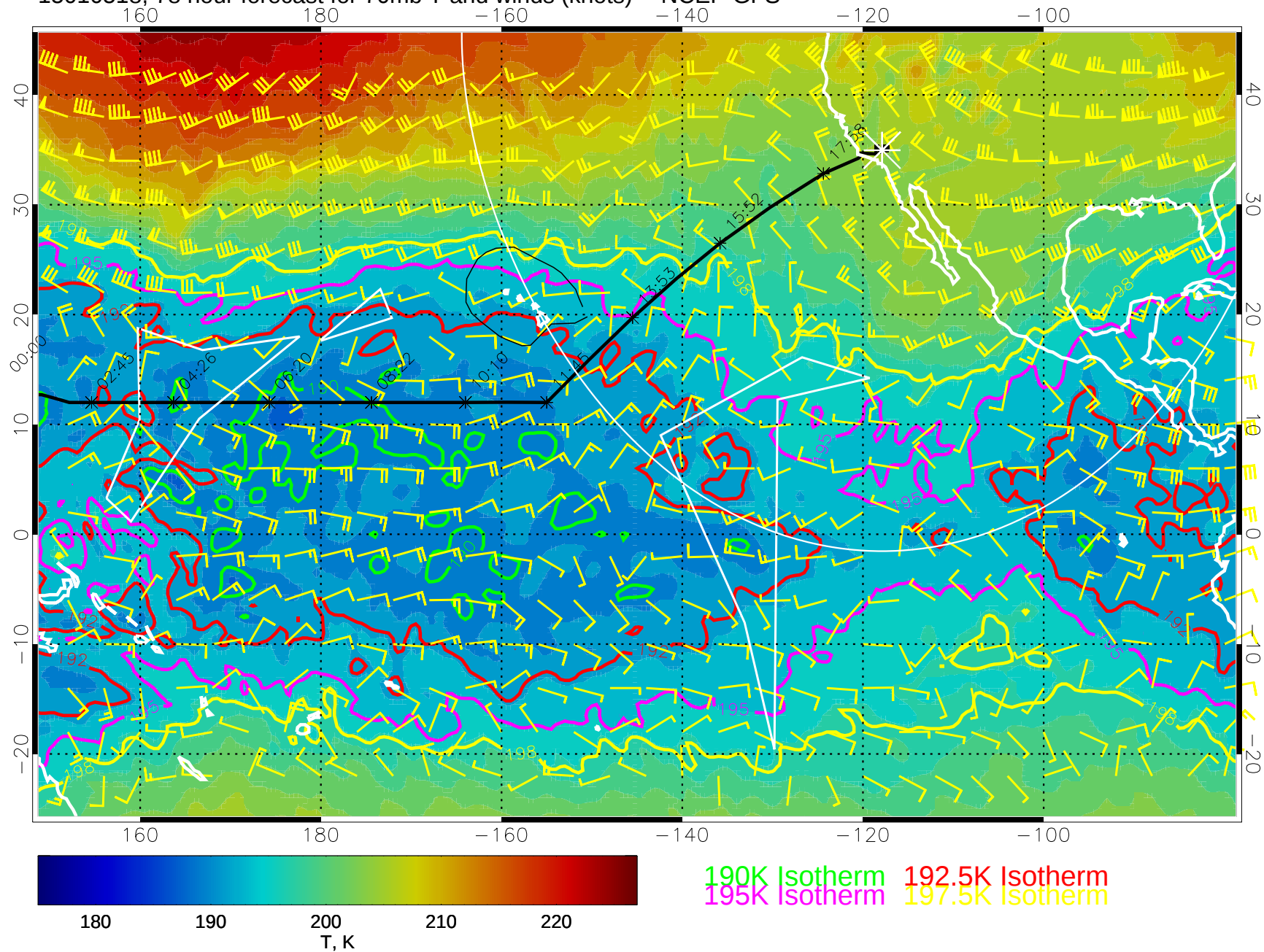
15010518, 78 hour forecast for 70mb T and winds (knots) -- NCEP GFS
