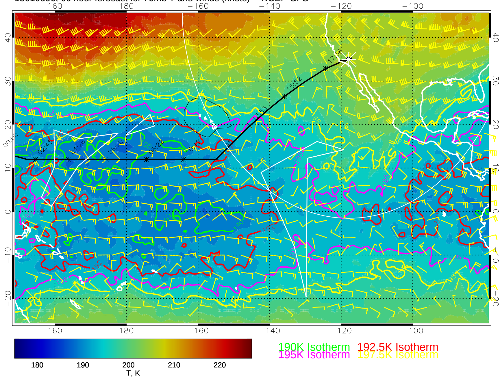
15010506, 66 hour forecast for 70mb T and winds (knots) -- NCEP GFS
