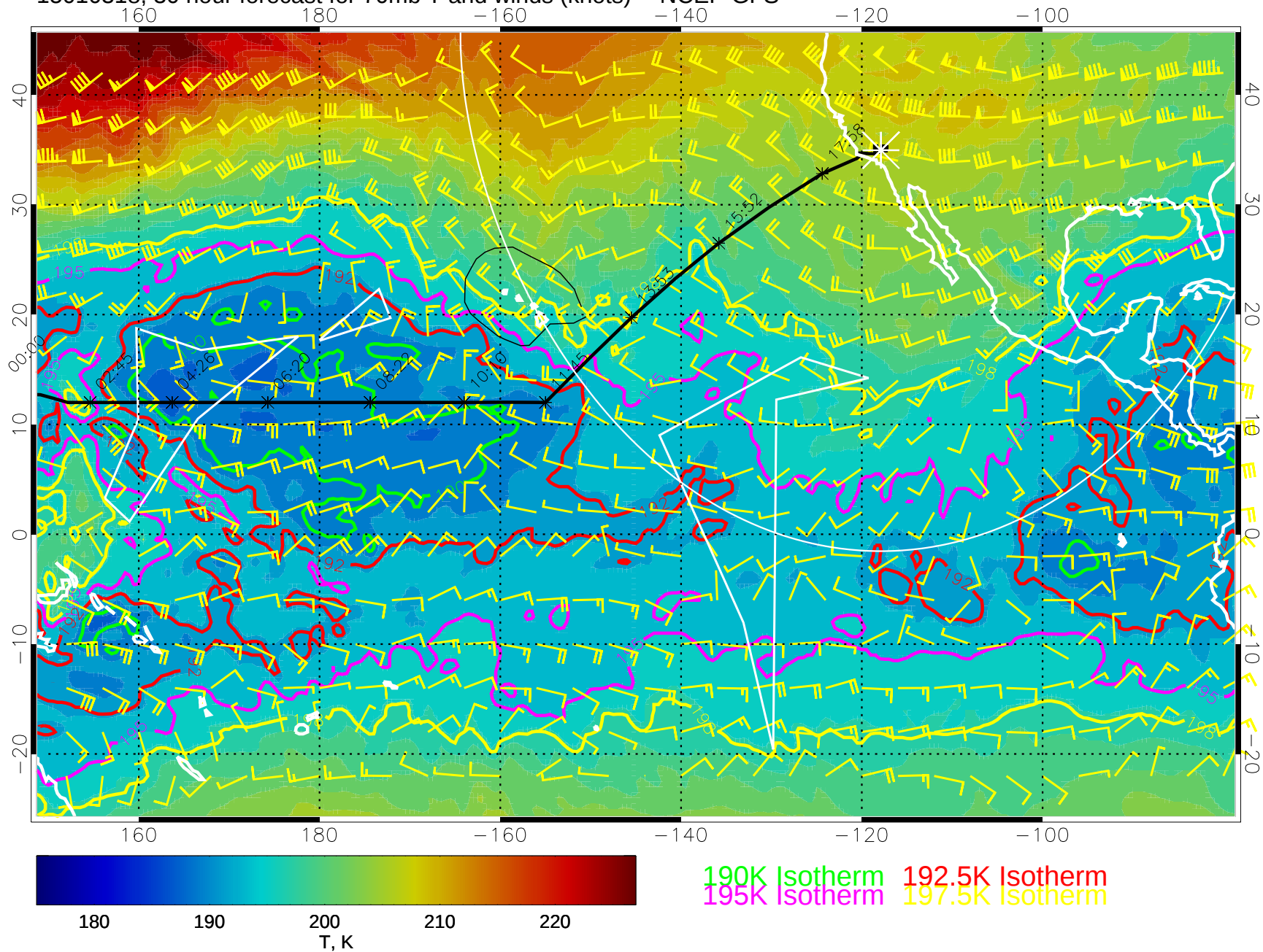
15010318, 30 hour forecast for 70mb T and winds (knots) -- NCEP GFS
