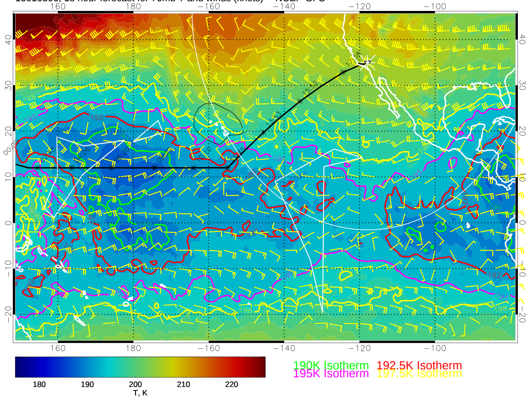
15010306, 18 hour forecast for 70mb T and winds (knots) -- NCEP GFS
