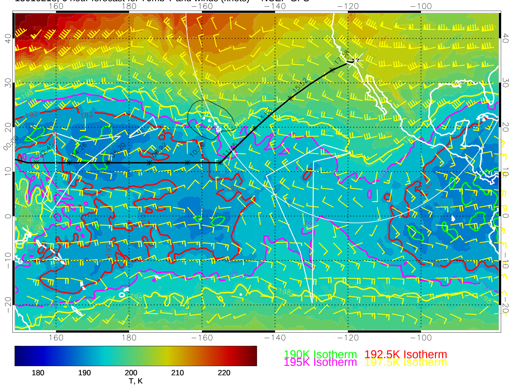
15010218, 6 hour forecast for 70mb T and winds (knots) -- NCEP GFS
