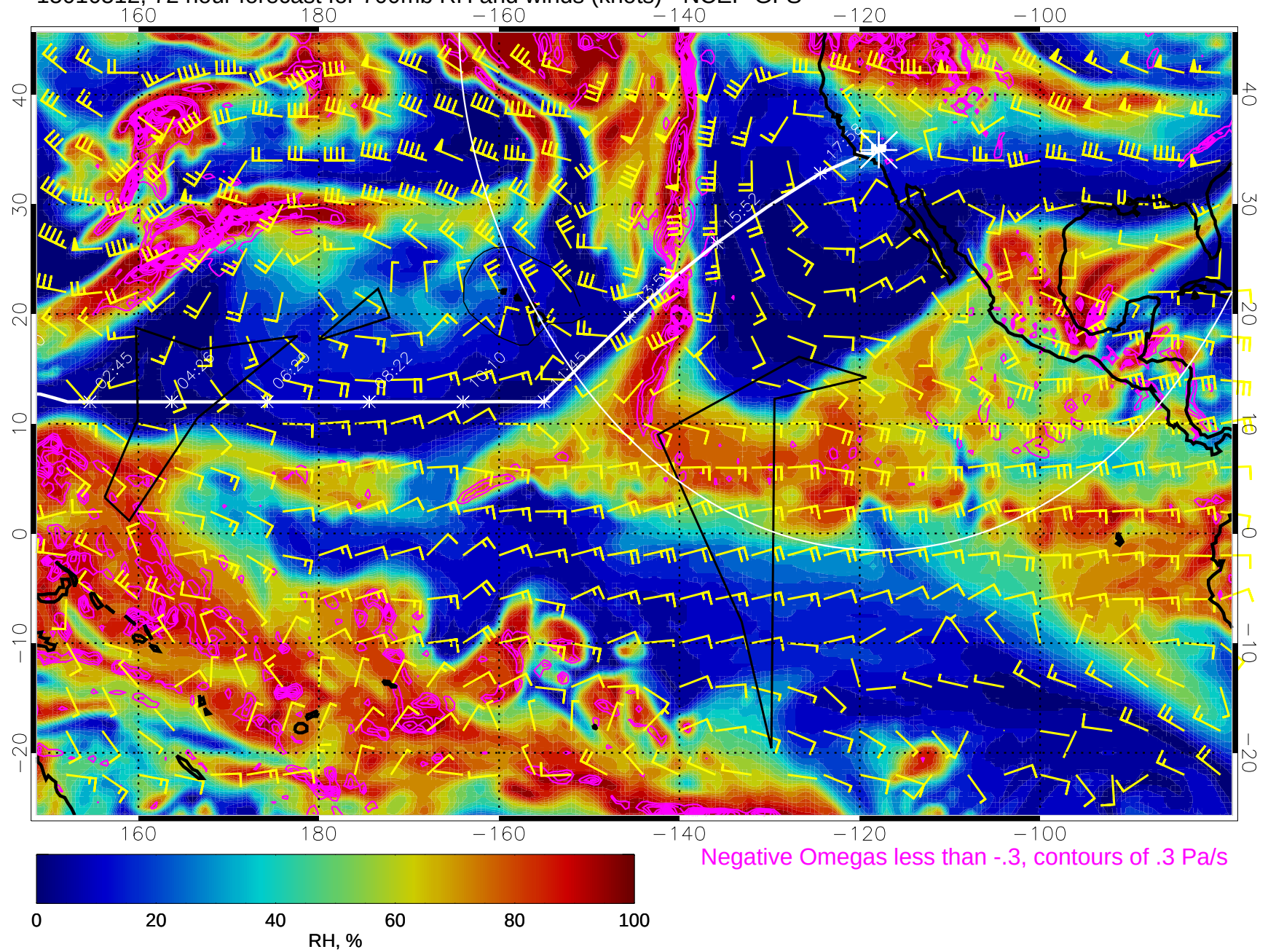
15010512, 72 hour forecast for 700mb RH and winds (knots) - NCEP GFS
