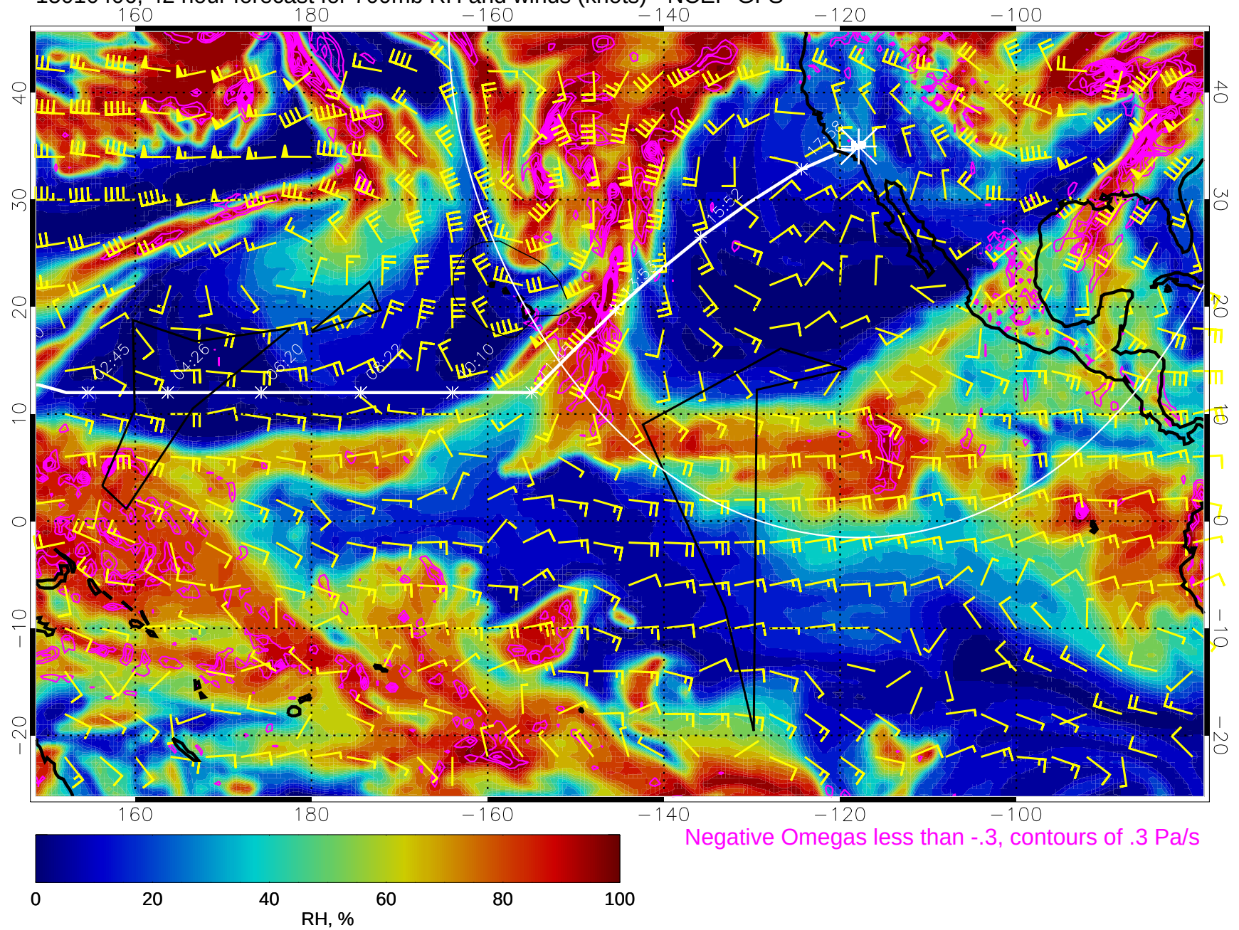
15010406, 42 hour forecast for 700mb RH and winds (knots) - NCEP GFS
