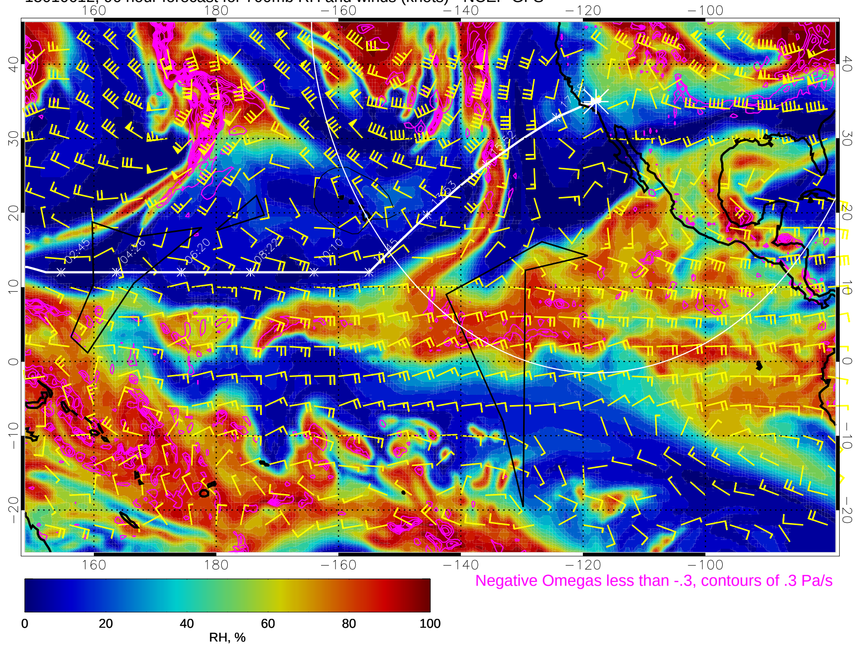
15010612, 96 hour forecast for 700mb RH and winds (knots) - NCEP GFS
