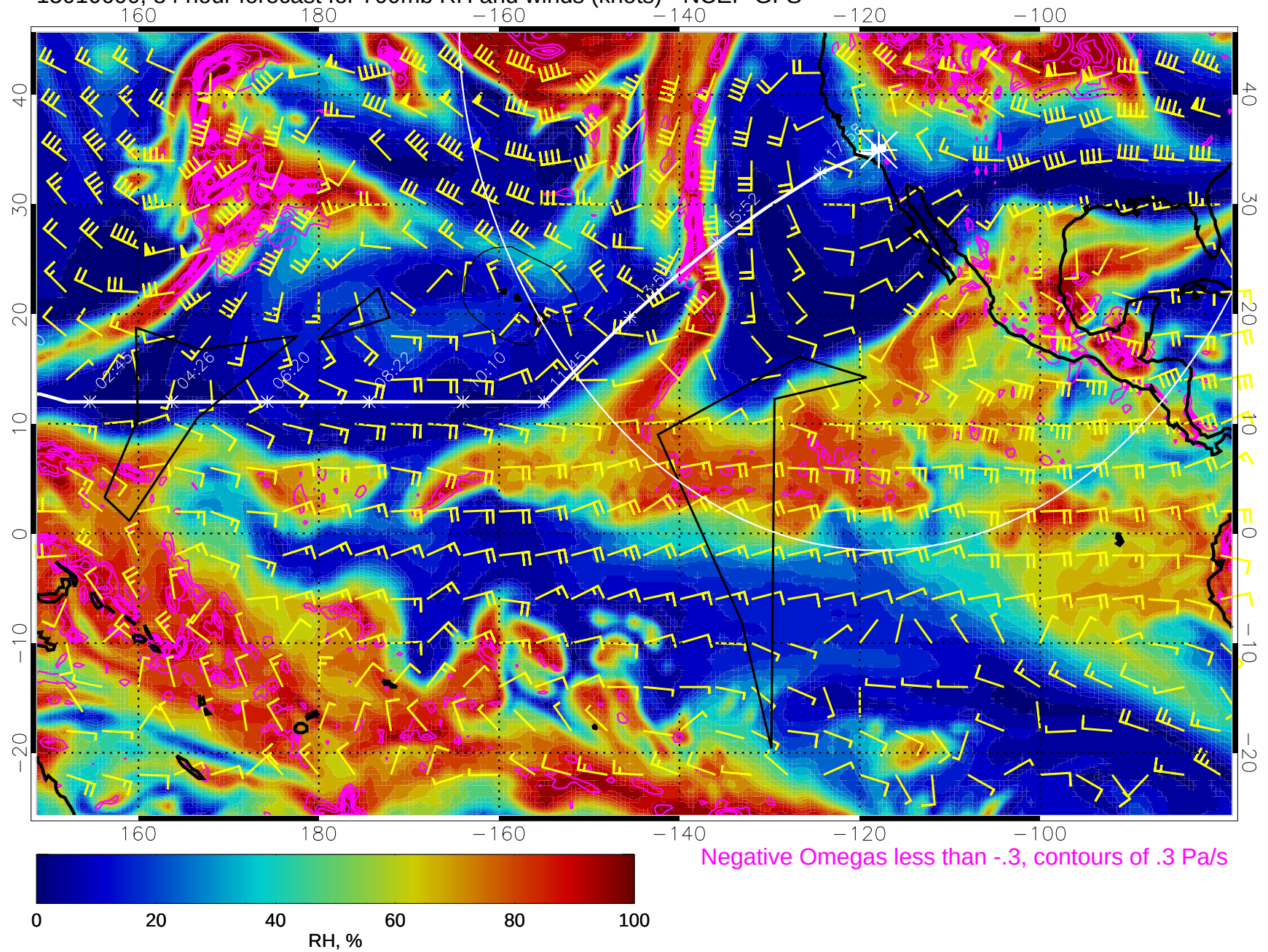
15010600, 84 hour forecast for 700mb RH and winds (knots) - NCEP GFS
