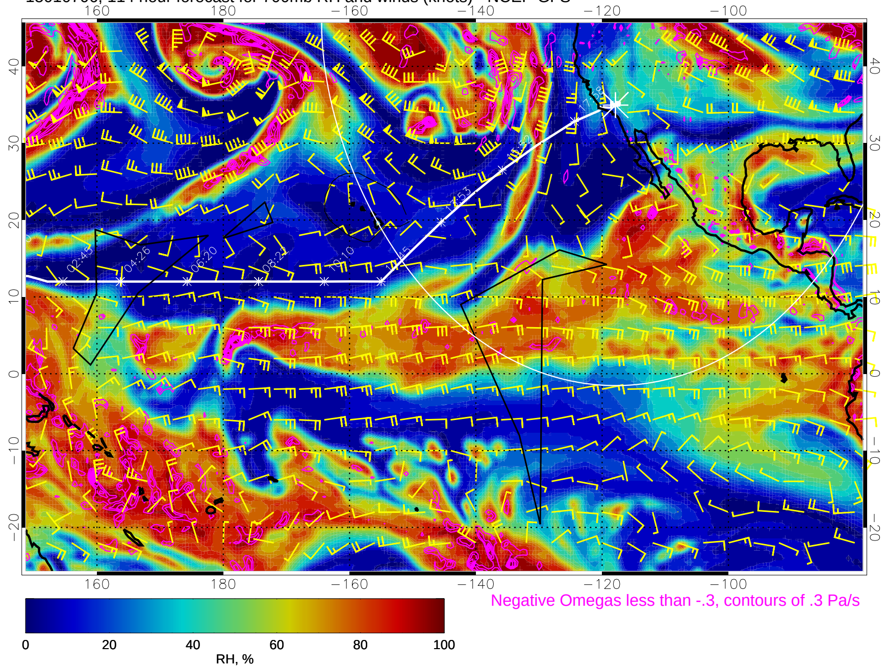
15010706, 114 hour forecast for 700mb RH and winds (knots) - NCEP GFS
