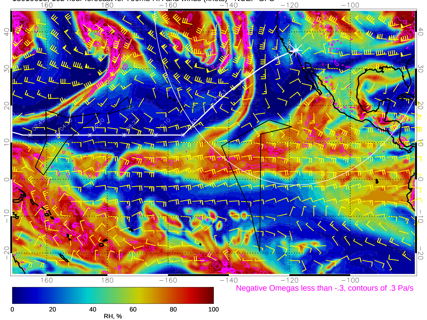
15010618, 102 hour forecast for 700mb RH and winds (knots) - NCEP GFS
