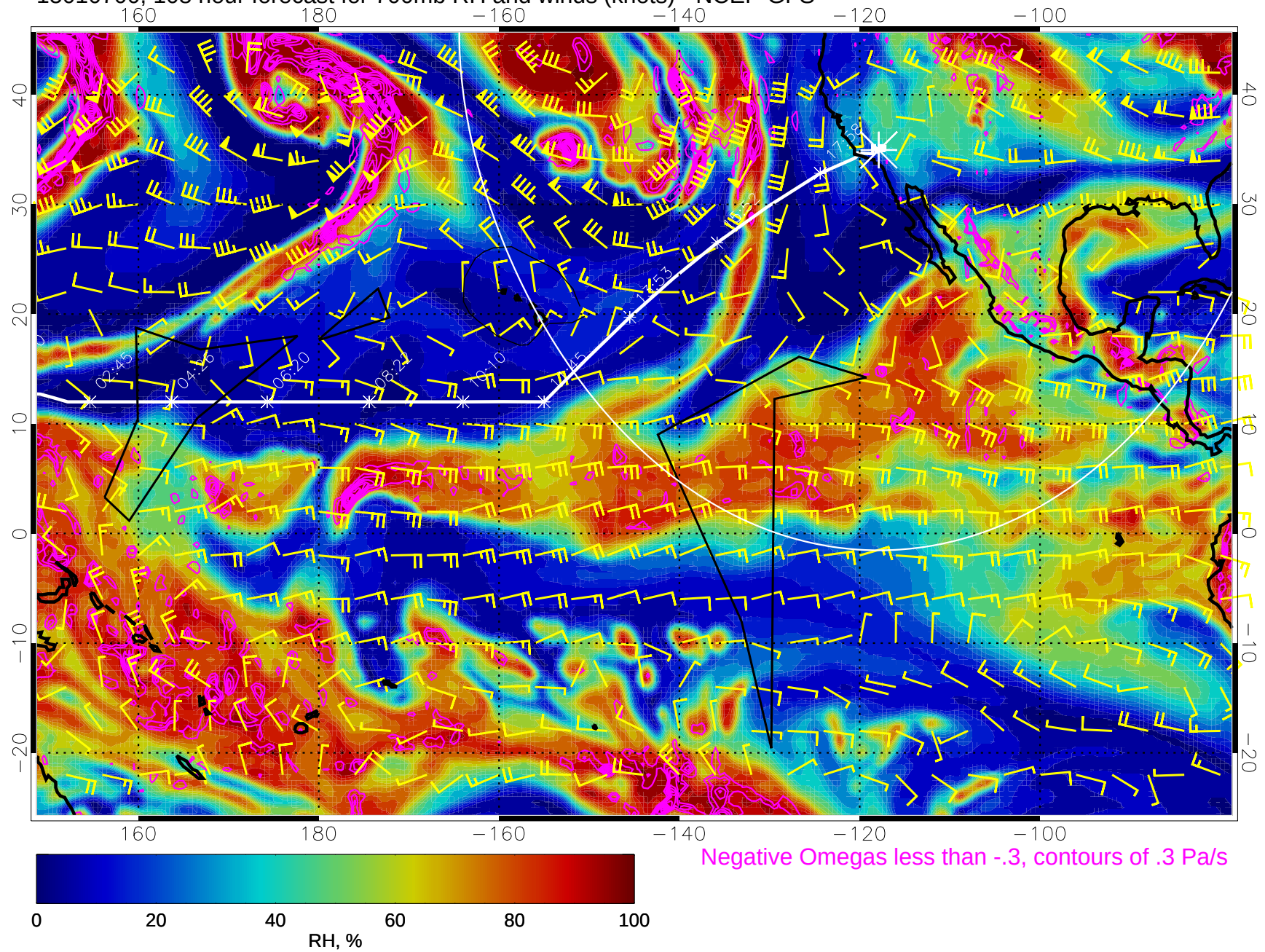
15010700, 108 hour forecast for 700mb RH and winds (knots) - NCEP GFS
