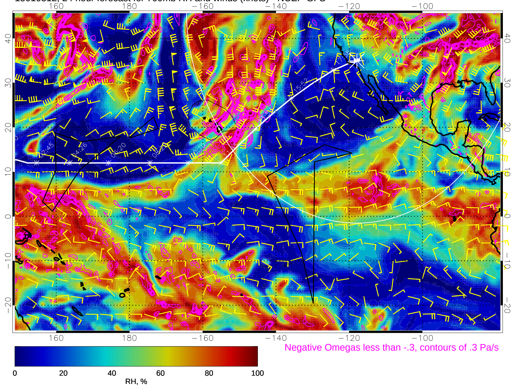
15010312, 24 hour forecast for 700mb RH and winds (knots) - NCEP GFS
