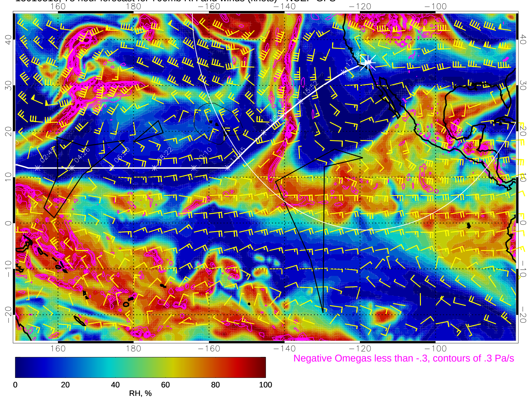
15010518, 78 hour forecast for 700mb RH and winds (knots) - NCEP GFS
