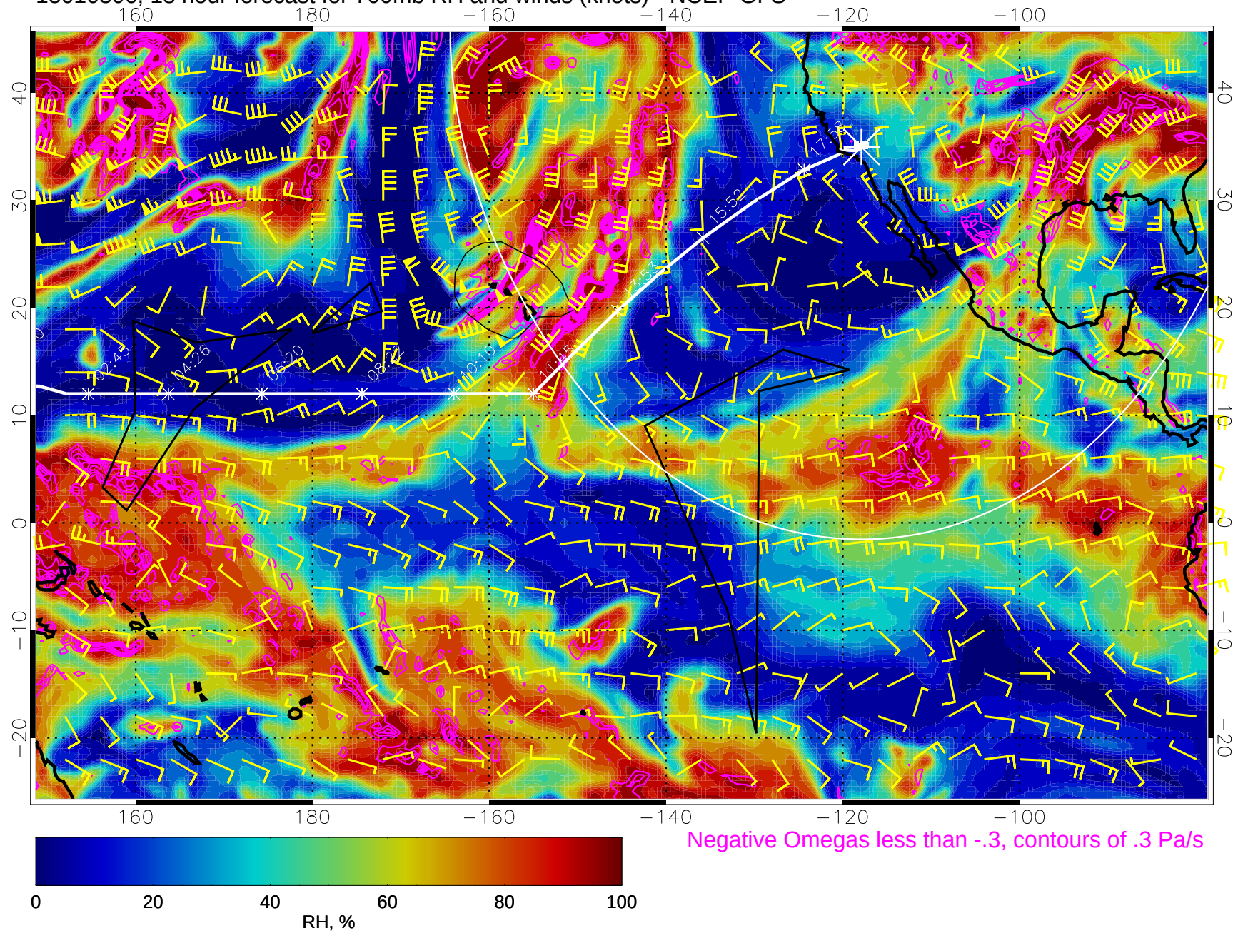
15010306, 18 hour forecast for 700mb RH and winds (knots) - NCEP GFS
