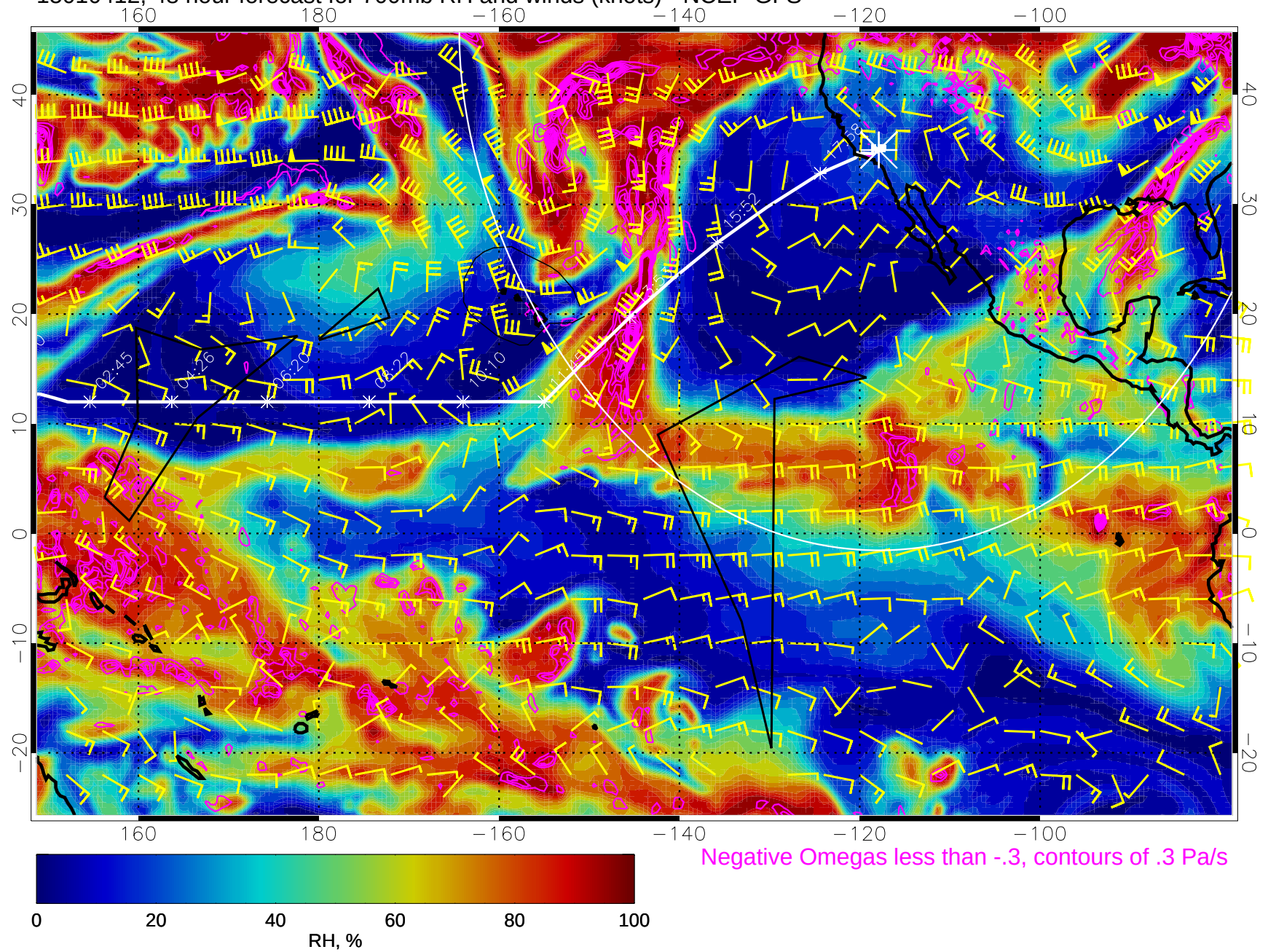
15010412, 48 hour forecast for 700mb RH and winds (knots) - NCEP GFS
