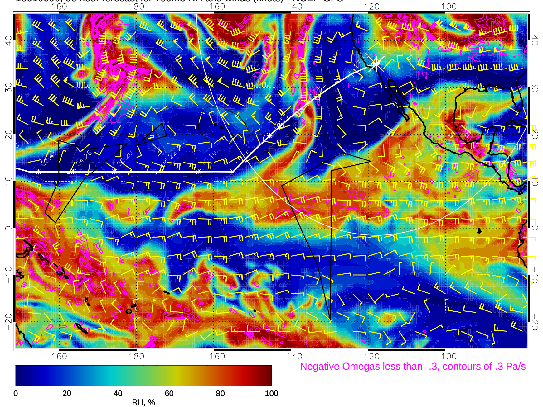
15010606, 90 hour forecast for 700mb RH and winds (knots) - NCEP GFS
