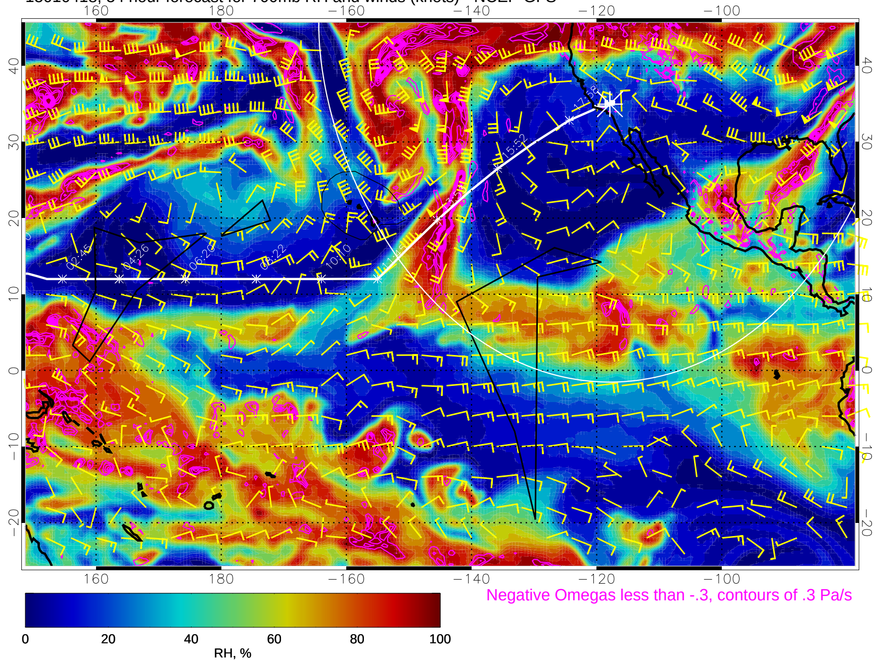
15010418, 54 hour forecast for 700mb RH and winds (knots) - NCEP GFS
