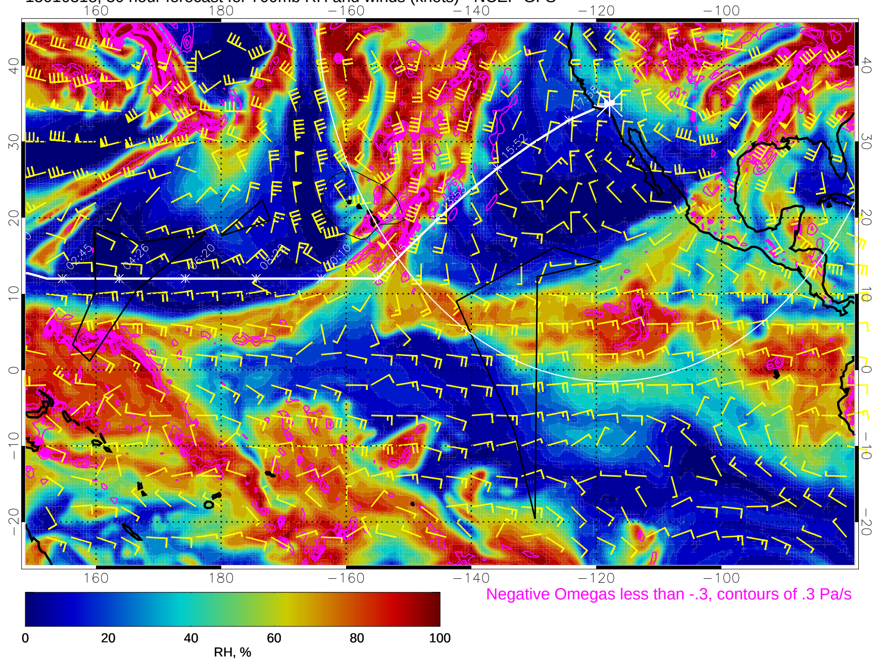
15010318, 30 hour forecast for 700mb RH and winds (knots) - NCEP GFS
