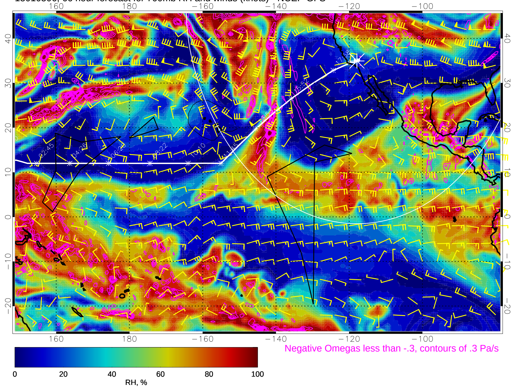
15010506, 66 hour forecast for 700mb RH and winds (knots) - NCEP GFS
