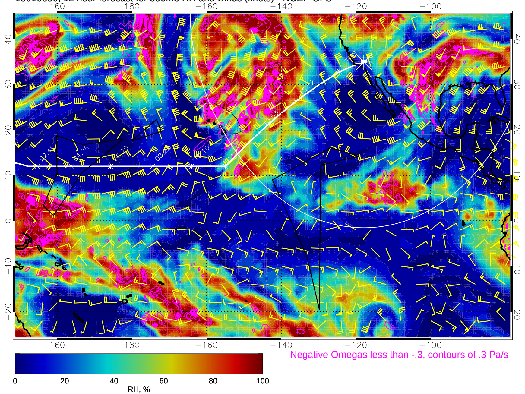
15010300, 12 hour forecast for 500mb RH and winds (knots) - NCEP GFS
