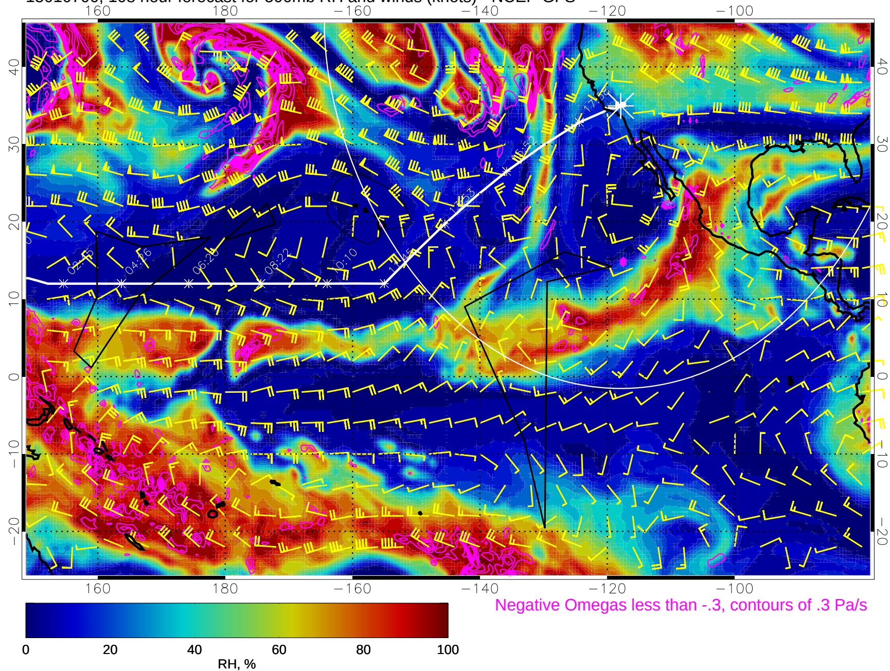
15010700, 108 hour forecast for 500mb RH and winds (knots) - NCEP GFS
