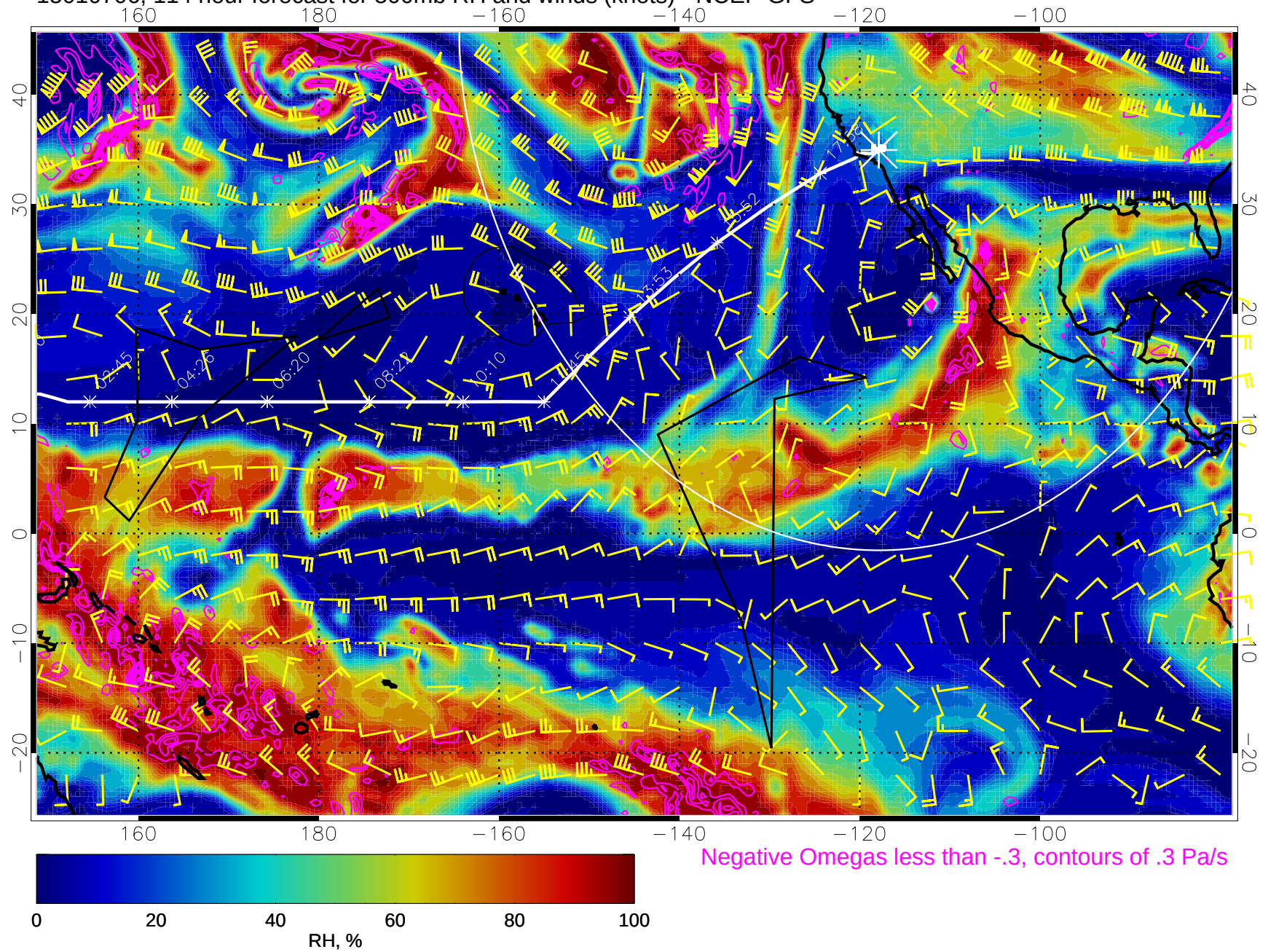
15010706, 114 hour forecast for 500mb RH and winds (knots) - NCEP GFS
