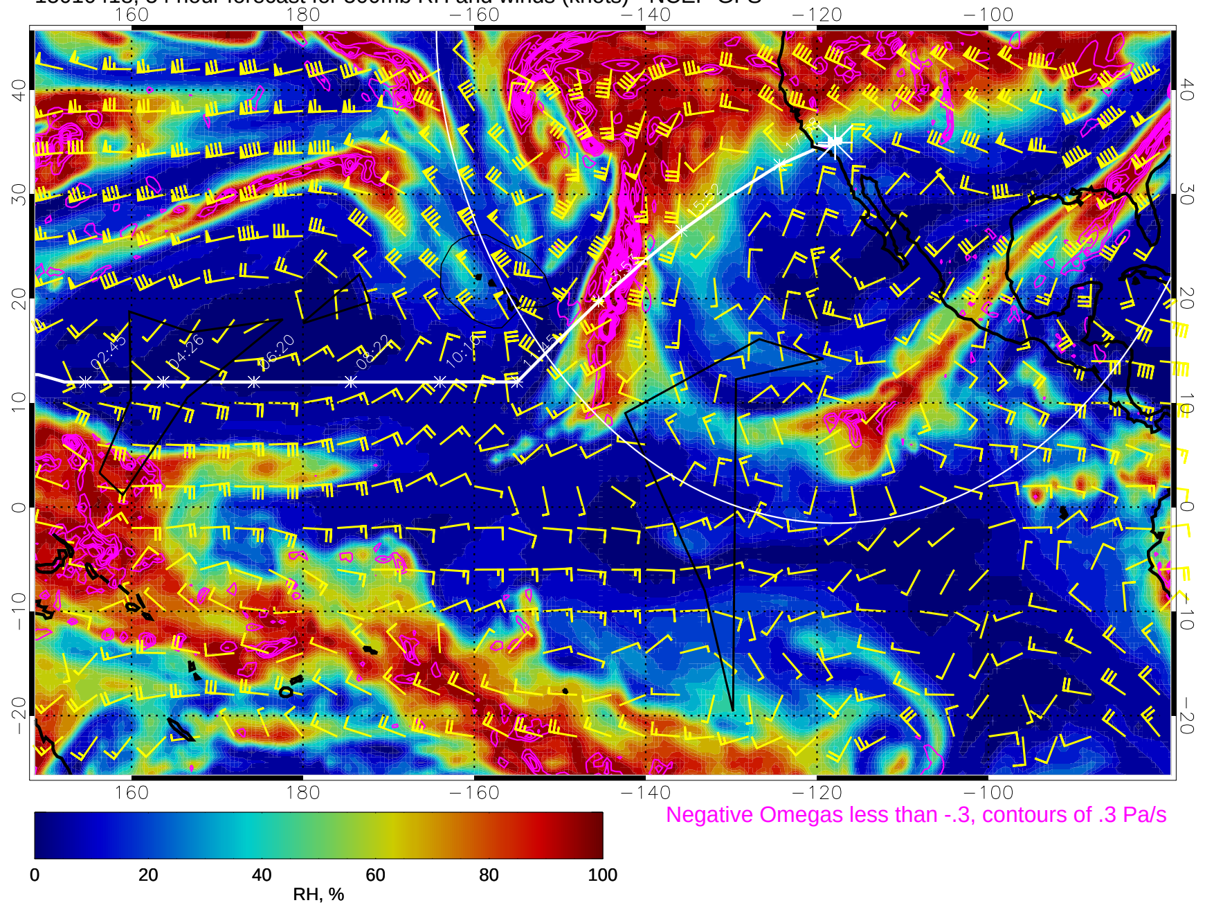
15010418, 54 hour forecast for 500mb RH and winds (knots) - NCEP GFS
