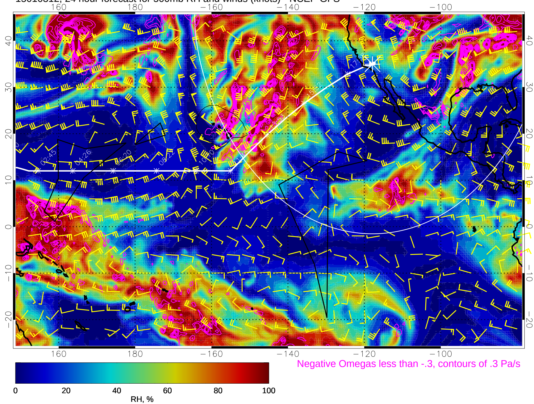
15010312, 24 hour forecast for 500mb RH and winds (knots) - NCEP GFS
