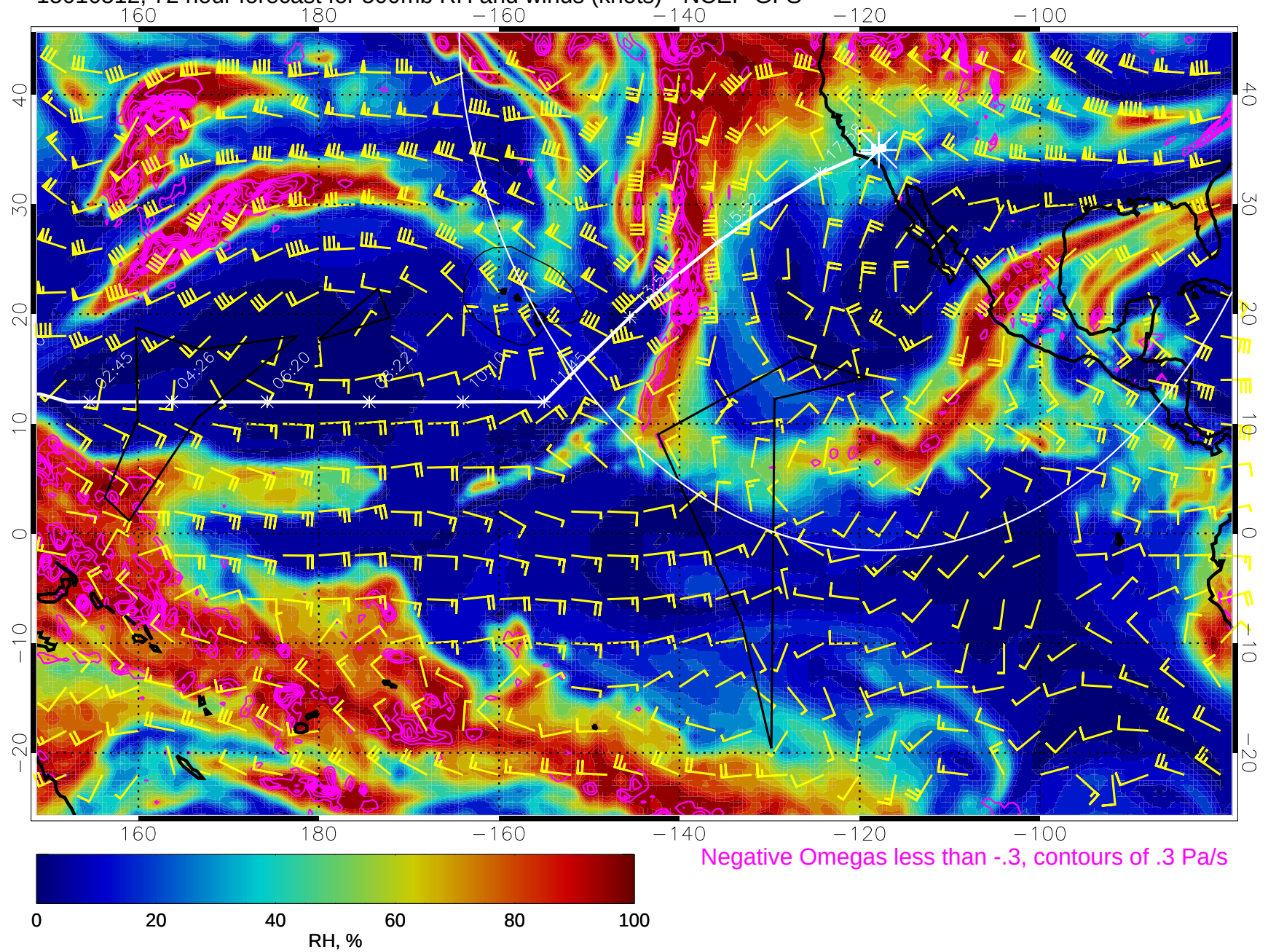
15010512, 72 hour forecast for 500mb RH and winds (knots) - NCEP GFS
