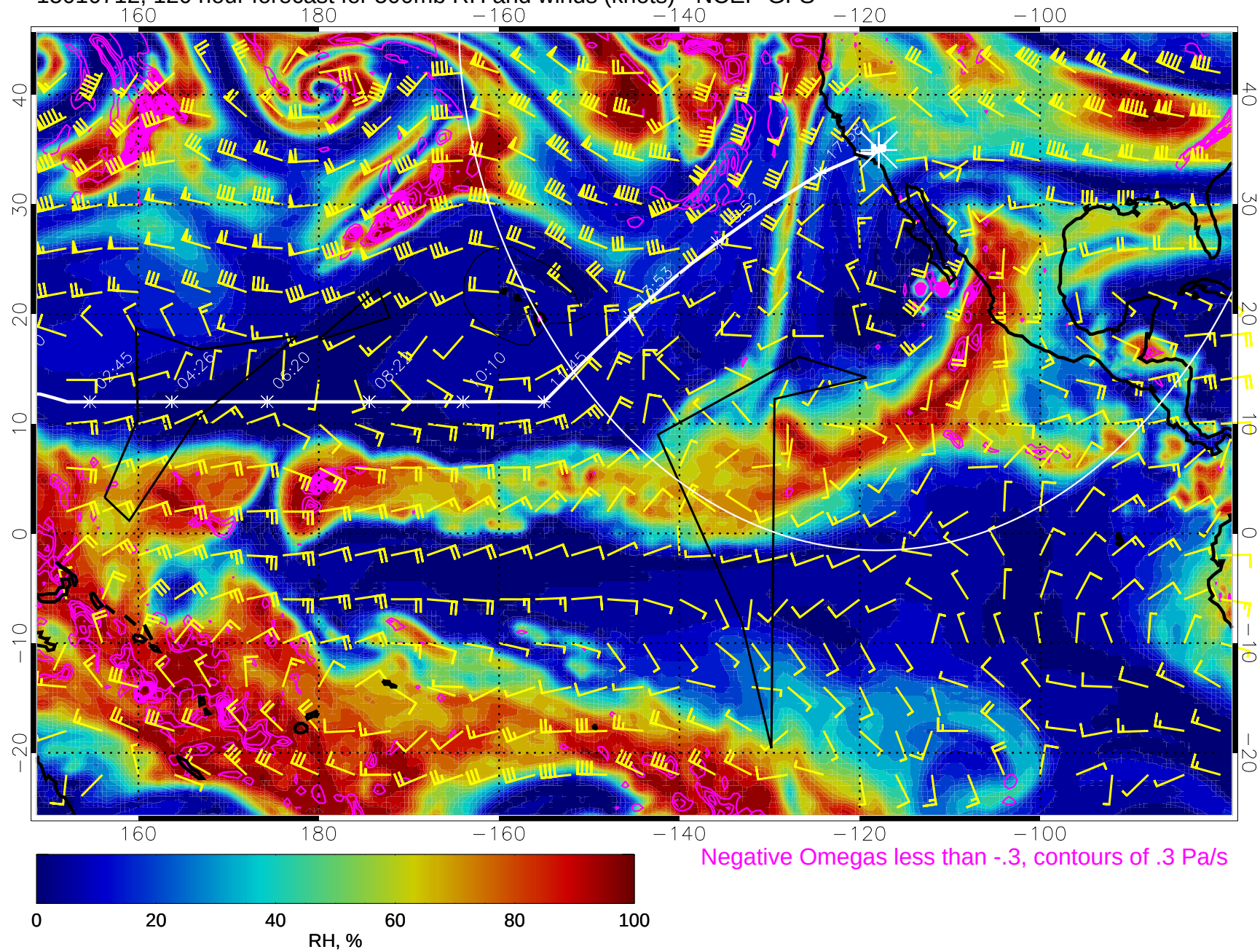
15010712, 120 hour forecast for 500mb RH and winds (knots) - NCEP GFS
