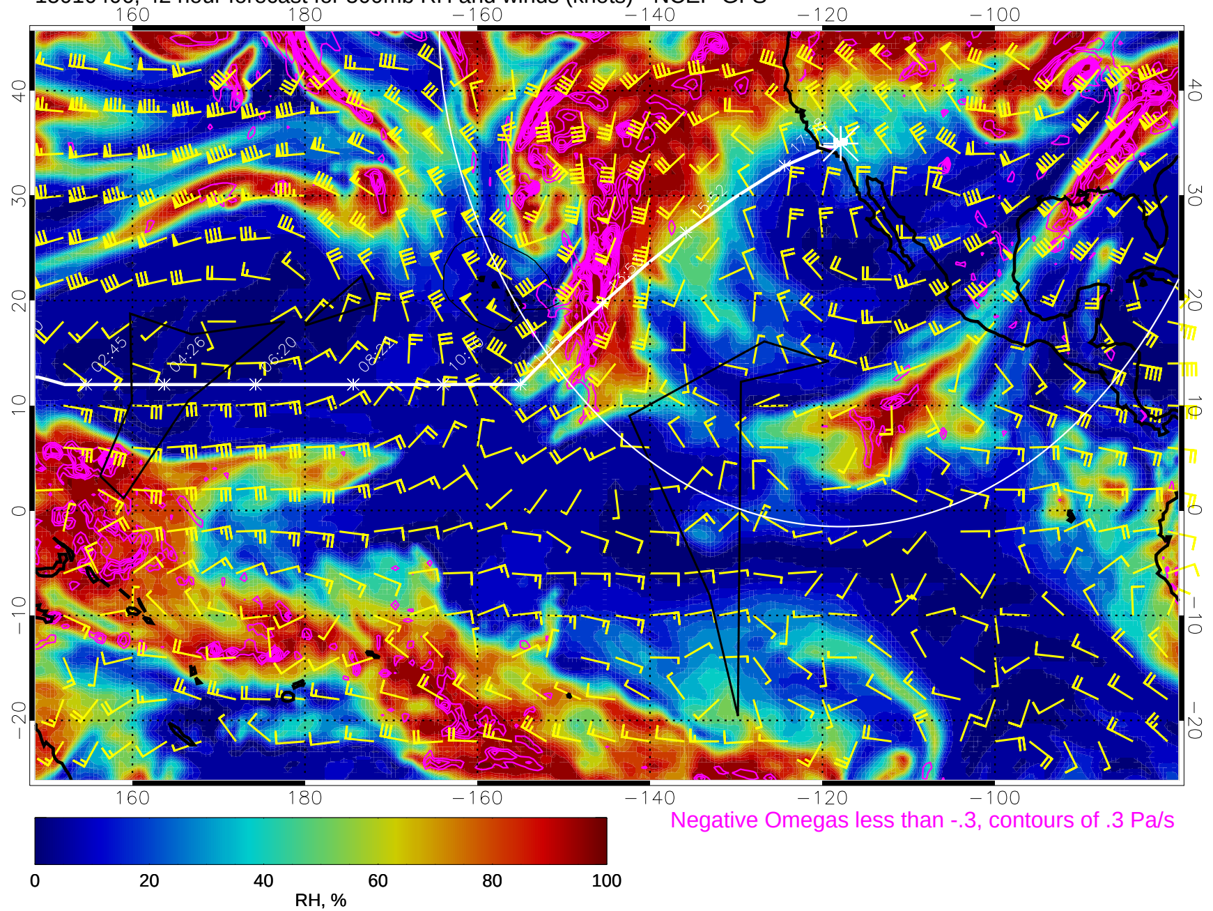
15010406, 42 hour forecast for 500mb RH and winds (knots) - NCEP GFS
