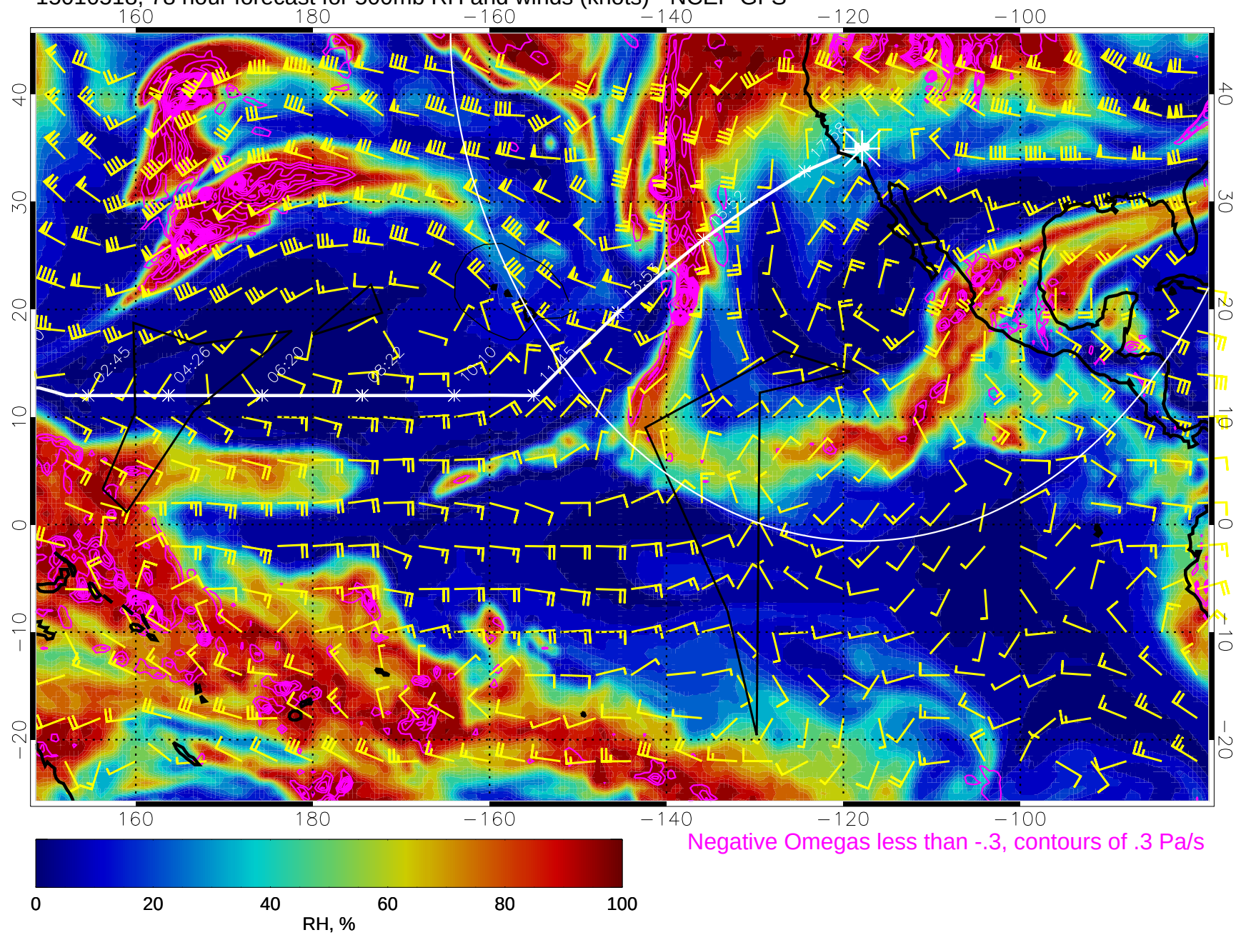
15010518, 78 hour forecast for 500mb RH and winds (knots) - NCEP GFS
