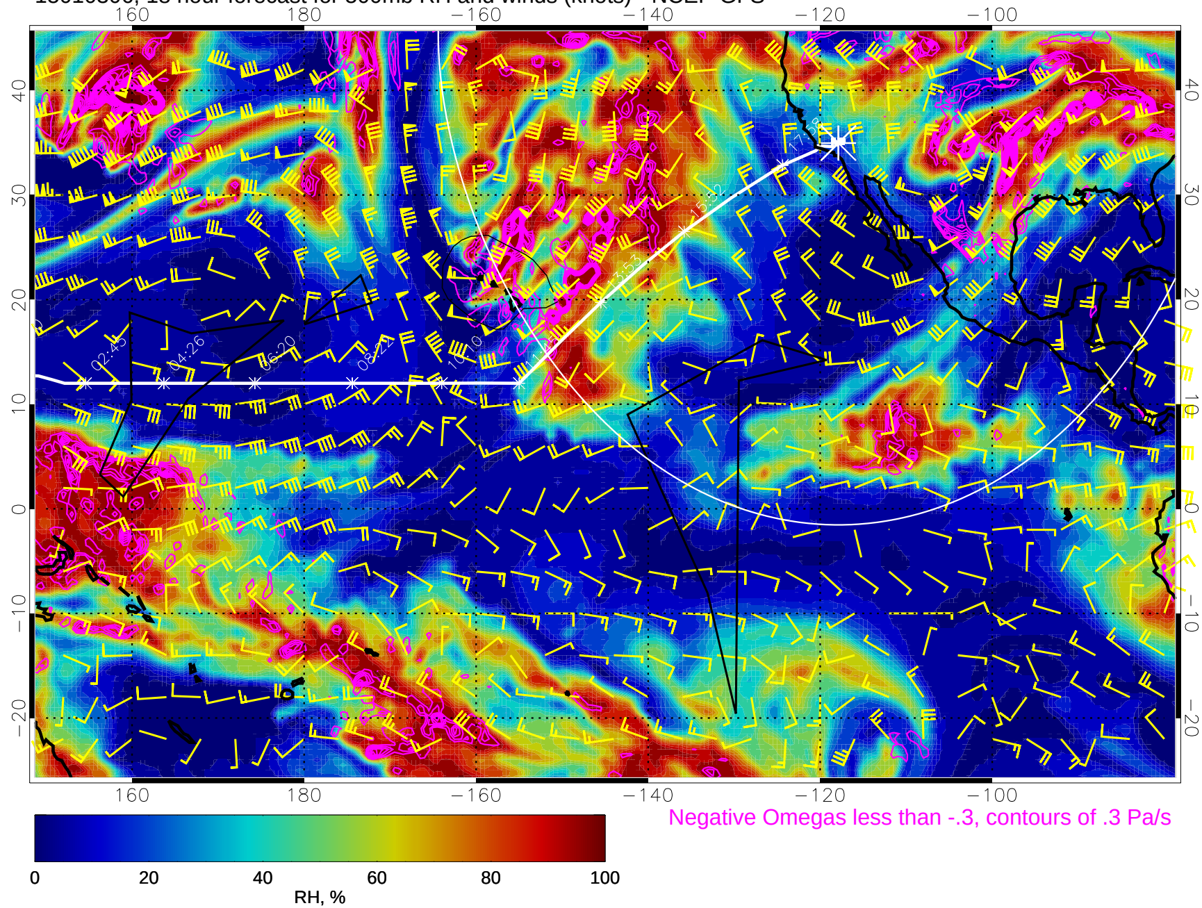
15010306, 18 hour forecast for 500mb RH and winds (knots) - NCEP GFS
