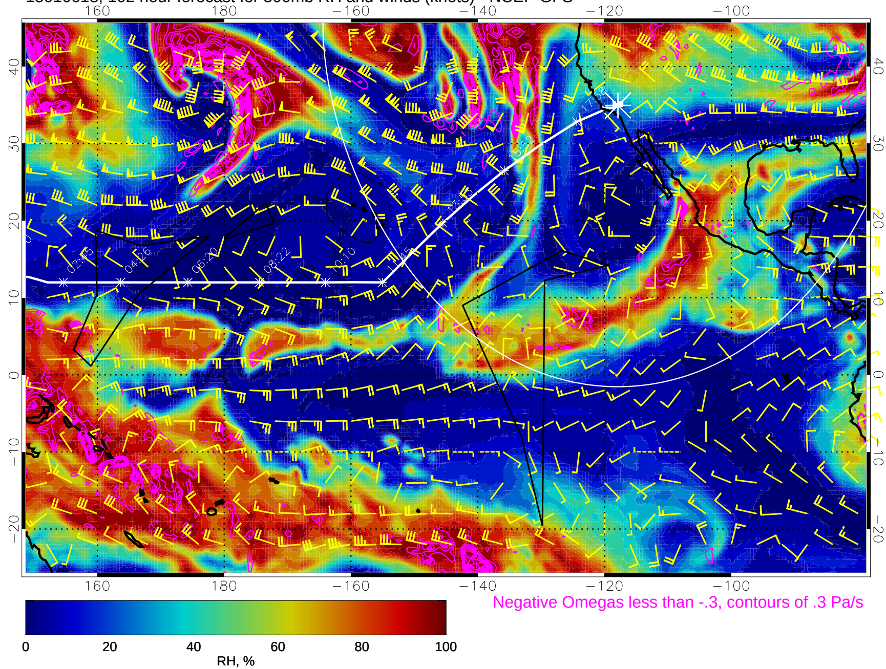
15010618, 102 hour forecast for 500mb RH and winds (knots) - NCEP GFS
