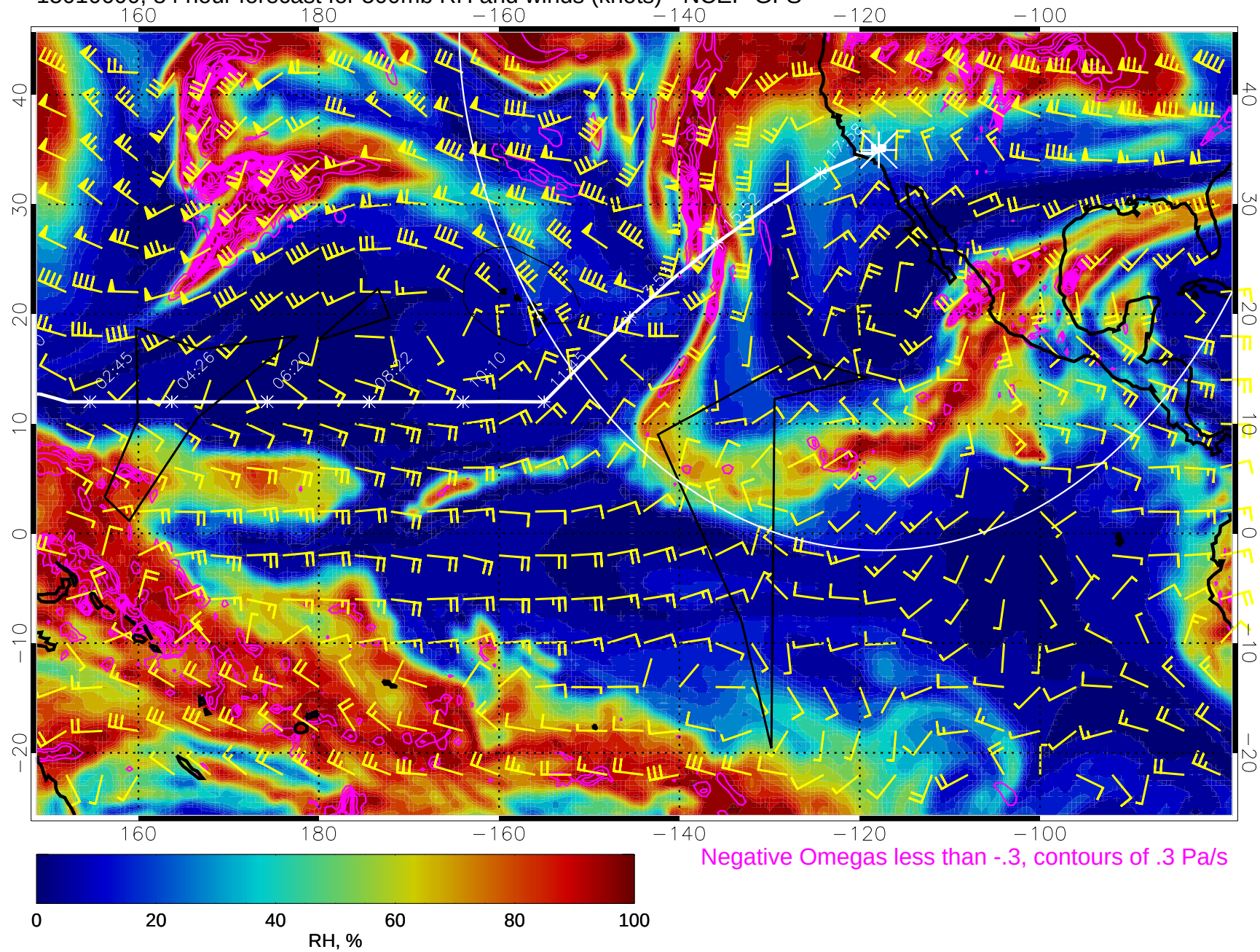
15010600, 84 hour forecast for 500mb RH and winds (knots) - NCEP GFS
