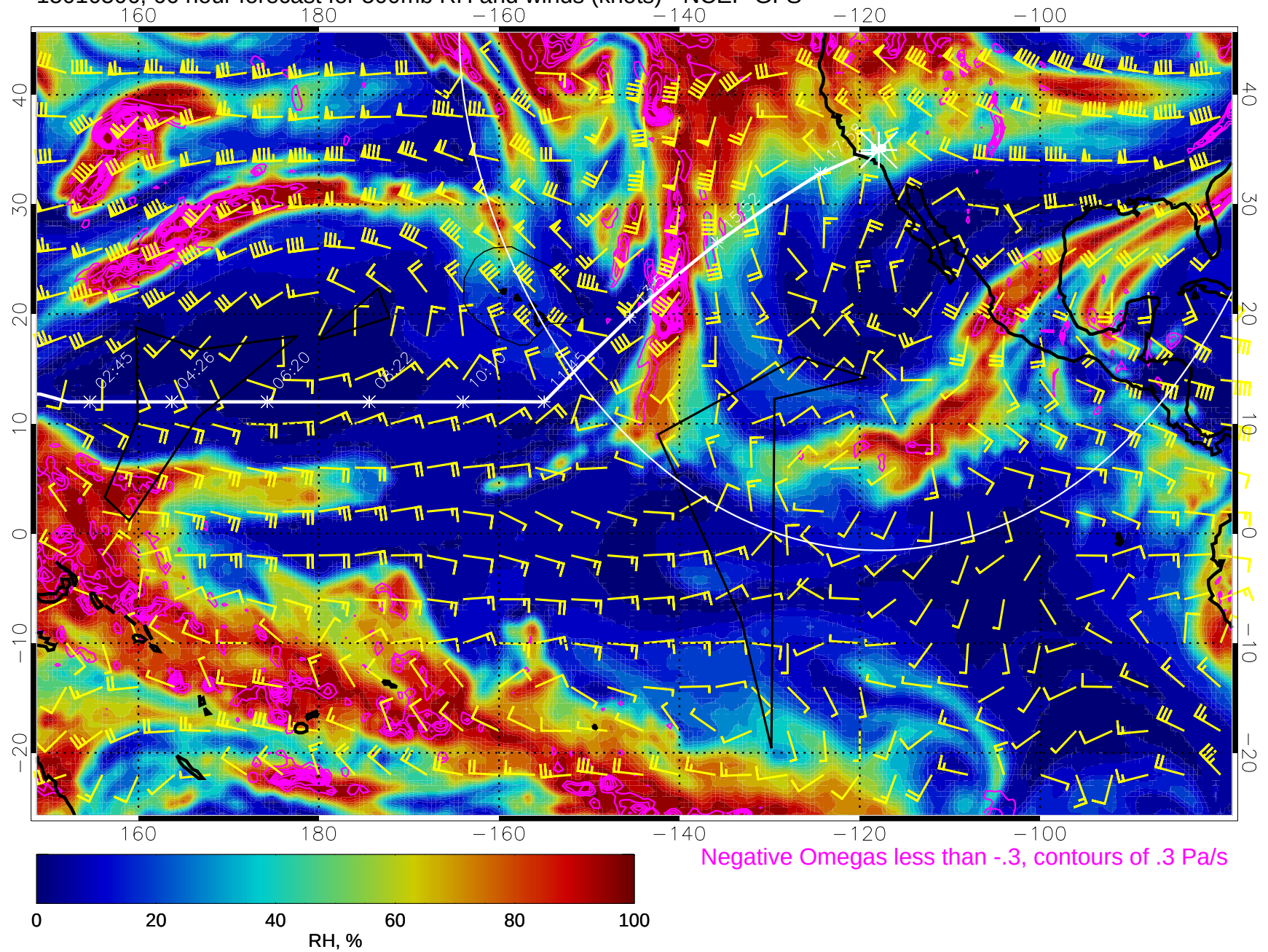
15010506, 66 hour forecast for 500mb RH and winds (knots) - NCEP GFS
