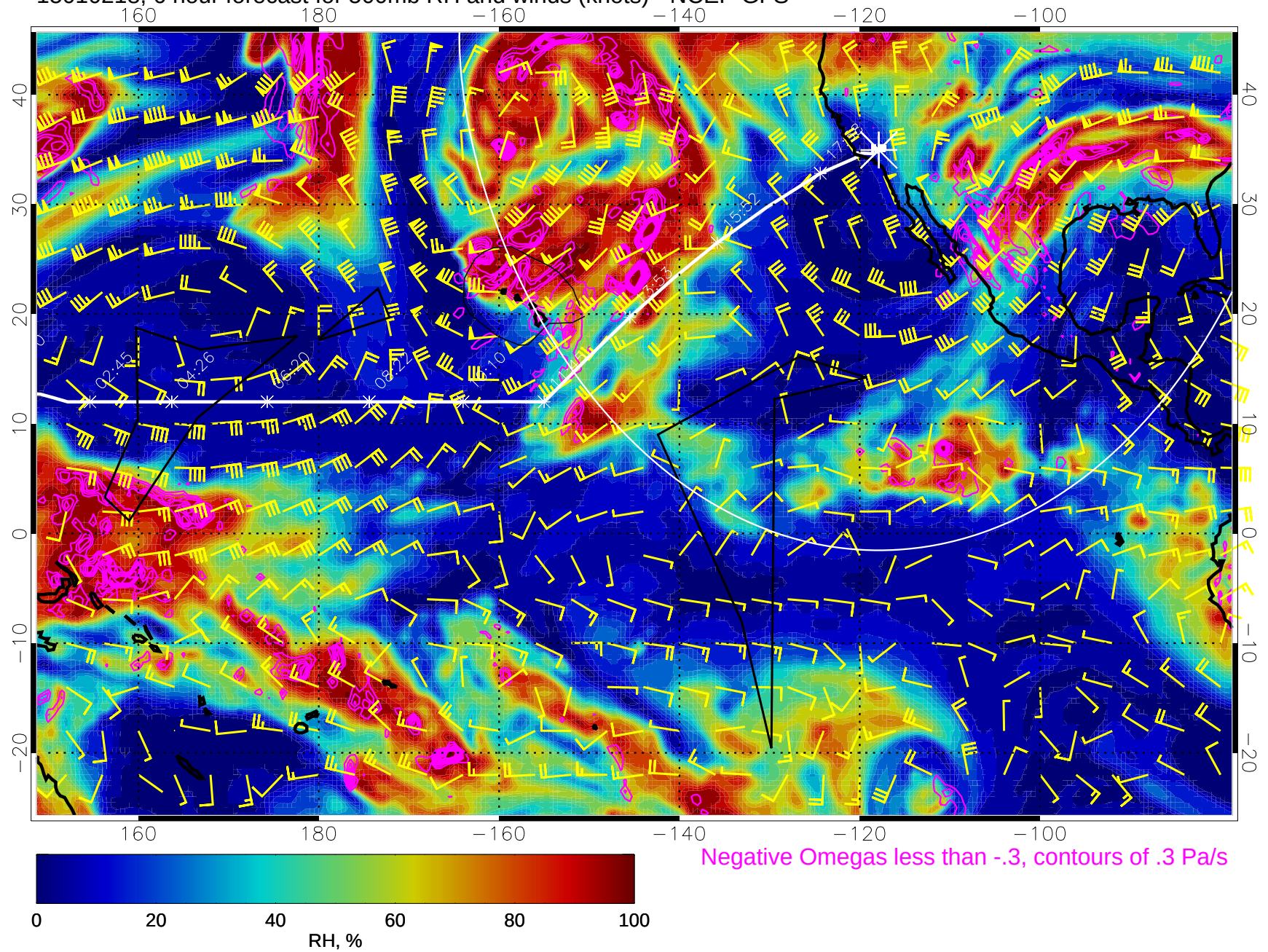
15010218, 6 hour forecast for 500mb RH and winds (knots) - NCEP GFS
