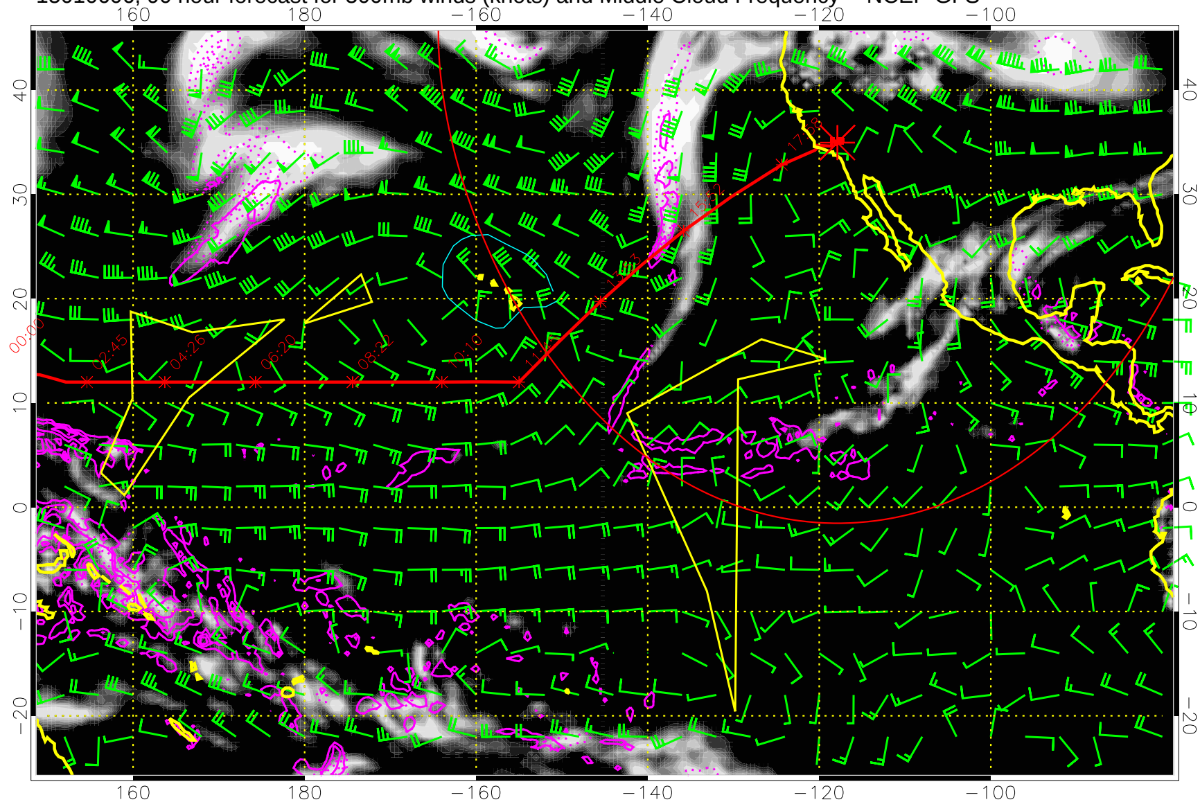
15010606, 90 hour forecast for 500mb winds (knots) and Middle Cloud Frequency -- NCEP GFS
