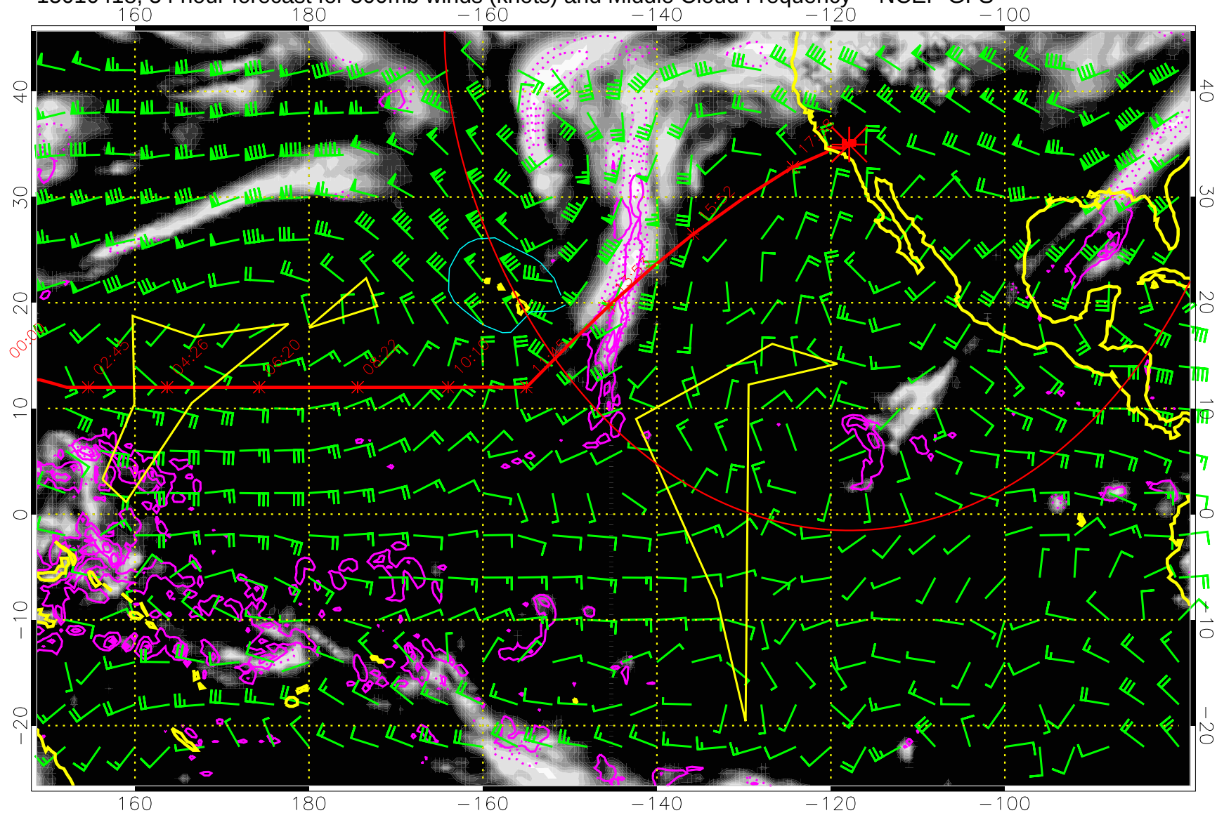
15010418, 54 hour forecast for 500mb winds (knots) and Middle Cloud Frequency -- NCEP GFS
