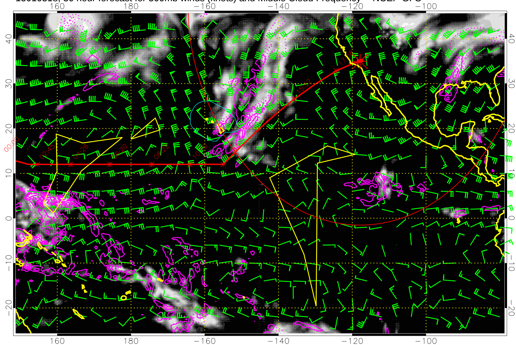
15010318, 30 hour forecast for 500mb winds (knots) and Middle Cloud Frequency -- NCEP GFS
