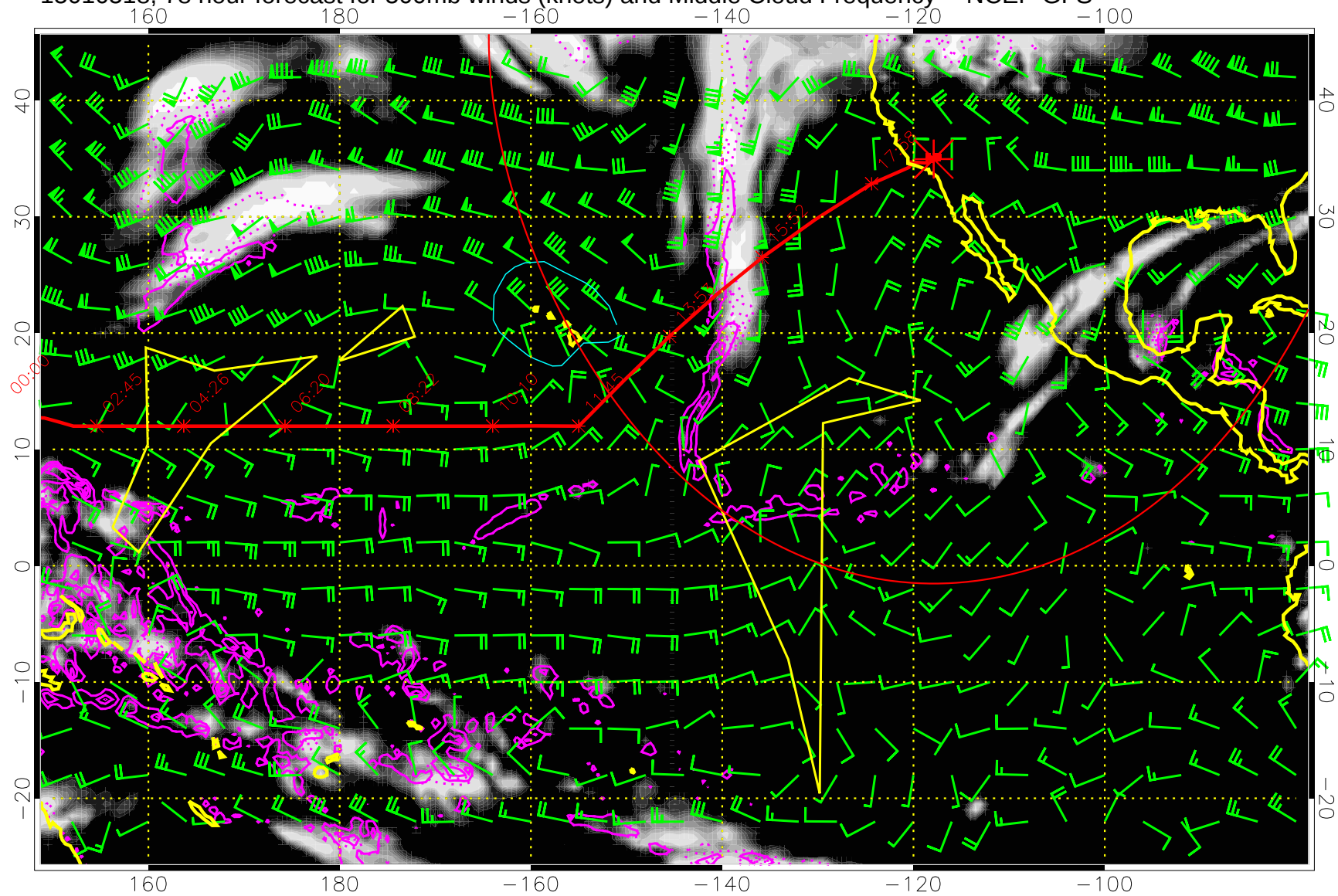
15010518, 78 hour forecast for 500mb winds (knots) and Middle Cloud Frequency -- NCEP GFS
