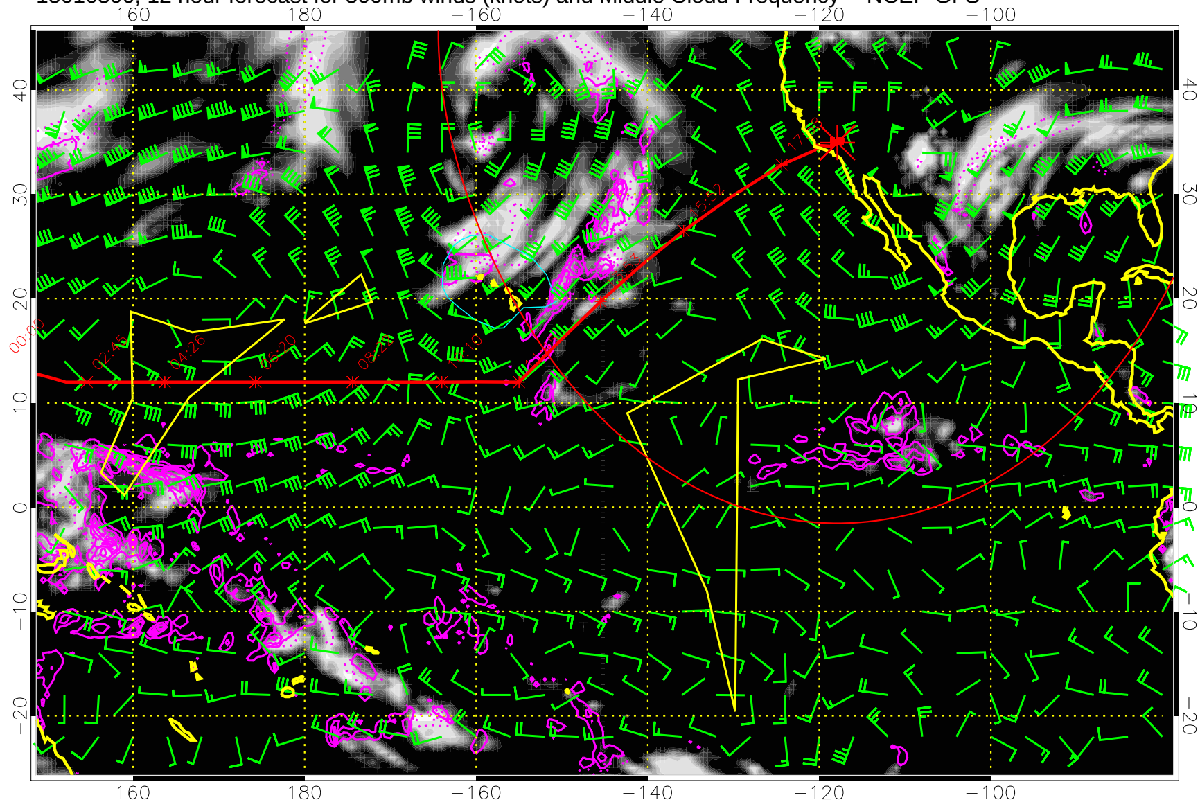
15010300, 12 hour forecast for 500mb winds (knots) and Middle Cloud Frequency -- NCEP GFS
