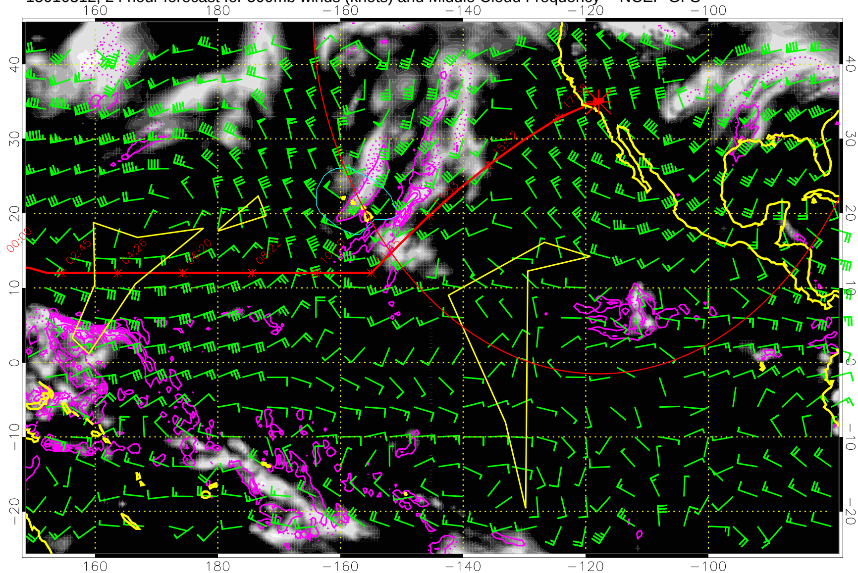
15010312, 24 hour forecast for 500mb winds (knots) and Middle Cloud Frequency -- NCEP GFS
