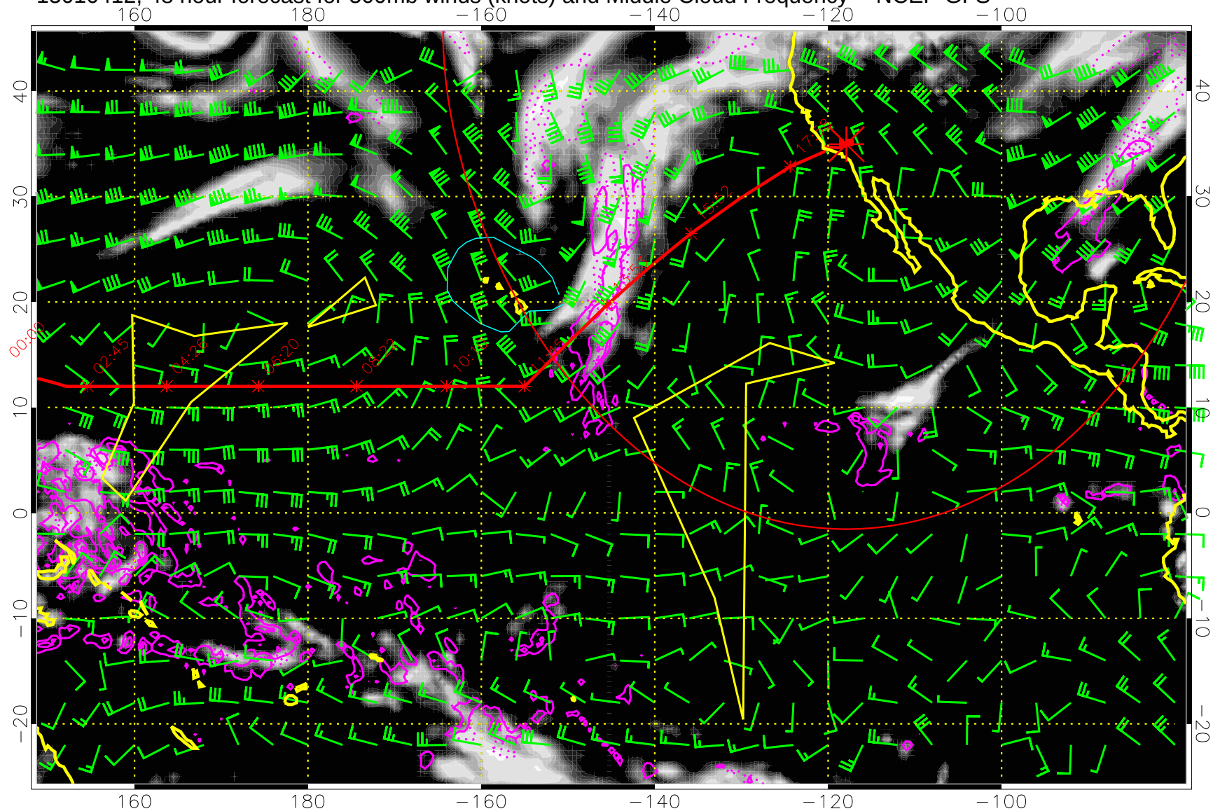
15010412, 48 hour forecast for 500mb winds (knots) and Middle Cloud Frequency -- NCEP GFS
