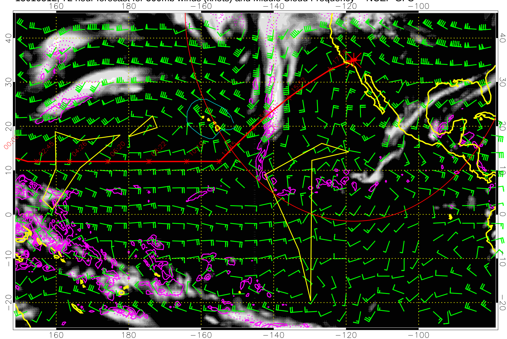
15010512, 72 hour forecast for 500mb winds (knots) and Middle Cloud Frequency -- NCEP GFS
