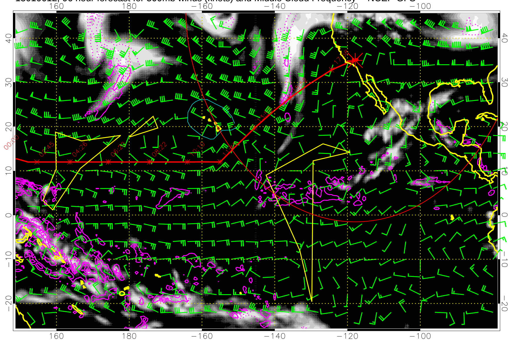
15010612, 96 hour forecast for 500mb winds (knots) and Middle Cloud Frequency -- NCEP GFS
