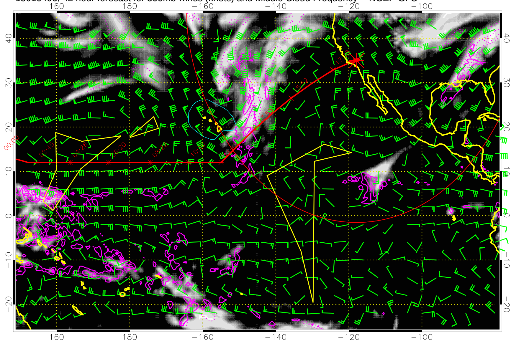
15010406, 42 hour forecast for 500mb winds (knots) and Middle Cloud Frequency -- NCEP GFS
