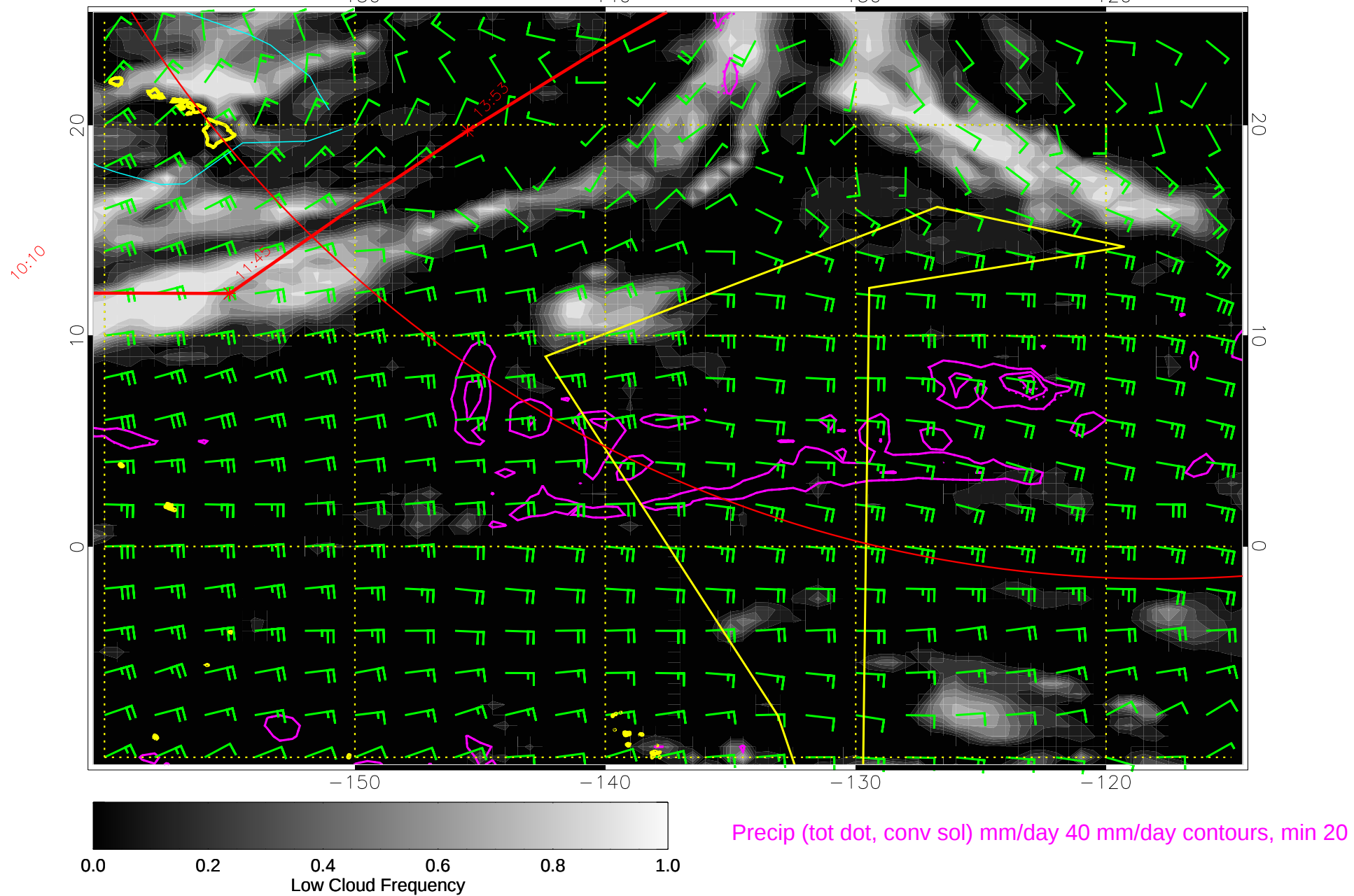
15010618, 102 hour forecast for 850mb winds (knots) and Low Cloud Frequency -- NCEP GFS
