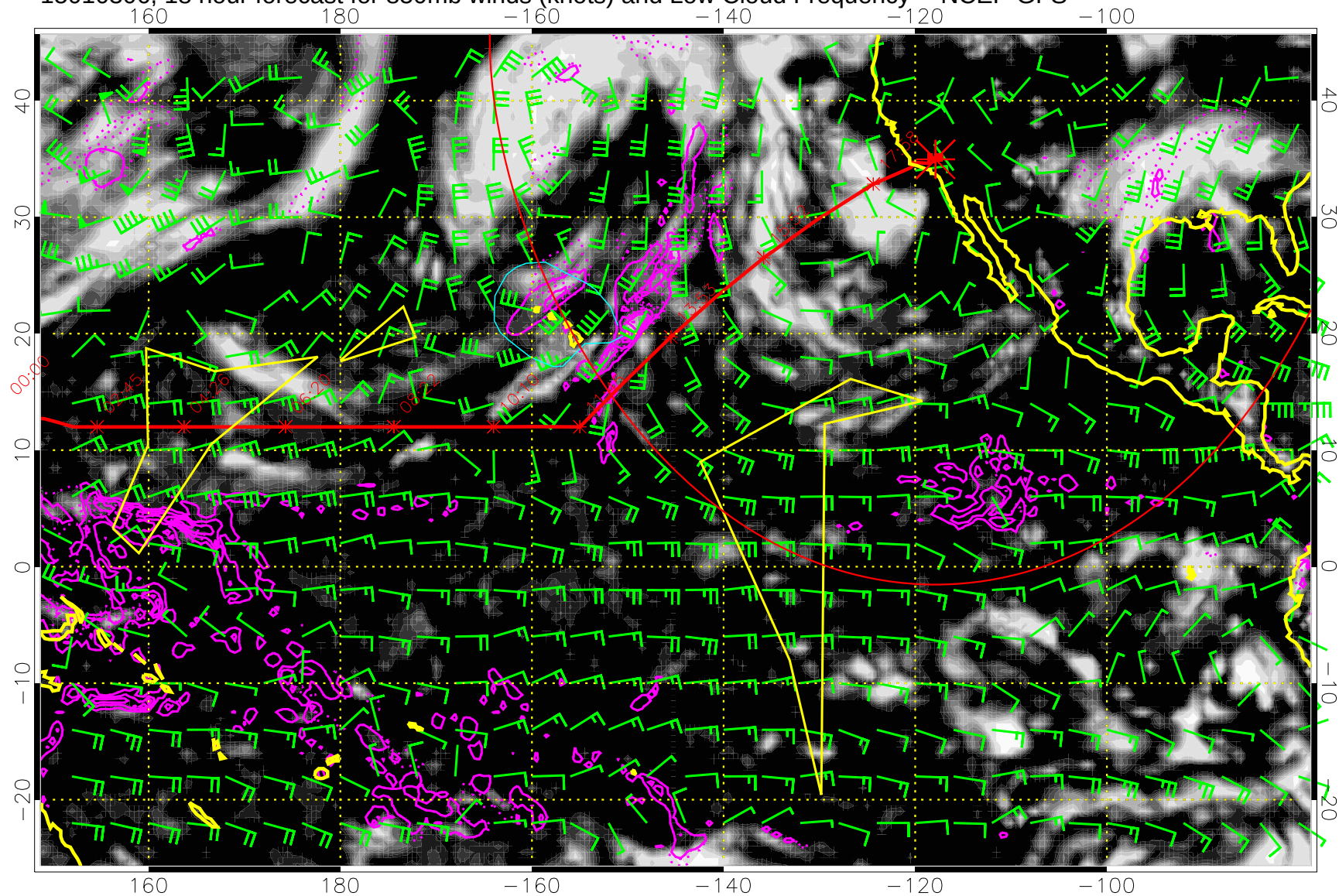
15010306, 18 hour forecast for 850mb winds (knots) and Low Cloud Frequency -- NCEP GFS
