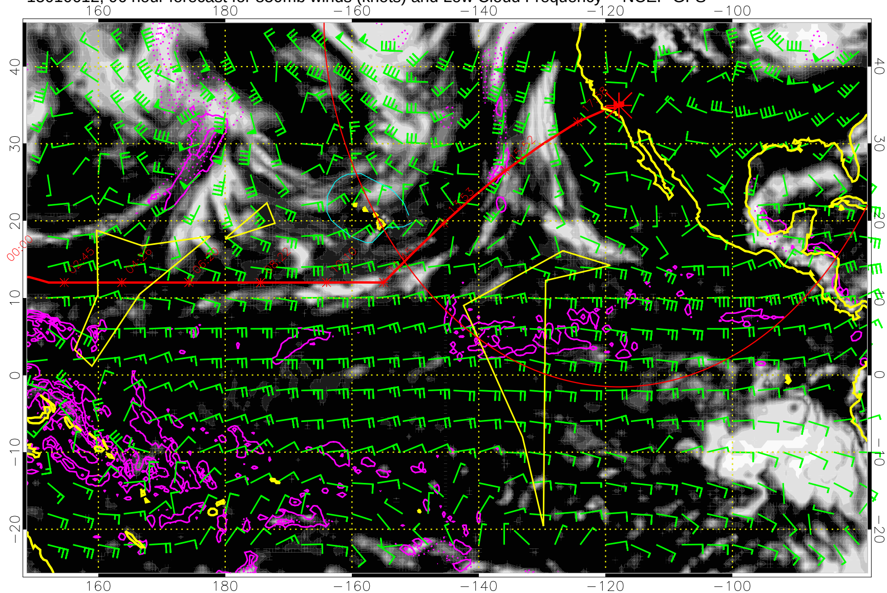
15010612, 96 hour forecast for 850mb winds (knots) and Low Cloud Frequency -- NCEP GFS
