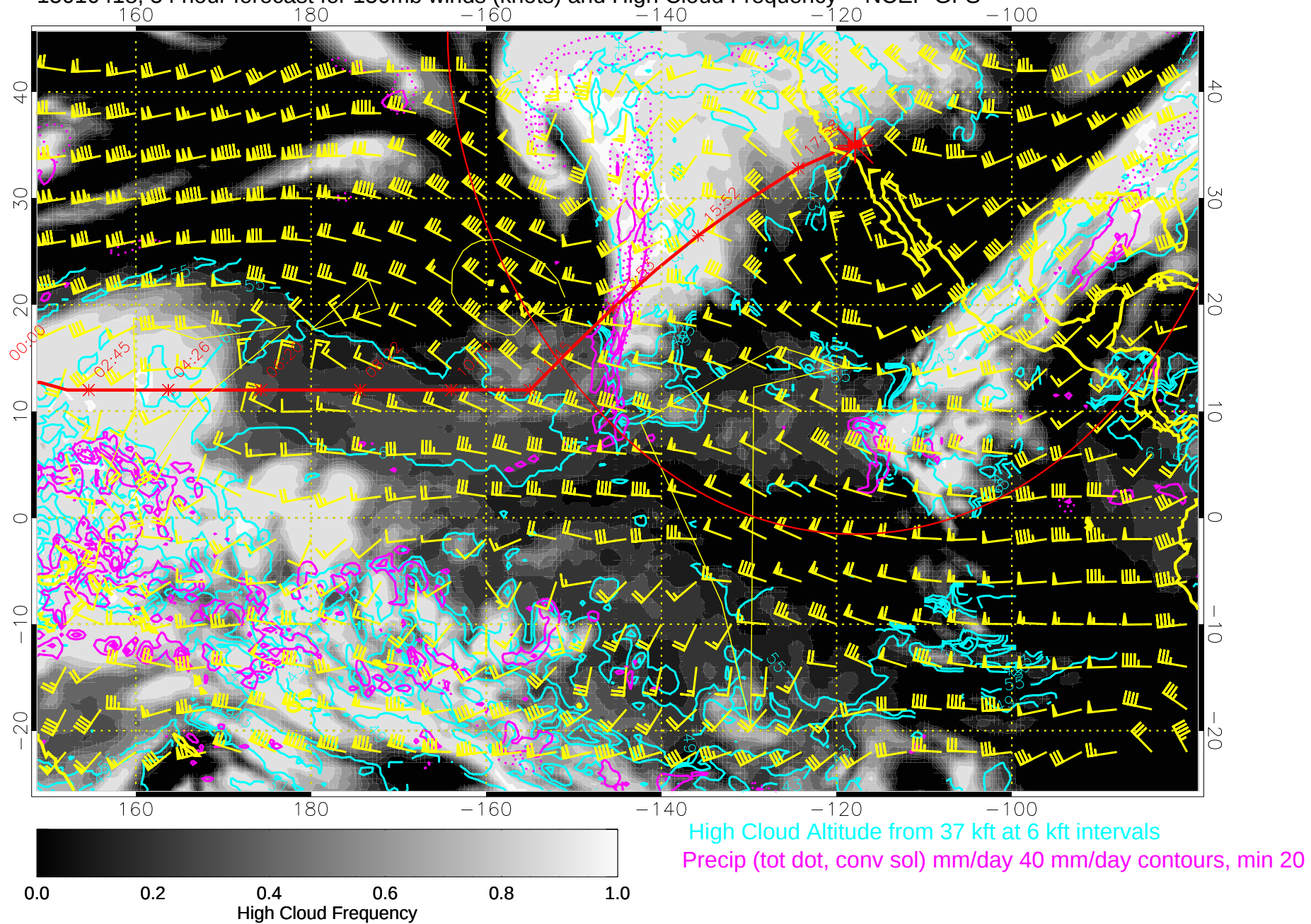
15010418, 54 hour forecast for 150mb winds (knots) and High Cloud Frequency -- NCEP GFS
