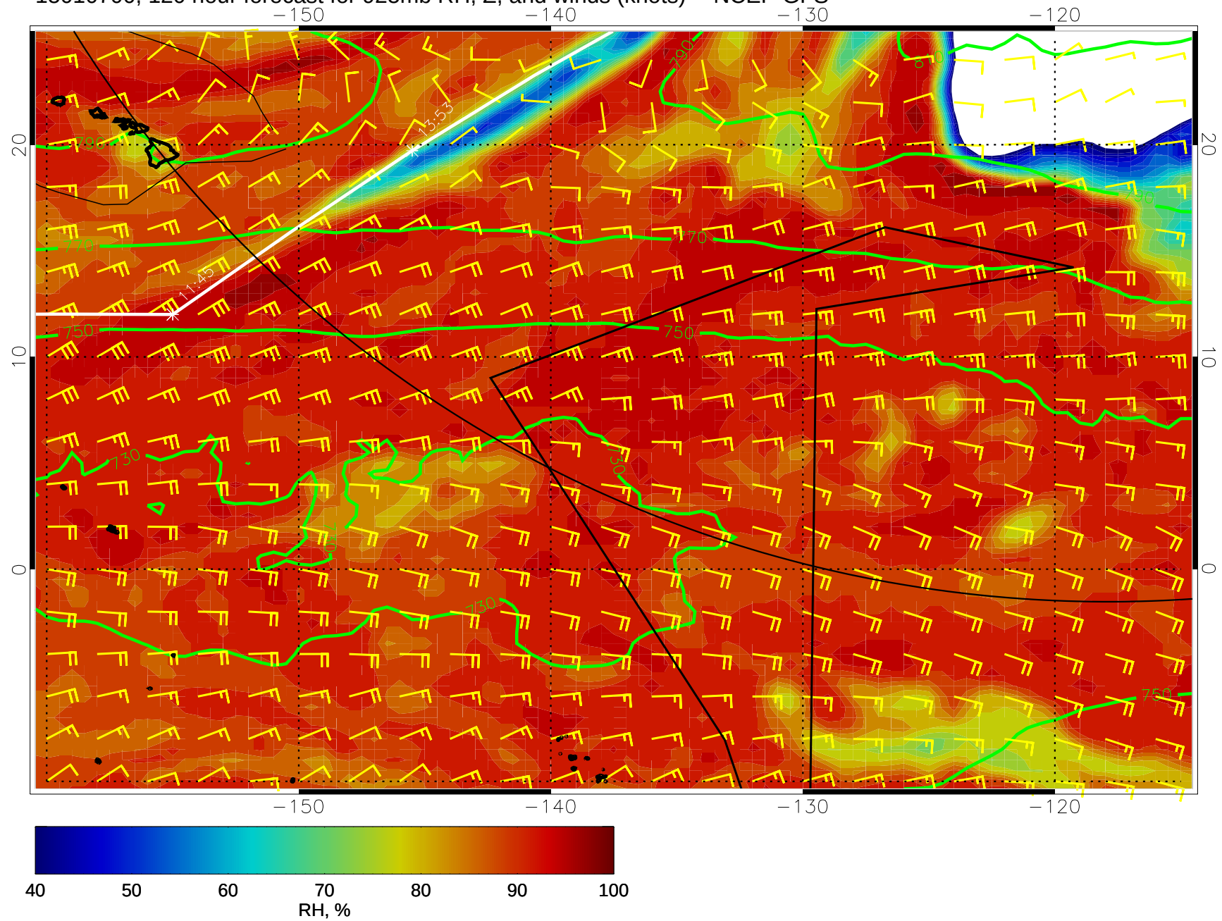
15010700, 120 hour forecast for 925mb RH, Z, and winds (knots) -- NCEP GFS
