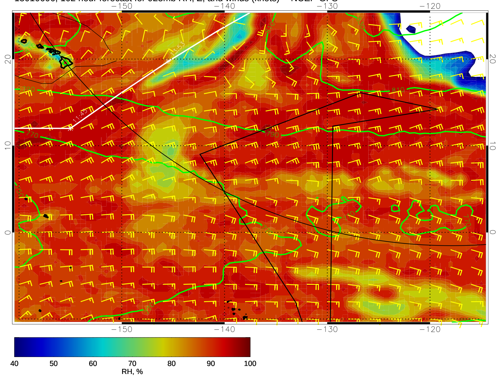
15010606, 102 hour forecast for 925mb RH, Z, and winds (knots) -- NCEP GFS
