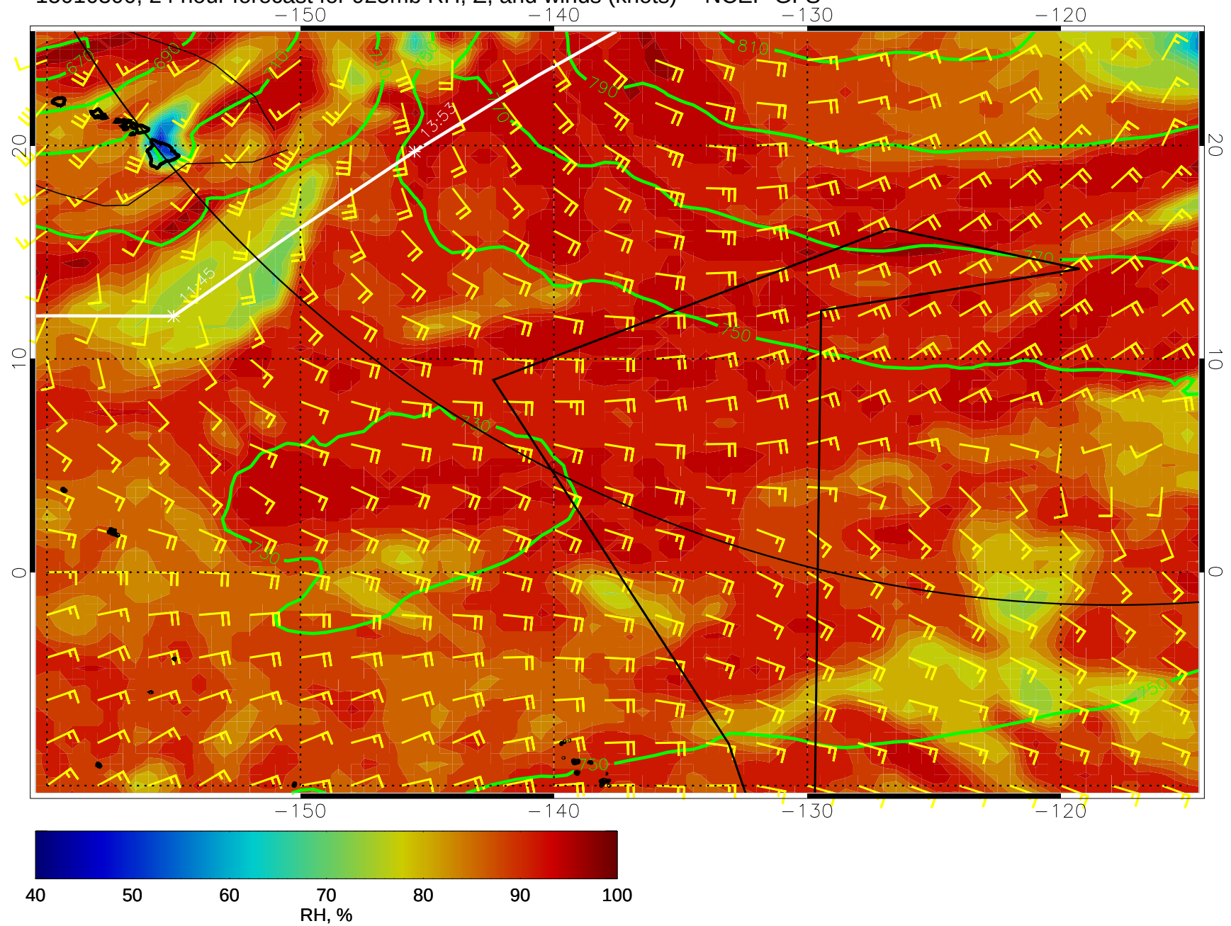
15010300, 24 hour forecast for 925mb RH, Z, and winds (knots) -- NCEP GFS
