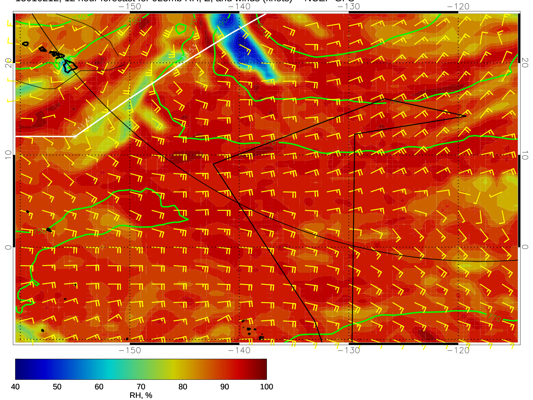
15010212, 12 hour forecast for 925mb RH, Z, and winds (knots) -- NCEP GFS
