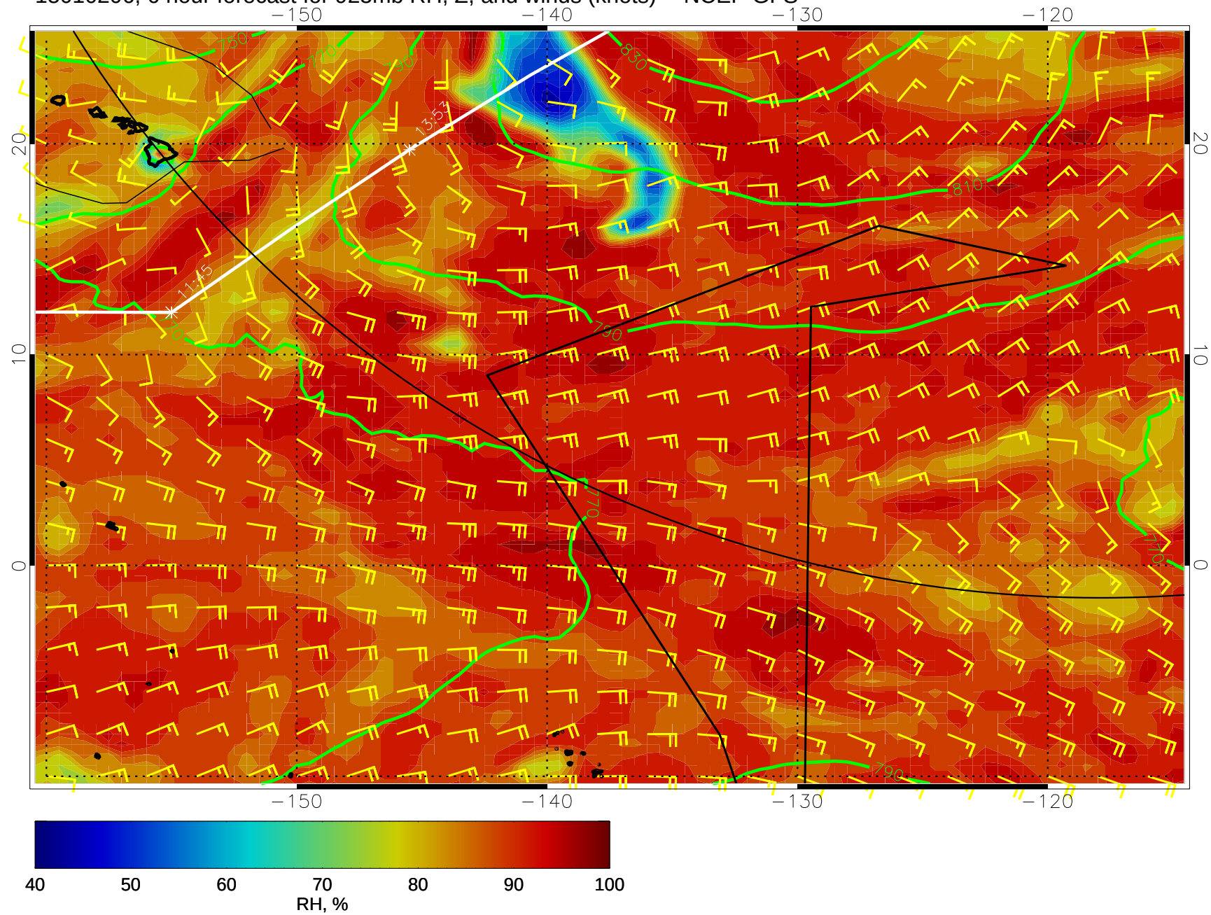
15010206, 6 hour forecast for 925mb RH, Z, and winds (knots) -- NCEP GFS
