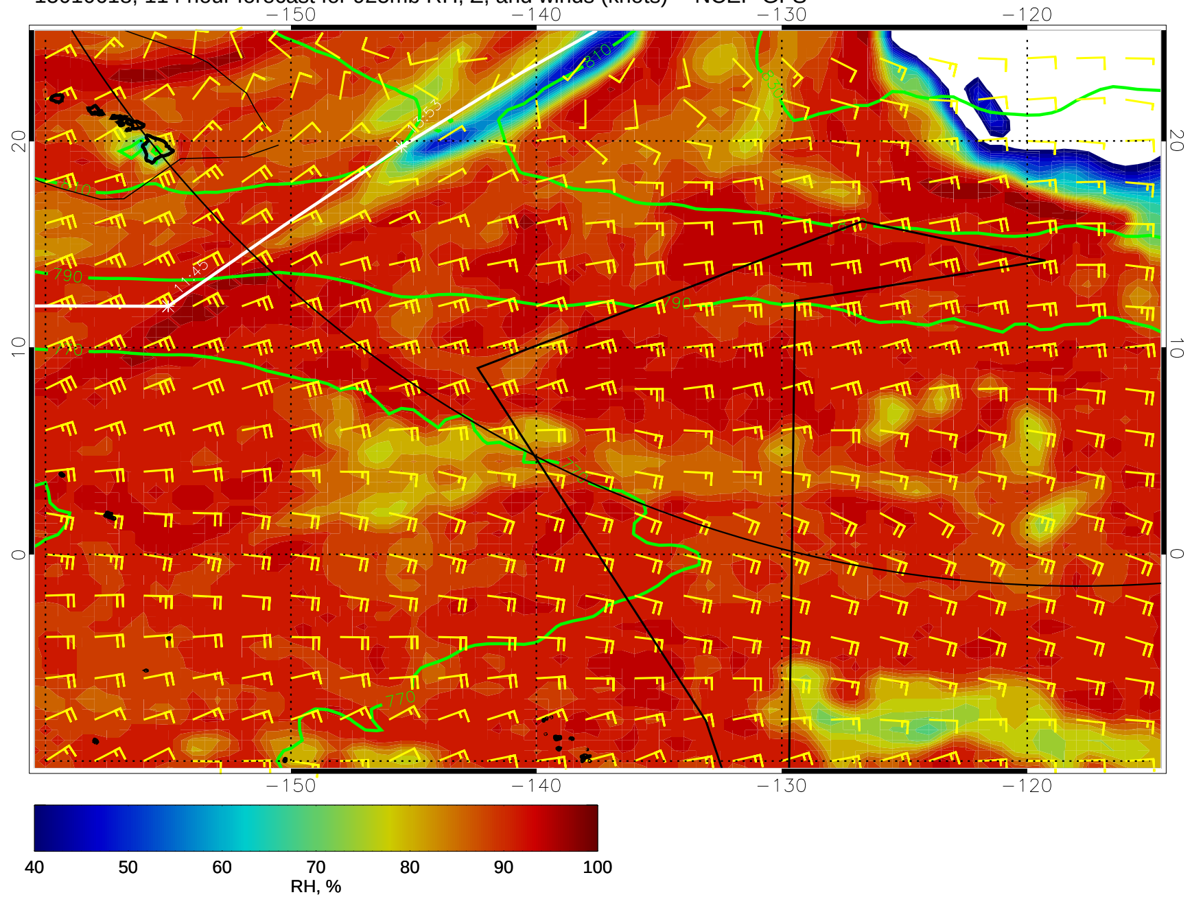
15010618, 114 hour forecast for 925mb RH, Z, and winds (knots) -- NCEP GFS
