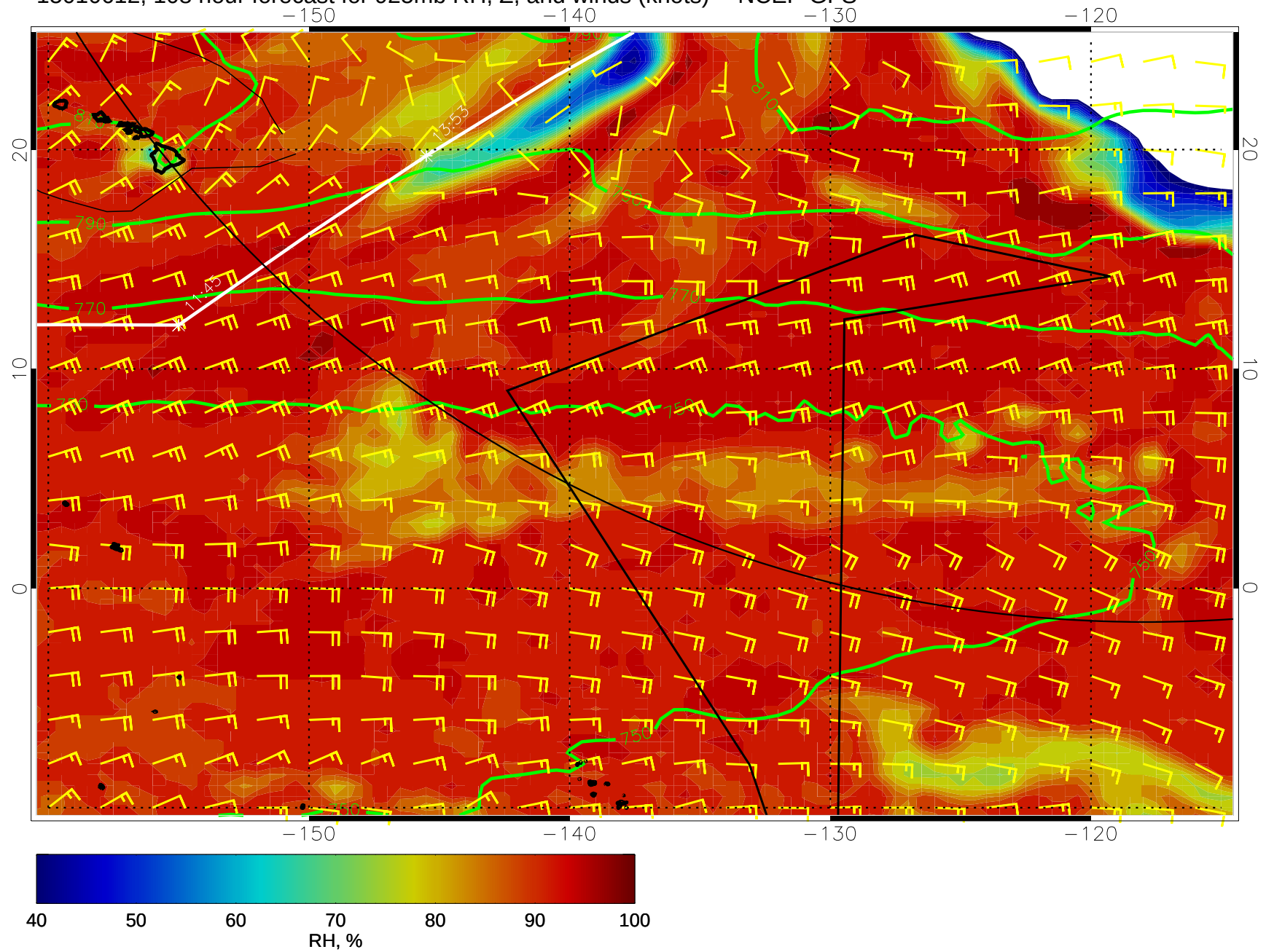
15010612, 108 hour forecast for 925mb RH, Z, and winds (knots) -- NCEP GFS
