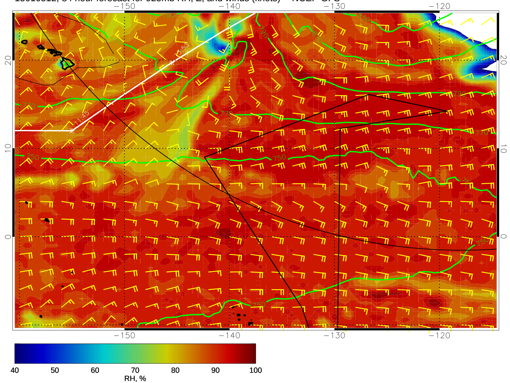
15010512, 84 hour forecast for 925mb RH, Z, and winds (knots) -- NCEP GFS
