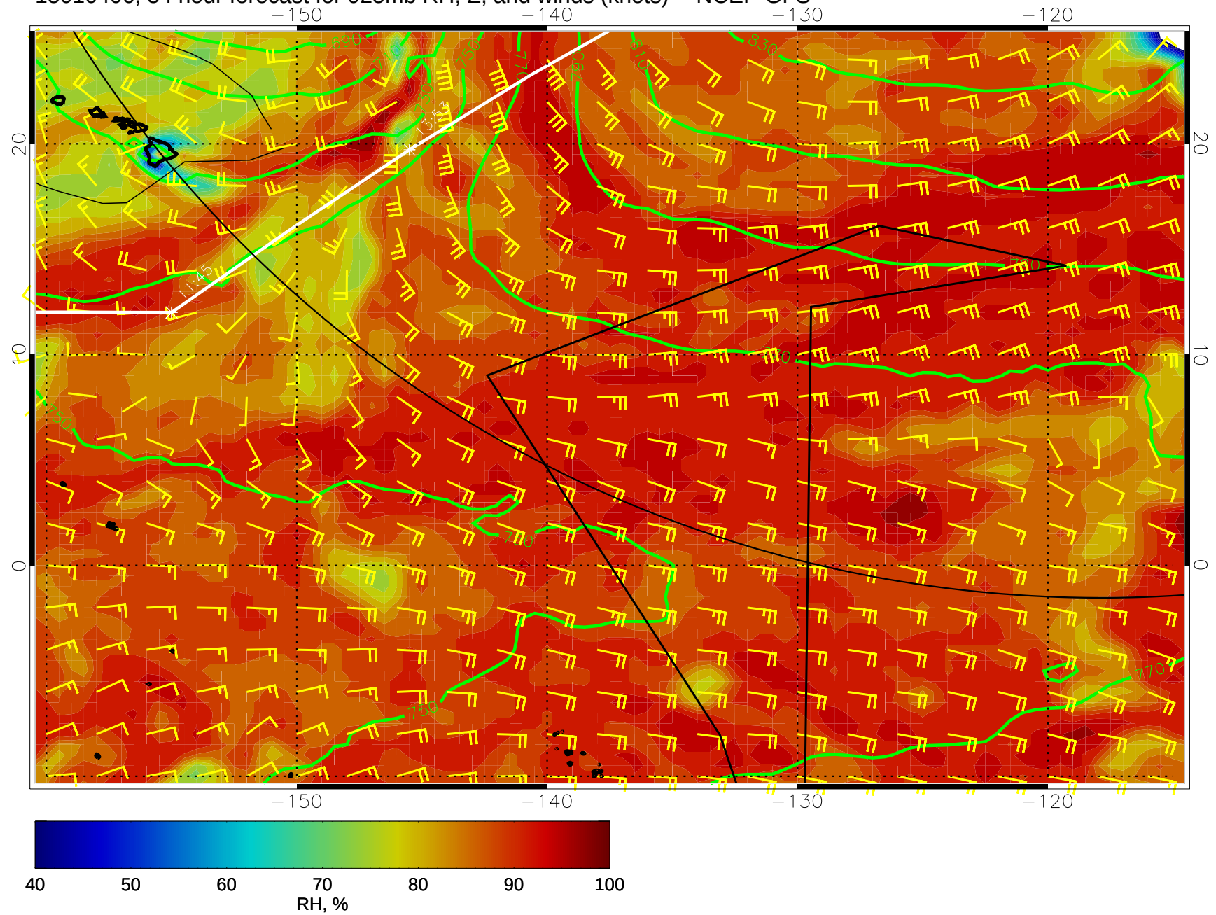
15010406, 54 hour forecast for 925mb RH, Z, and winds (knots) -- NCEP GFS
