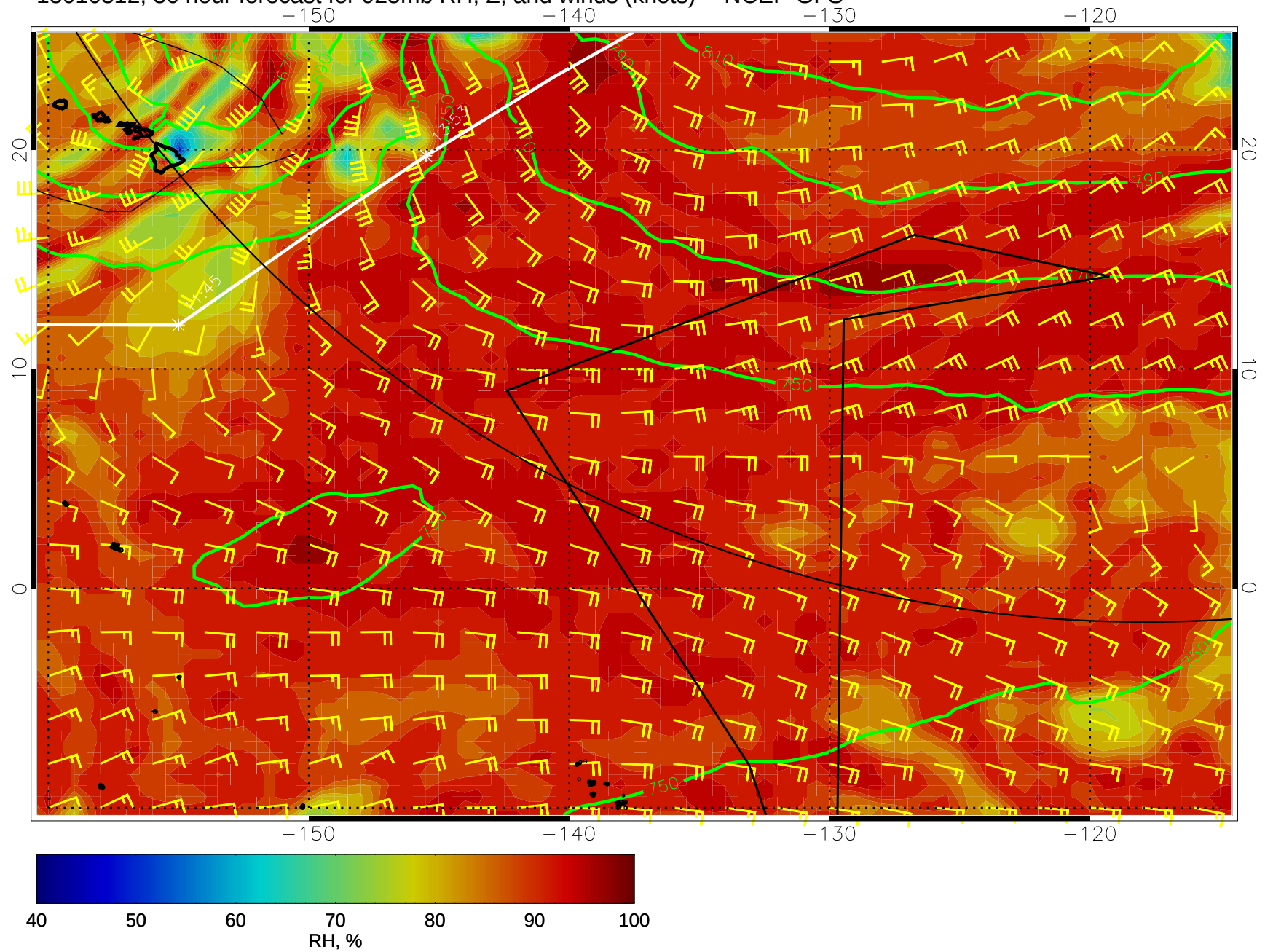
15010312, 36 hour forecast for 925mb RH, Z, and winds (knots) -- NCEP GFS
