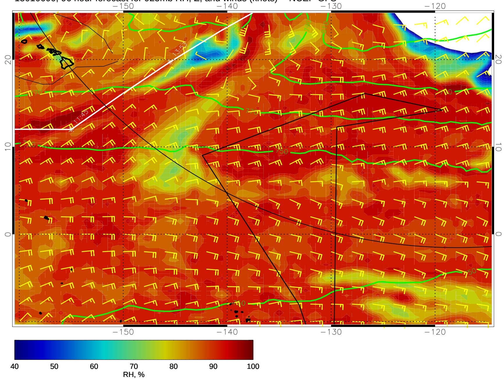
15010600, 96 hour forecast for 925mb RH, Z, and winds (knots) -- NCEP GFS
