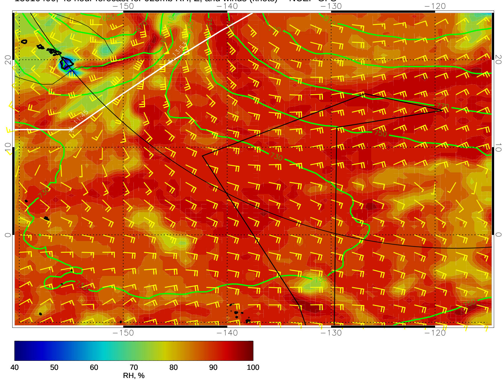
15010400, 48 hour forecast for 925mb RH, Z, and winds (knots) -- NCEP GFS
