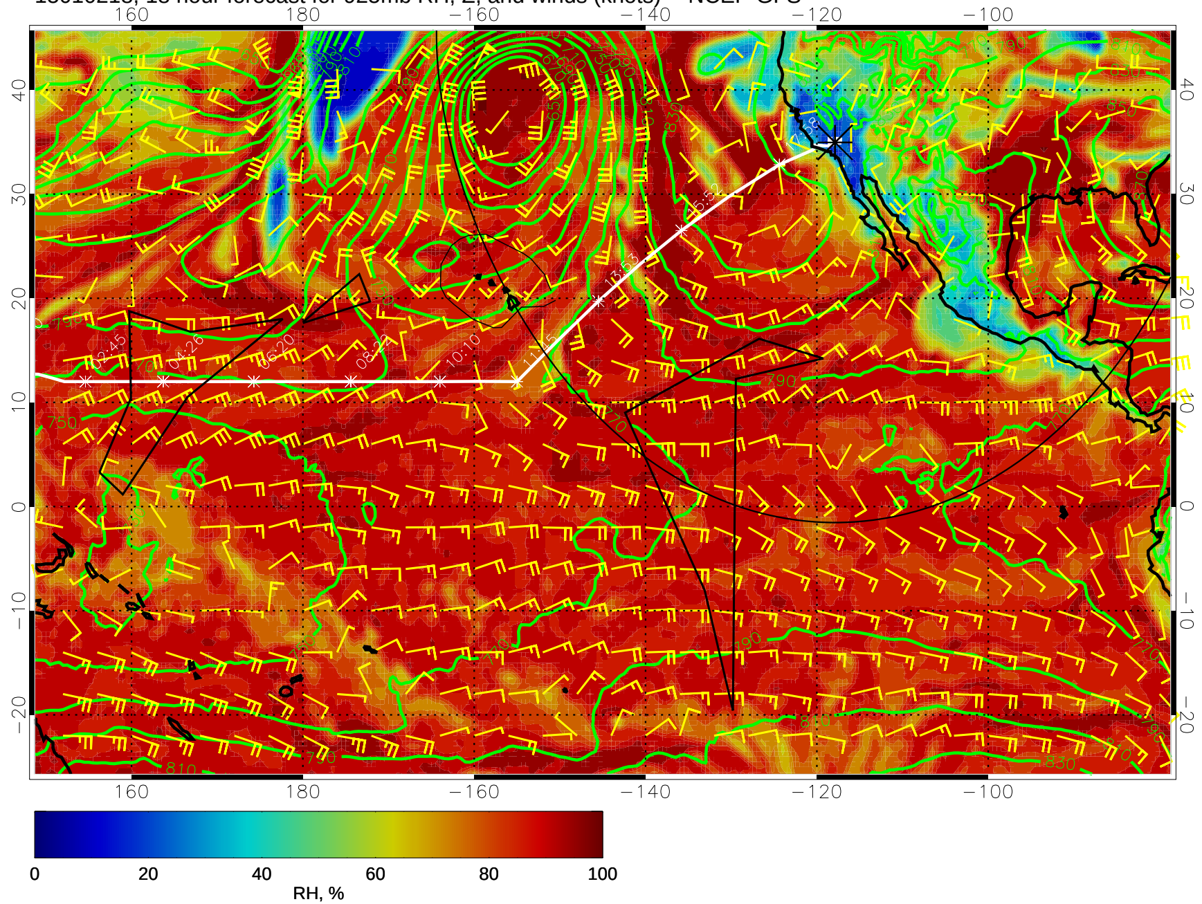
15010218, 18 hour forecast for 925mb RH, Z, and winds (knots) -- NCEP GFS
