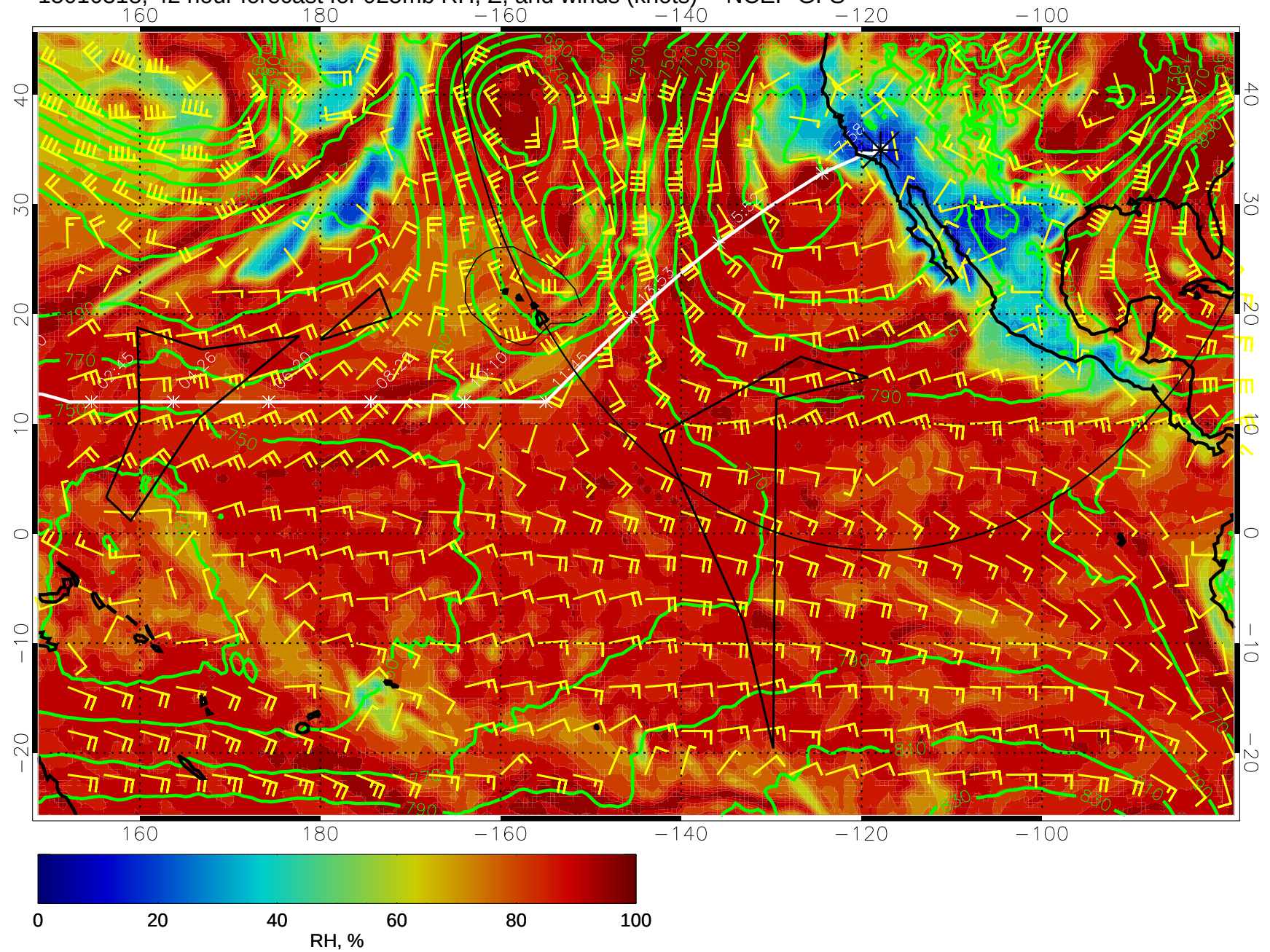
15010318, 42 hour forecast for 925mb RH, Z, and winds (knots) -- NCEP GFS
