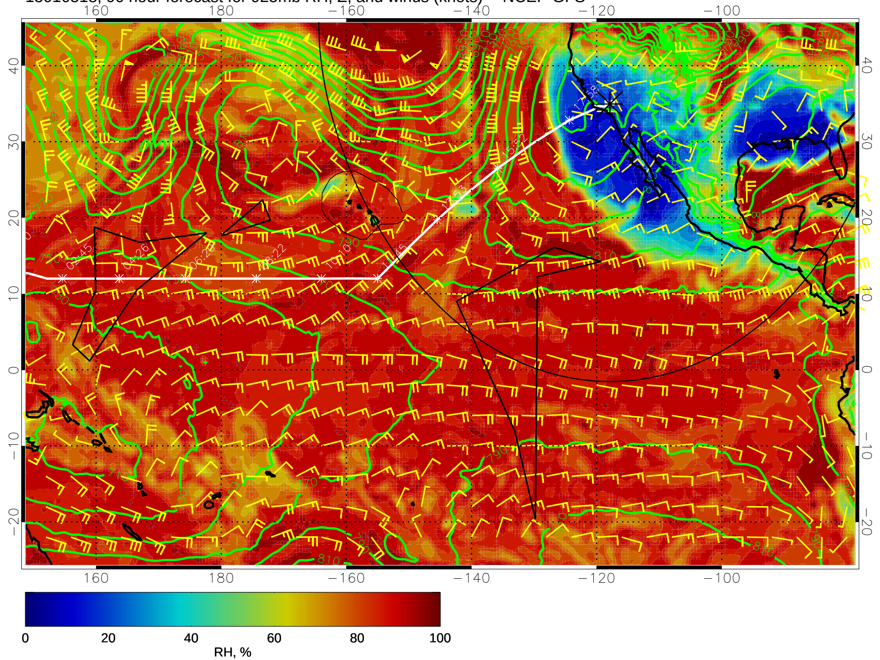
15010518, 90 hour forecast for 925mb RH, Z, and winds (knots) -- NCEP GFS
