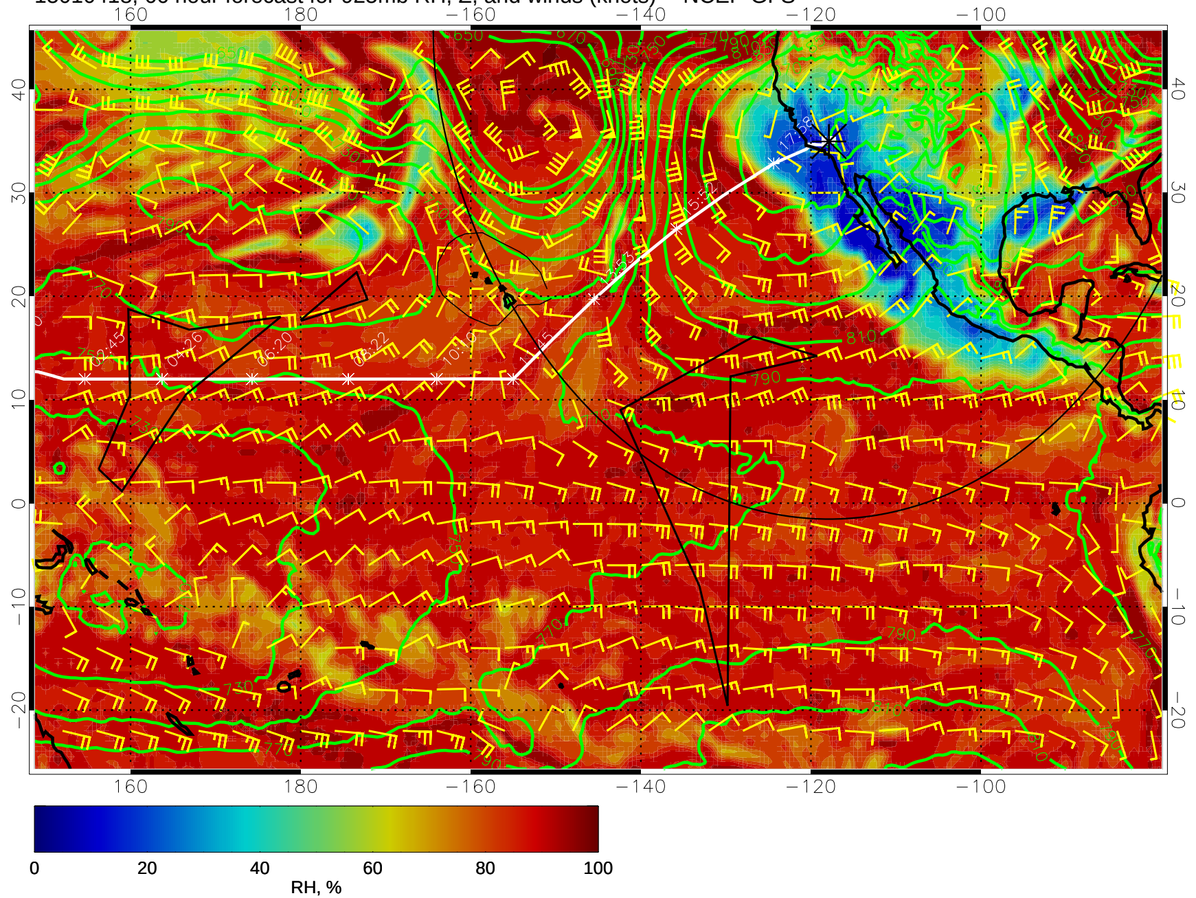
15010418, 66 hour forecast for 925mb RH, Z, and winds (knots) -- NCEP GFS
