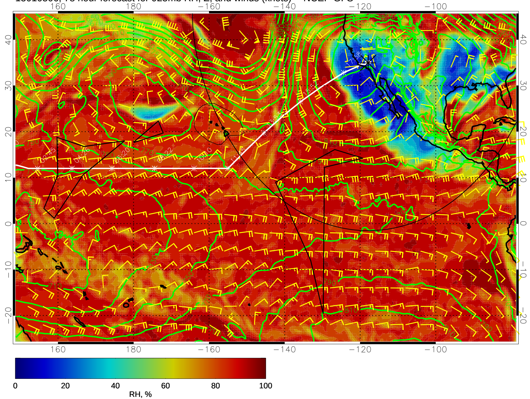
15010506, 78 hour forecast for 925mb RH, Z, and winds (knots) -- NCEP GFS
