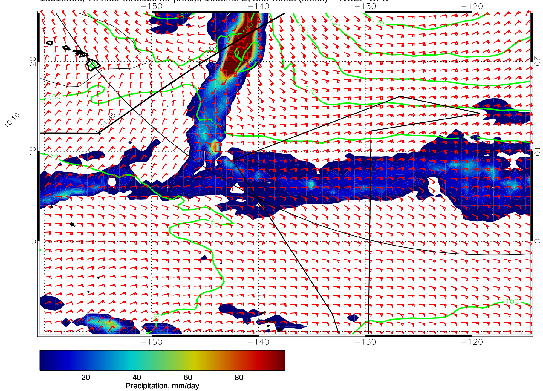
15010506, 78 hour forecast for precip, 1000mb Z, and winds (knots) -- NCEP GFS
