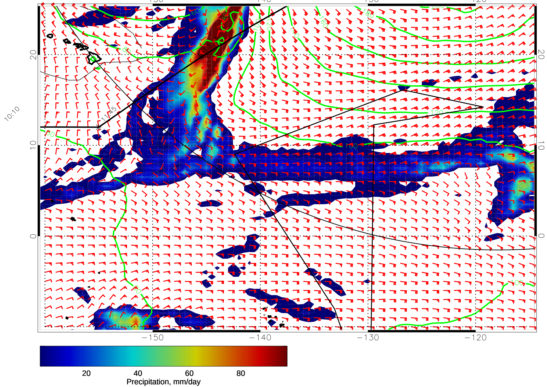
15010418, 66 hour forecast for precip, 1000mb Z, and winds (knots) -- NCEP GFS
