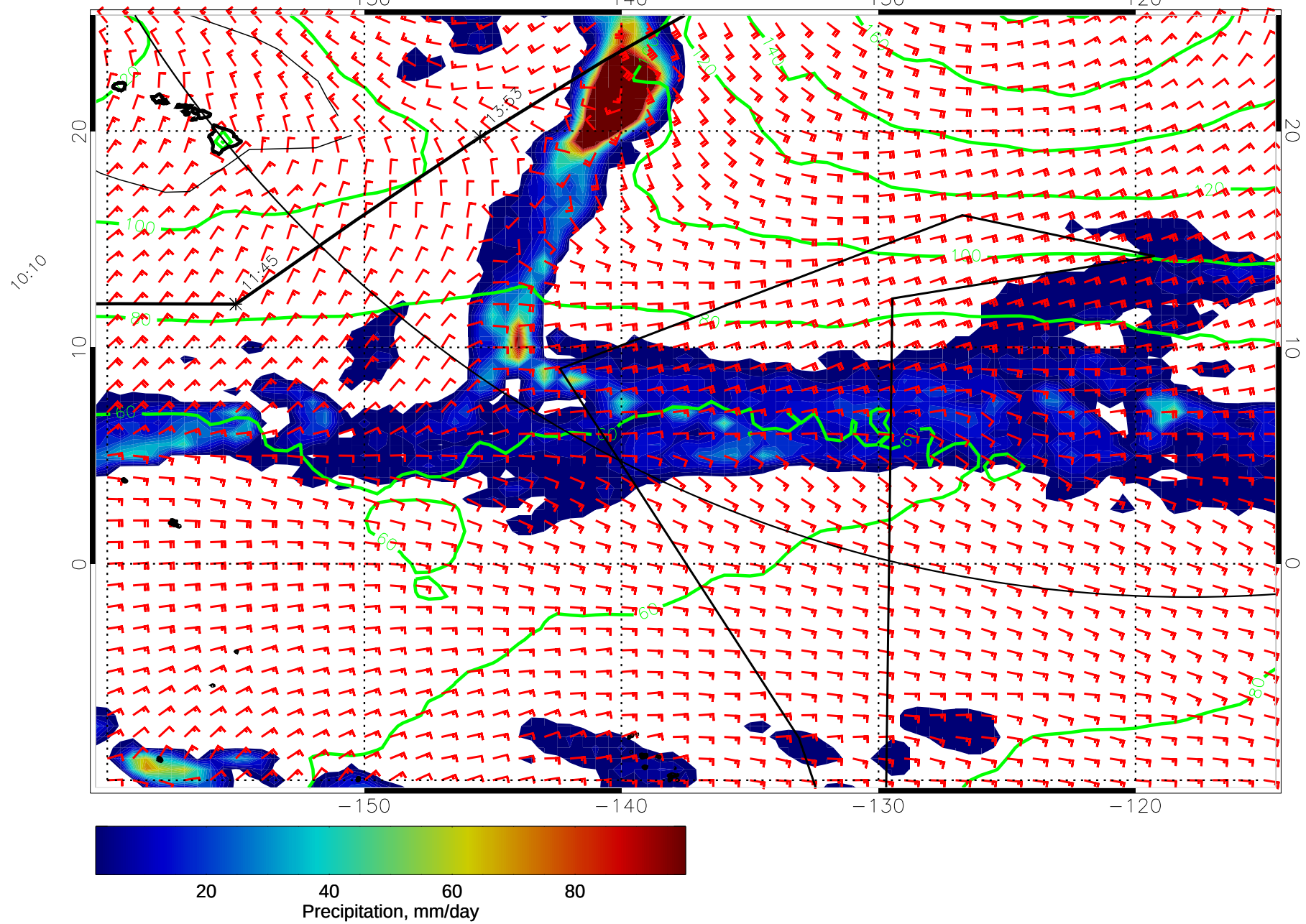
15010512, 84 hour forecast for precip, 1000mb Z, and winds (knots) -- NCEP GFS
