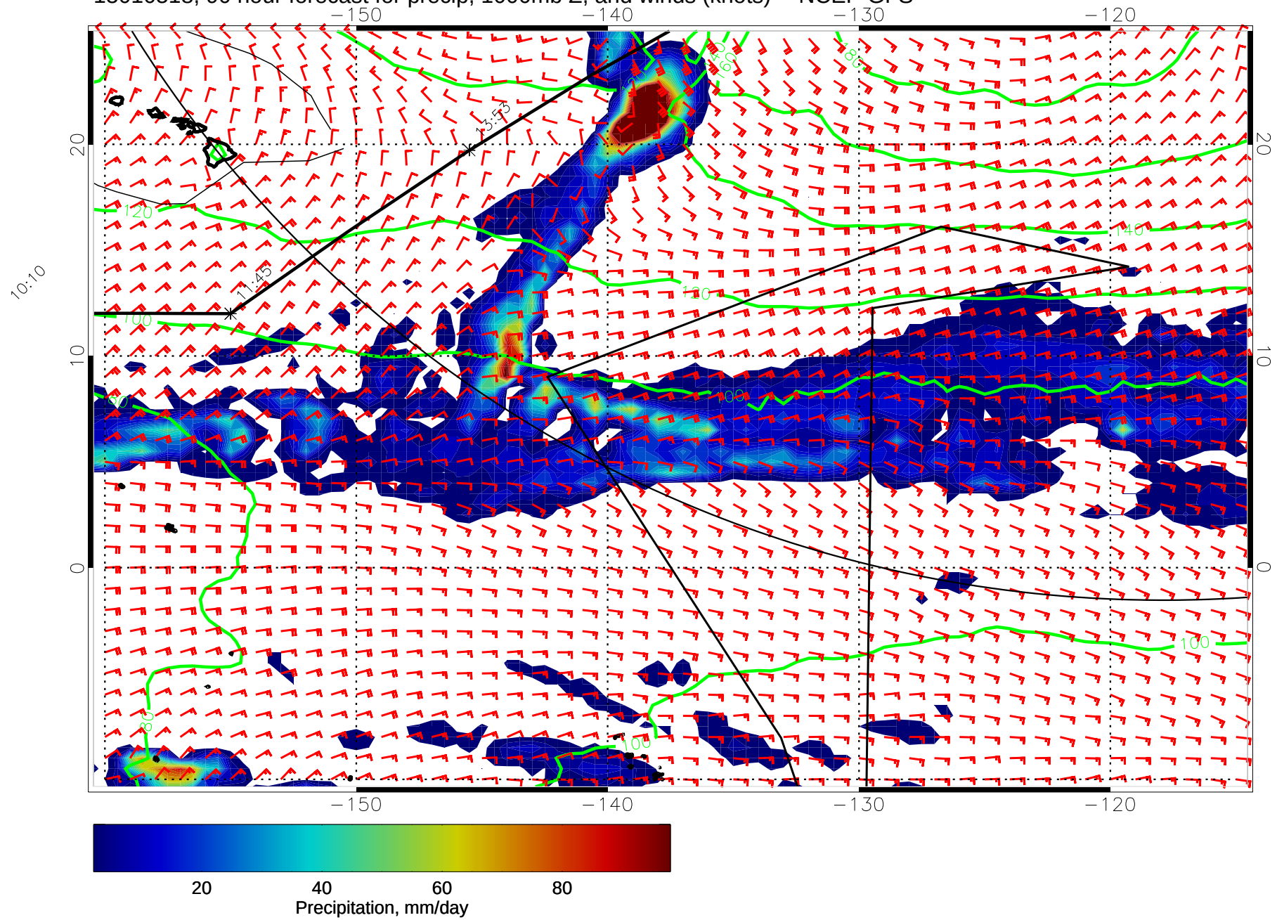
15010518, 90 hour forecast for precip, 1000mb Z, and winds (knots) -- NCEP GFS
