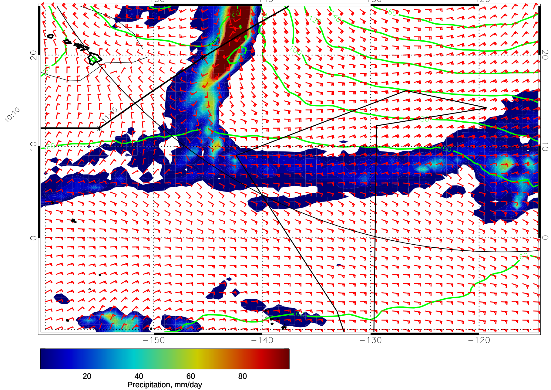
15010500, 72 hour forecast for precip, 1000mb Z, and winds (knots) -- NCEP GFS
