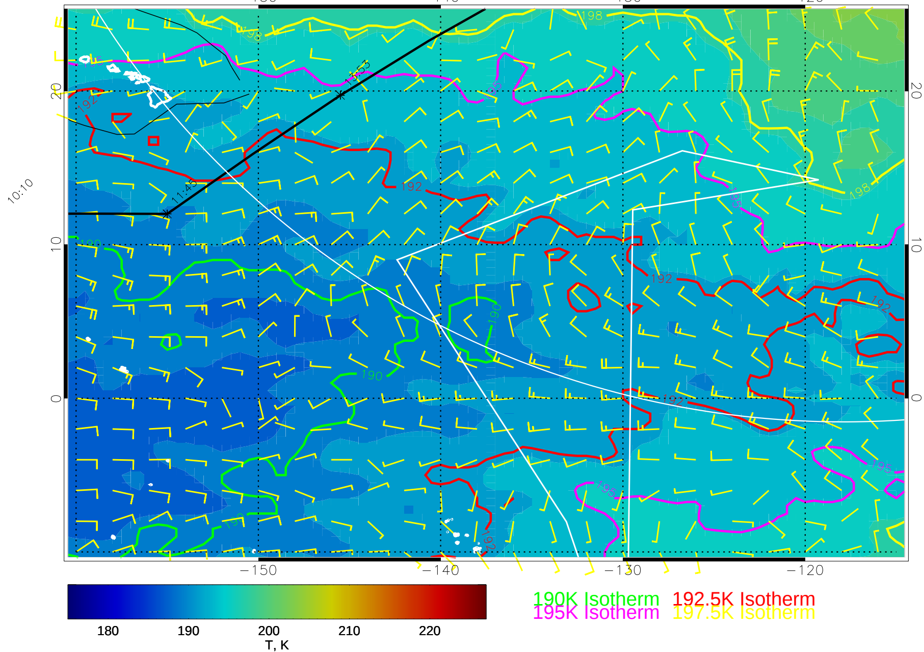
15010612, 108 hour forecast for 70mb T and winds (knots) -- NCEP GFS
