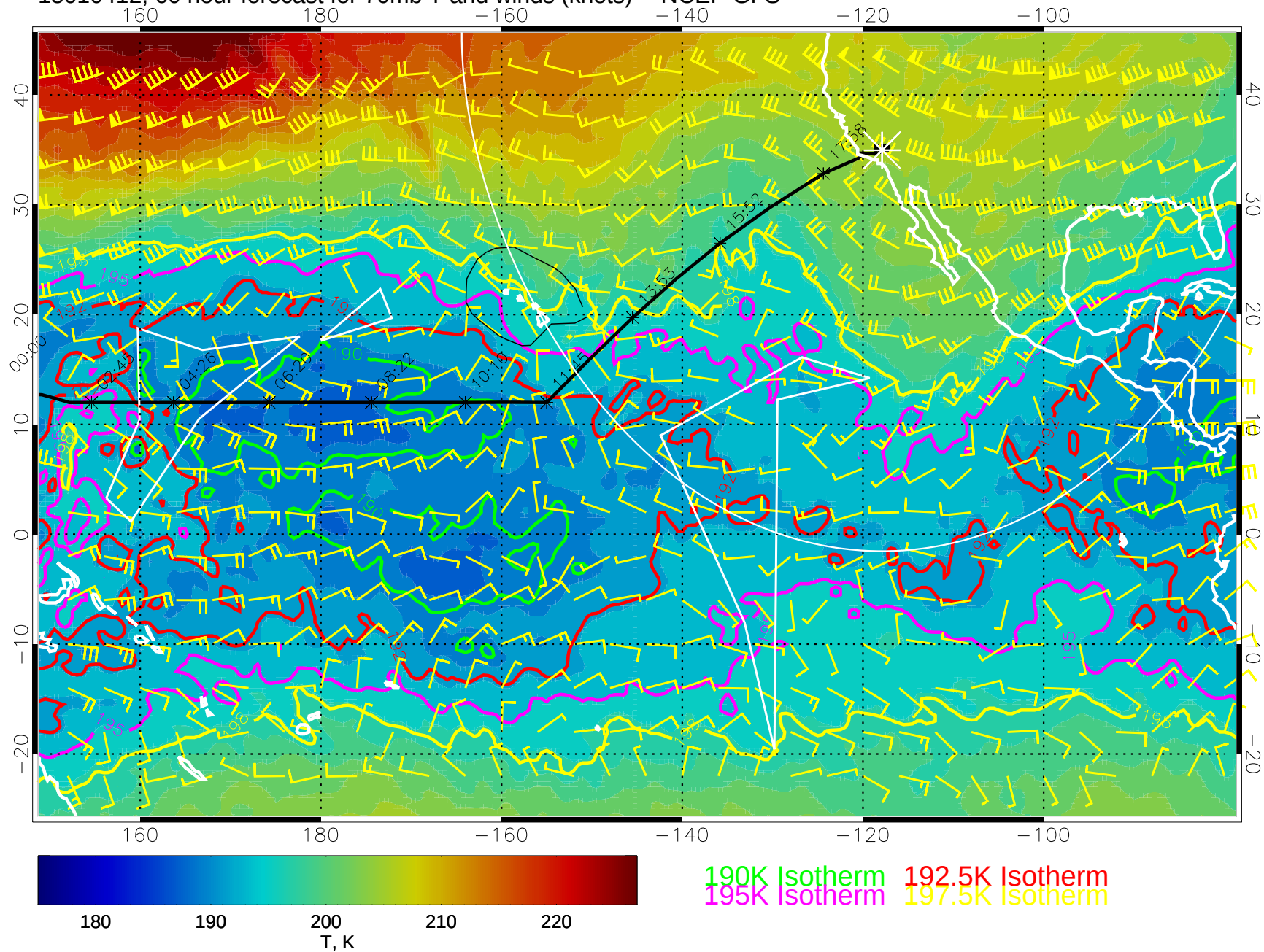
15010412, 60 hour forecast for 70mb T and winds (knots) -- NCEP GFS
