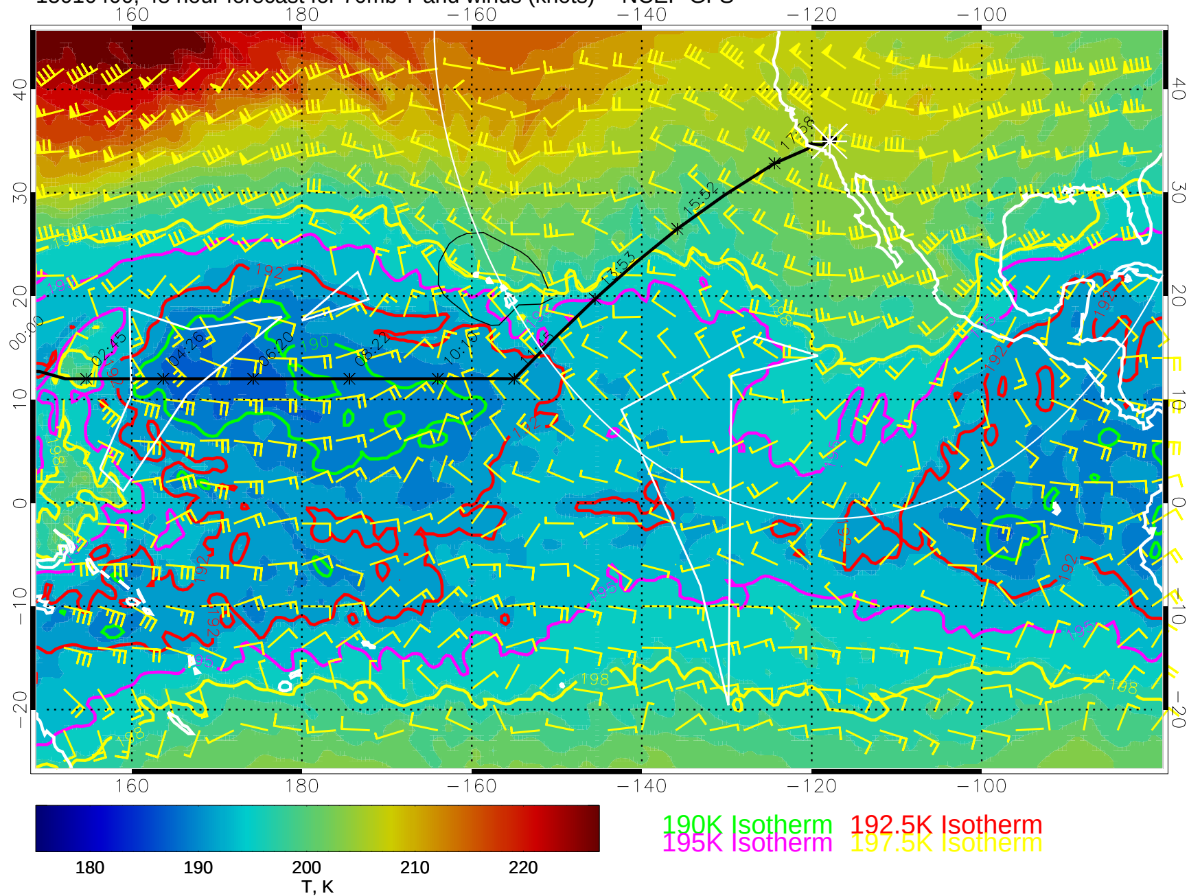
15010400, 48 hour forecast for 70mb T and winds (knots) -- NCEP GFS
