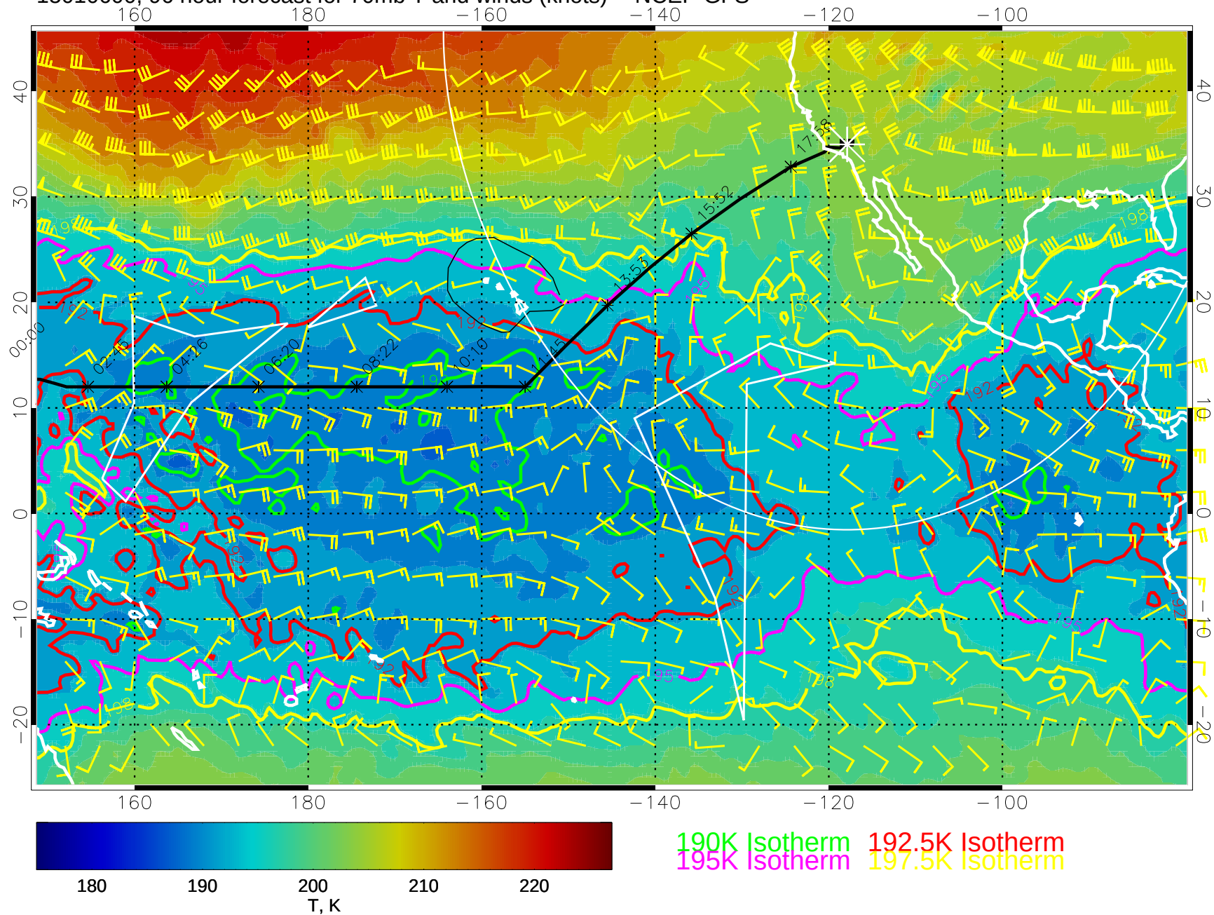
15010600, 96 hour forecast for 70mb T and winds (knots) -- NCEP GFS
