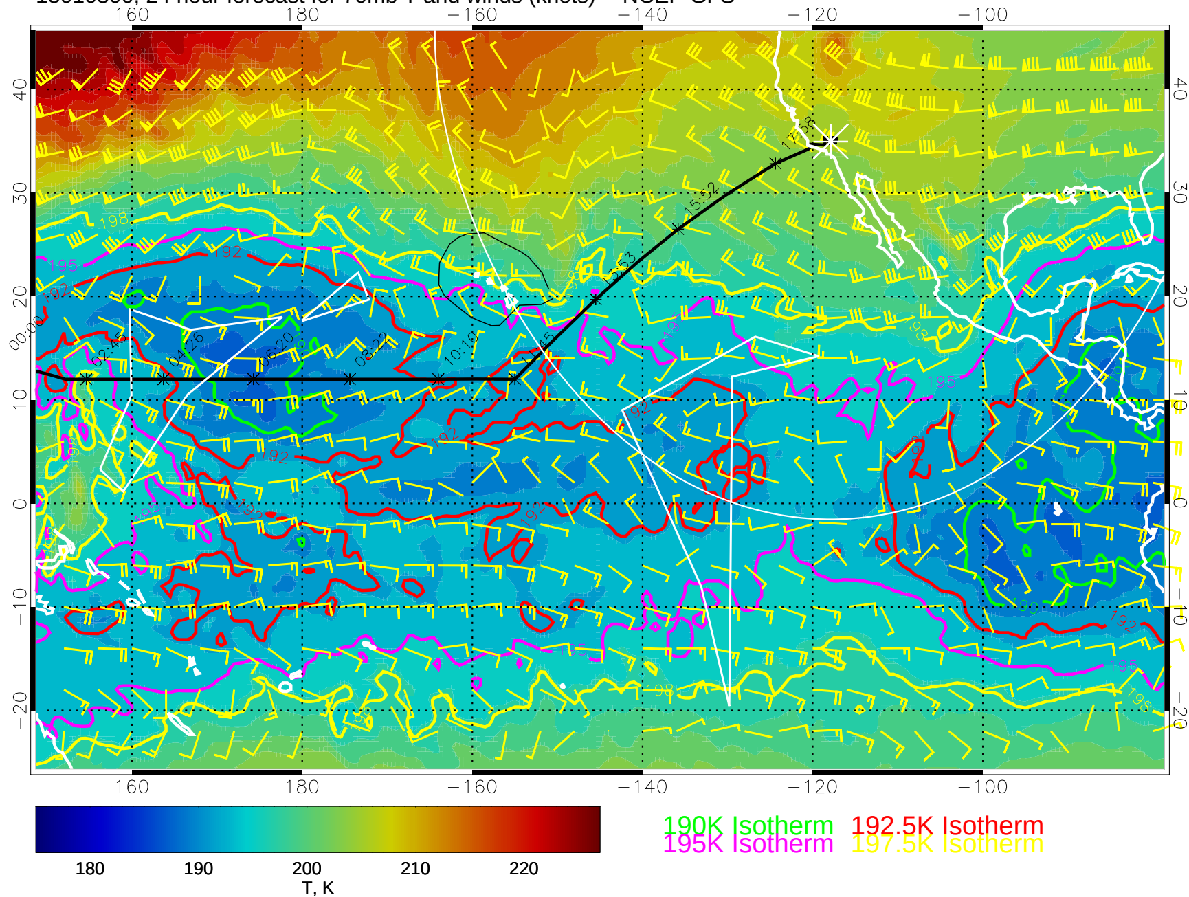
15010300, 24 hour forecast for 70mb T and winds (knots) -- NCEP GFS
