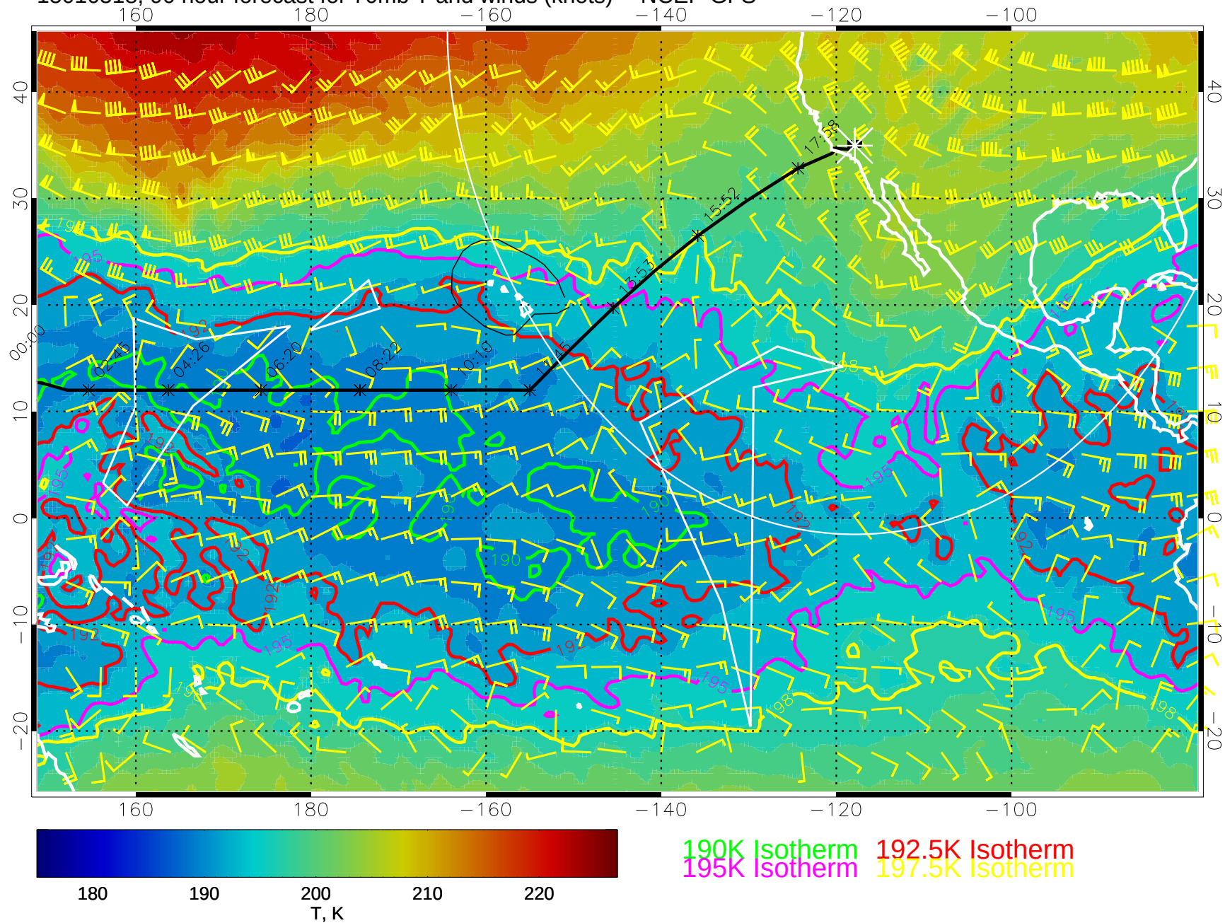
15010518, 90 hour forecast for 70mb T and winds (knots) -- NCEP GFS
