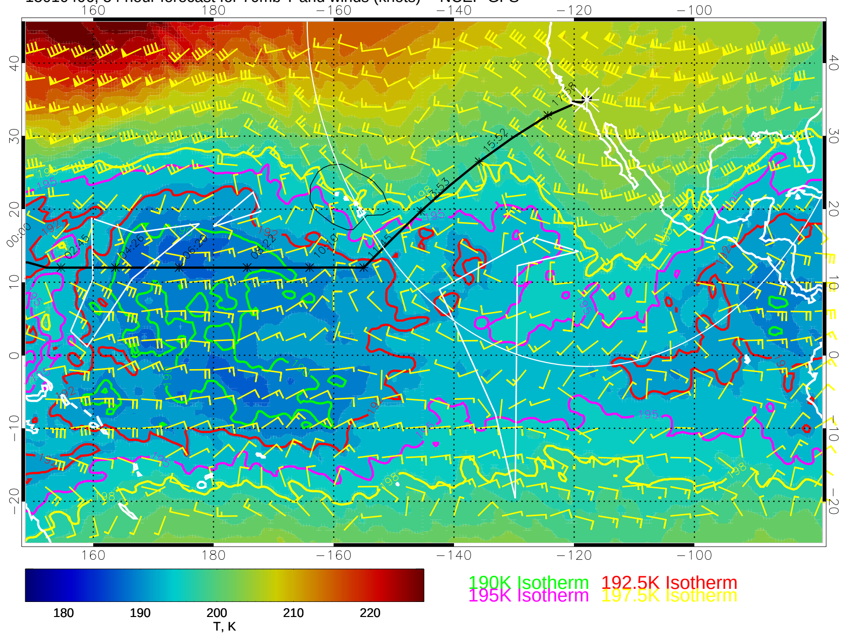
15010406, 54 hour forecast for 70mb T and winds (knots) -- NCEP GFS
