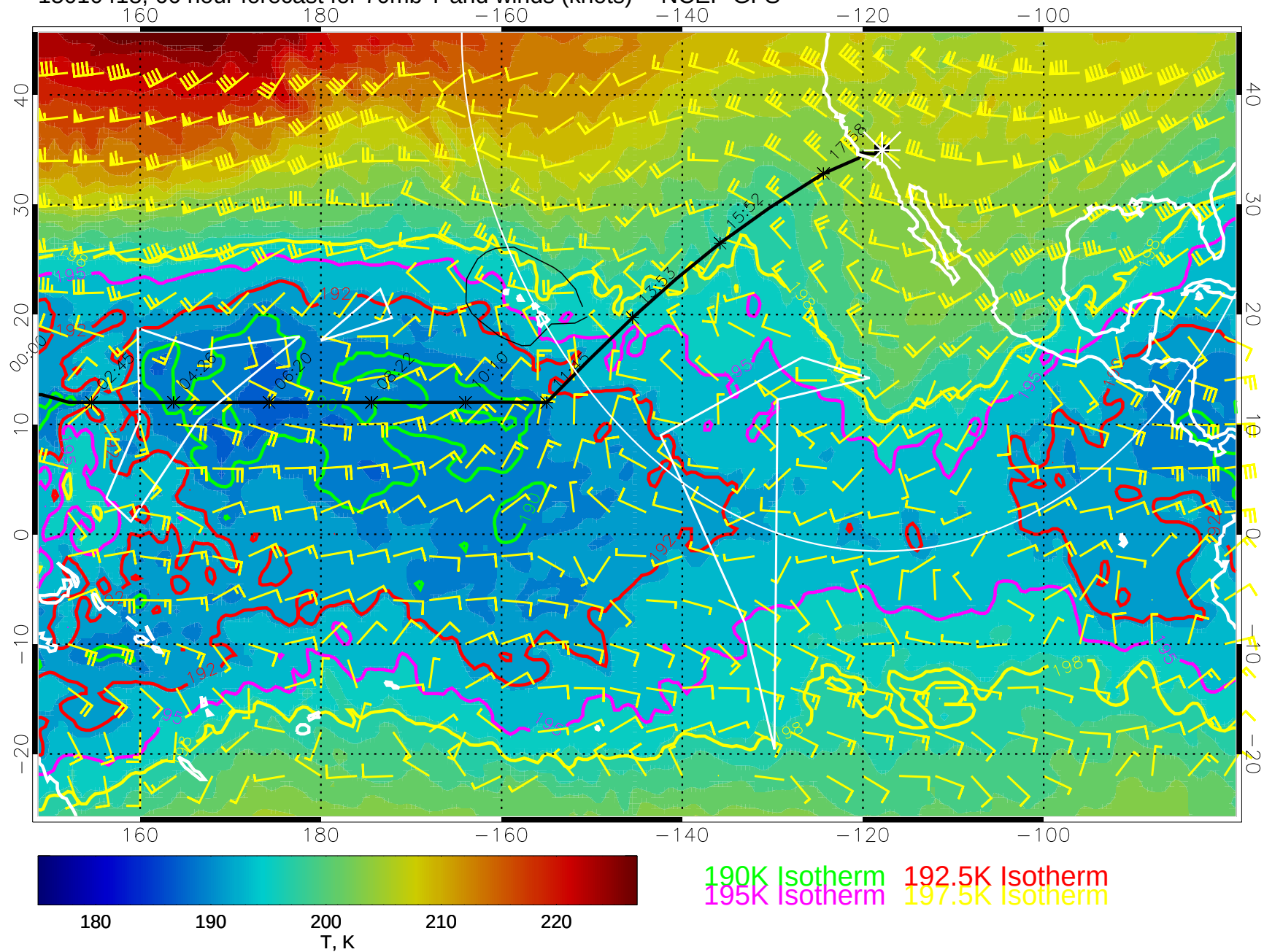
15010418, 66 hour forecast for 70mb T and winds (knots) -- NCEP GFS
