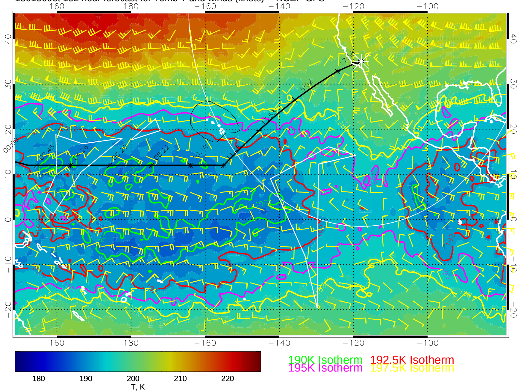
15010606, 102 hour forecast for 70mb T and winds (knots) -- NCEP GFS
