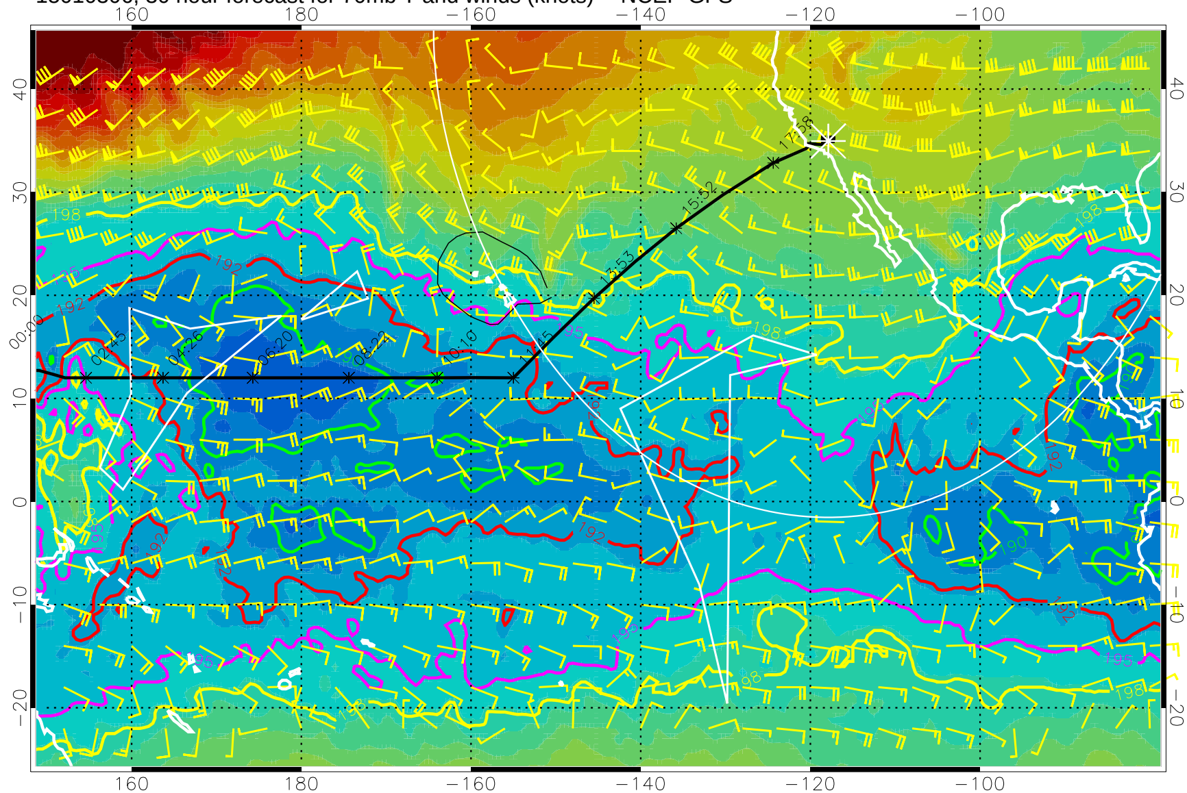
15010306, 30 hour forecast for 70mb T and winds (knots) -- NCEP GFS
