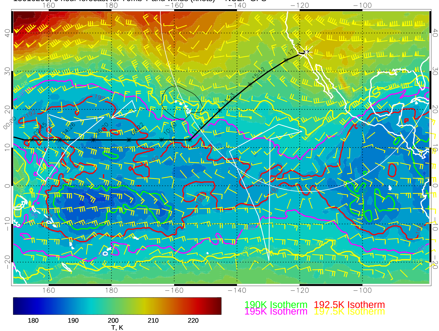
15010206, 6 hour forecast for 70mb T and winds (knots) -- NCEP GFS
