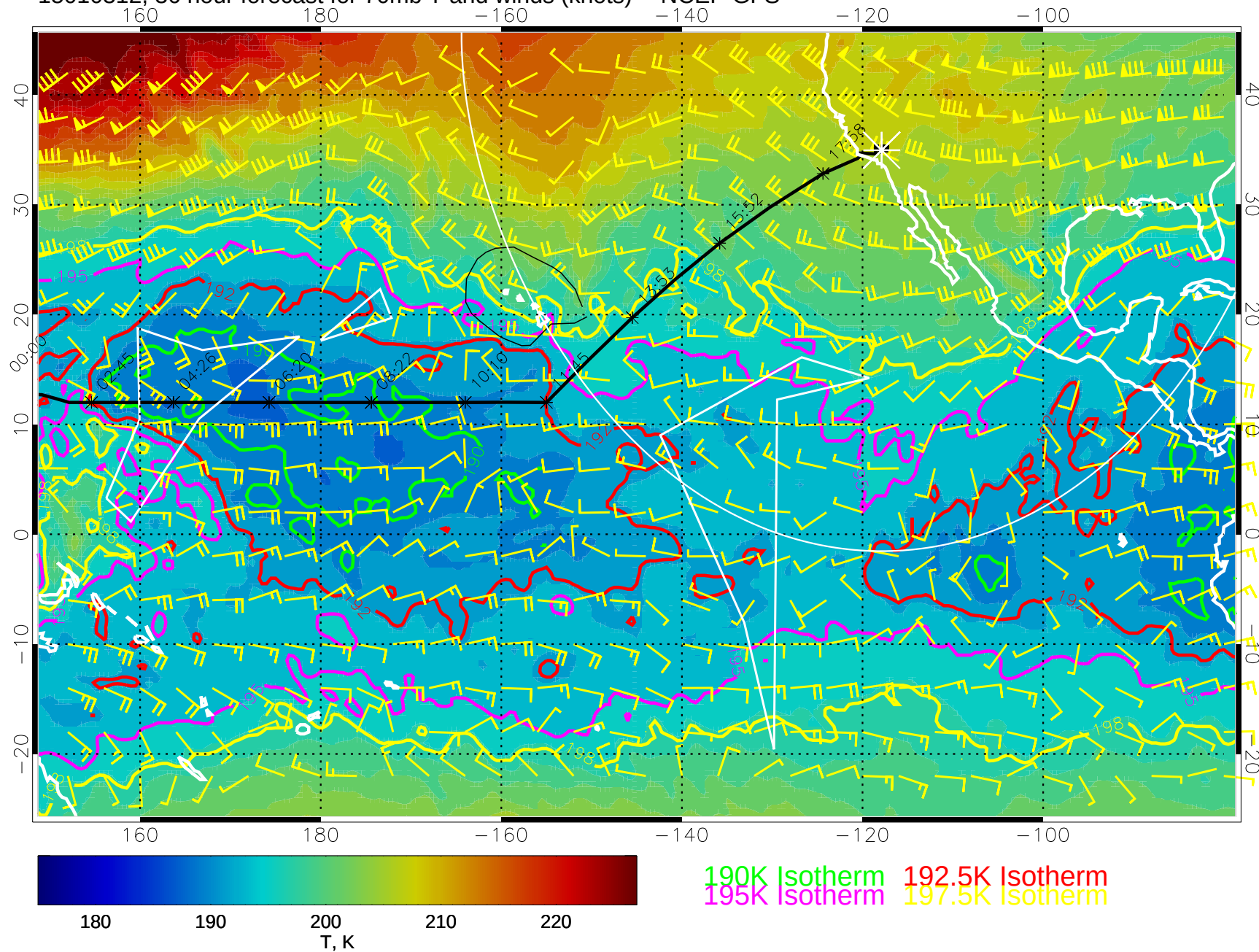
15010312, 36 hour forecast for 70mb T and winds (knots) -- NCEP GFS
