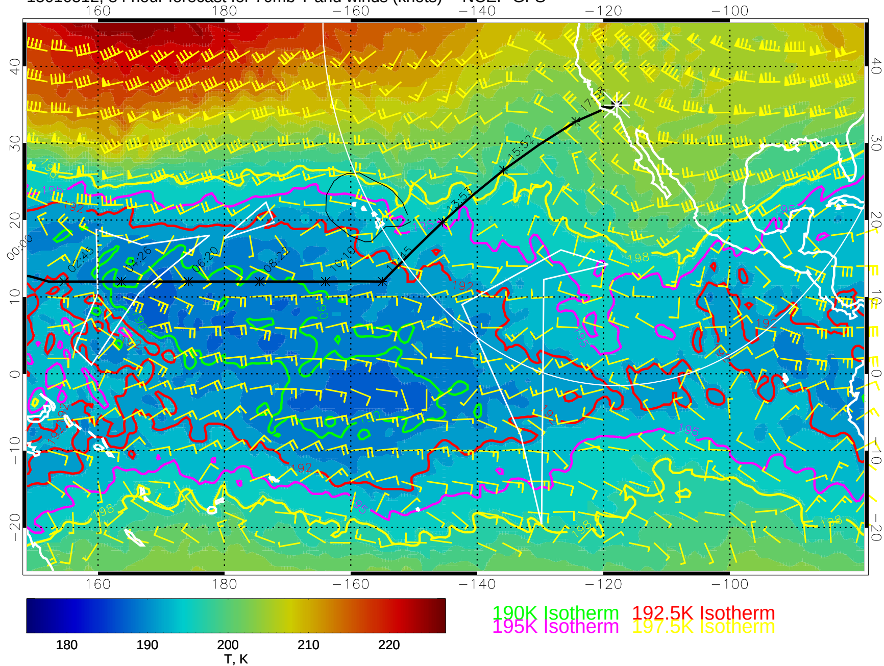
15010512, 84 hour forecast for 70mb T and winds (knots) -- NCEP GFS
