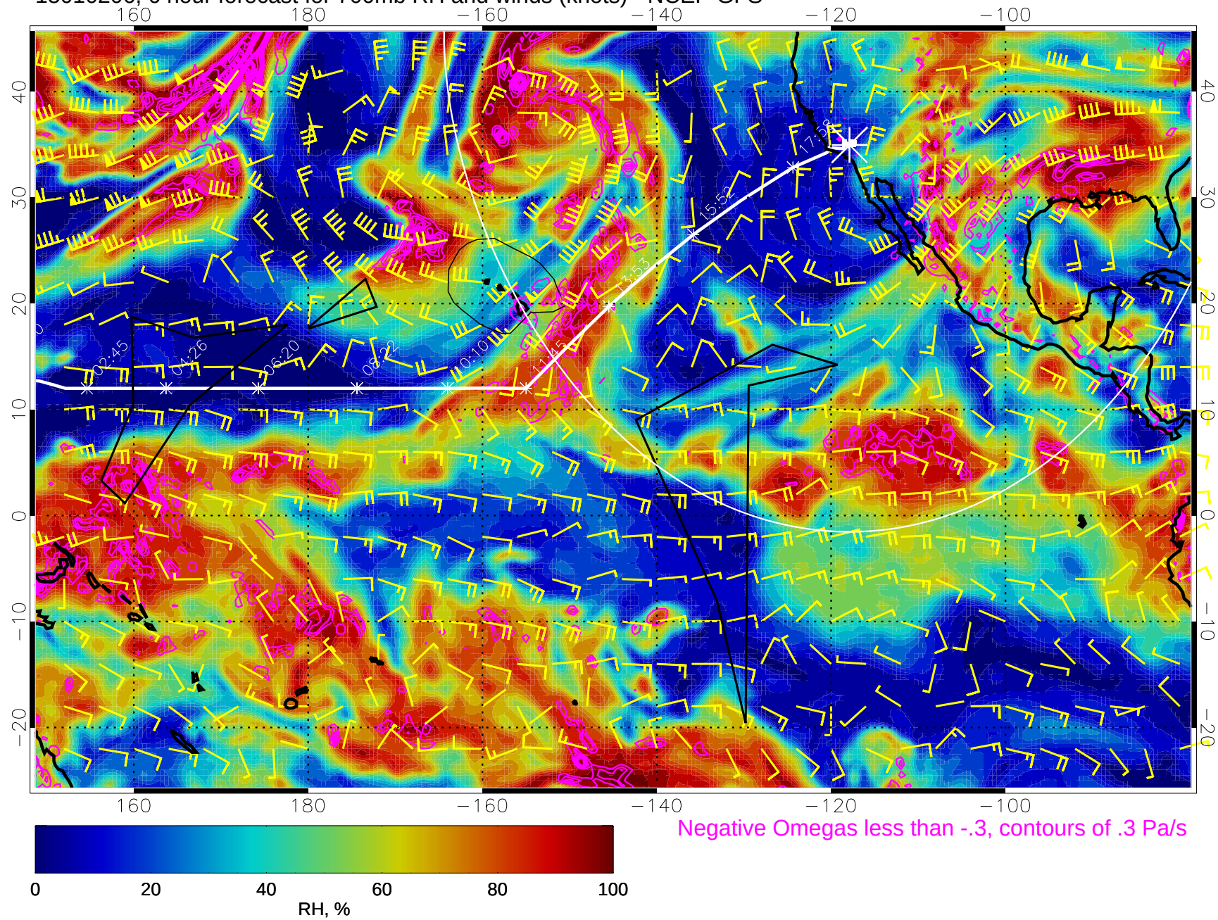
15010206, 6 hour forecast for 700mb RH and winds (knots) - NCEP GFS
