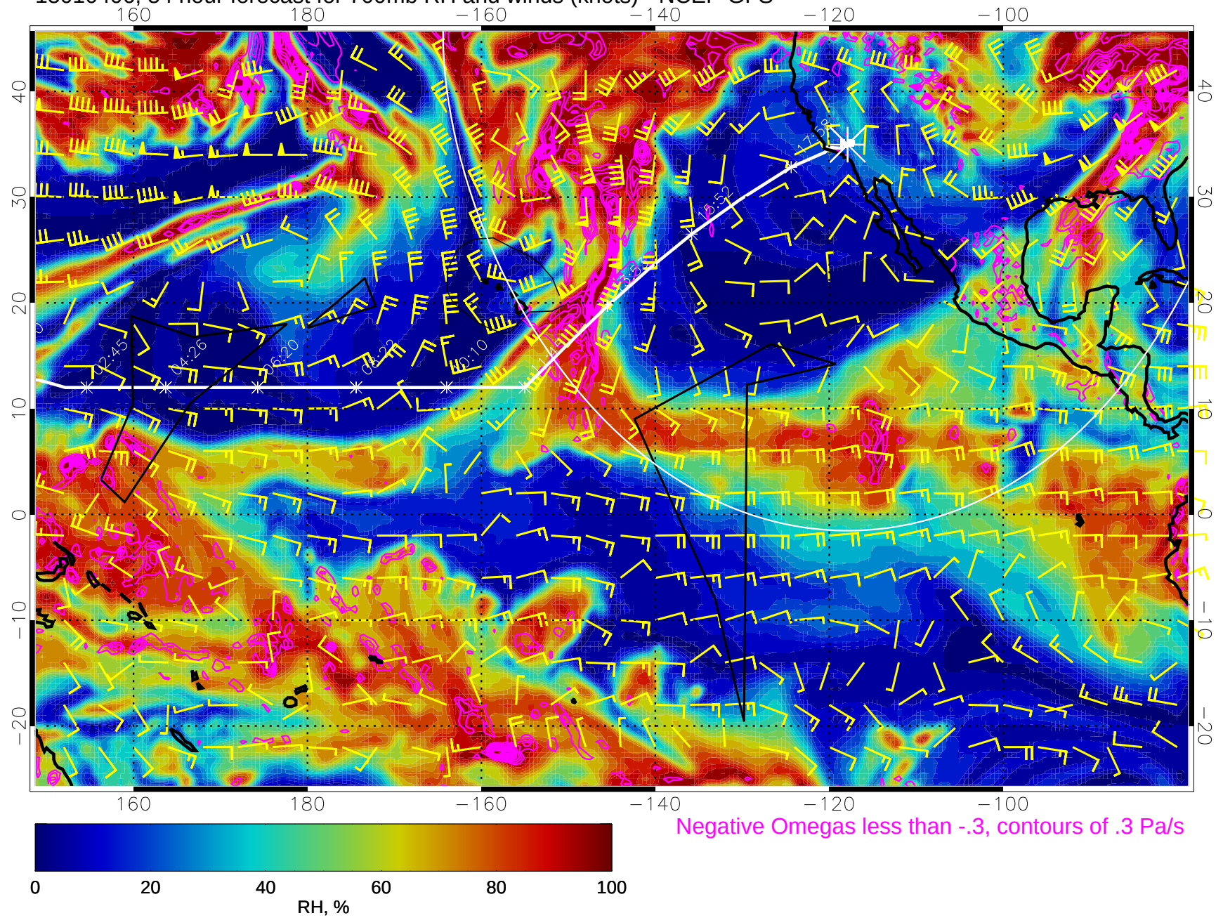
15010406, 54 hour forecast for 700mb RH and winds (knots) - NCEP GFS
