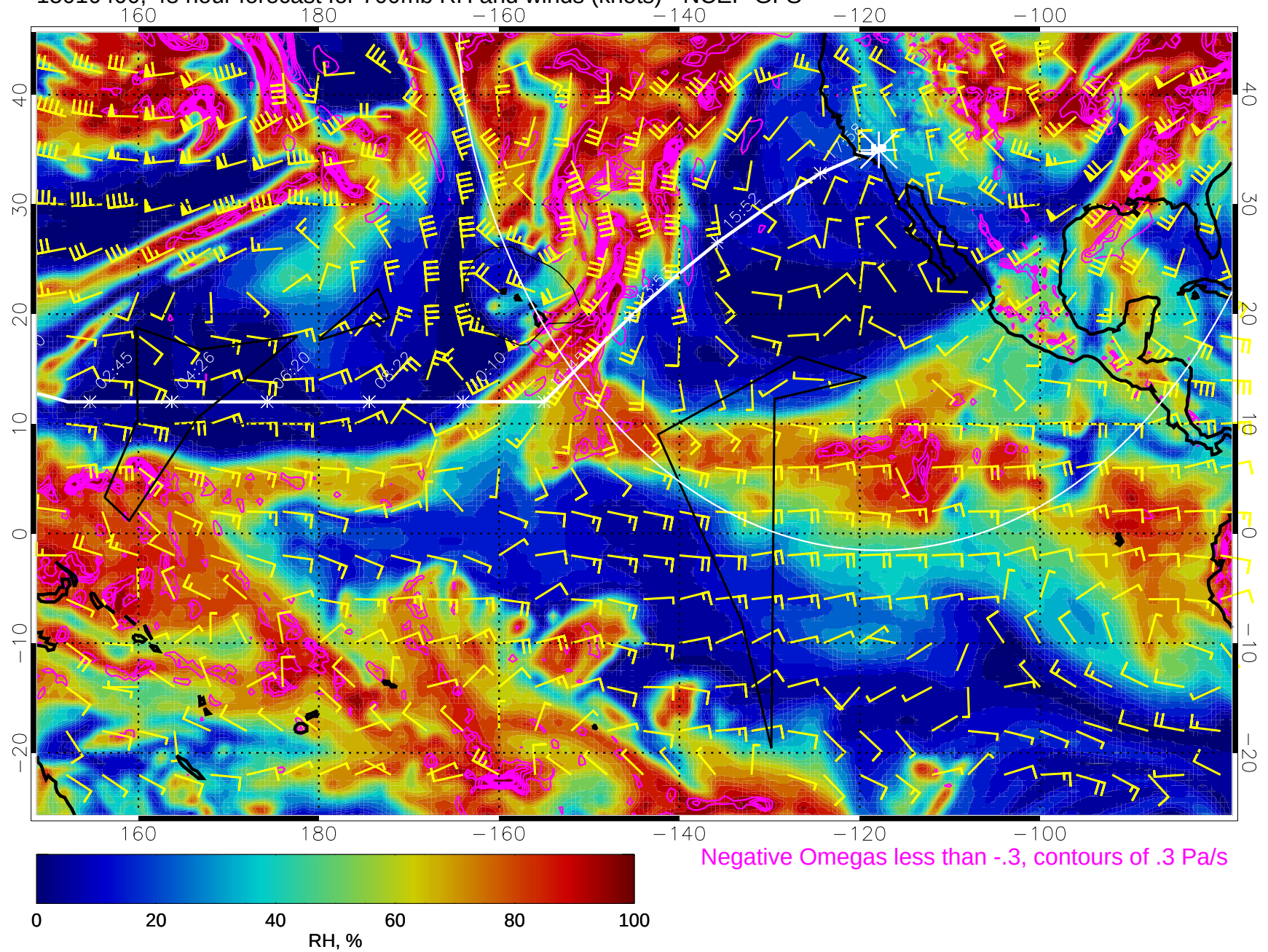
15010400, 48 hour forecast for 700mb RH and winds (knots) - NCEP GFS
