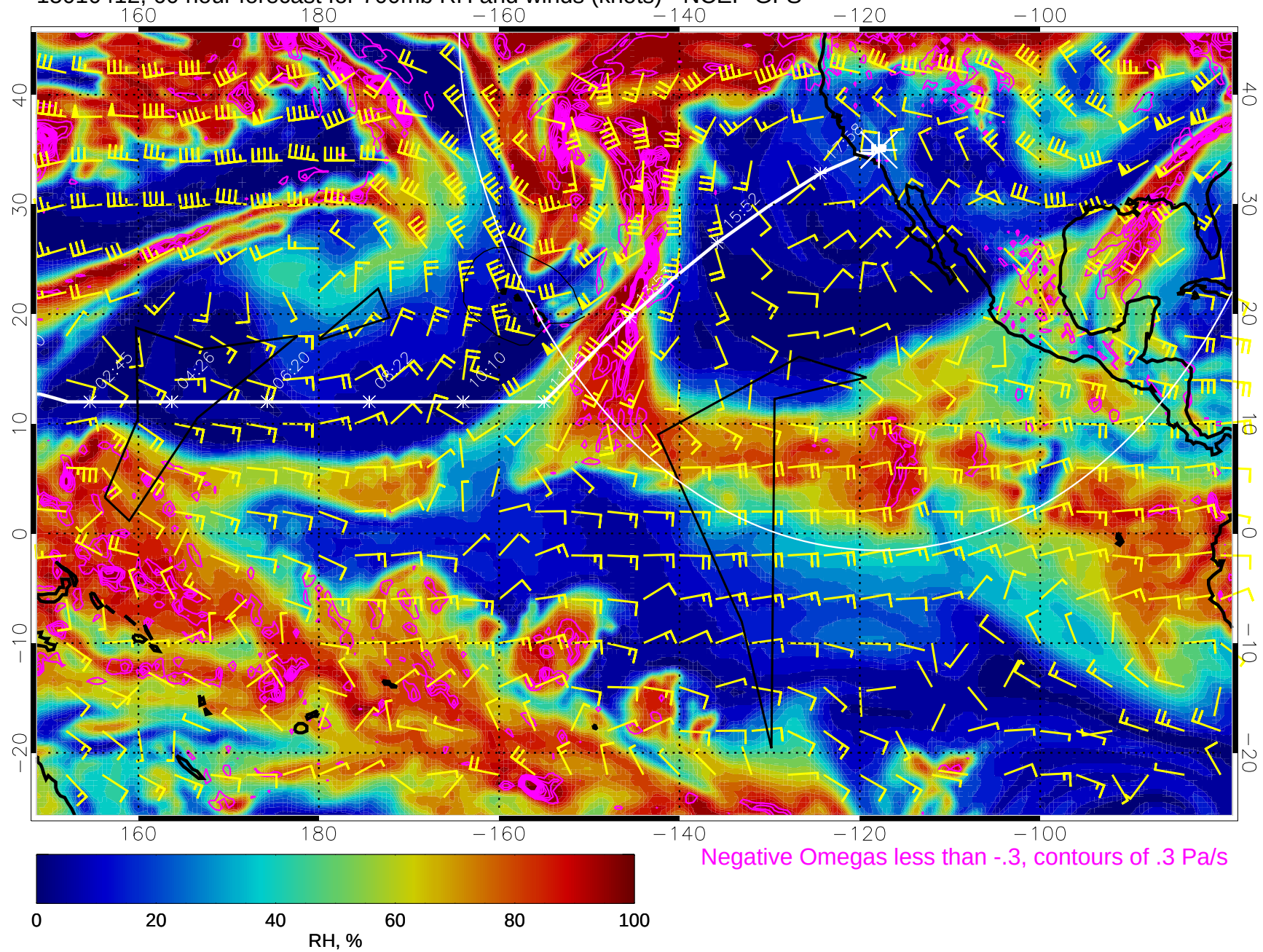
15010412, 60 hour forecast for 700mb RH and winds (knots) - NCEP GFS
