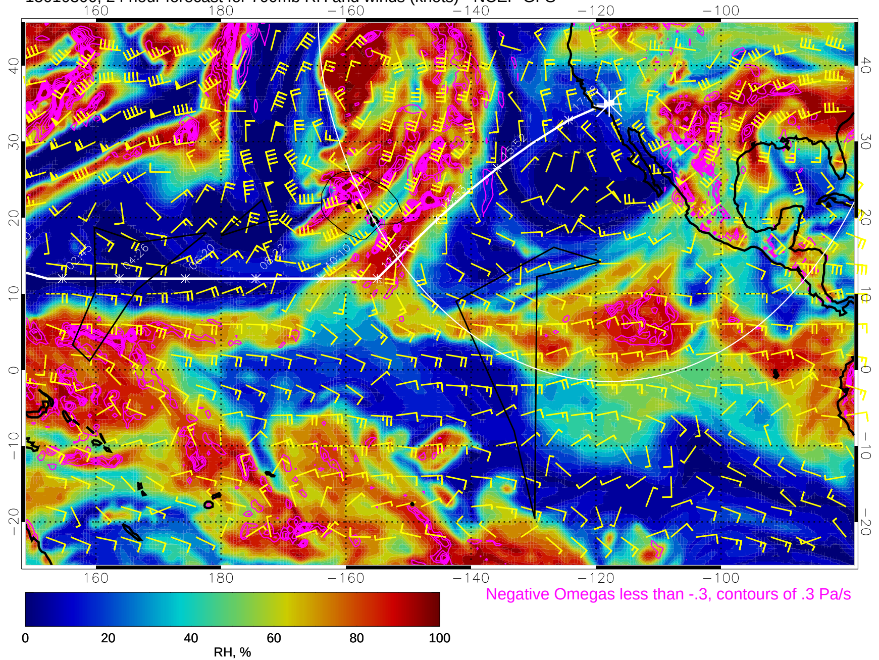
15010300, 24 hour forecast for 700mb RH and winds (knots) - NCEP GFS
