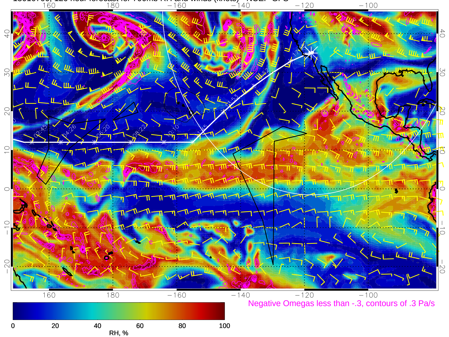
15010700, 120 hour forecast for 700mb RH and winds (knots) - NCEP GFS
