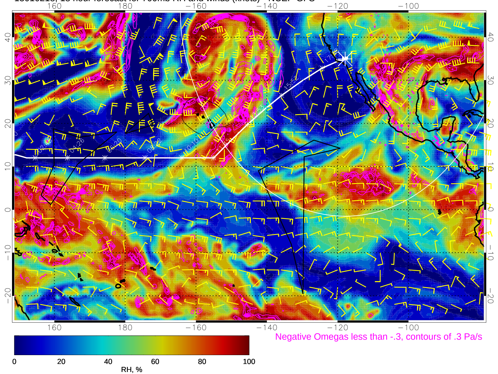
15010218, 18 hour forecast for 700mb RH and winds (knots) - NCEP GFS
