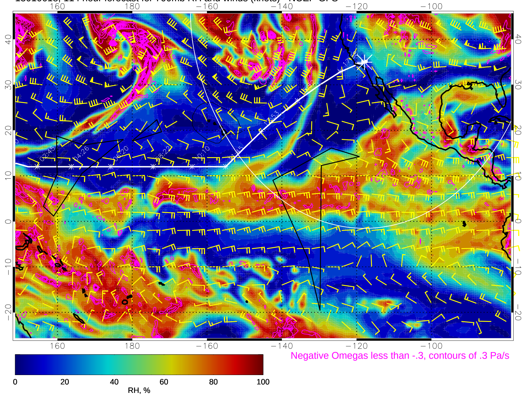
15010618, 114 hour forecast for 700mb RH and winds (knots) - NCEP GFS
