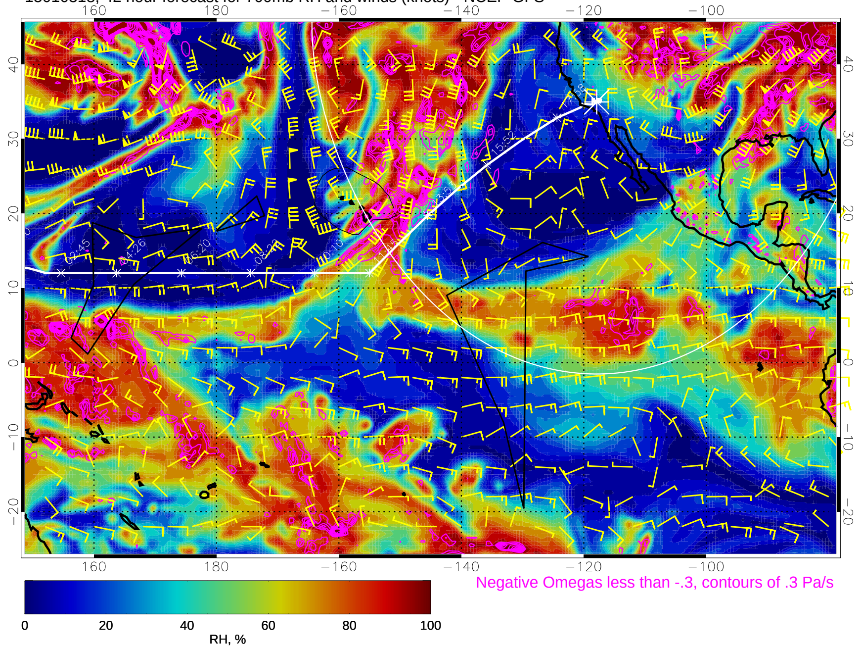
15010318, 42 hour forecast for 700mb RH and winds (knots) - NCEP GFS
