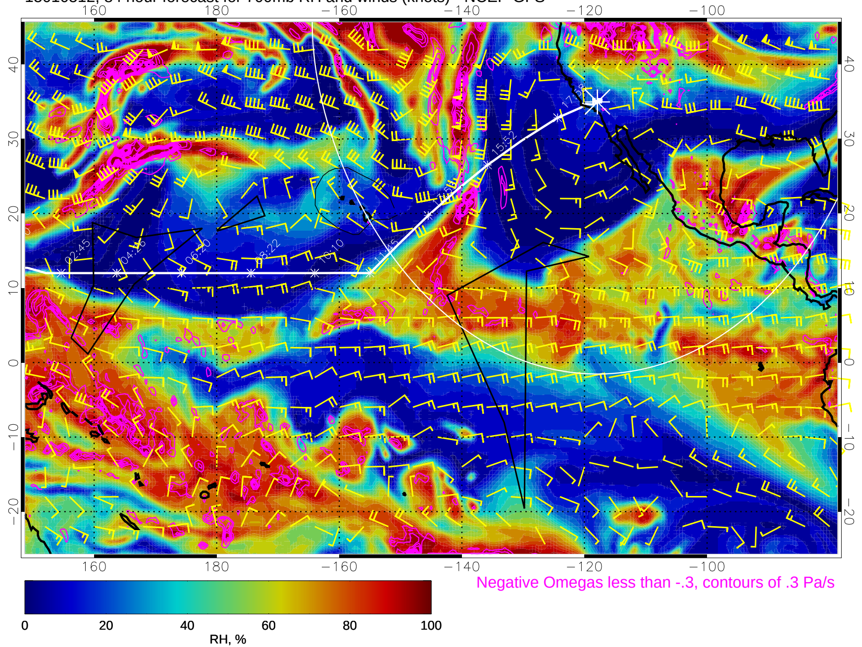
15010512, 84 hour forecast for 700mb RH and winds (knots) - NCEP GFS
