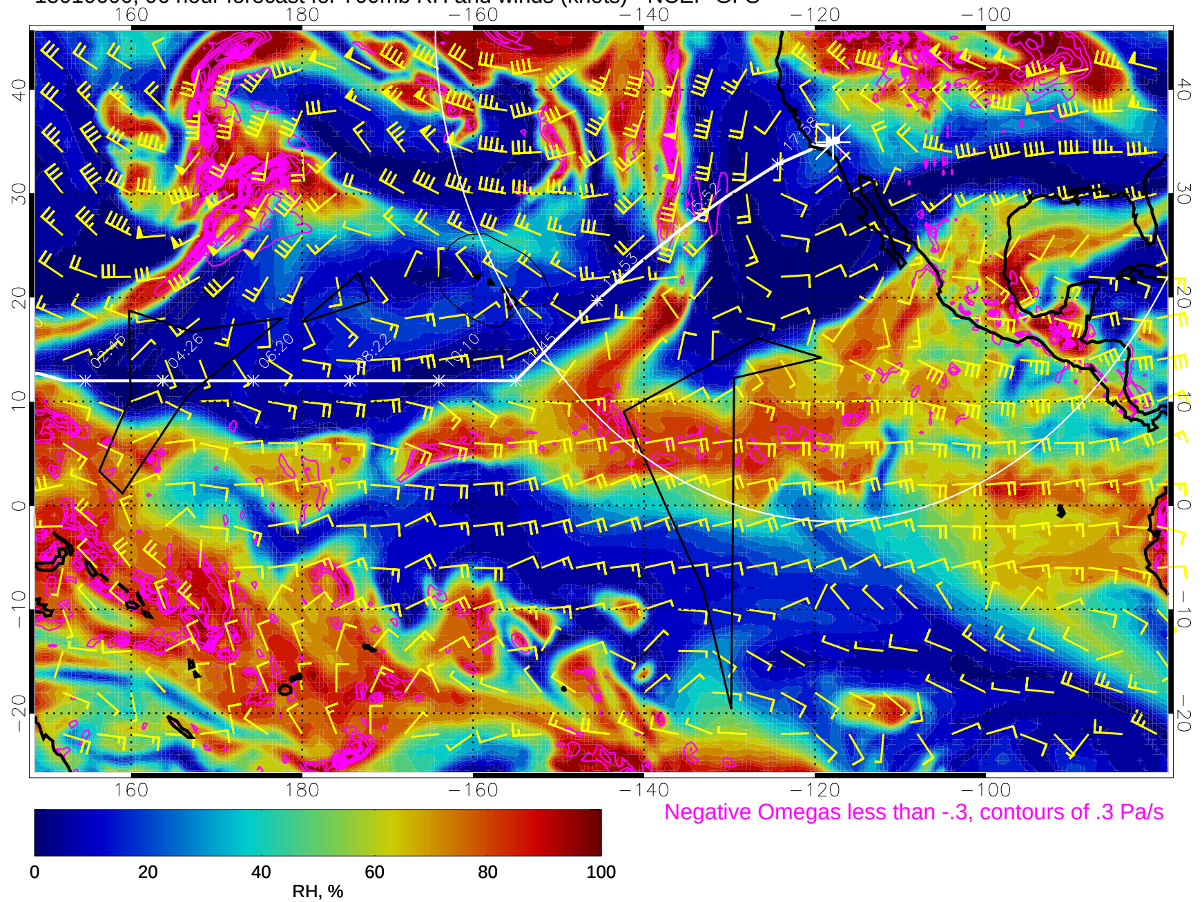
15010600, 96 hour forecast for 700mb RH and winds (knots) - NCEP GFS
