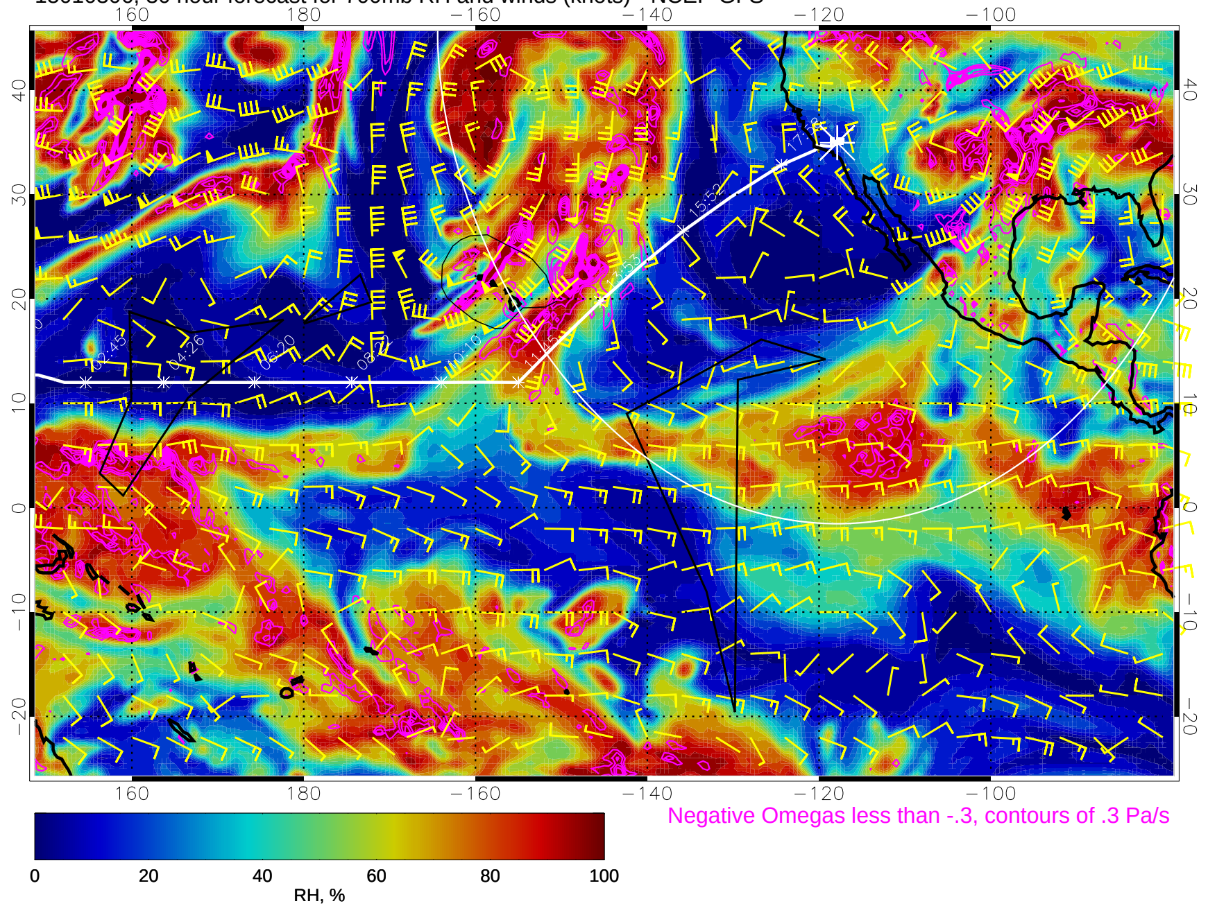
15010306, 30 hour forecast for 700mb RH and winds (knots) - NCEP GFS
