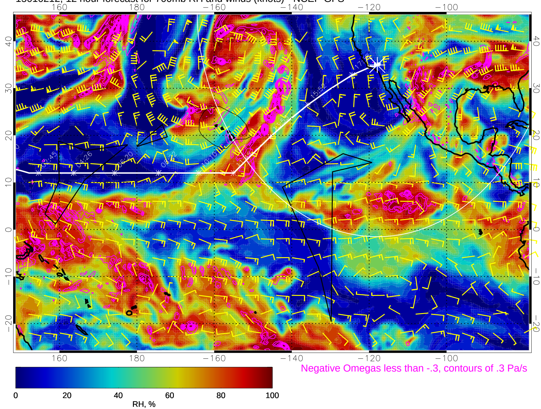
15010212, 12 hour forecast for 700mb RH and winds (knots) - NCEP GFS
