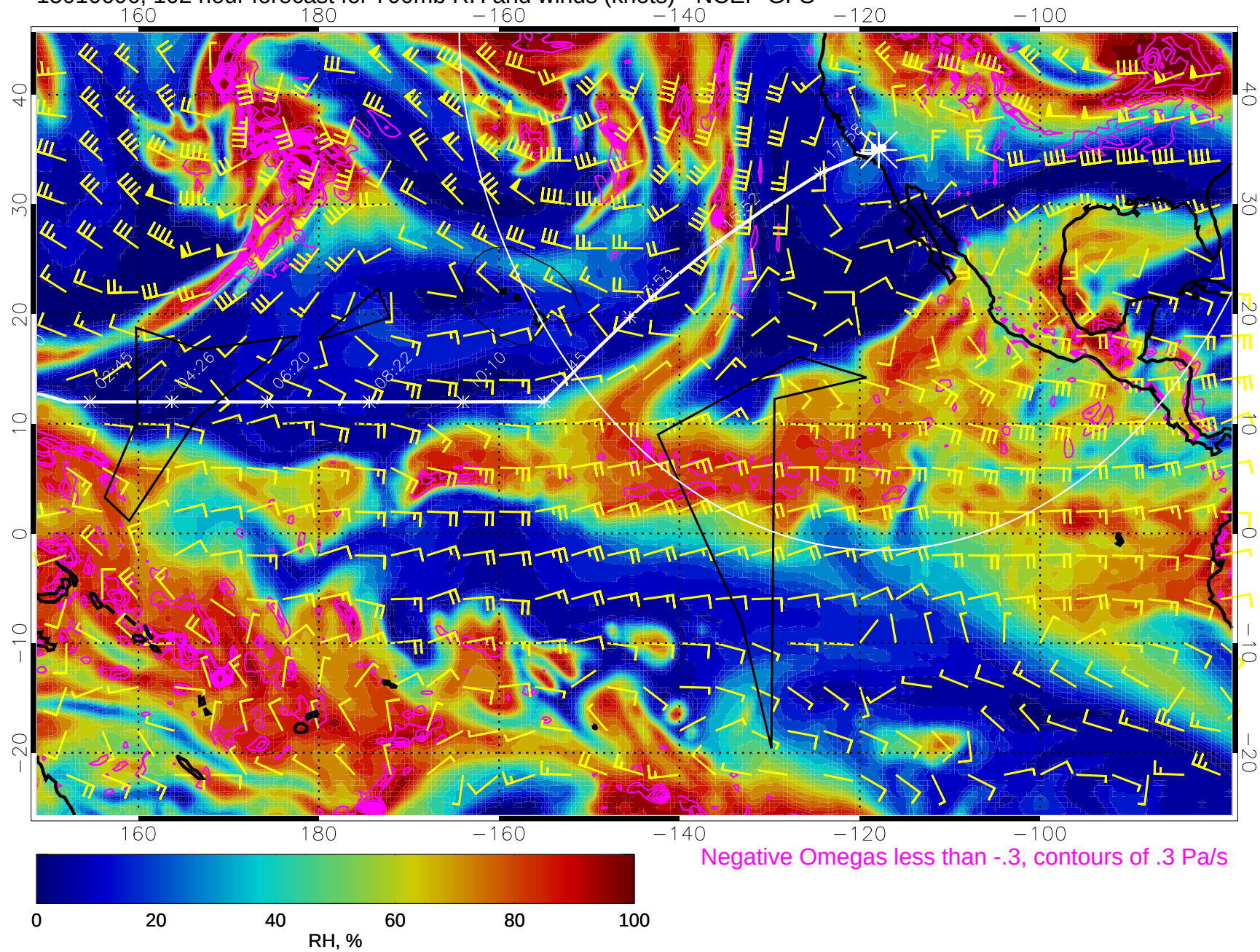
15010606, 102 hour forecast for 700mb RH and winds (knots) - NCEP GFS
