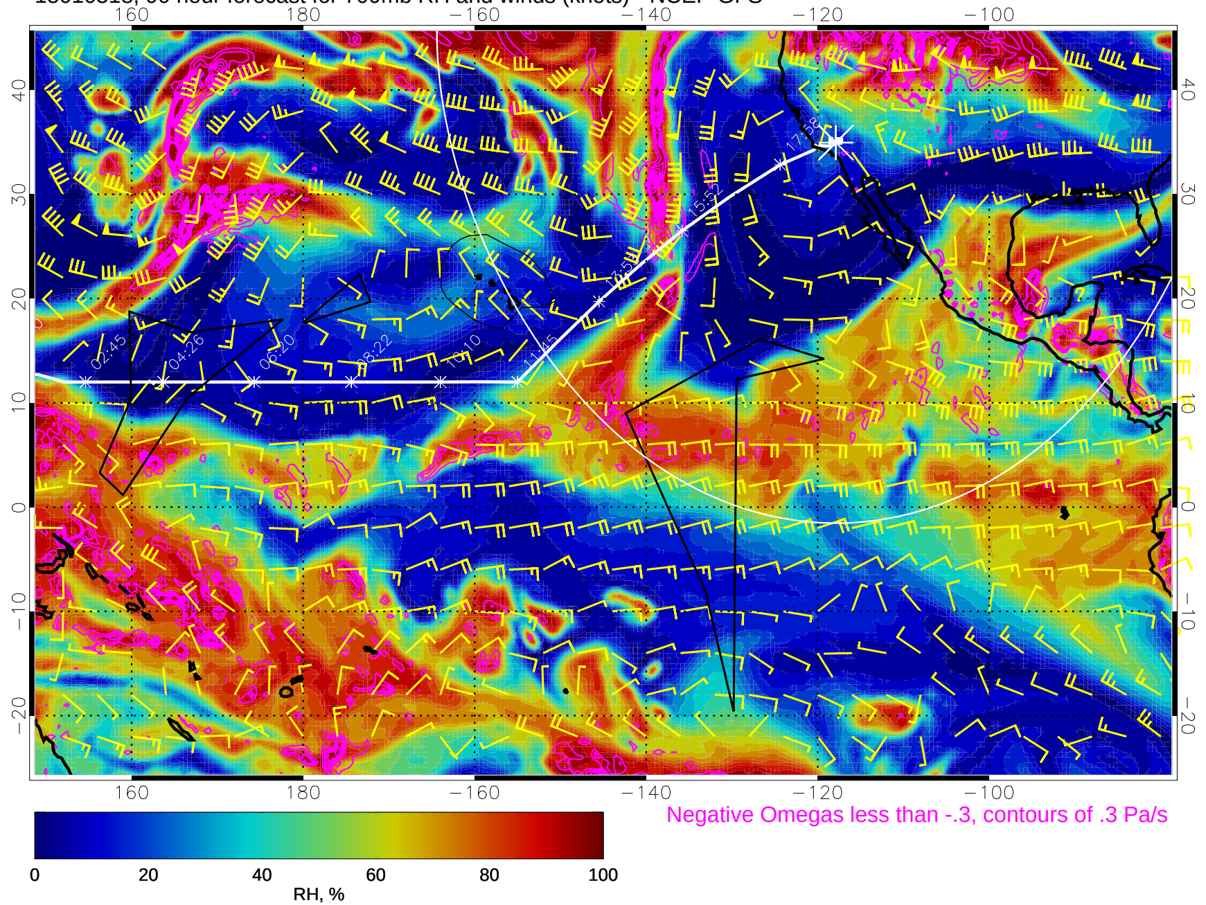
15010518, 90 hour forecast for 700mb RH and winds (knots) - NCEP GFS
