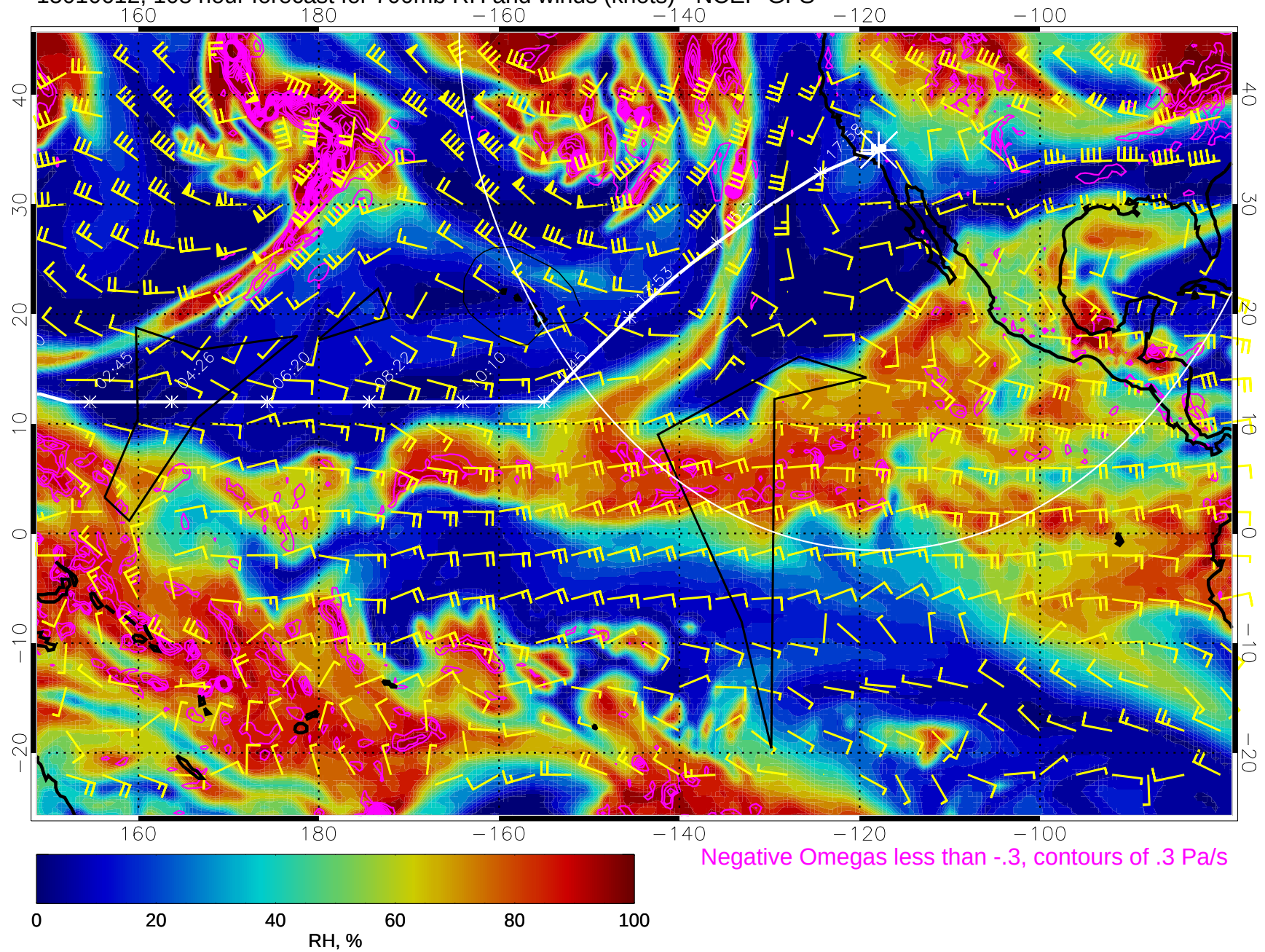
15010612, 108 hour forecast for 700mb RH and winds (knots) - NCEP GFS
