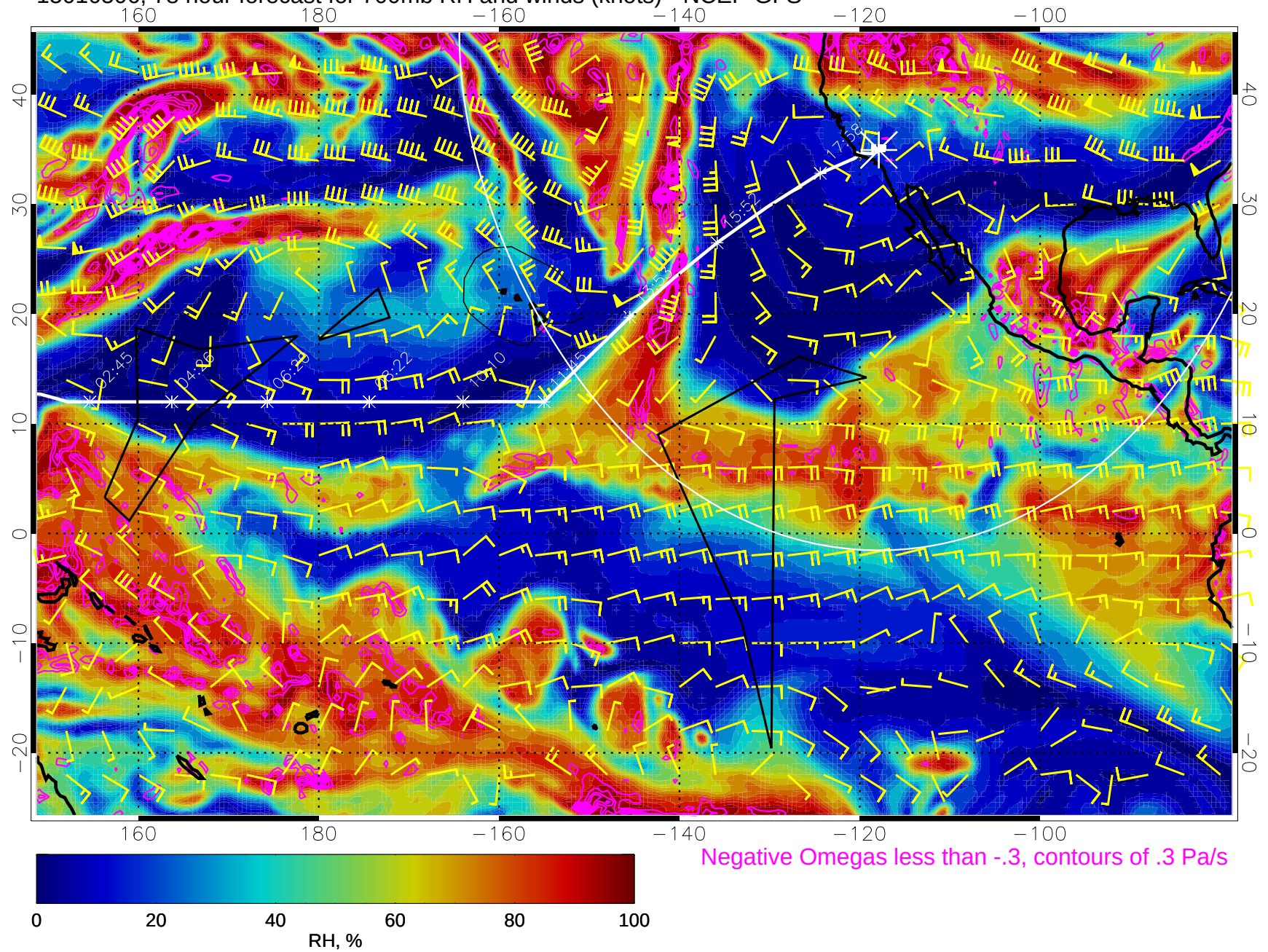
15010506, 78 hour forecast for 700mb RH and winds (knots) - NCEP GFS
