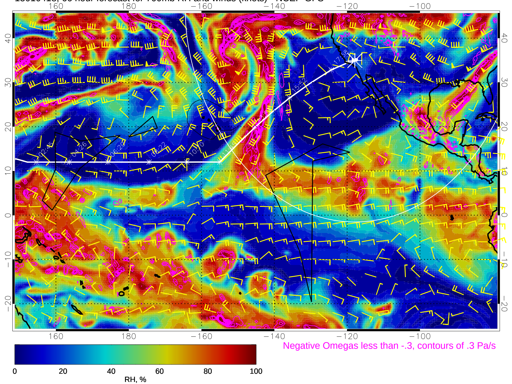
15010418, 66 hour forecast for 700mb RH and winds (knots) - NCEP GFS
