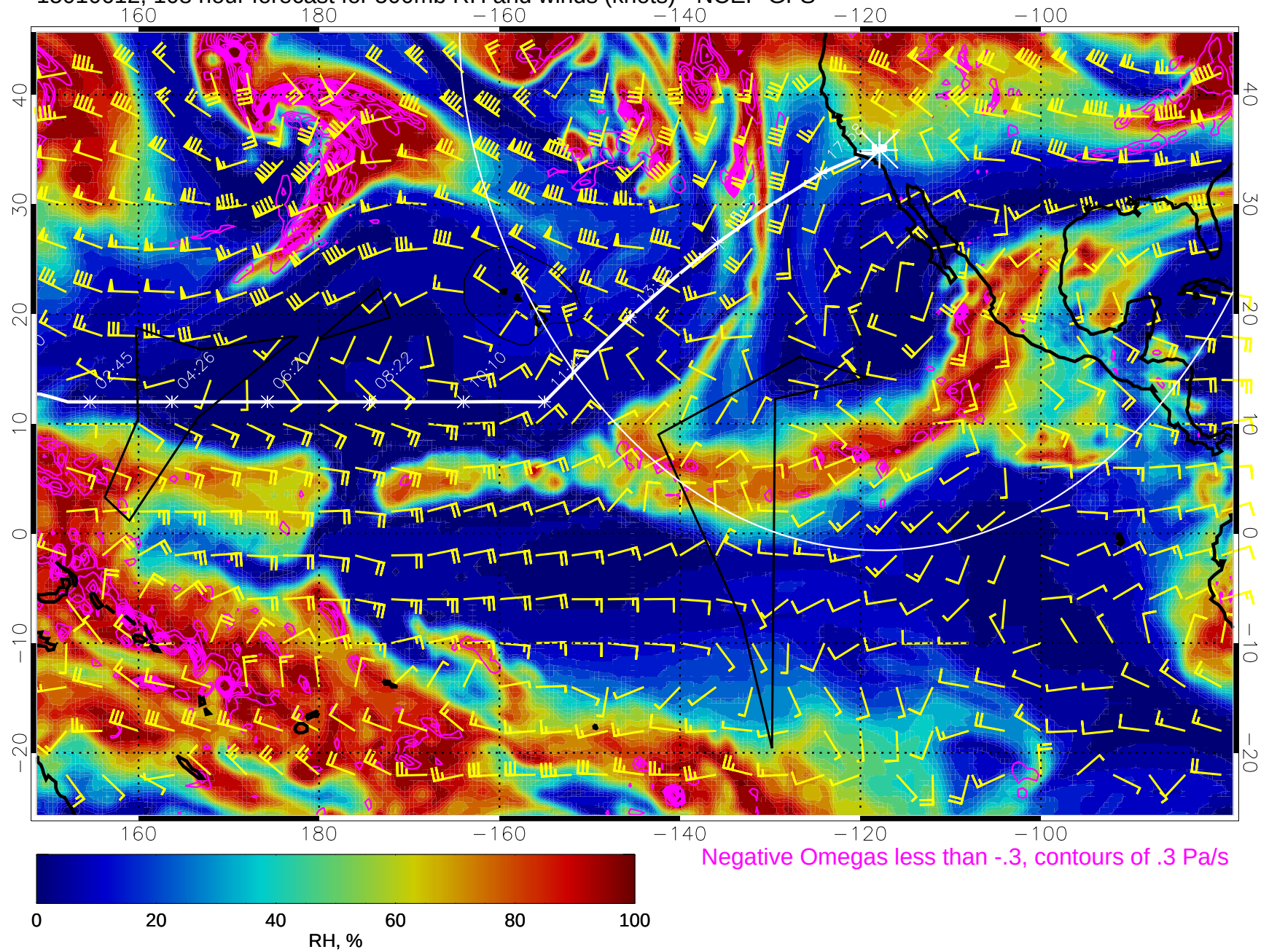
15010612, 108 hour forecast for 500mb RH and winds (knots) - NCEP GFS
