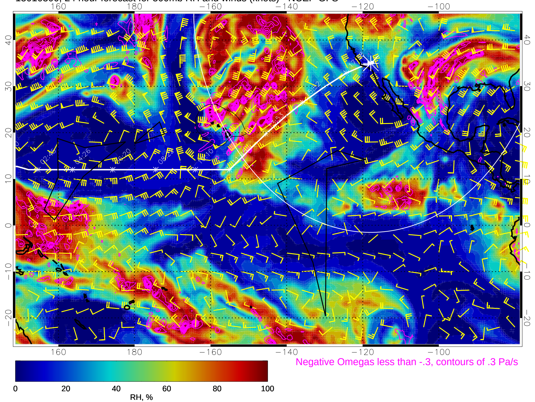
15010300, 24 hour forecast for 500mb RH and winds (knots) - NCEP GFS
