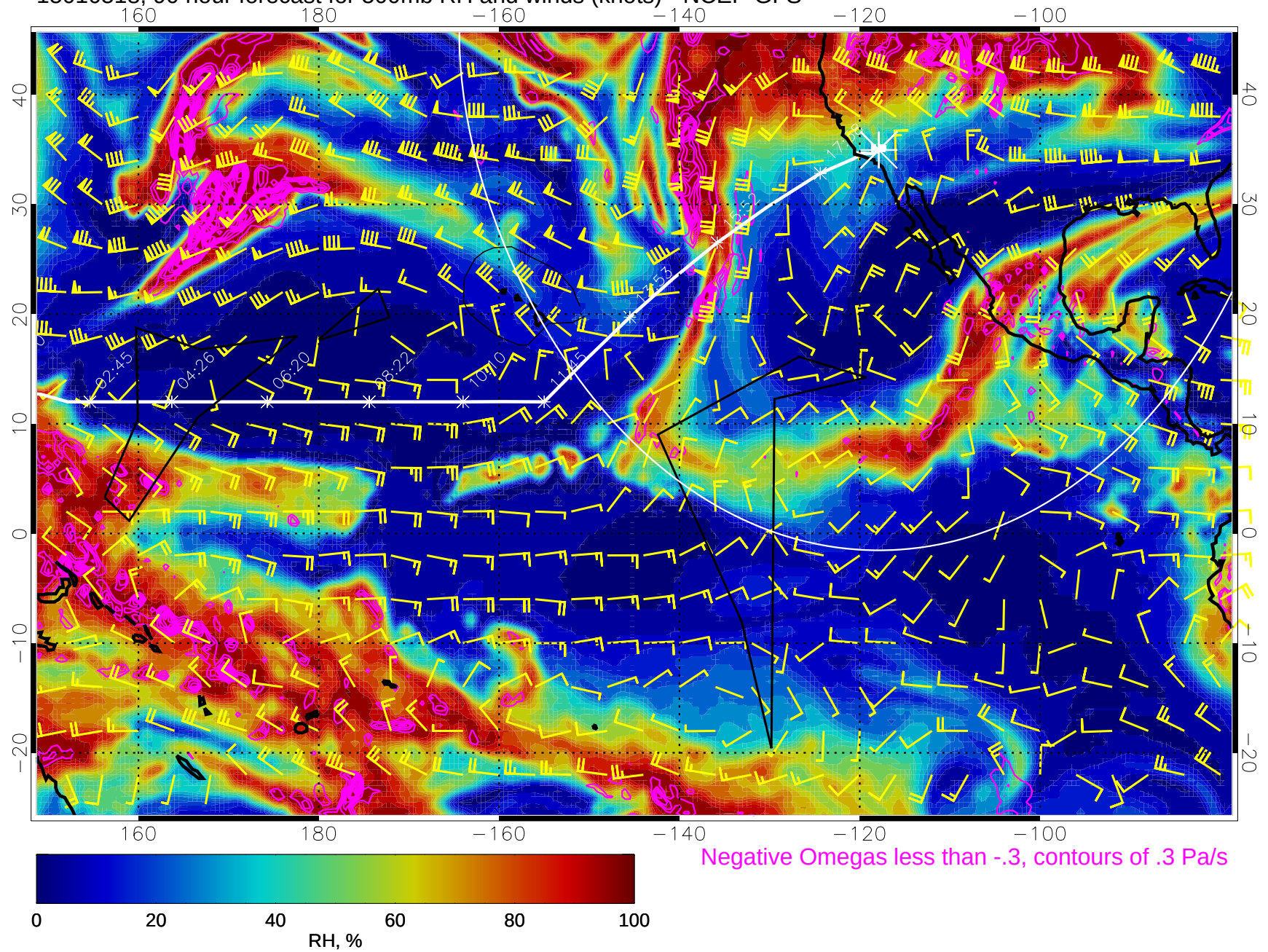
15010518, 90 hour forecast for 500mb RH and winds (knots) - NCEP GFS
