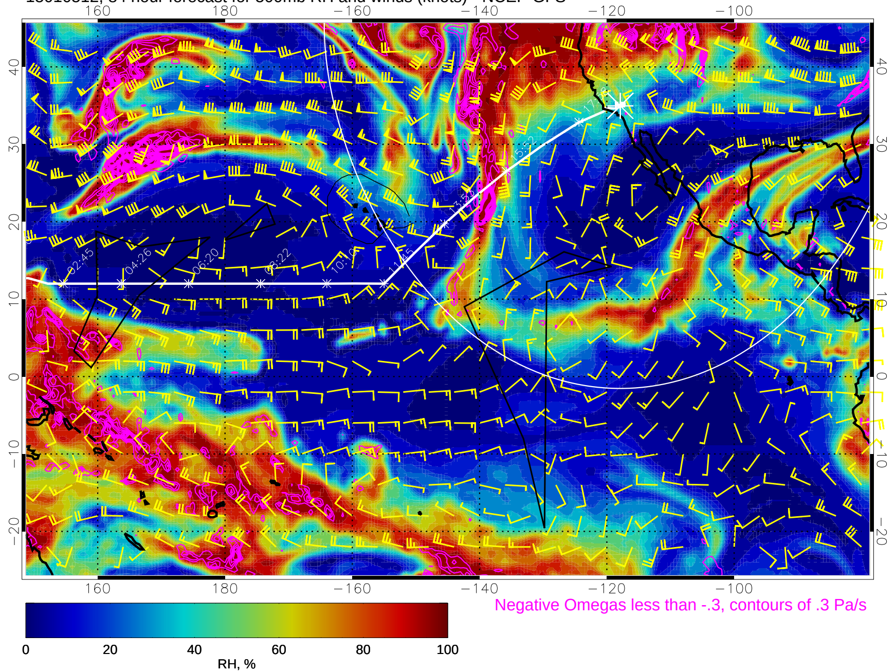
15010512, 84 hour forecast for 500mb RH and winds (knots) - NCEP GFS
