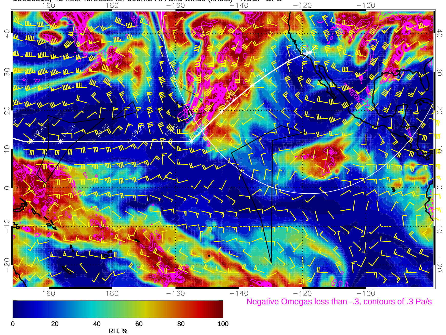
15010318, 42 hour forecast for 500mb RH and winds (knots) - NCEP GFS
