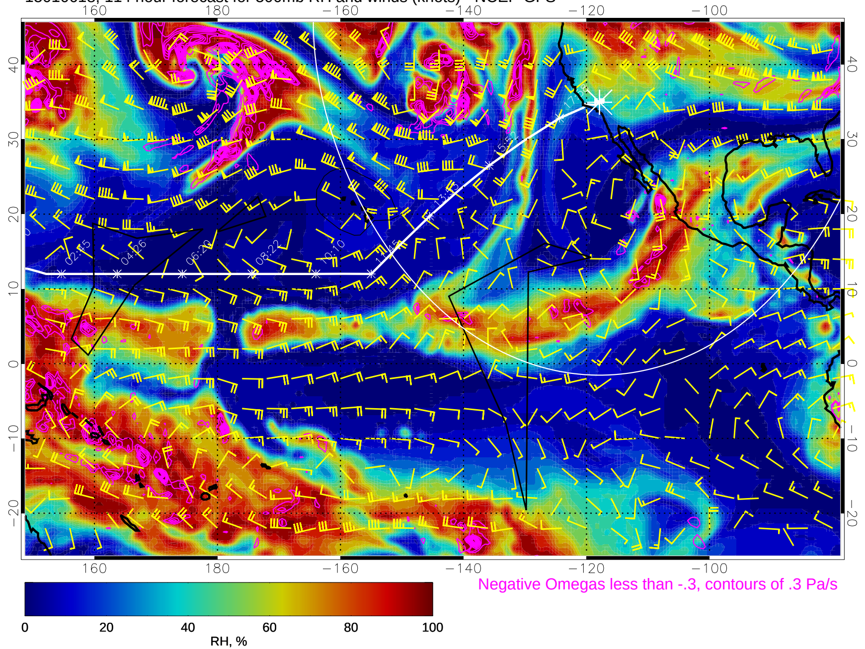
15010618, 114 hour forecast for 500mb RH and winds (knots) - NCEP GFS
