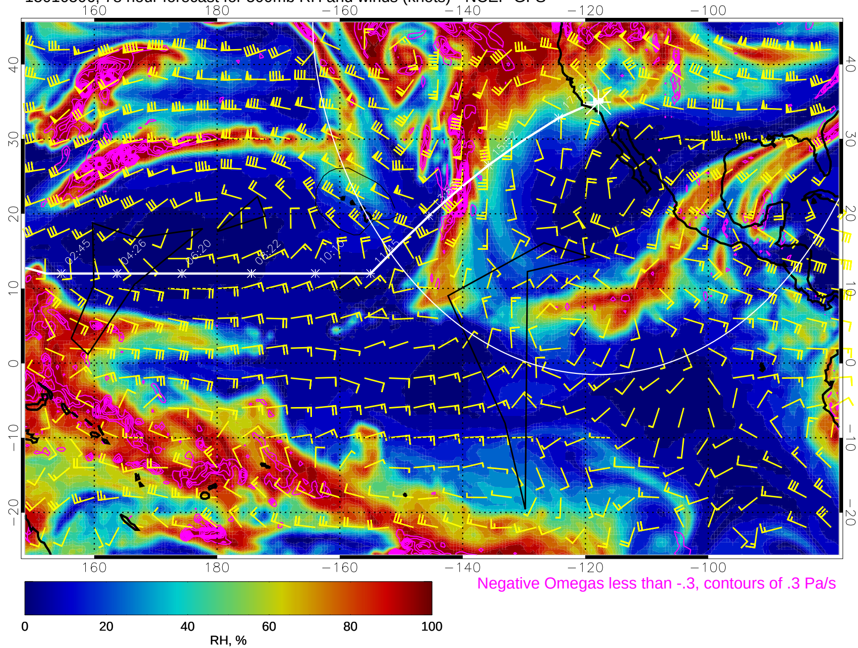
15010506, 78 hour forecast for 500mb RH and winds (knots) - NCEP GFS
