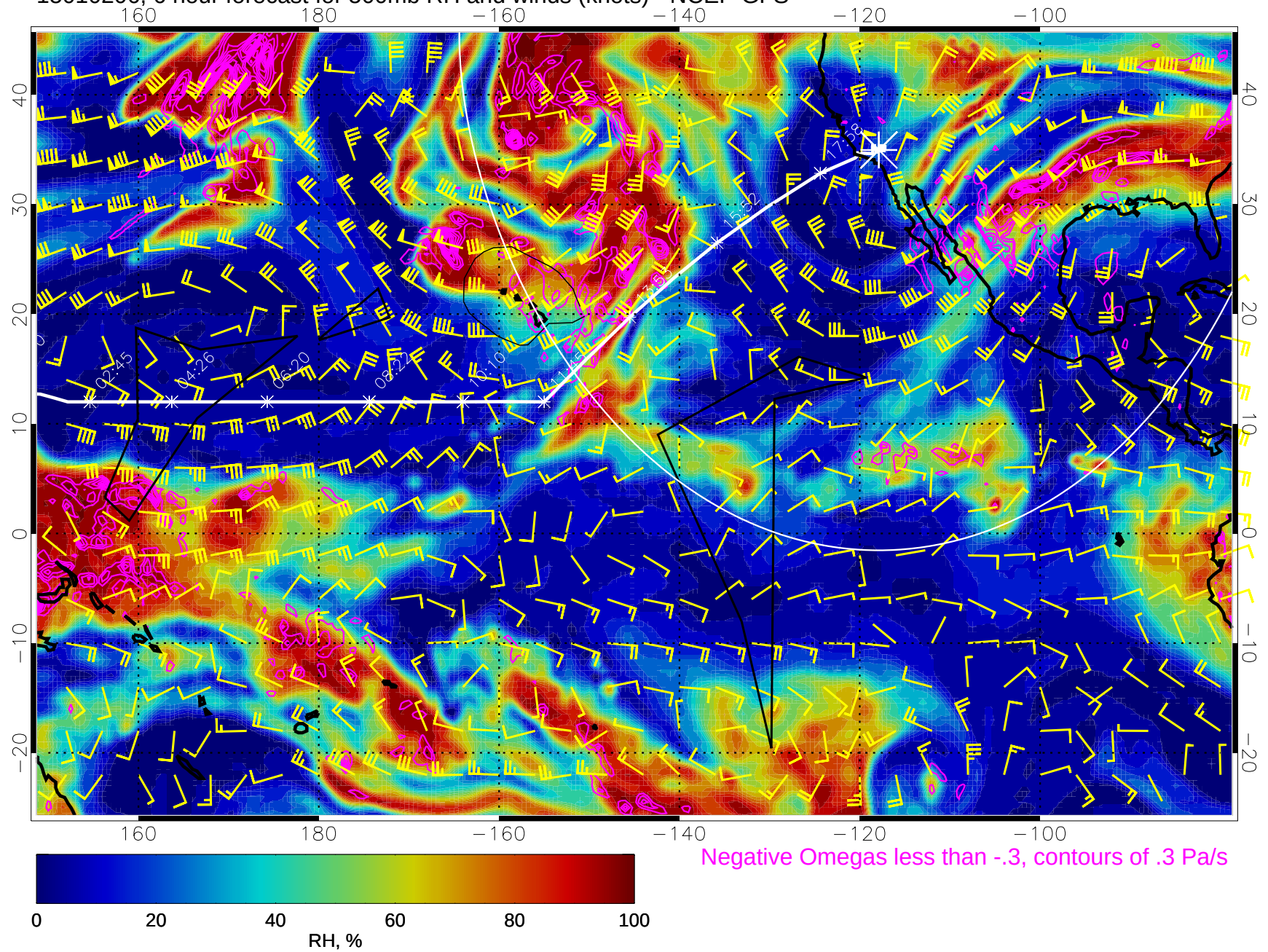
15010206, 6 hour forecast for 500mb RH and winds (knots) - NCEP GFS
