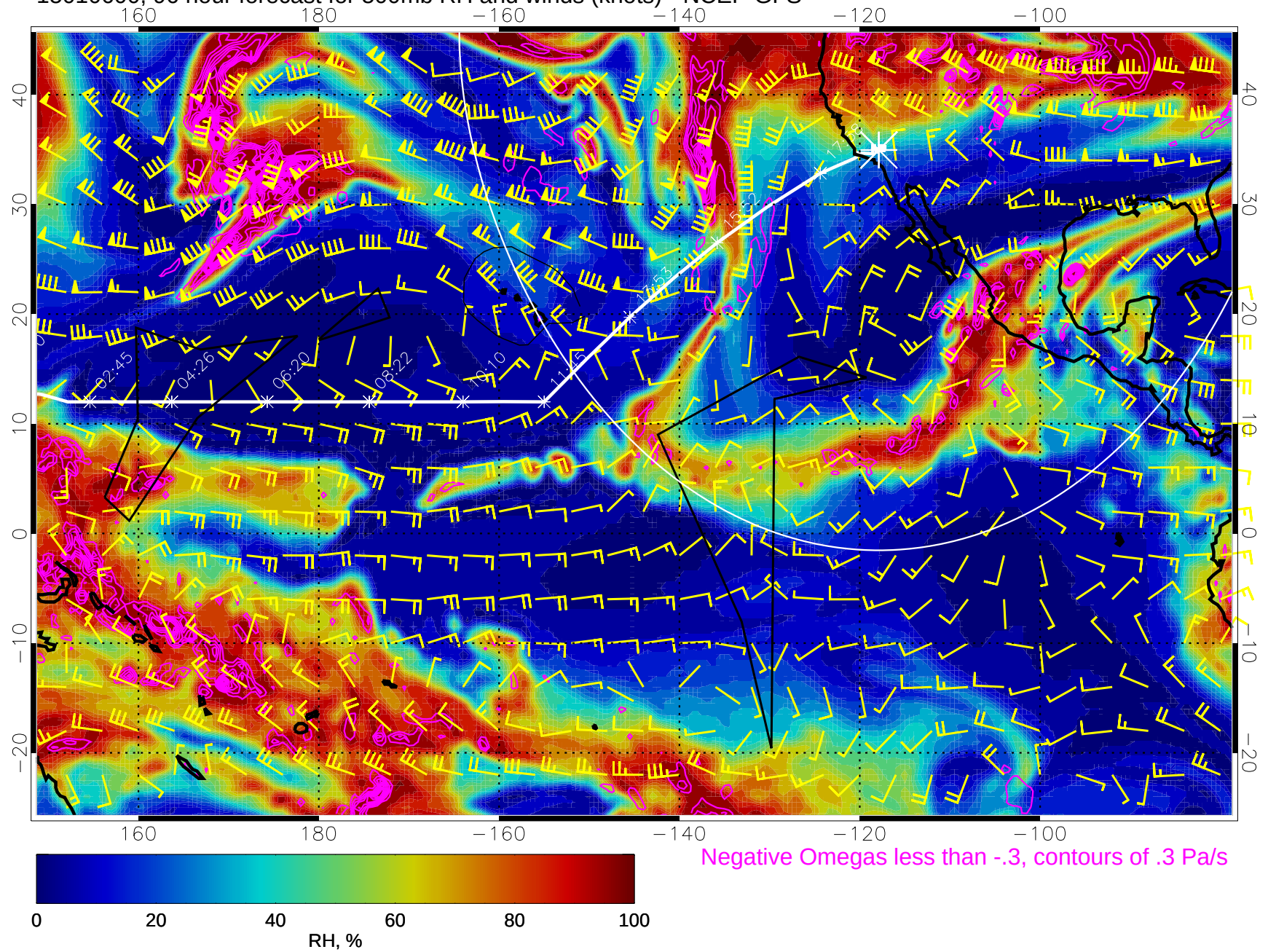
15010600, 96 hour forecast for 500mb RH and winds (knots) - NCEP GFS
