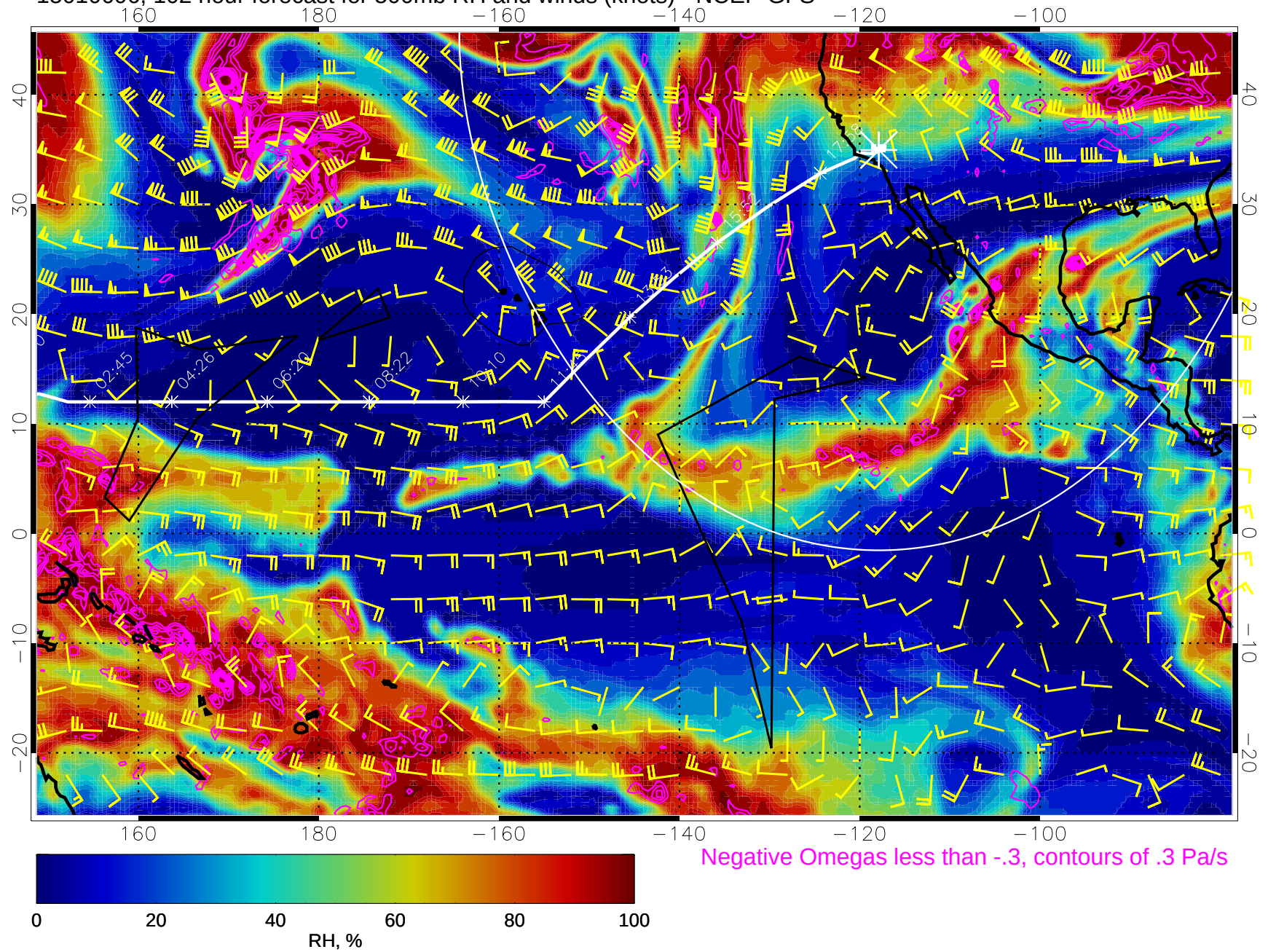
15010606, 102 hour forecast for 500mb RH and winds (knots) - NCEP GFS
