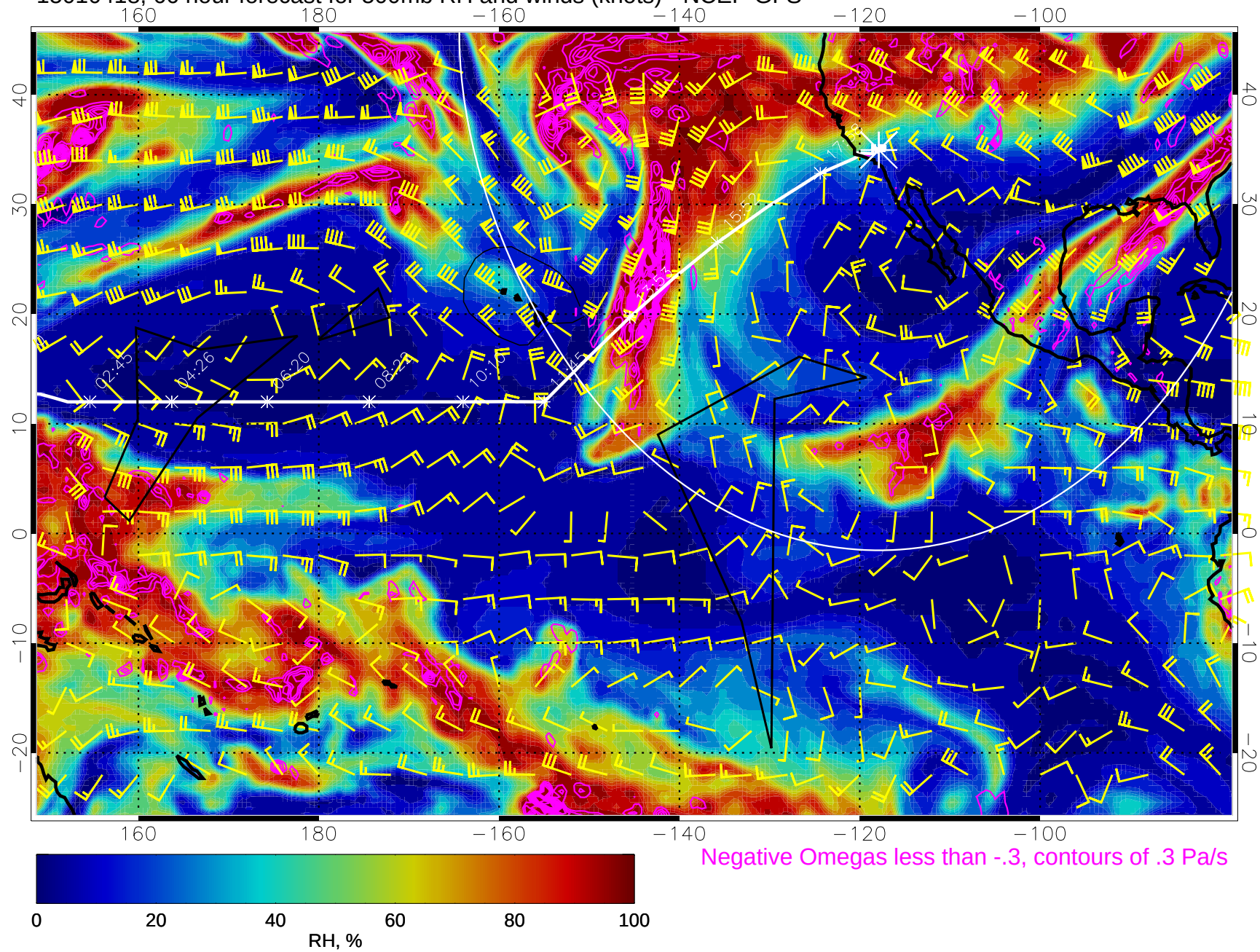
15010418, 66 hour forecast for 500mb RH and winds (knots) - NCEP GFS
