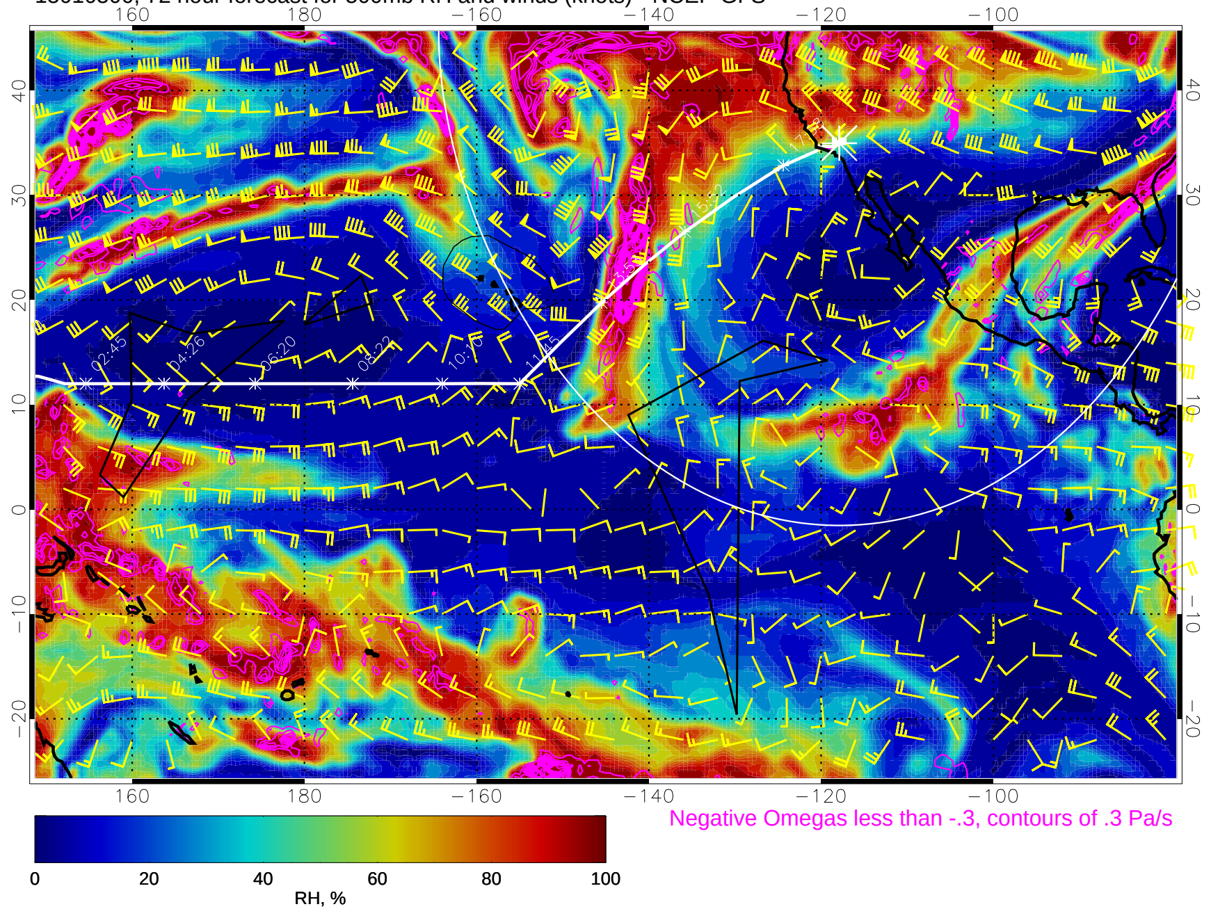
15010500, 72 hour forecast for 500mb RH and winds (knots) - NCEP GFS
