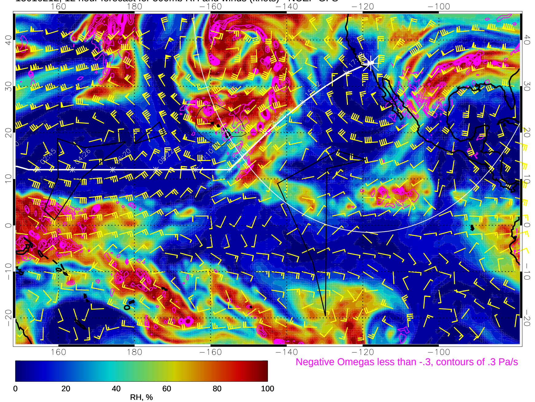
15010212, 12 hour forecast for 500mb RH and winds (knots) - NCEP GFS
