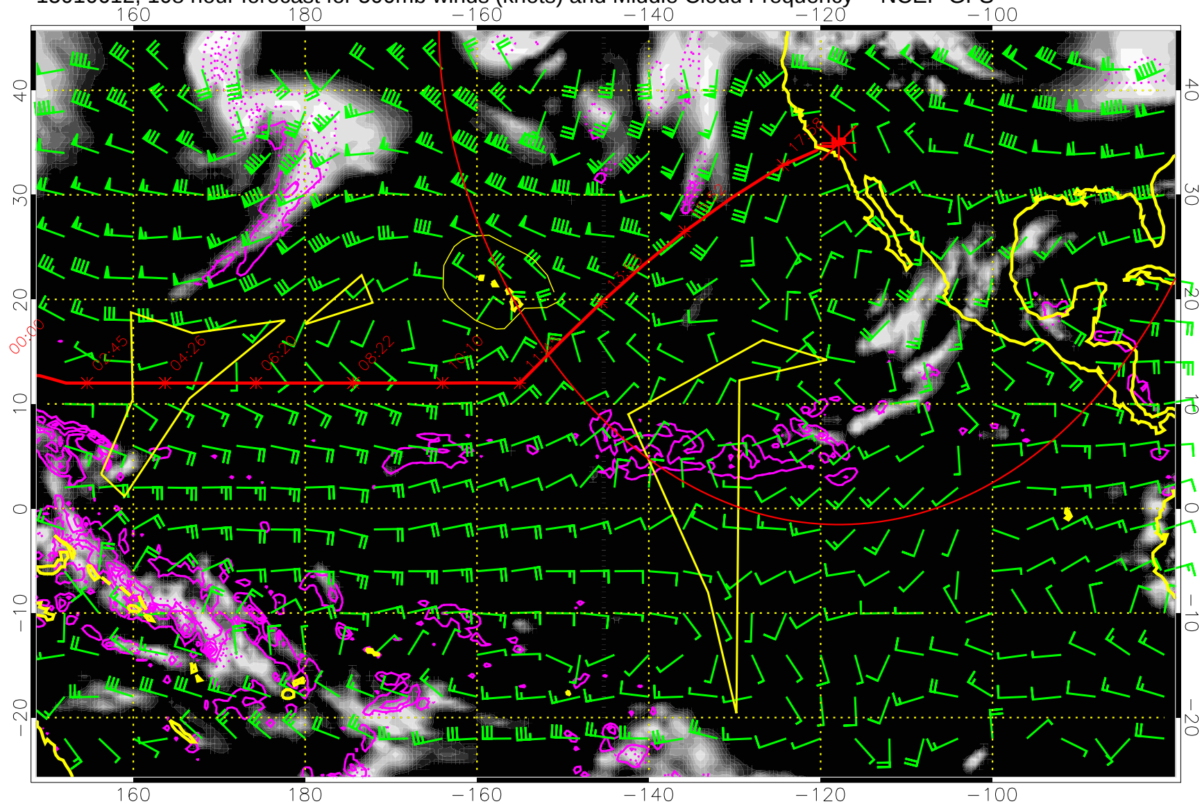
15010612, 108 hour forecast for 500mb winds (knots) and Middle Cloud Frequency -- NCEP GFS
