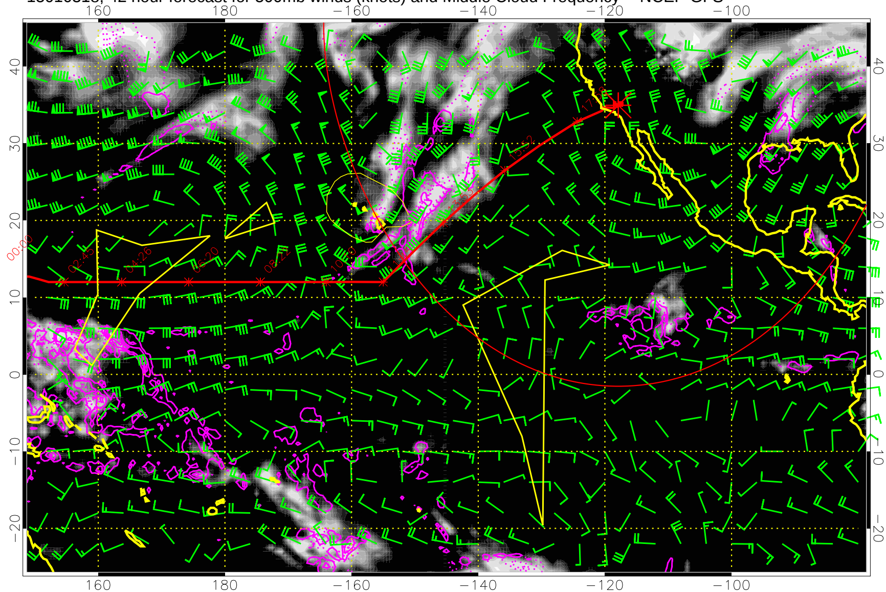
15010318, 42 hour forecast for 500mb winds (knots) and Middle Cloud Frequency -- NCEP GFS
