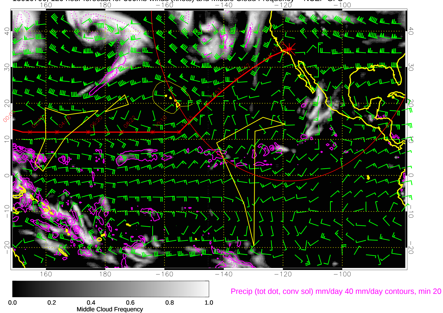
15010700, 120 hour forecast for 500mb winds (knots) and Middle Cloud Frequency -- NCEP GFS
