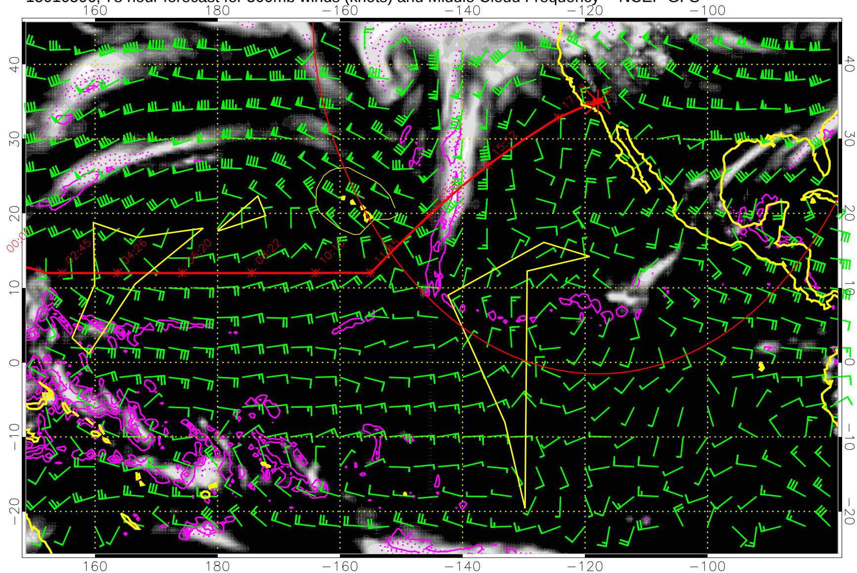
15010506, 78 hour forecast for 500mb winds (knots) and Middle Cloud Frequency -- NCEP GFS
