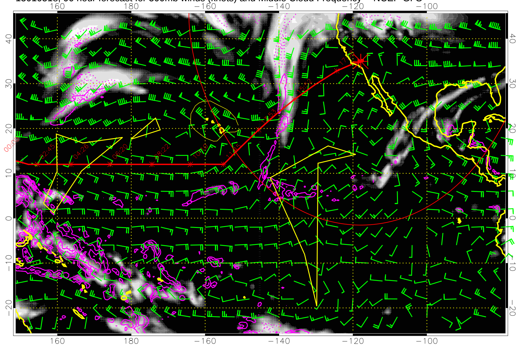
15010518, 90 hour forecast for 500mb winds (knots) and Middle Cloud Frequency -- NCEP GFS
