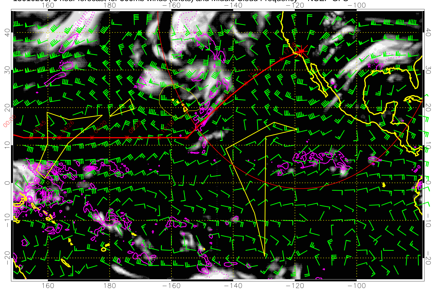
15010206, 6 hour forecast for 500mb winds (knots) and Middle Cloud Frequency -- NCEP GFS
