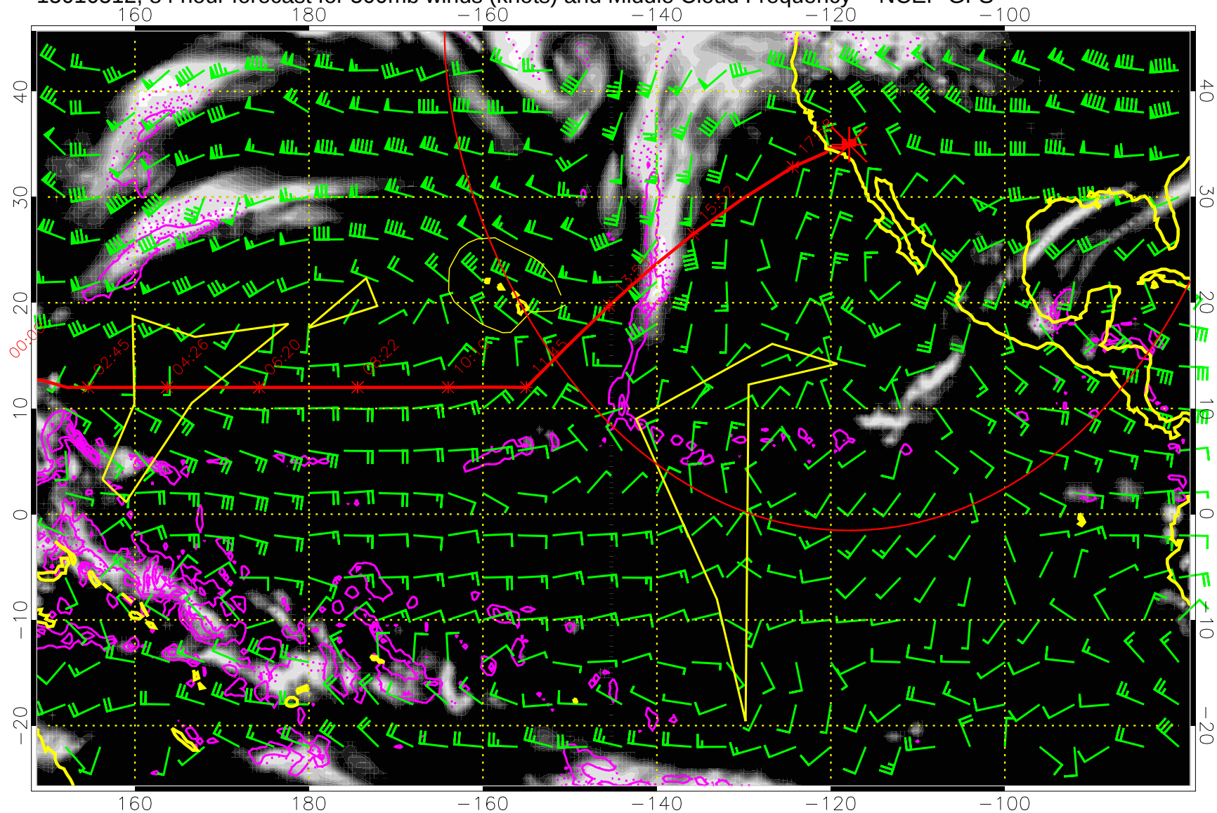
15010512, 84 hour forecast for 500mb winds (knots) and Middle Cloud Frequency -- NCEP GFS
