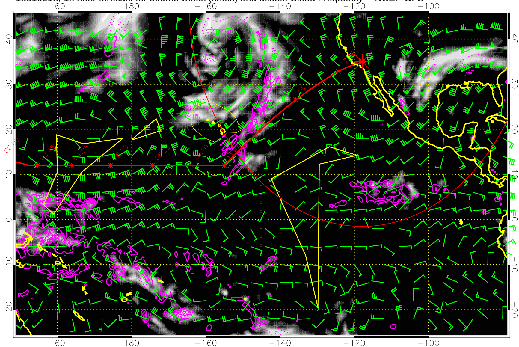
15010218, 18 hour forecast for 500mb winds (knots) and Middle Cloud Frequency -- NCEP GFS
