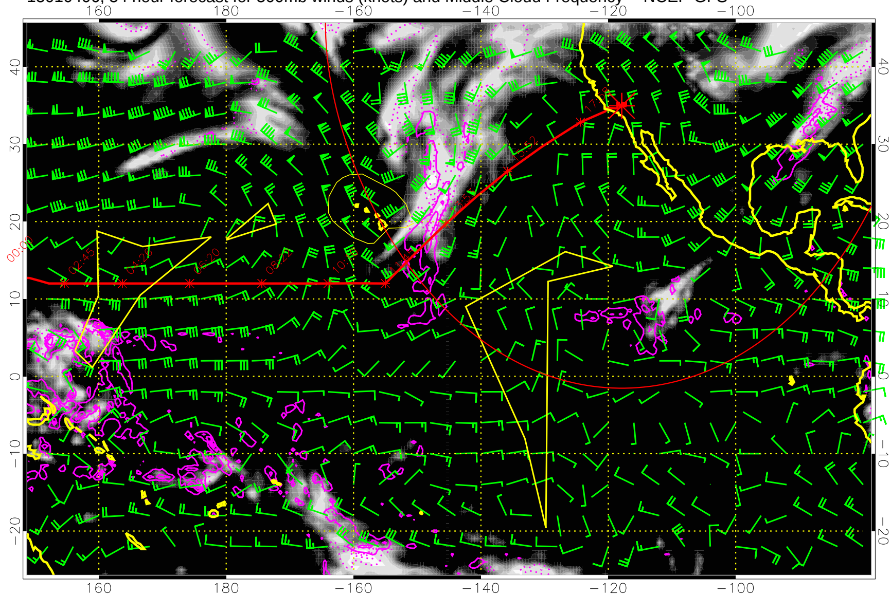
15010406, 54 hour forecast for 500mb winds (knots) and Middle Cloud Frequency -- NCEP GFS
