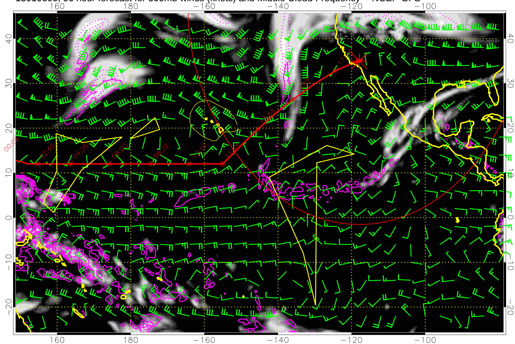
15010600, 96 hour forecast for 500mb winds (knots) and Middle Cloud Frequency -- NCEP GFS
