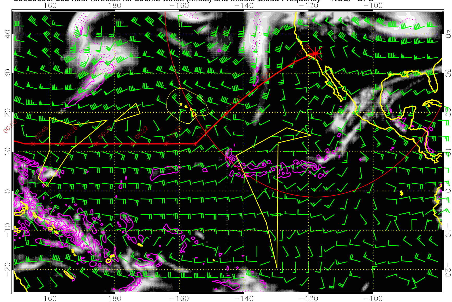
15010606, 102 hour forecast for 500mb winds (knots) and Middle Cloud Frequency -- NCEP GFS
