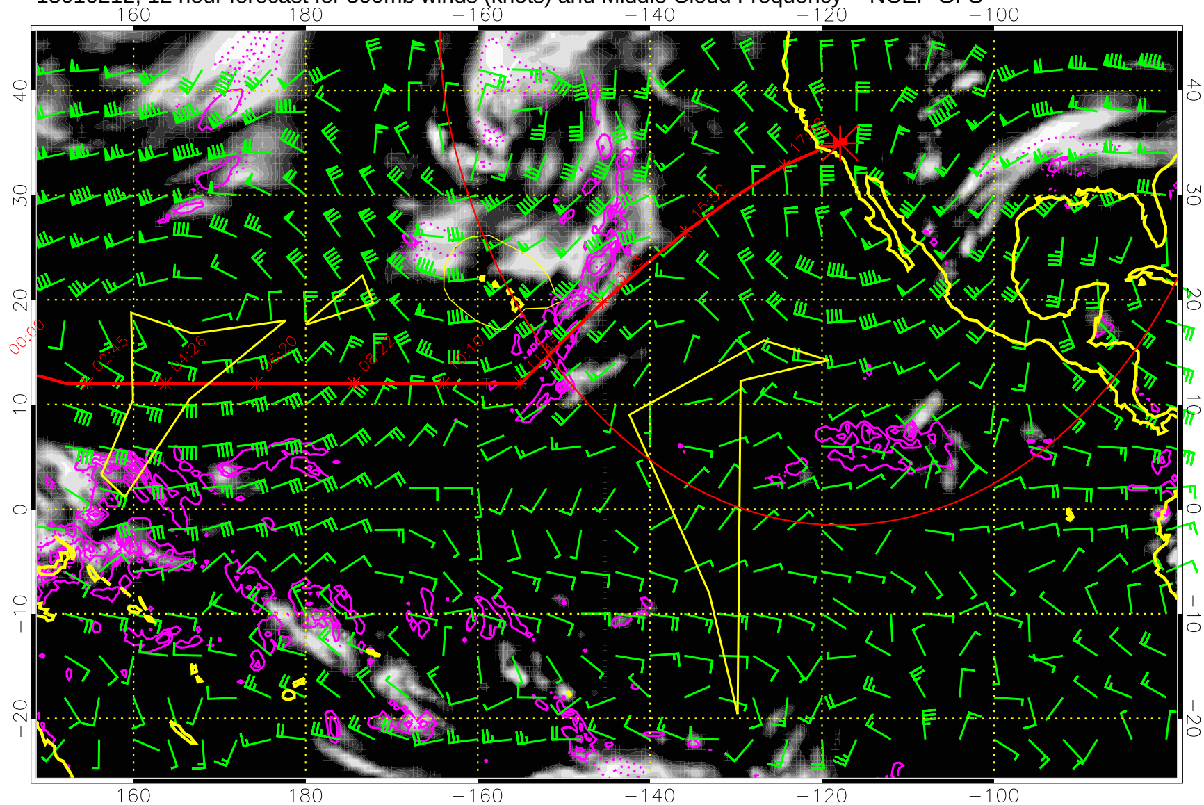
15010212, 12 hour forecast for 500mb winds (knots) and Middle Cloud Frequency -- NCEP GFS
