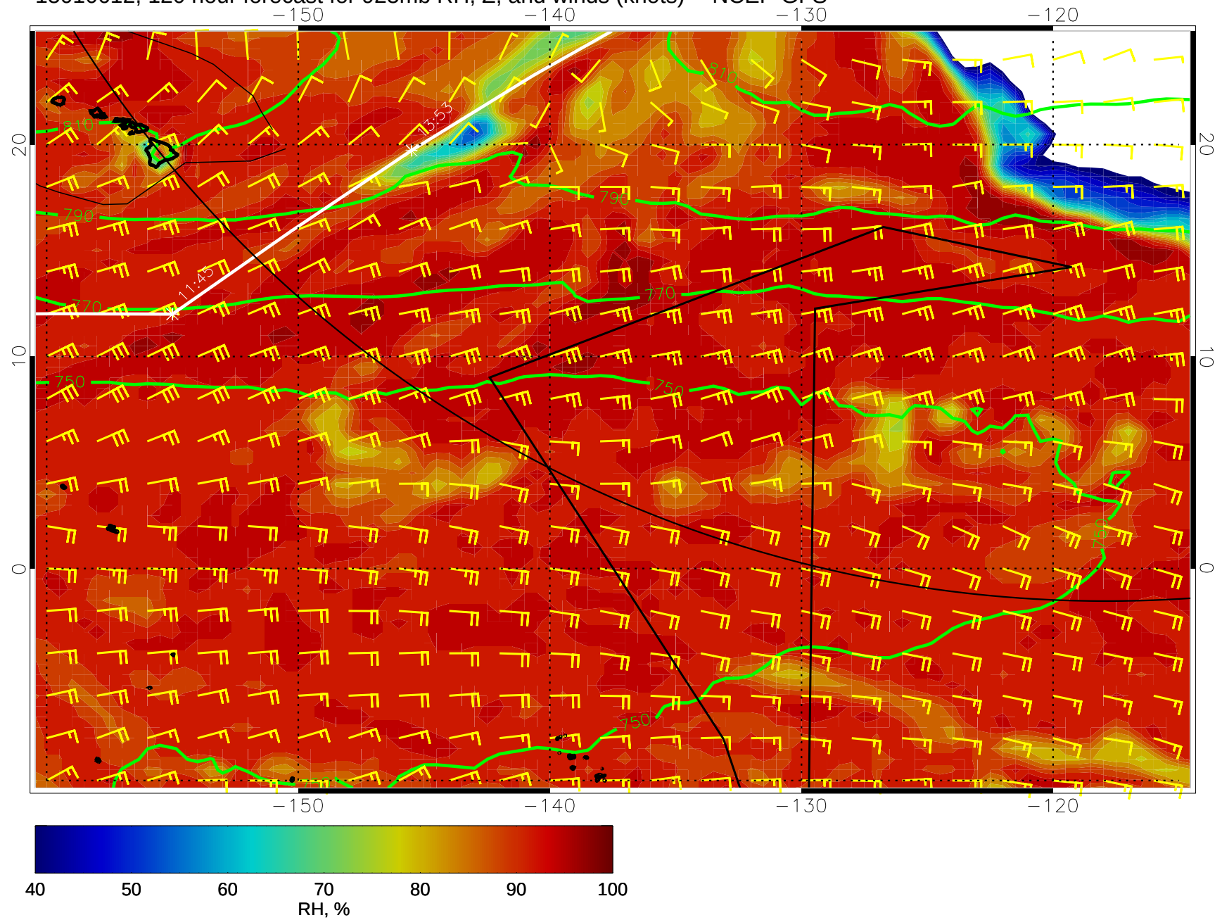
15010612, 120 hour forecast for 925mb RH, Z, and winds (knots) -- NCEP GFS
