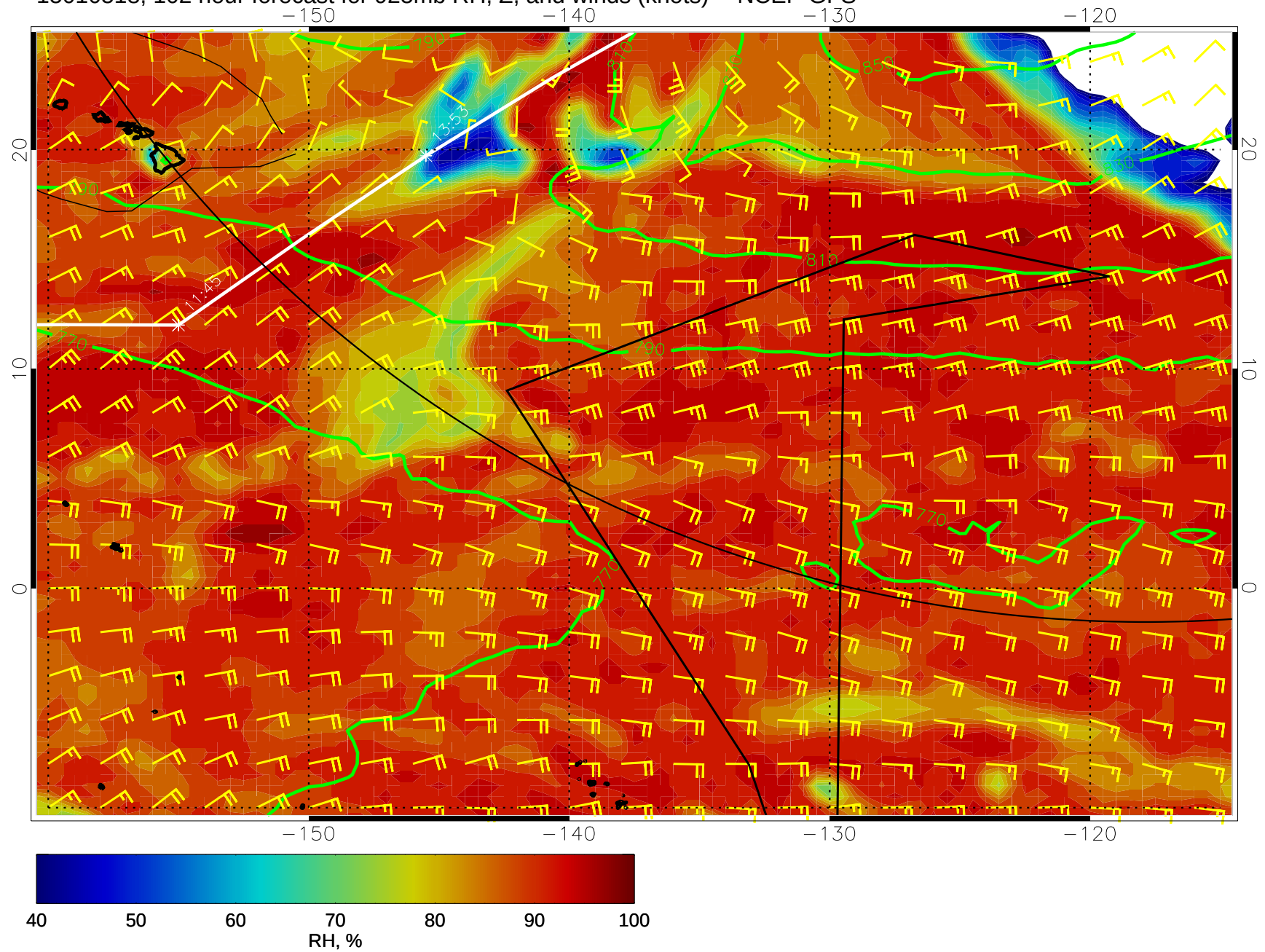
15010518, 102 hour forecast for 925mb RH, Z, and winds (knots) -- NCEP GFS
