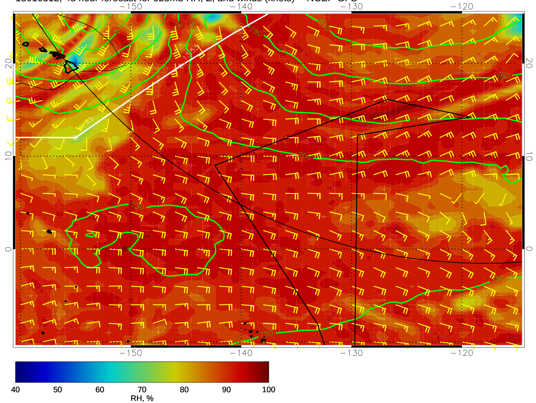
15010312, 48 hour forecast for 925mb RH, Z, and winds (knots) -- NCEP GFS
