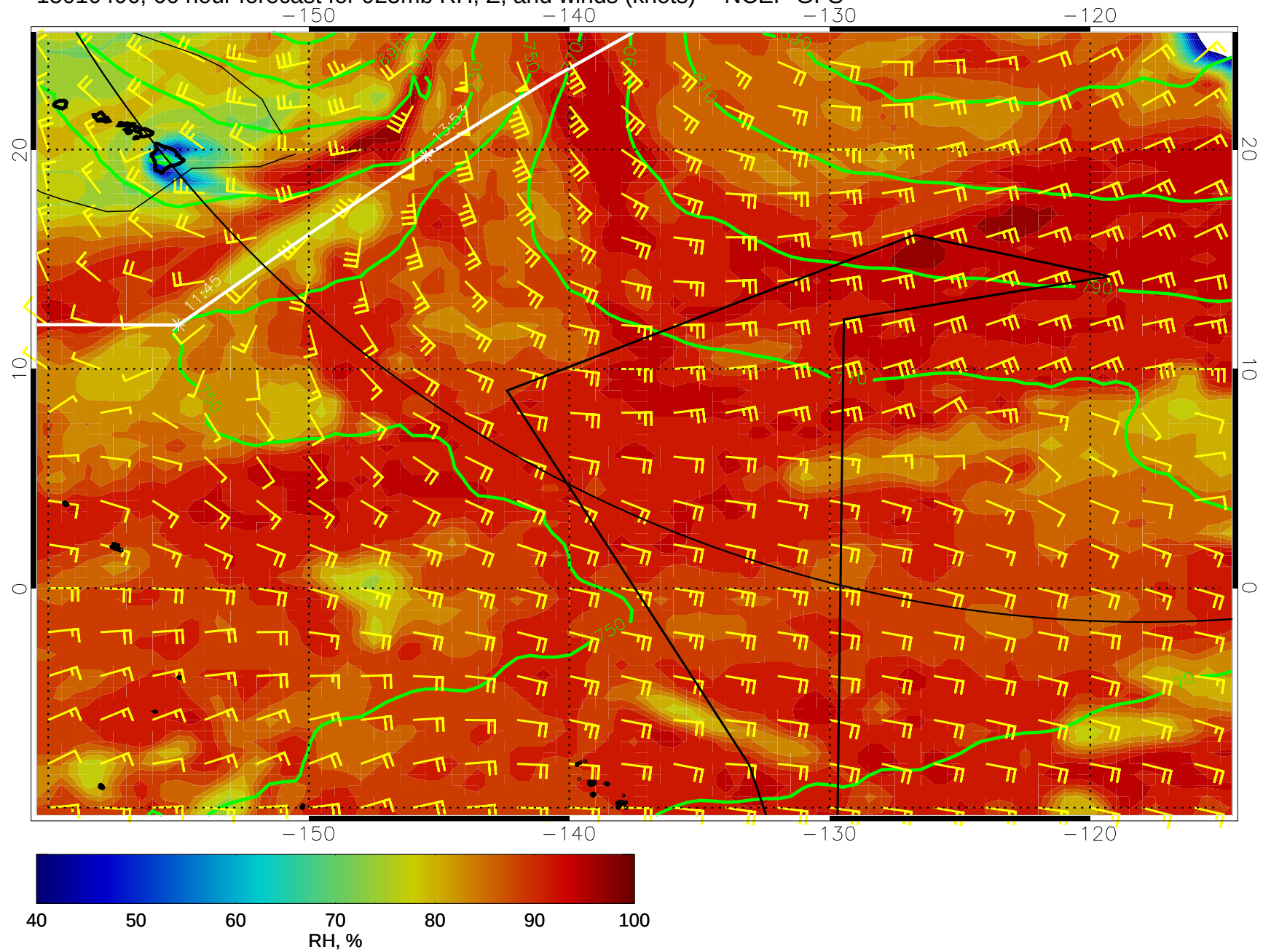
15010406, 66 hour forecast for 925mb RH, Z, and winds (knots) -- NCEP GFS
