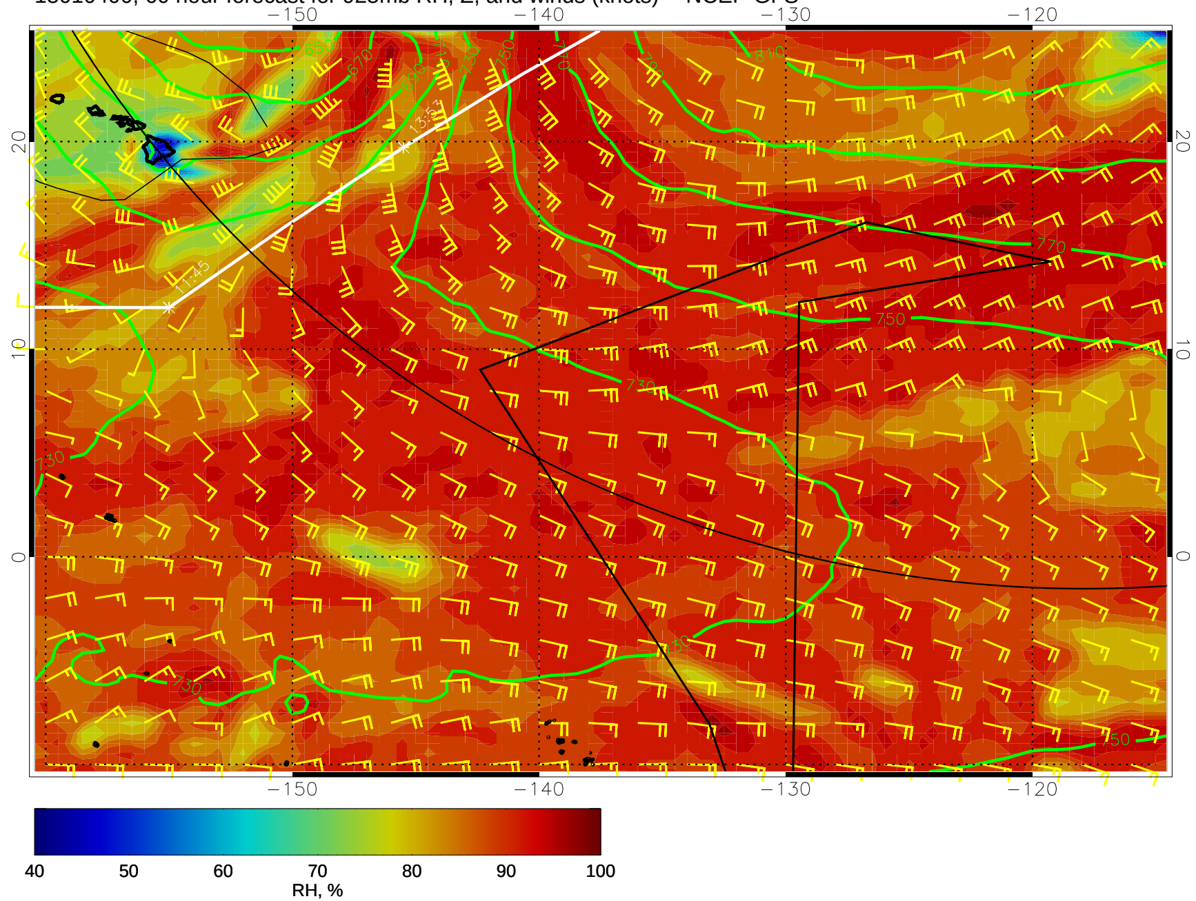
15010400, 60 hour forecast for 925mb RH, Z, and winds (knots) -- NCEP GFS
