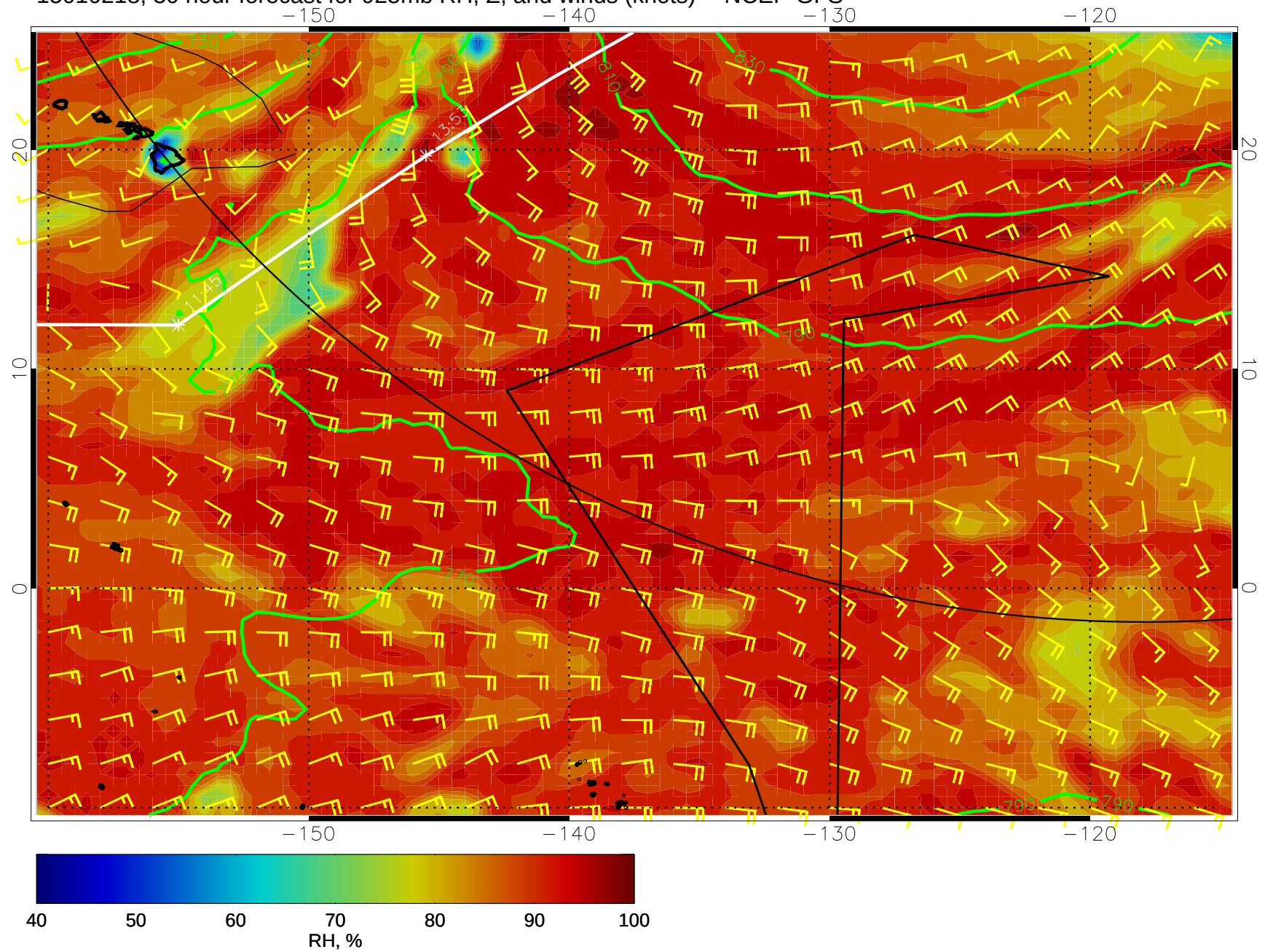
15010218, 30 hour forecast for 925mb RH, Z, and winds (knots) -- NCEP GFS
