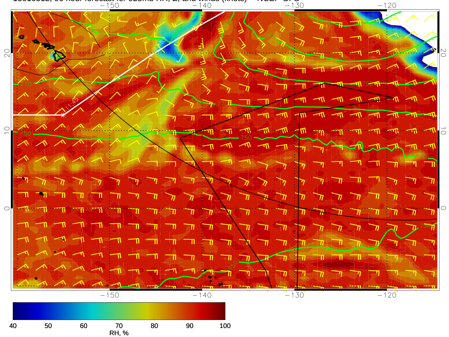
15010512, 96 hour forecast for 925mb RH, Z, and winds (knots) -- NCEP GFS
