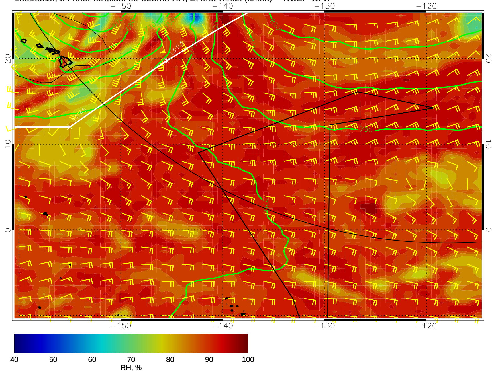
15010318, 54 hour forecast for 925mb RH, Z, and winds (knots) -- NCEP GFS
