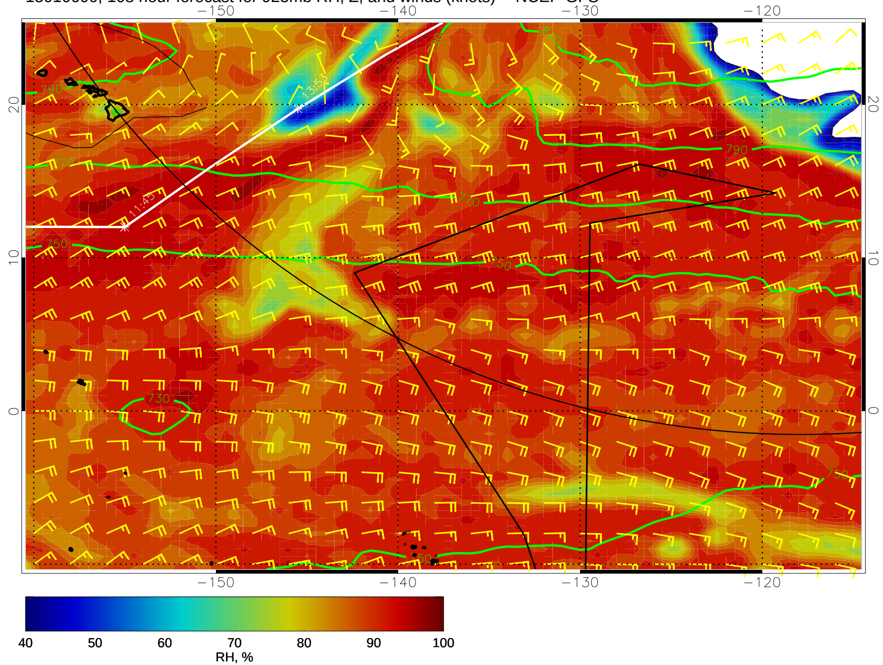
15010600, 108 hour forecast for 925mb RH, Z, and winds (knots) -- NCEP GFS
