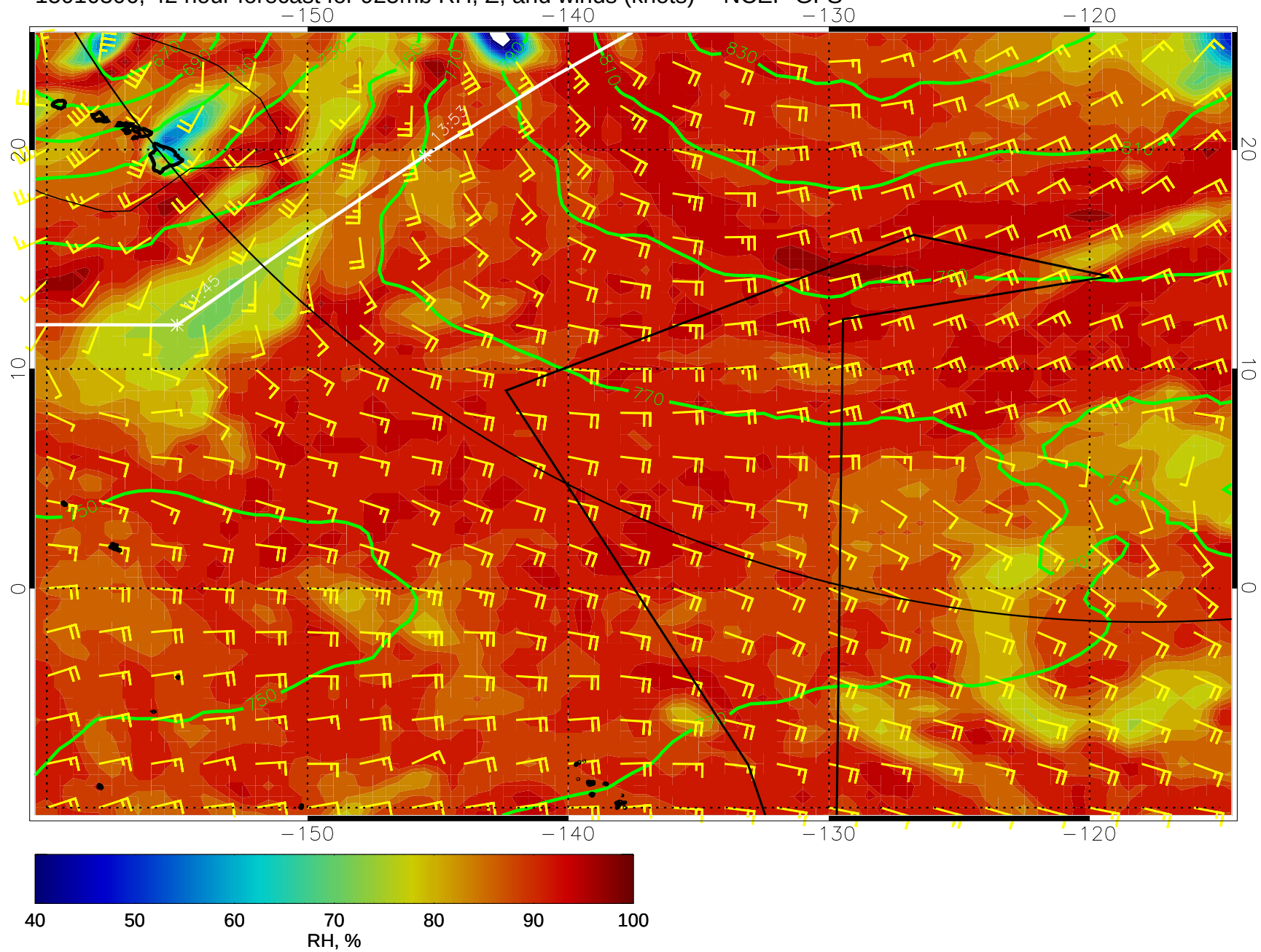
15010306, 42 hour forecast for 925mb RH, Z, and winds (knots) -- NCEP GFS
