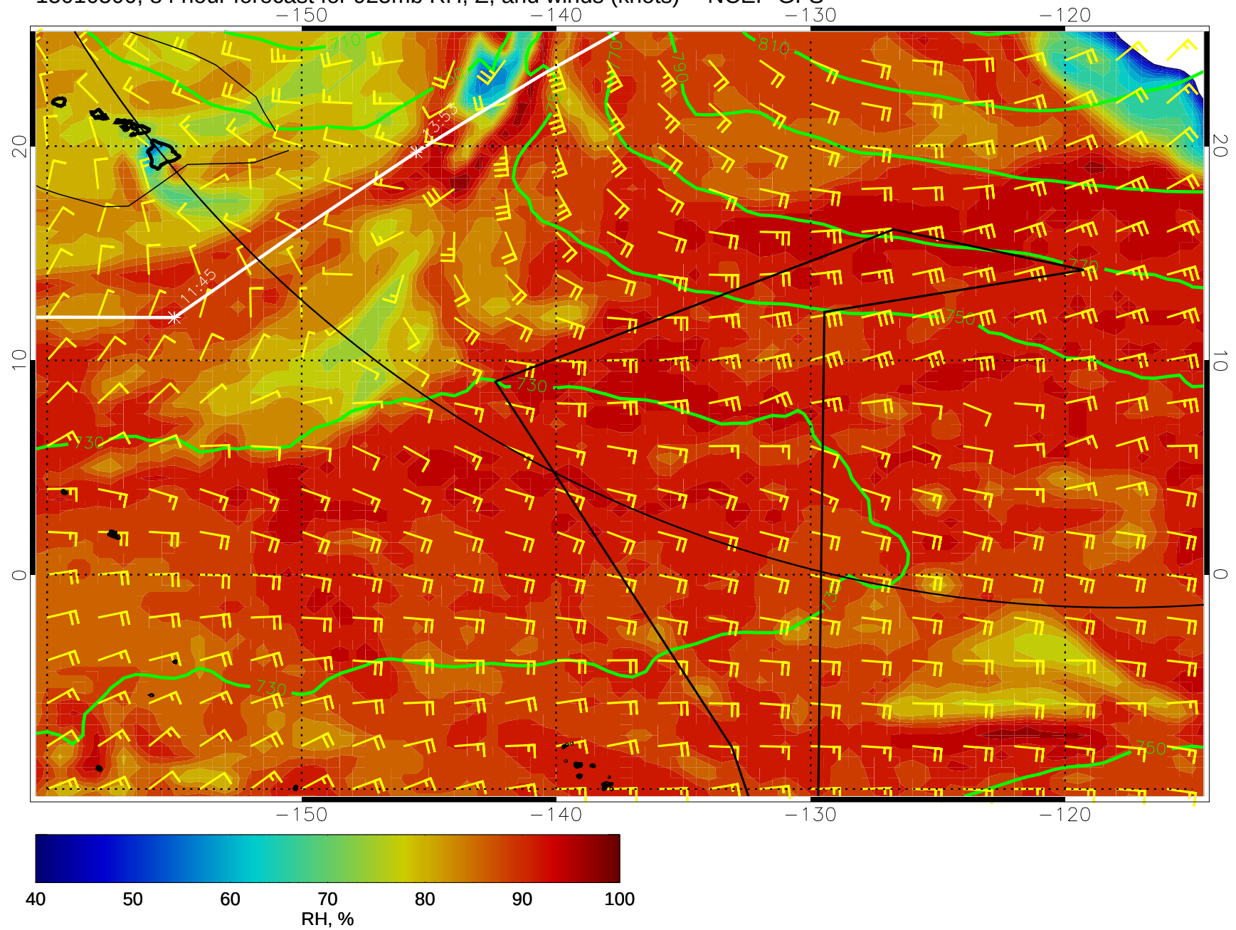
15010500, 84 hour forecast for 925mb RH, Z, and winds (knots) -- NCEP GFS
