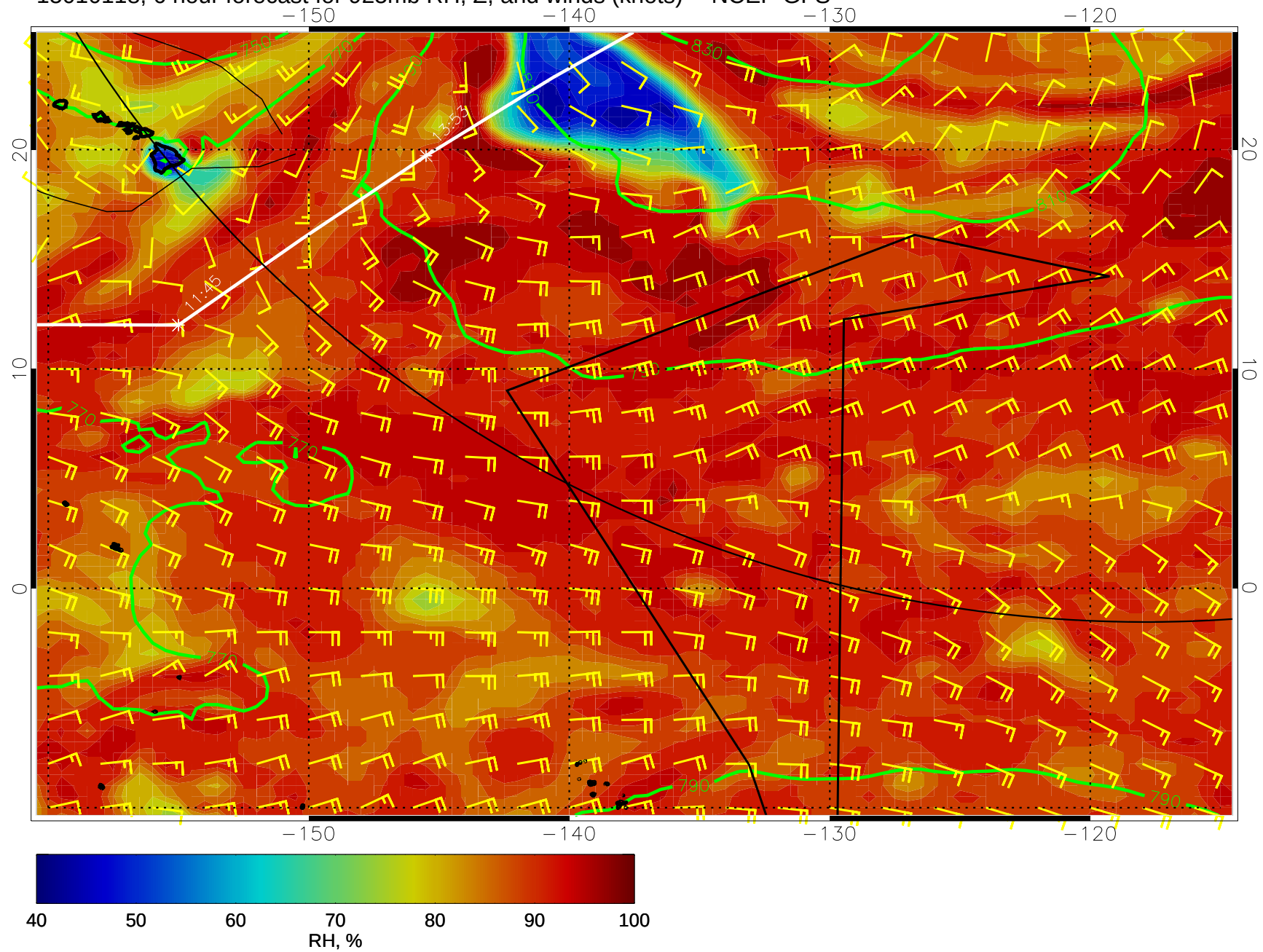
15010118, 6 hour forecast for 925mb RH, Z, and winds (knots) -- NCEP GFS
