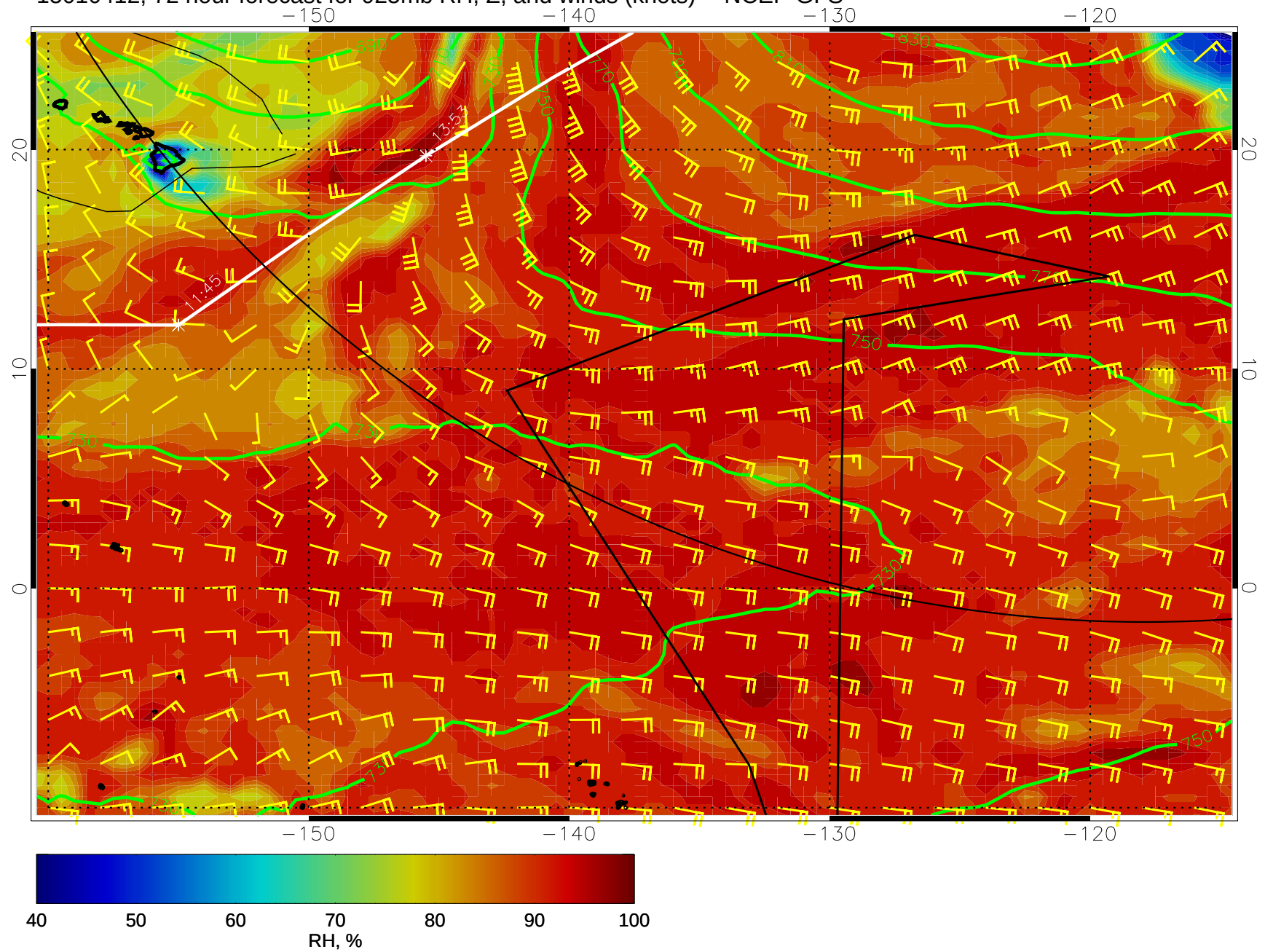
15010412, 72 hour forecast for 925mb RH, Z, and winds (knots) -- NCEP GFS
