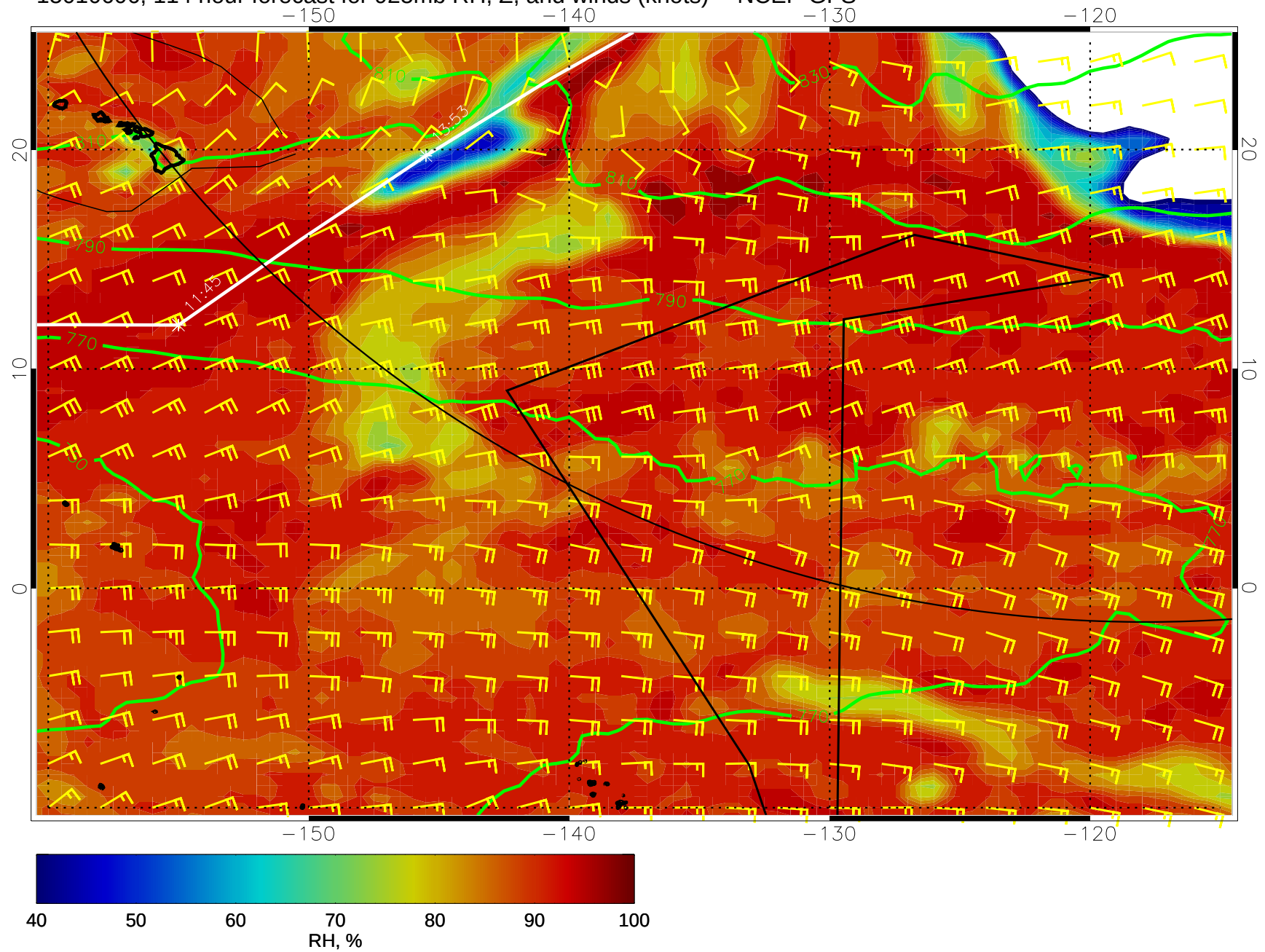
15010606, 114 hour forecast for 925mb RH, Z, and winds (knots) -- NCEP GFS
