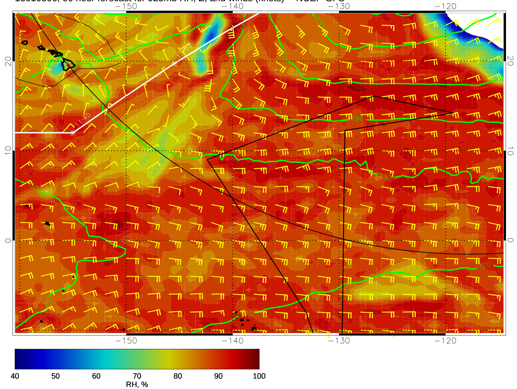
15010506, 90 hour forecast for 925mb RH, Z, and winds (knots) -- NCEP GFS
