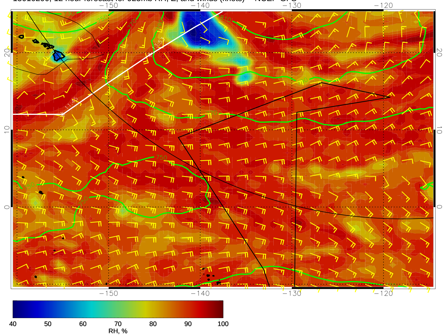
15010200, 12 hour forecast for 925mb RH, Z, and winds (knots) -- NCEP GFS
