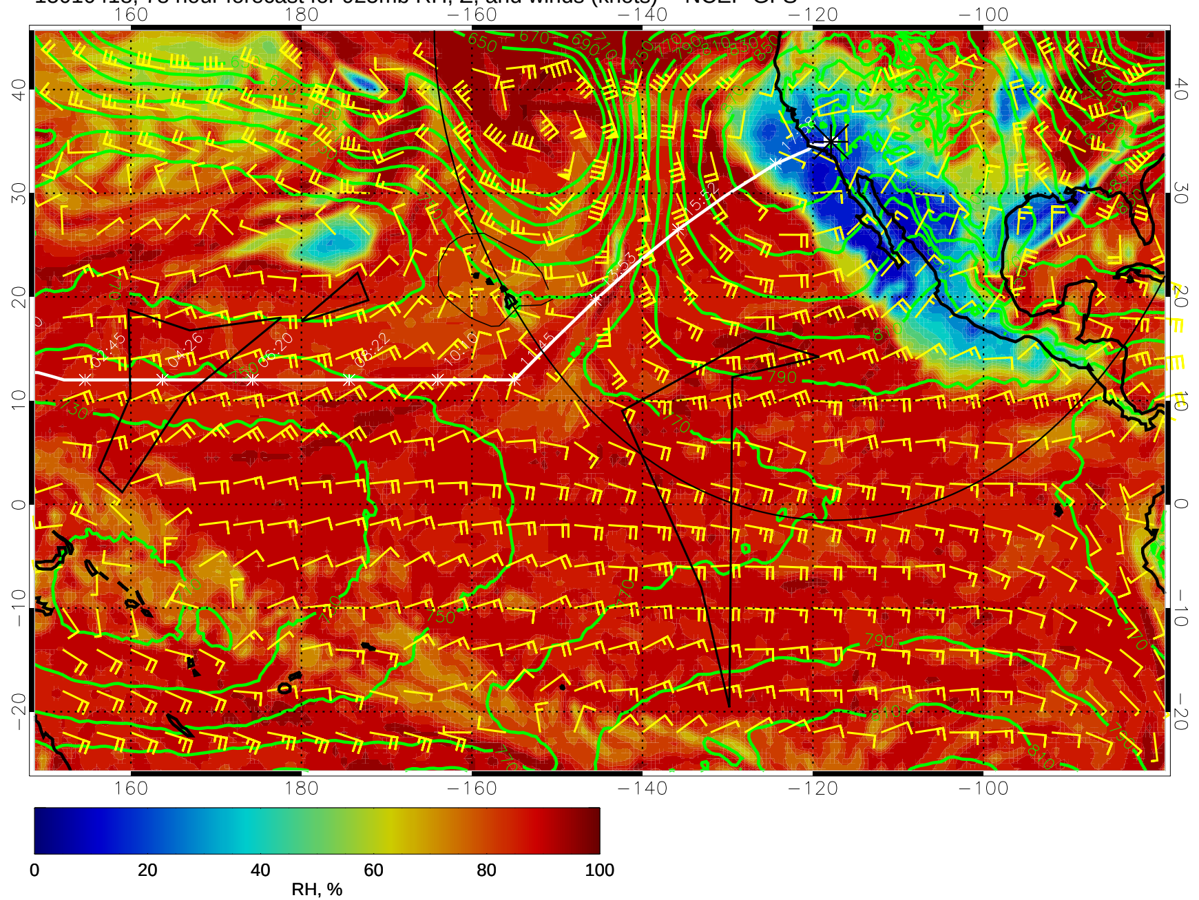
15010418, 78 hour forecast for 925mb RH, Z, and winds (knots) -- NCEP GFS
