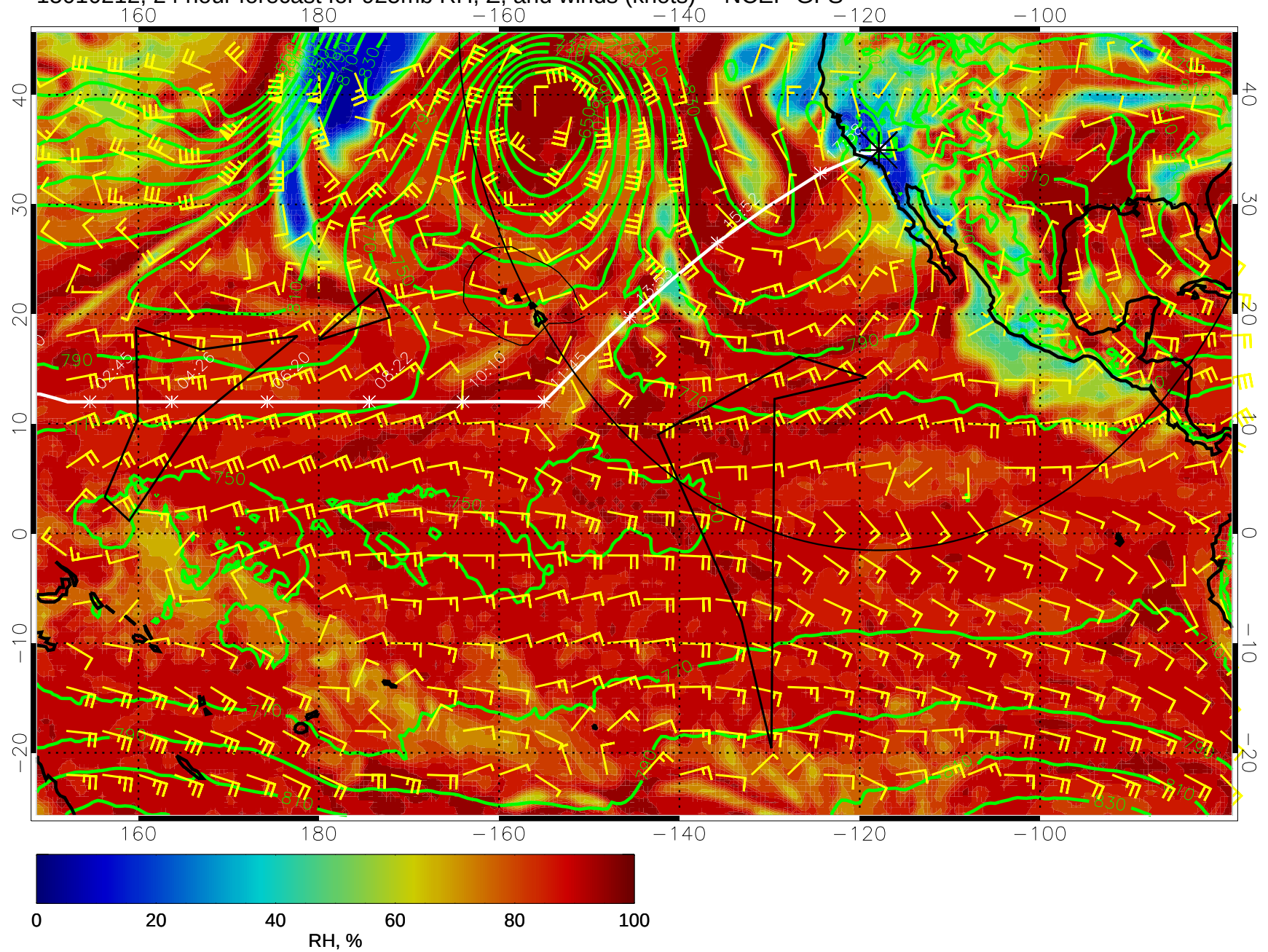
15010212, 24 hour forecast for 925mb RH, Z, and winds (knots) -- NCEP GFS
