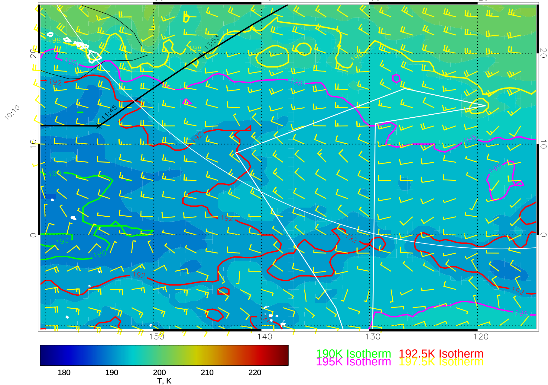
15010312, 48 hour forecast for 70mb T and winds (knots) -- NCEP GFS
