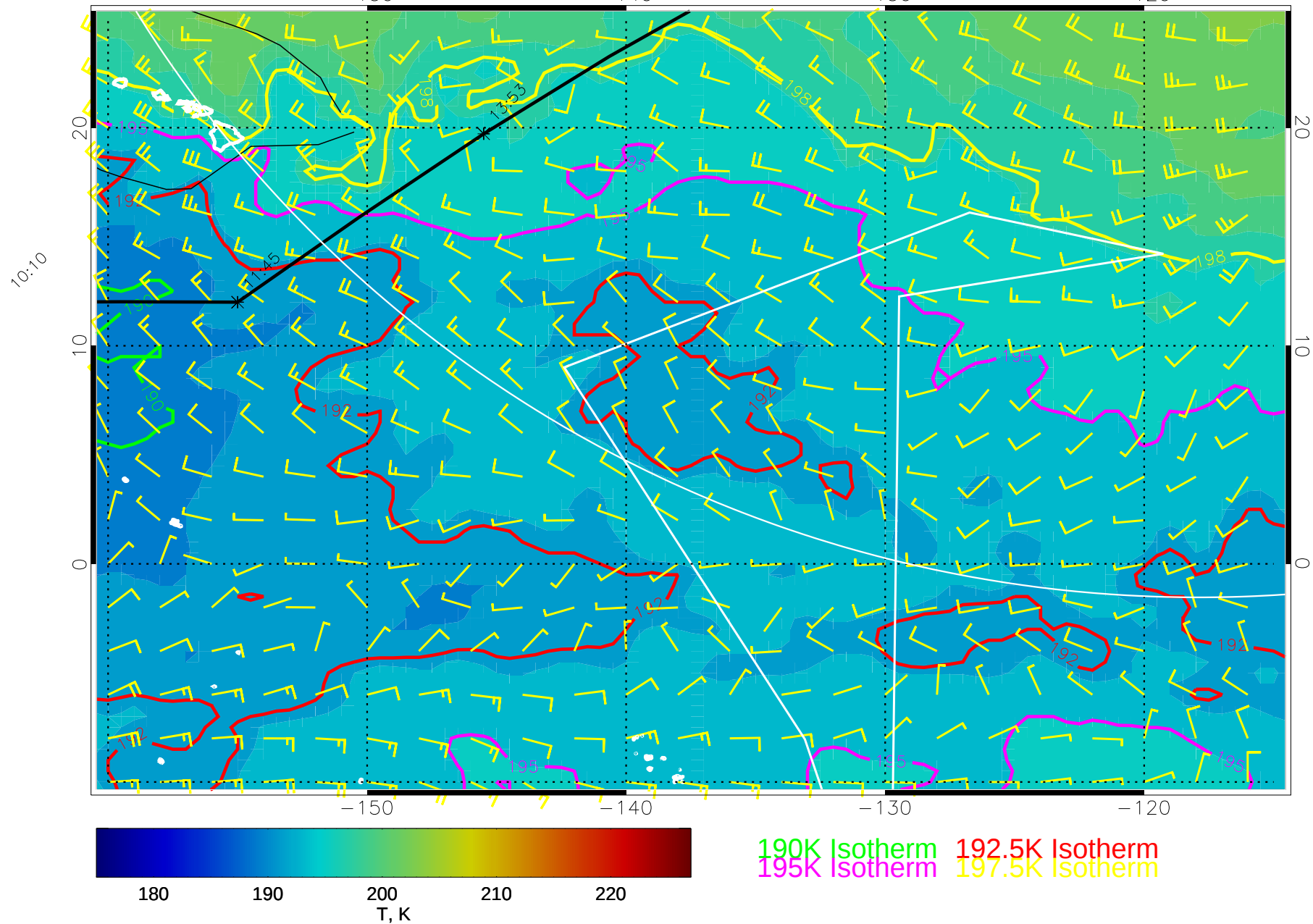
15010318, 54 hour forecast for 70mb T and winds (knots) -- NCEP GFS
