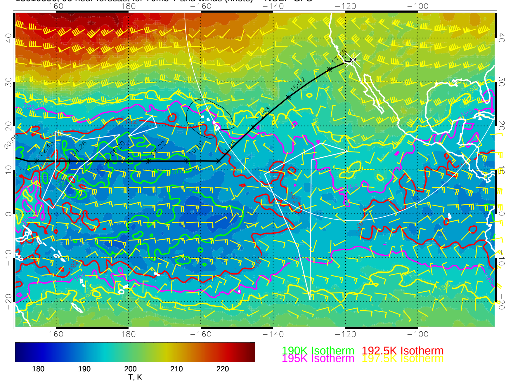
15010506, 90 hour forecast for 70mb T and winds (knots) -- NCEP GFS
