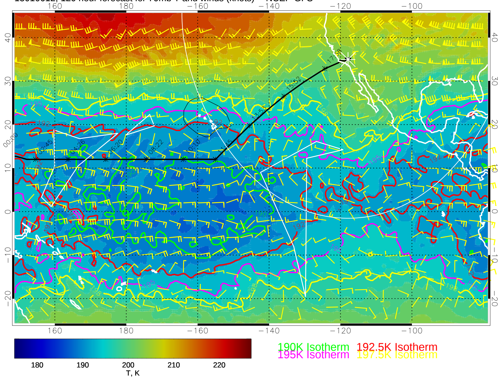
15010612, 120 hour forecast for 70mb T and winds (knots) -- NCEP GFS
