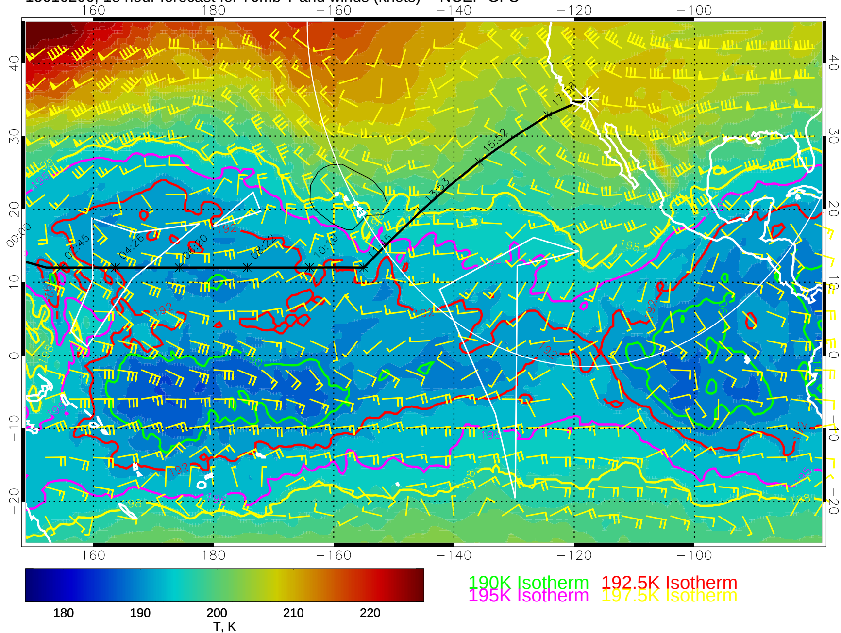
15010206, 18 hour forecast for 70mb T and winds (knots) -- NCEP GFS
