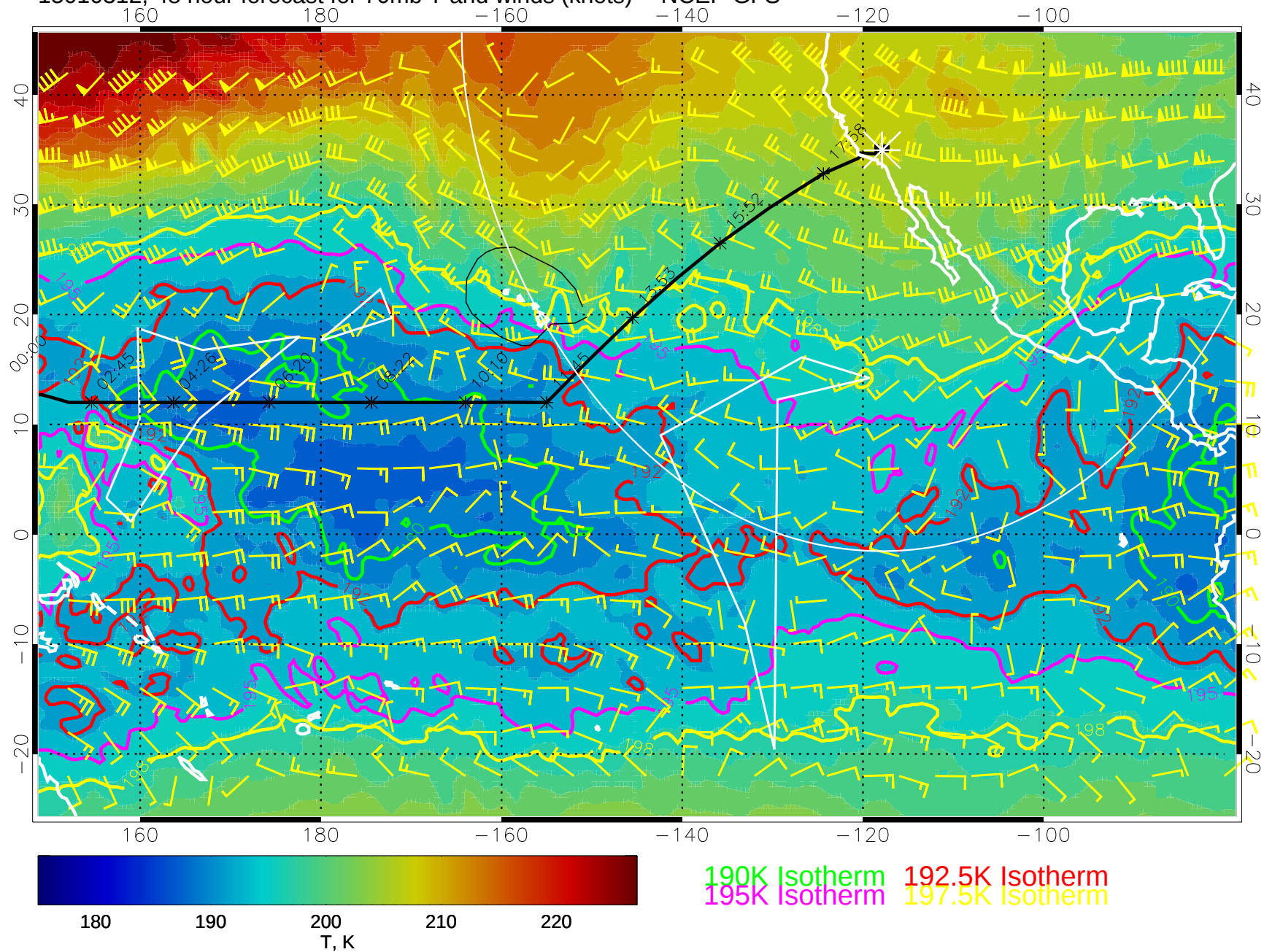
15010312, 48 hour forecast for 70mb T and winds (knots) -- NCEP GFS
