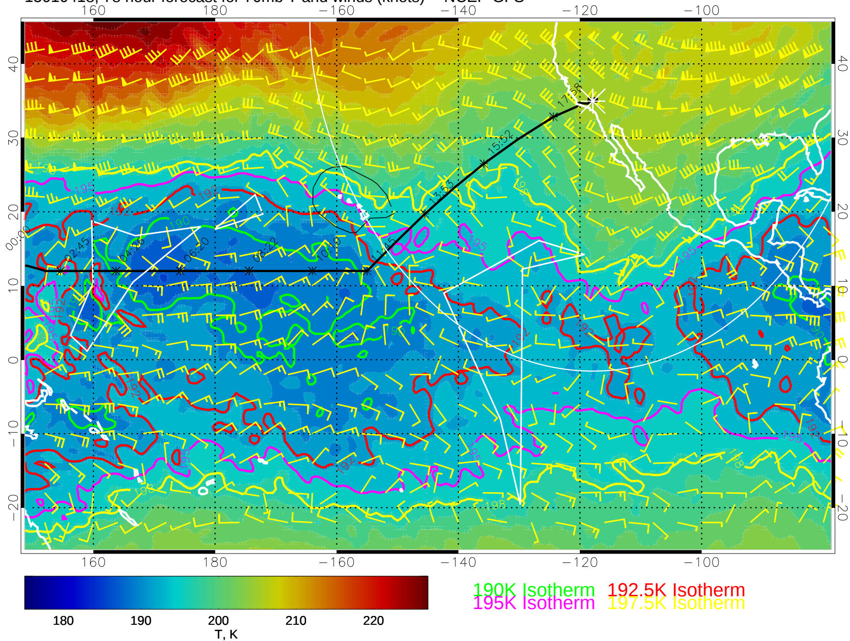
15010418, 78 hour forecast for 70mb T and winds (knots) -- NCEP GFS
