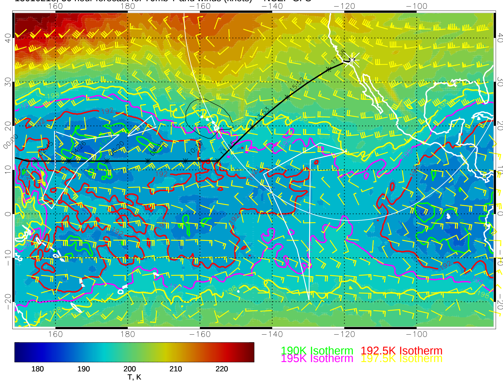
15010218, 30 hour forecast for 70mb T and winds (knots) -- NCEP GFS
