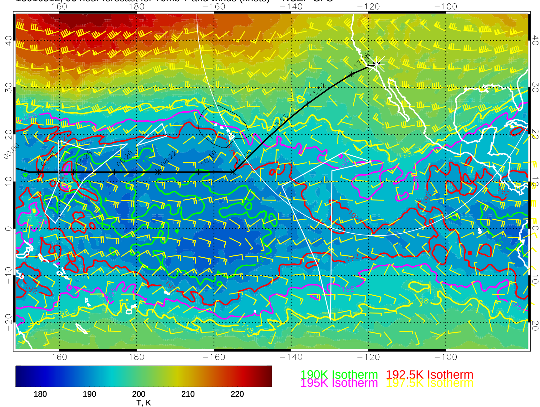
15010512, 96 hour forecast for 70mb T and winds (knots) -- NCEP GFS
