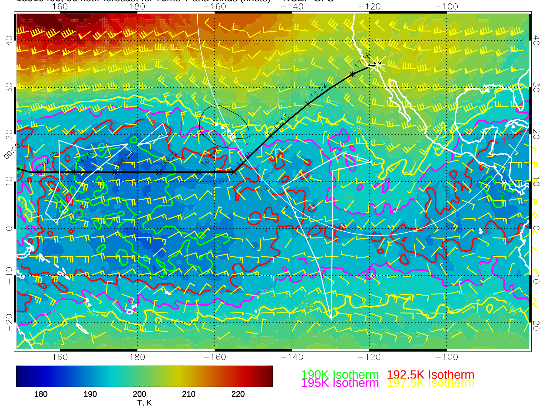
15010406, 66 hour forecast for 70mb T and winds (knots) -- NCEP GFS
