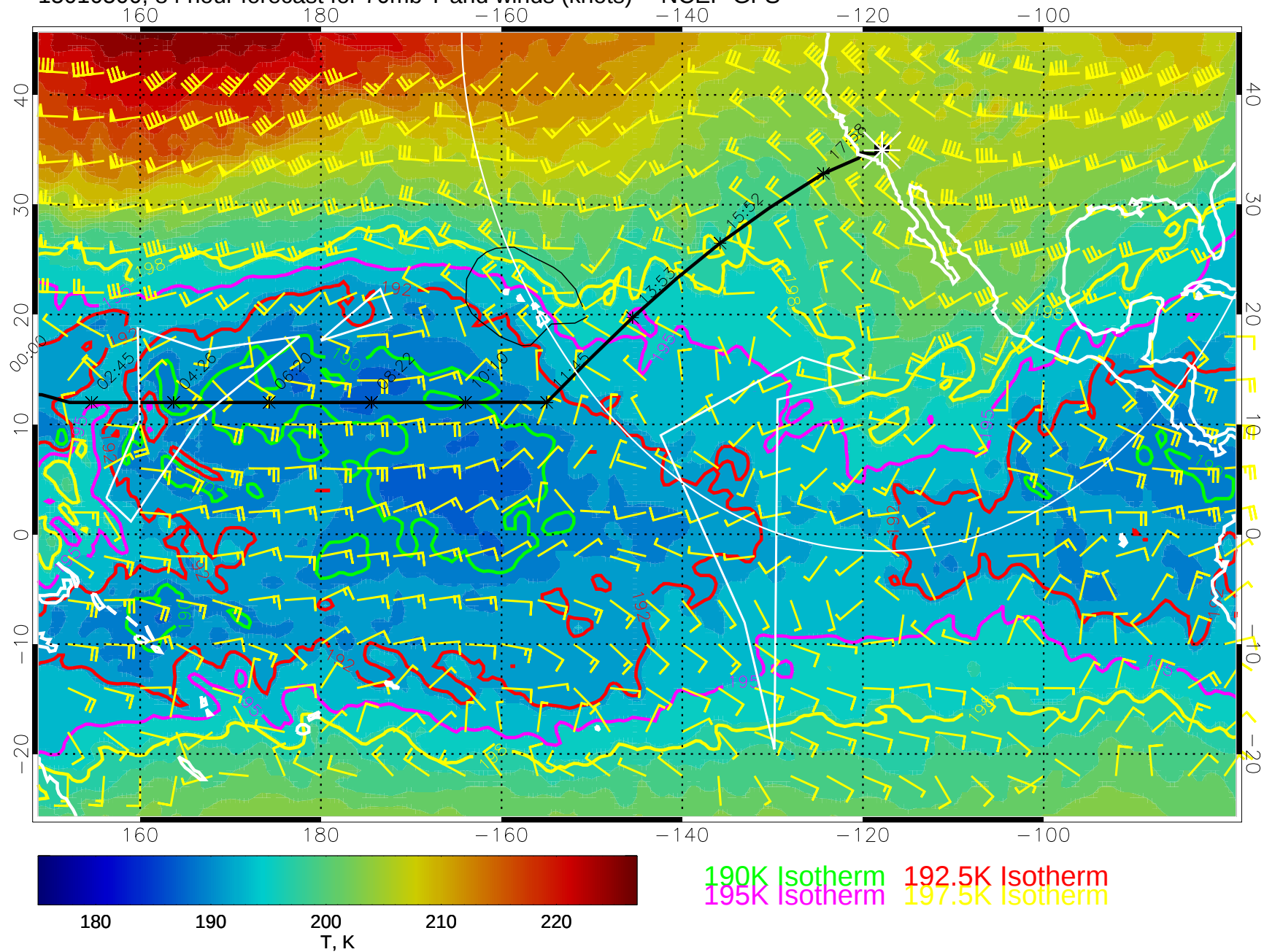
15010500, 84 hour forecast for 70mb T and winds (knots) -- NCEP GFS
