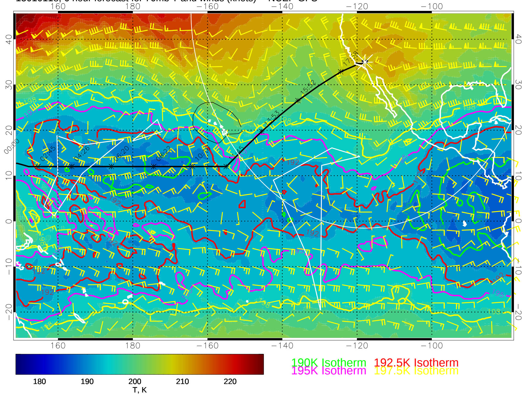
15010118, 6 hour forecast for 70mb T and winds (knots) -- NCEP GFS
