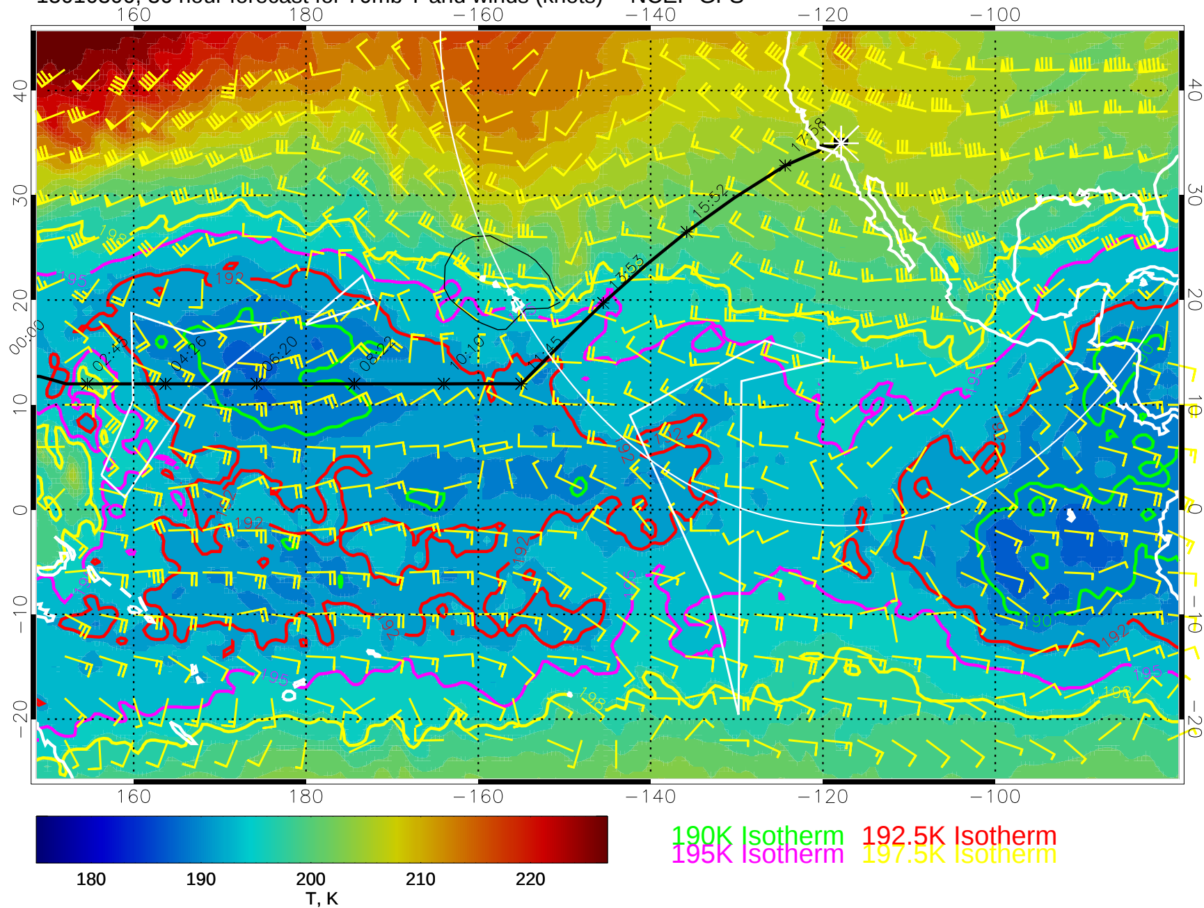
15010300, 36 hour forecast for 70mb T and winds (knots) -- NCEP GFS
