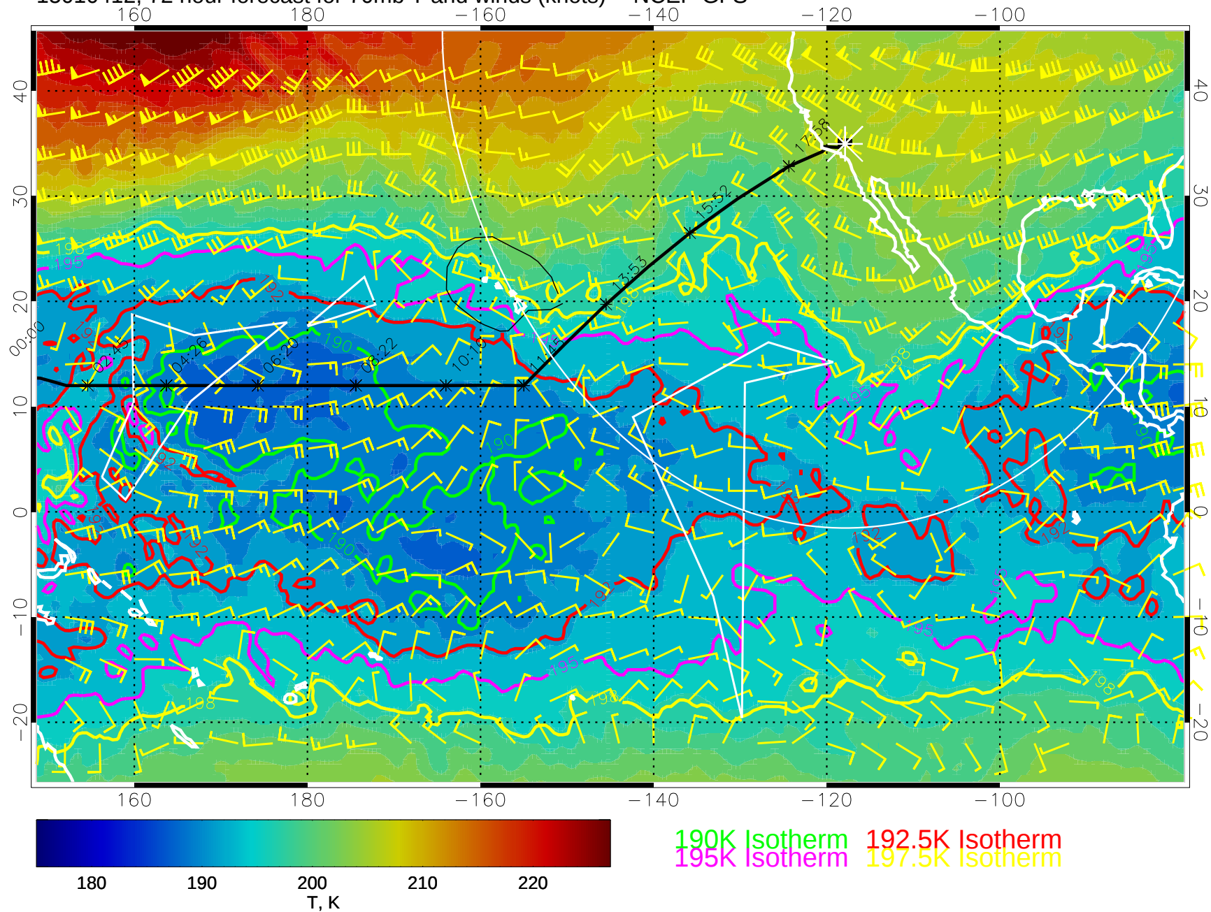
15010412, 72 hour forecast for 70mb T and winds (knots) -- NCEP GFS
