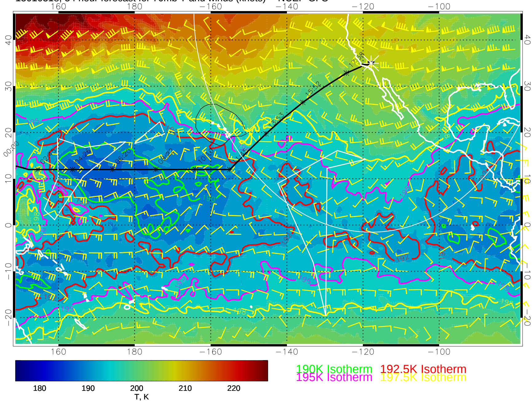
15010318, 54 hour forecast for 70mb T and winds (knots) -- NCEP GFS
