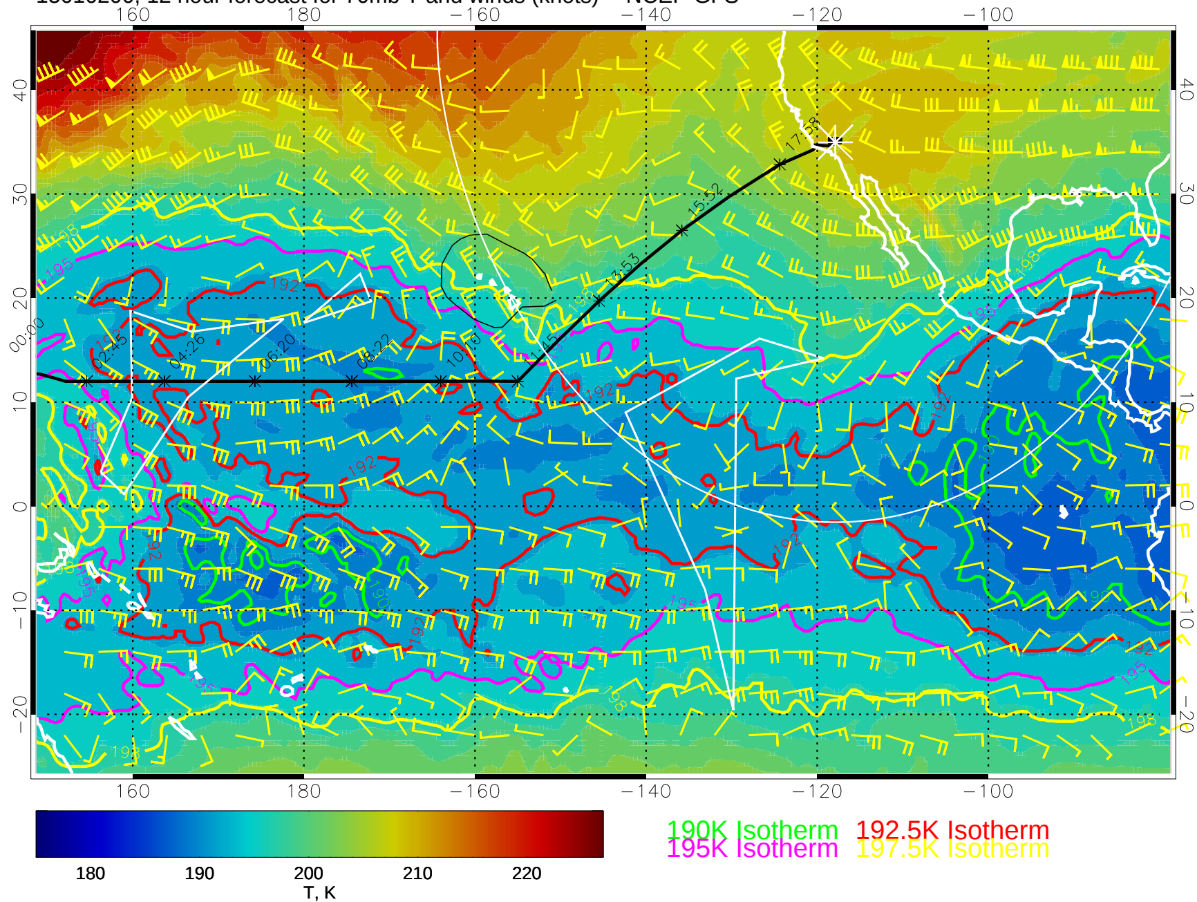
15010200, 12 hour forecast for 70mb T and winds (knots) -- NCEP GFS
