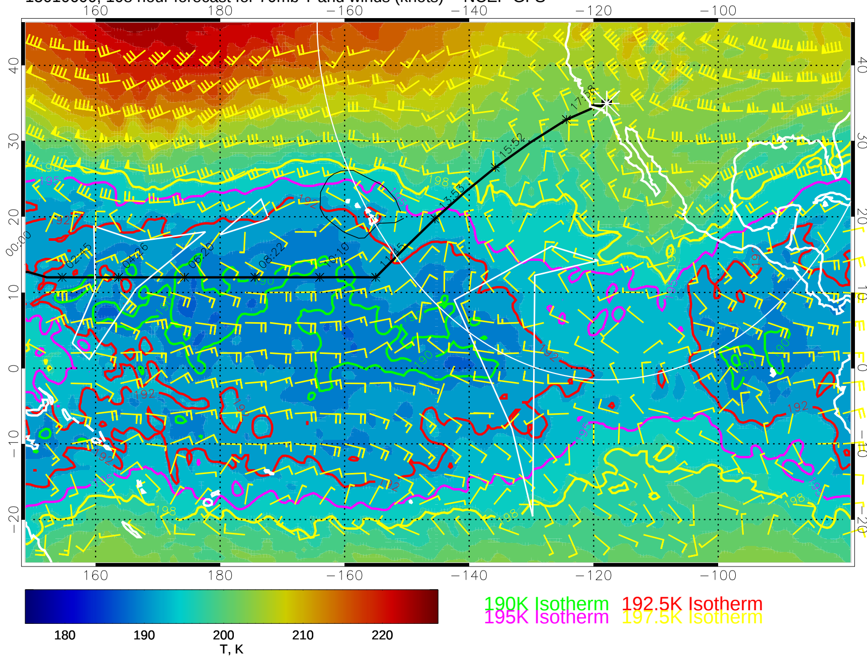
15010600, 108 hour forecast for 70mb T and winds (knots) -- NCEP GFS
