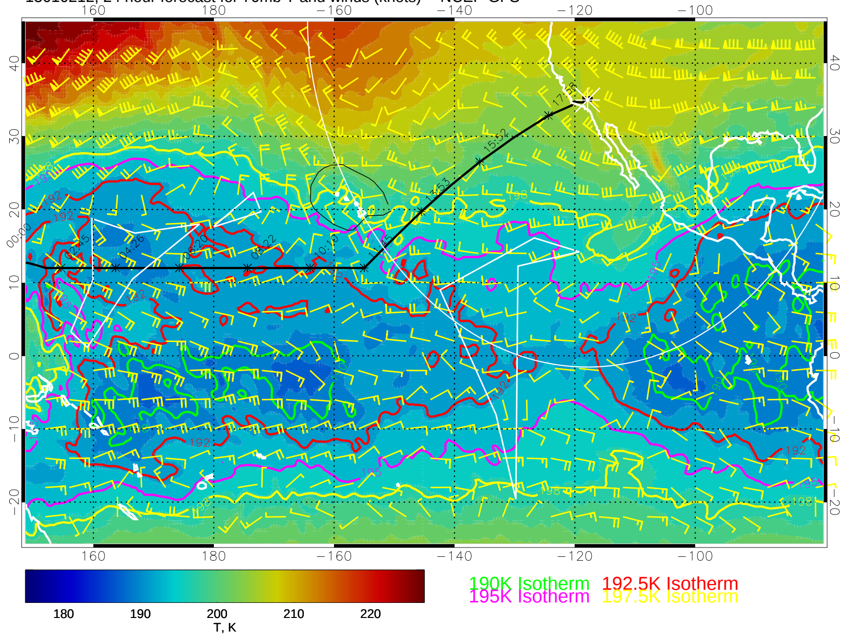
15010212, 24 hour forecast for 70mb T and winds (knots) -- NCEP GFS
