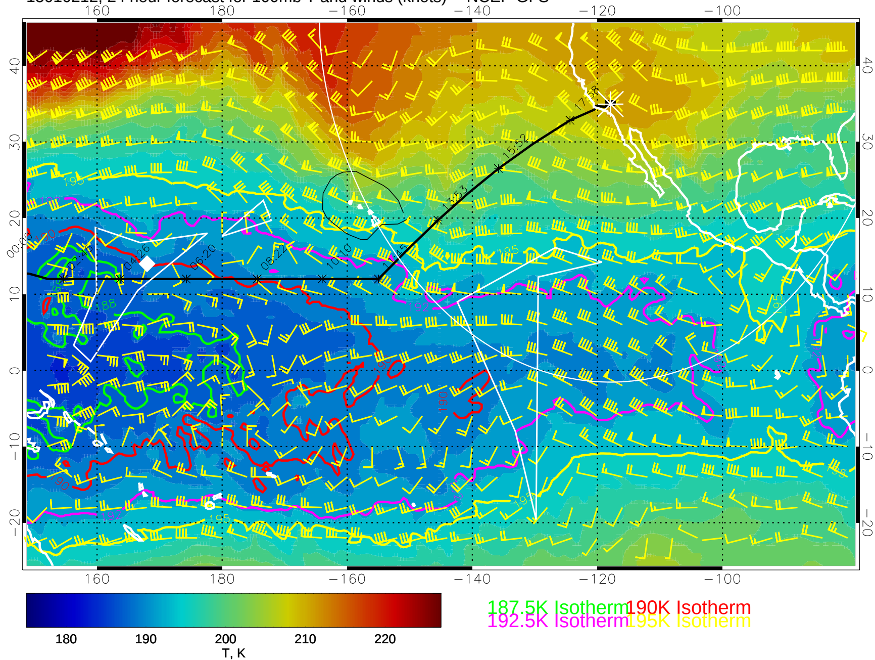
15010212, 24 hour forecast for 100mb T and winds (knots) -- NCEP GFS
