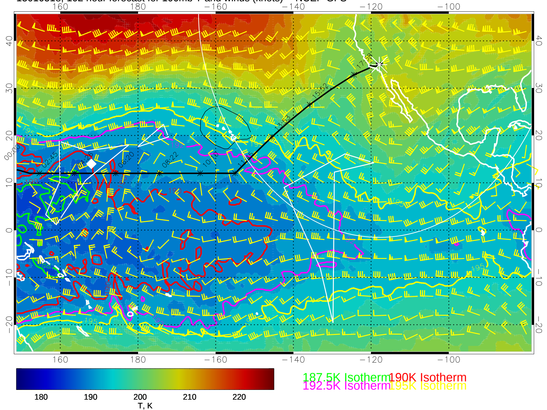
15010518, 102 hour forecast for 100mb T and winds (knots) -- NCEP GFS
