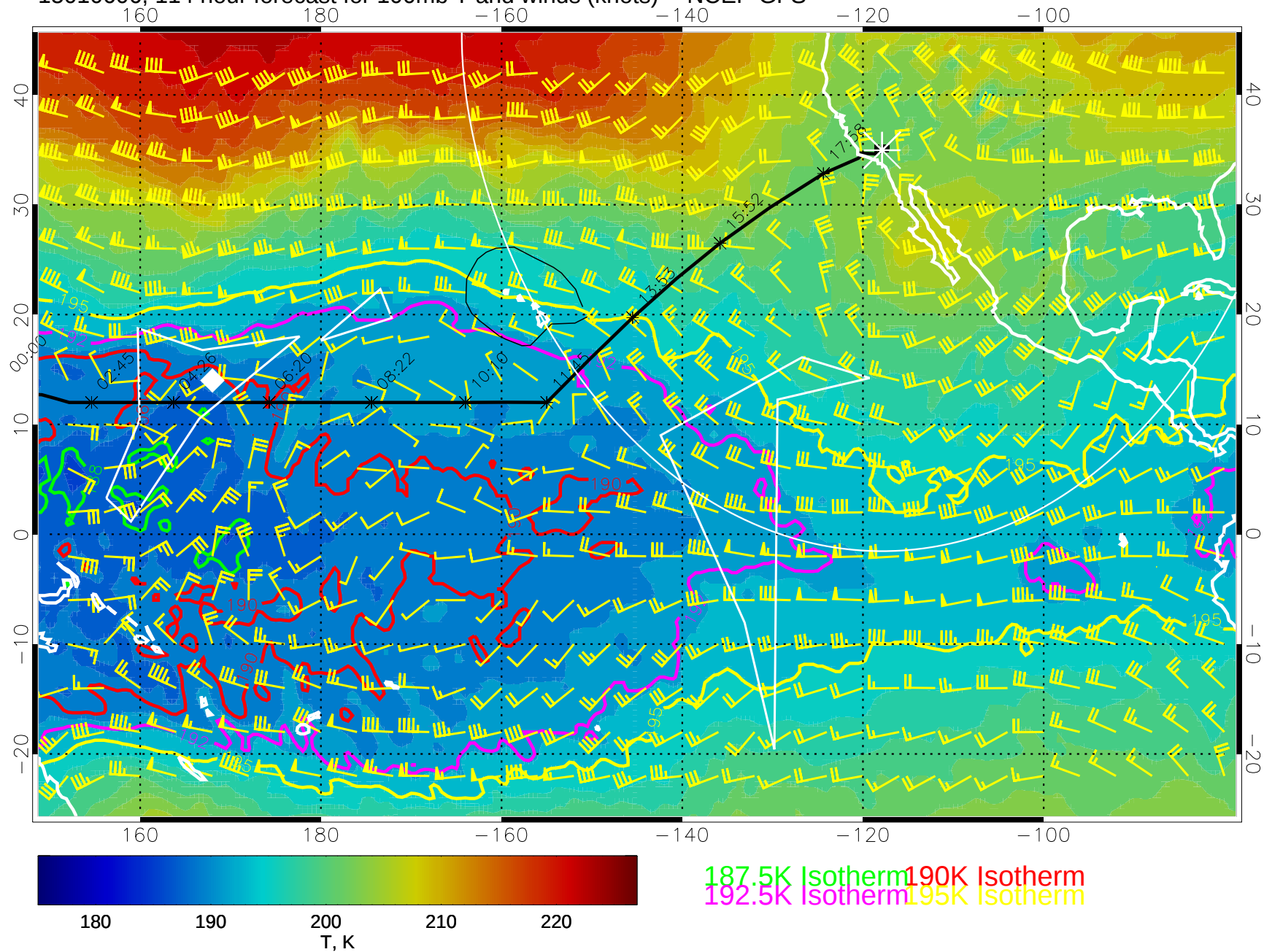
15010606, 114 hour forecast for 100mb T and winds (knots) -- NCEP GFS
