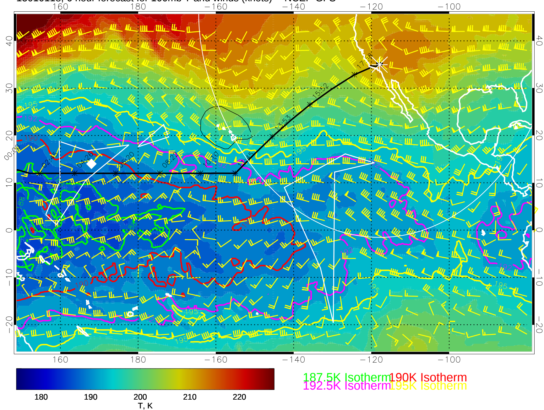
15010118, 6 hour forecast for 100mb T and winds (knots) -- NCEP GFS
