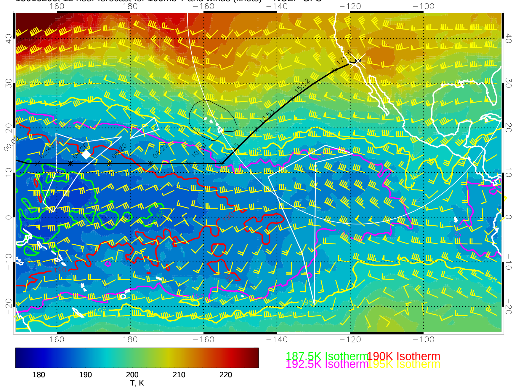
15010200, 12 hour forecast for 100mb T and winds (knots) -- NCEP GFS
