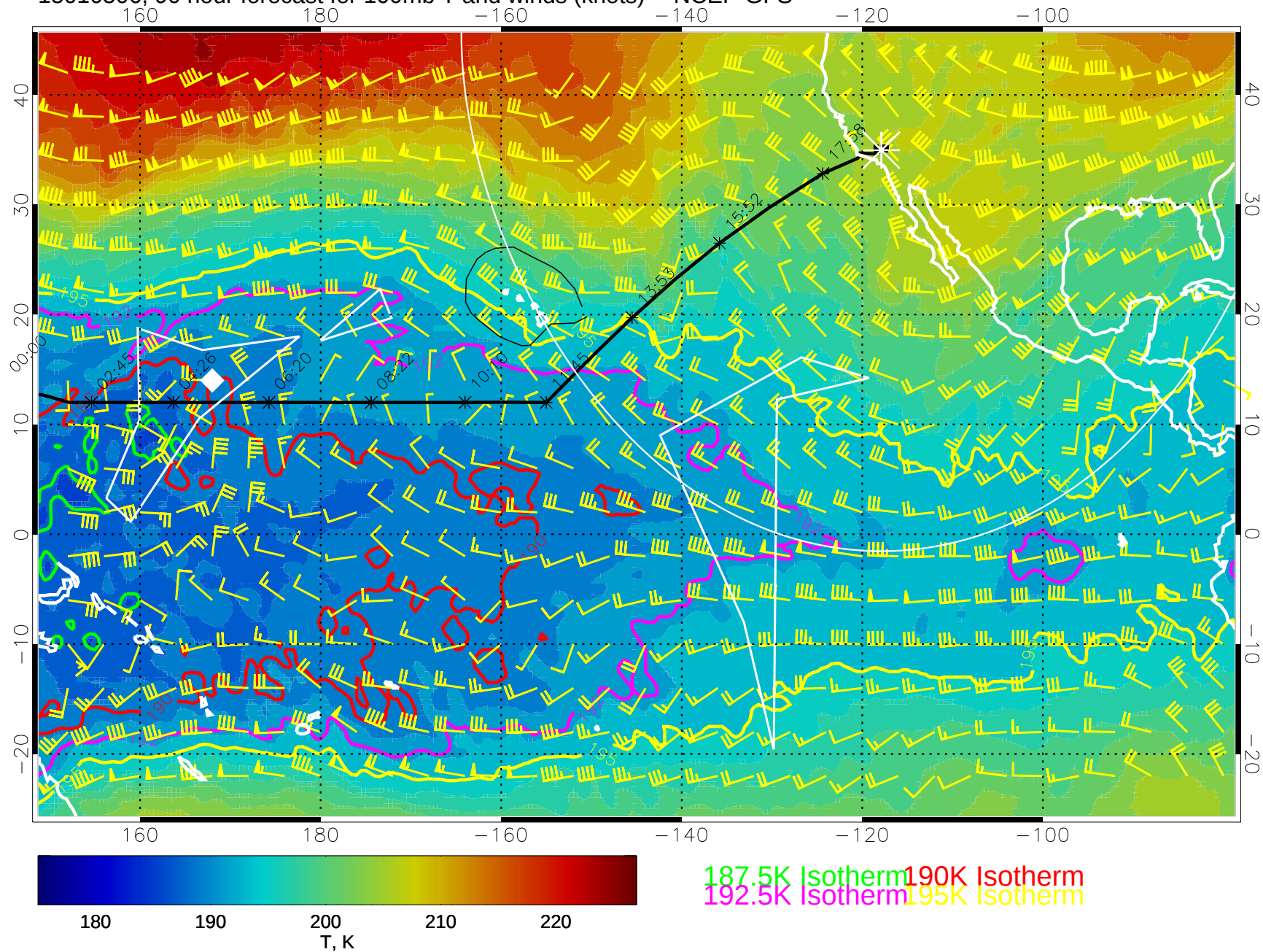
15010506, 90 hour forecast for 100mb T and winds (knots) -- NCEP GFS
