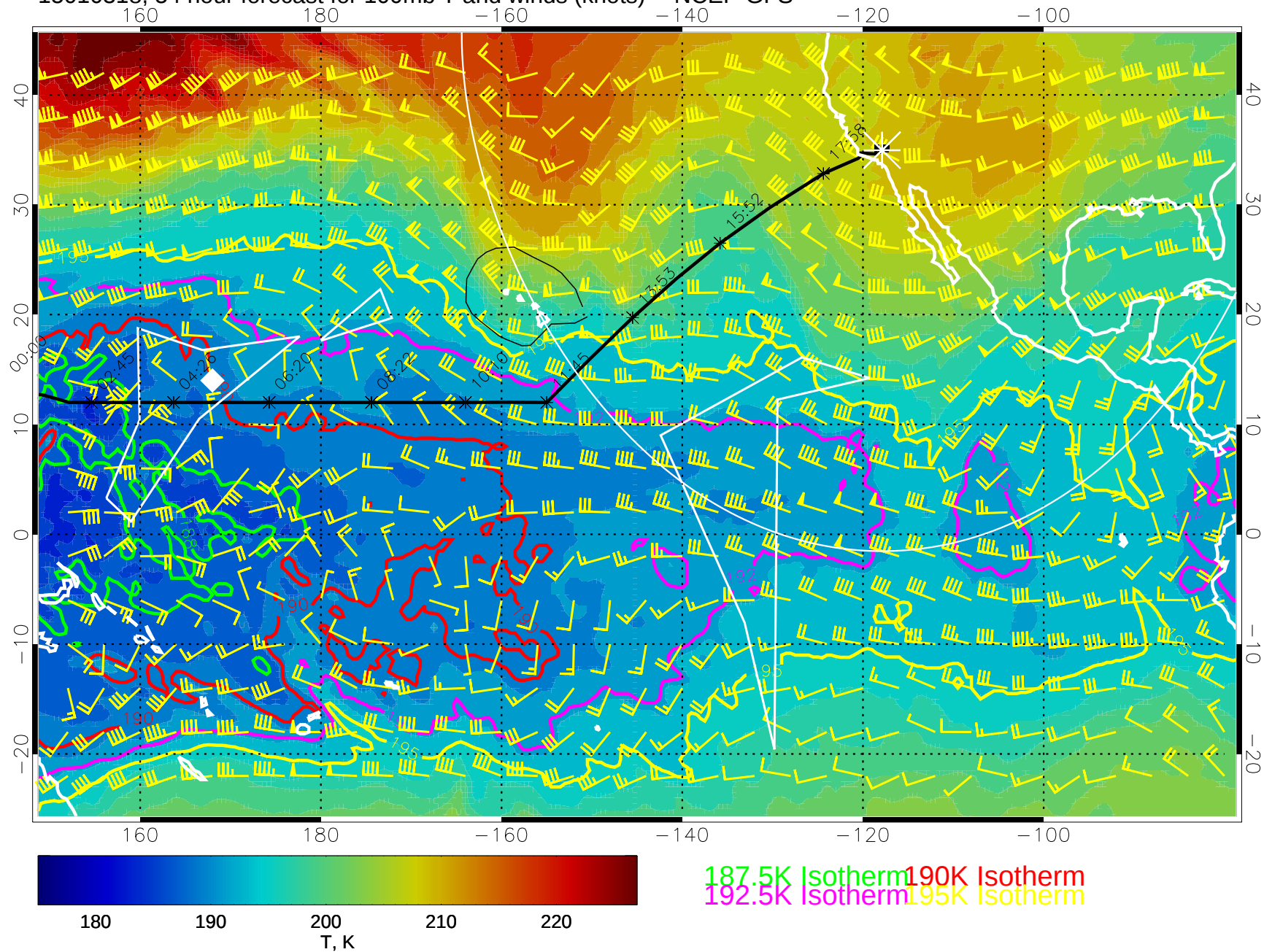
15010318, 54 hour forecast for 100mb T and winds (knots) -- NCEP GFS
