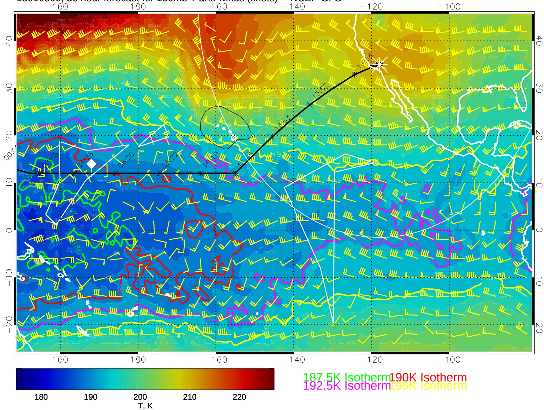
15010300, 36 hour forecast for 100mb T and winds (knots) -- NCEP GFS
