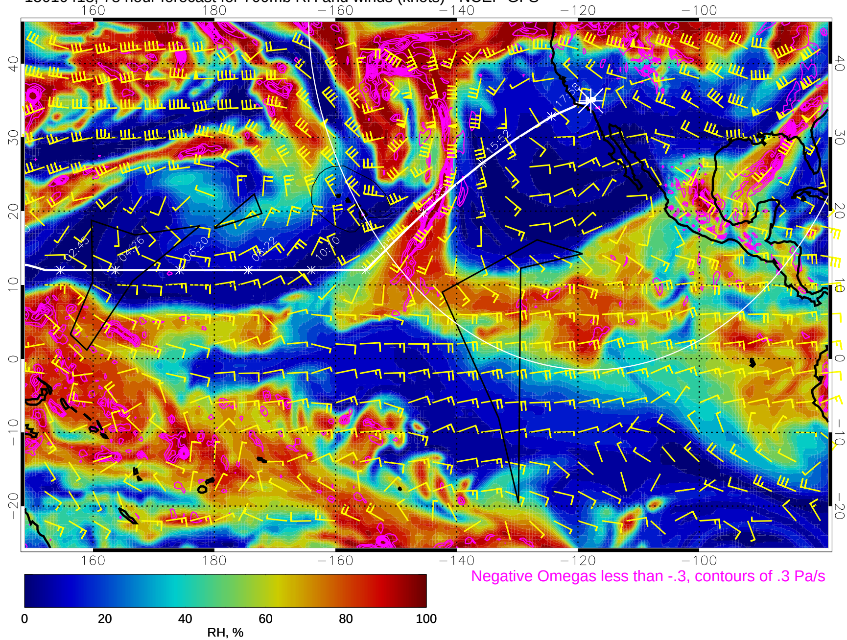
15010418, 78 hour forecast for 700mb RH and winds (knots) - NCEP GFS
