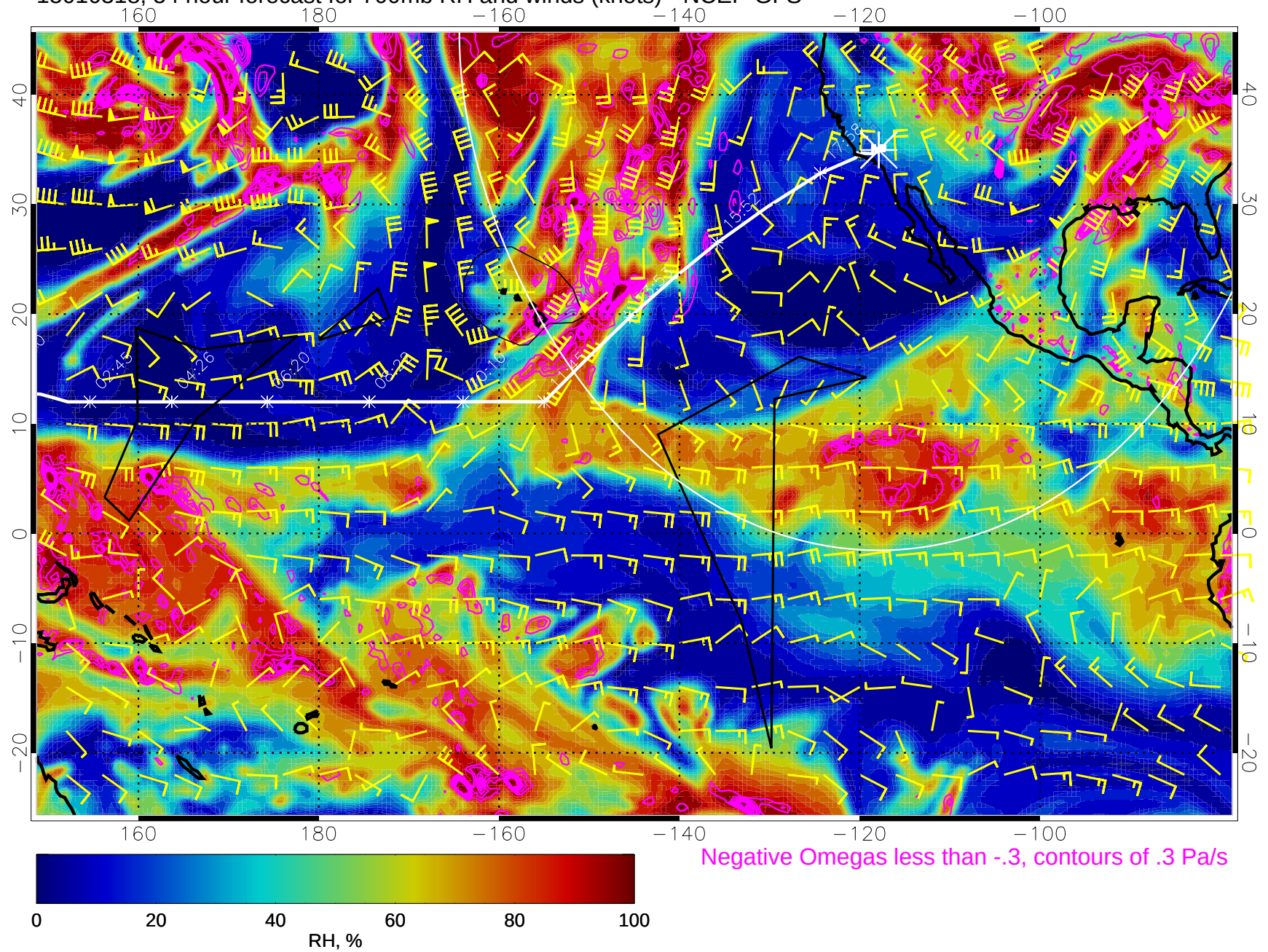
15010318, 54 hour forecast for 700mb RH and winds (knots) - NCEP GFS
