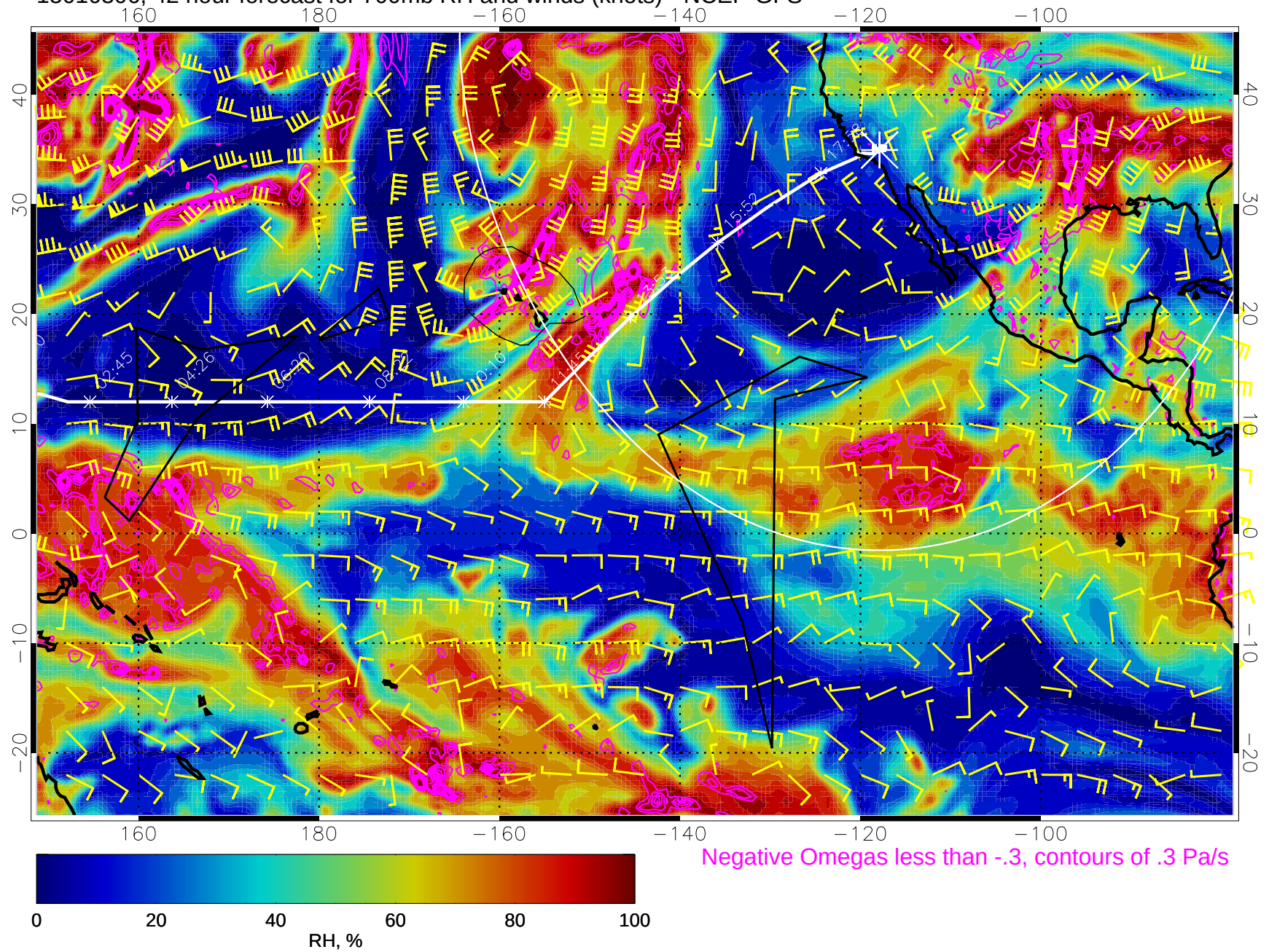
15010306, 42 hour forecast for 700mb RH and winds (knots) - NCEP GFS
