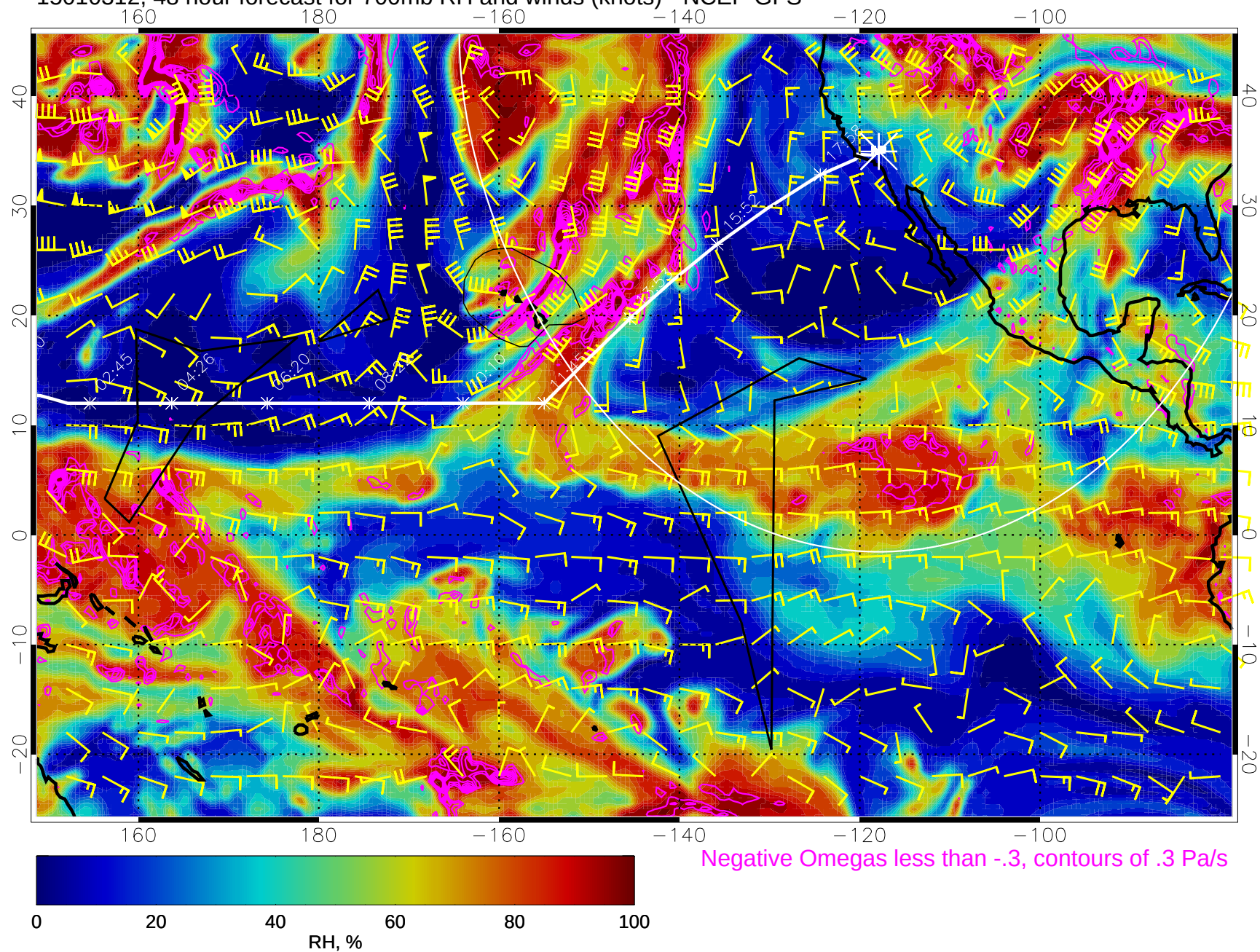
15010312, 48 hour forecast for 700mb RH and winds (knots) - NCEP GFS
