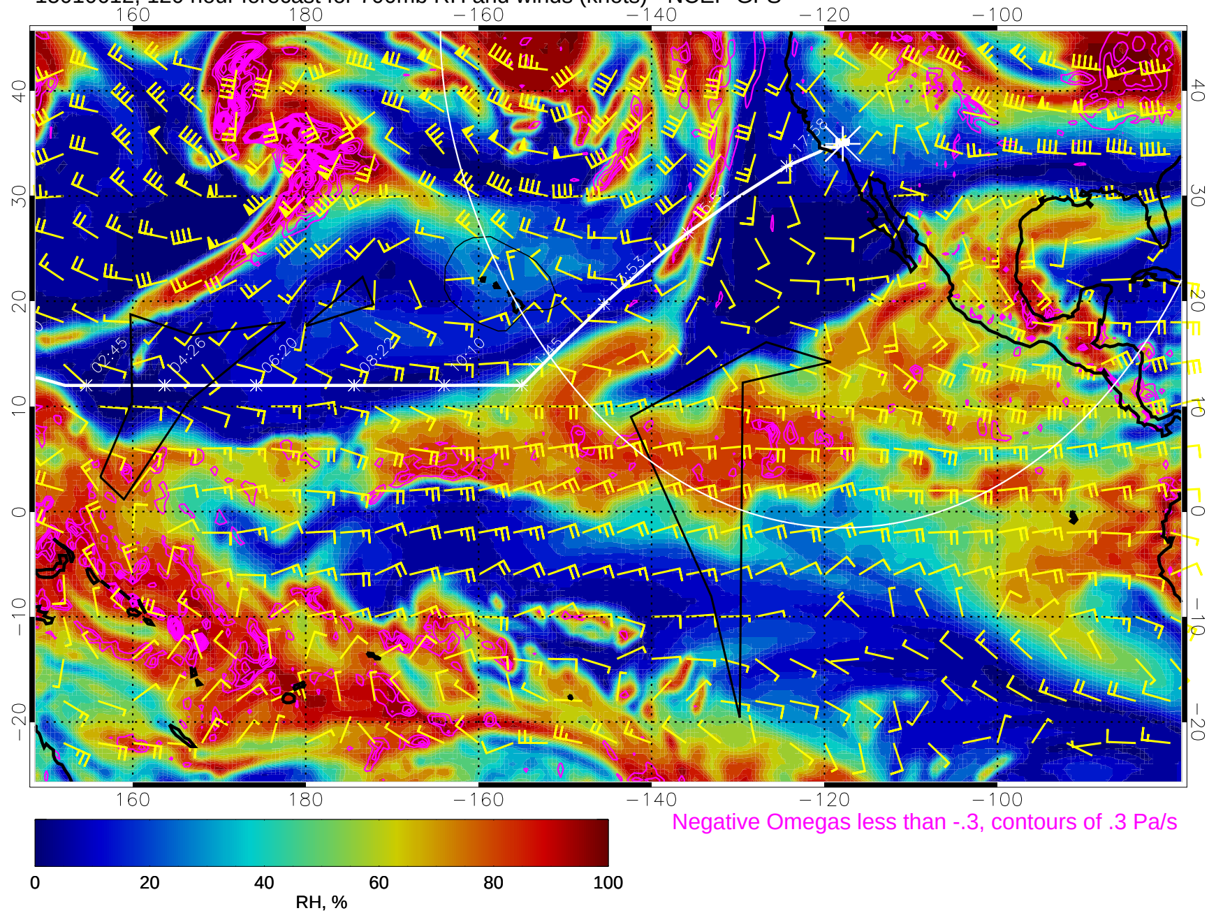
15010612, 120 hour forecast for 700mb RH and winds (knots) - NCEP GFS
