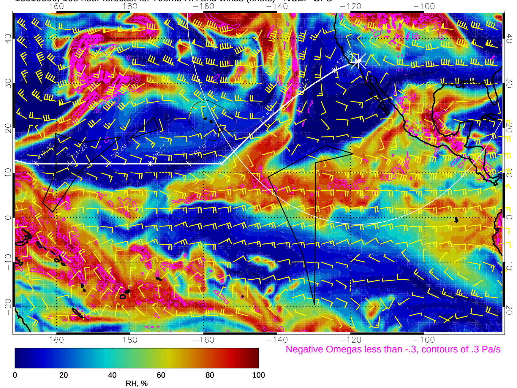
15010600, 108 hour forecast for 700mb RH and winds (knots) - NCEP GFS
