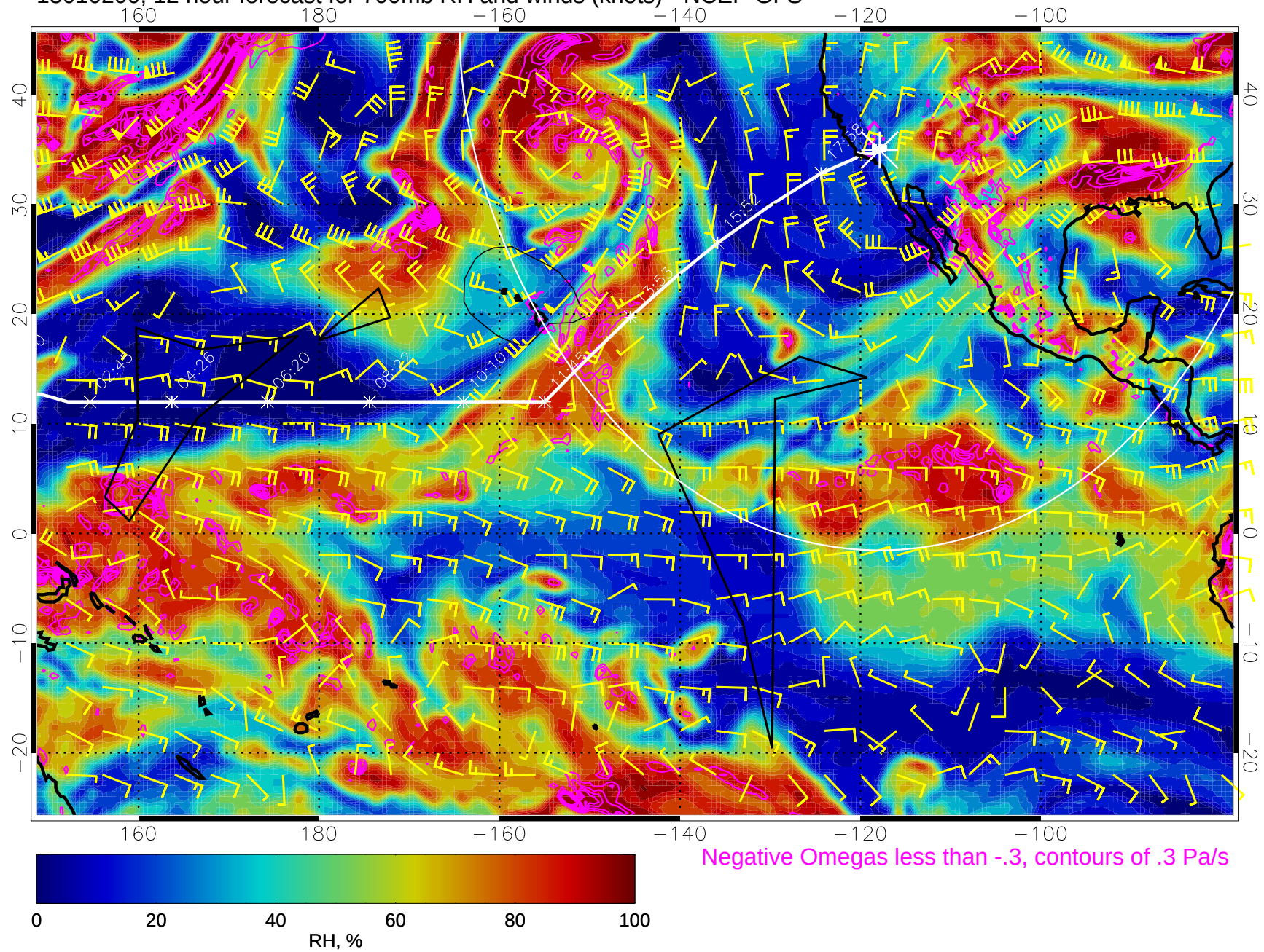
15010200, 12 hour forecast for 700mb RH and winds (knots) - NCEP GFS
