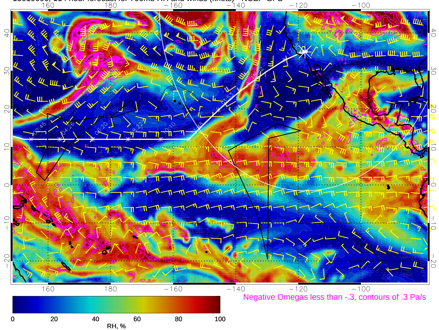
15010606, 114 hour forecast for 700mb RH and winds (knots) - NCEP GFS
