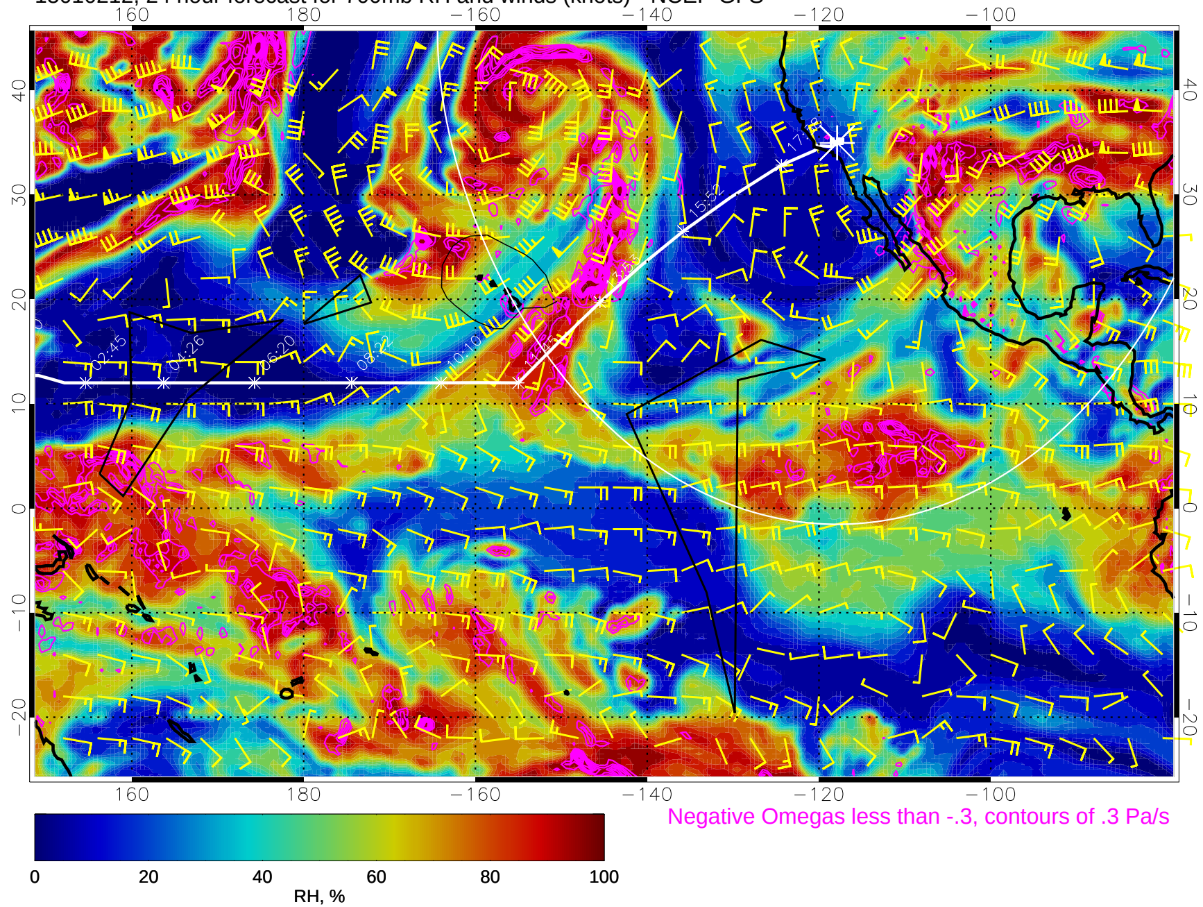
15010212, 24 hour forecast for 700mb RH and winds (knots) - NCEP GFS
