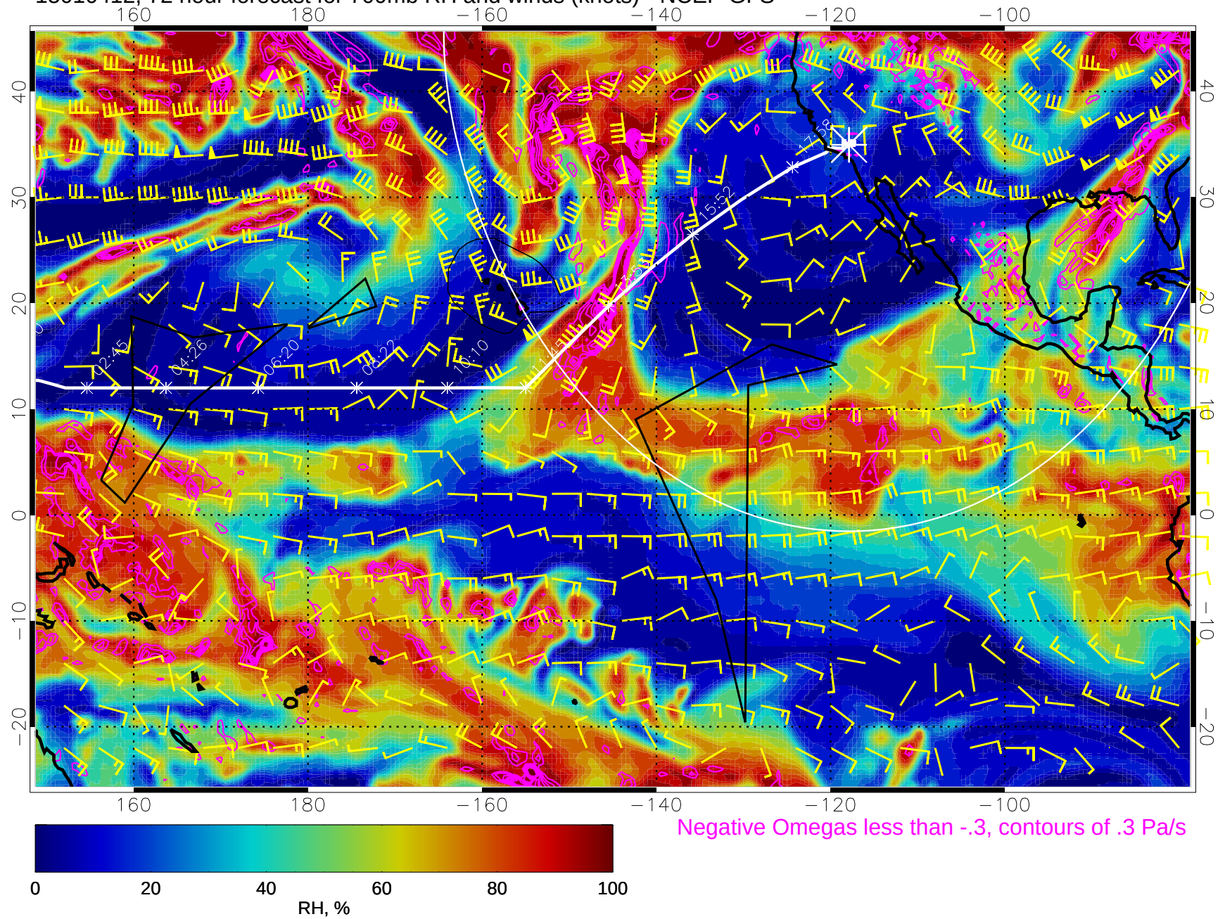
15010412, 72 hour forecast for 700mb RH and winds (knots) - NCEP GFS
