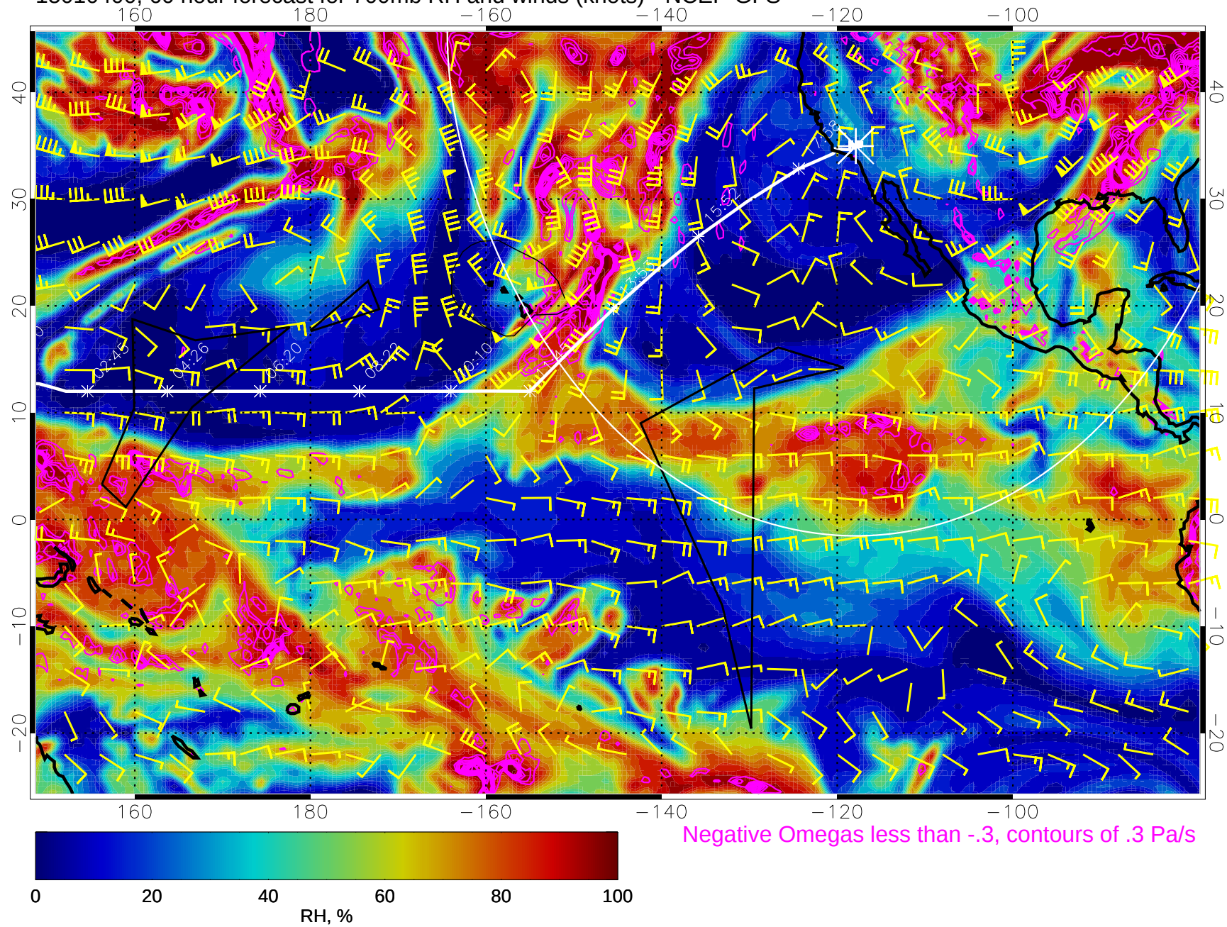
15010400, 60 hour forecast for 700mb RH and winds (knots) - NCEP GFS
