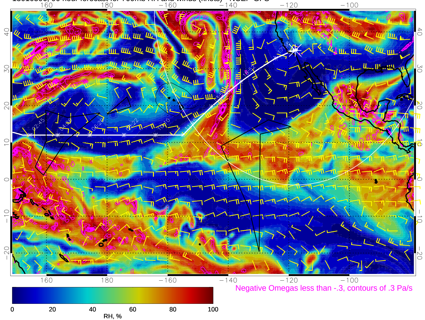
15010506, 90 hour forecast for 700mb RH and winds (knots) - NCEP GFS
