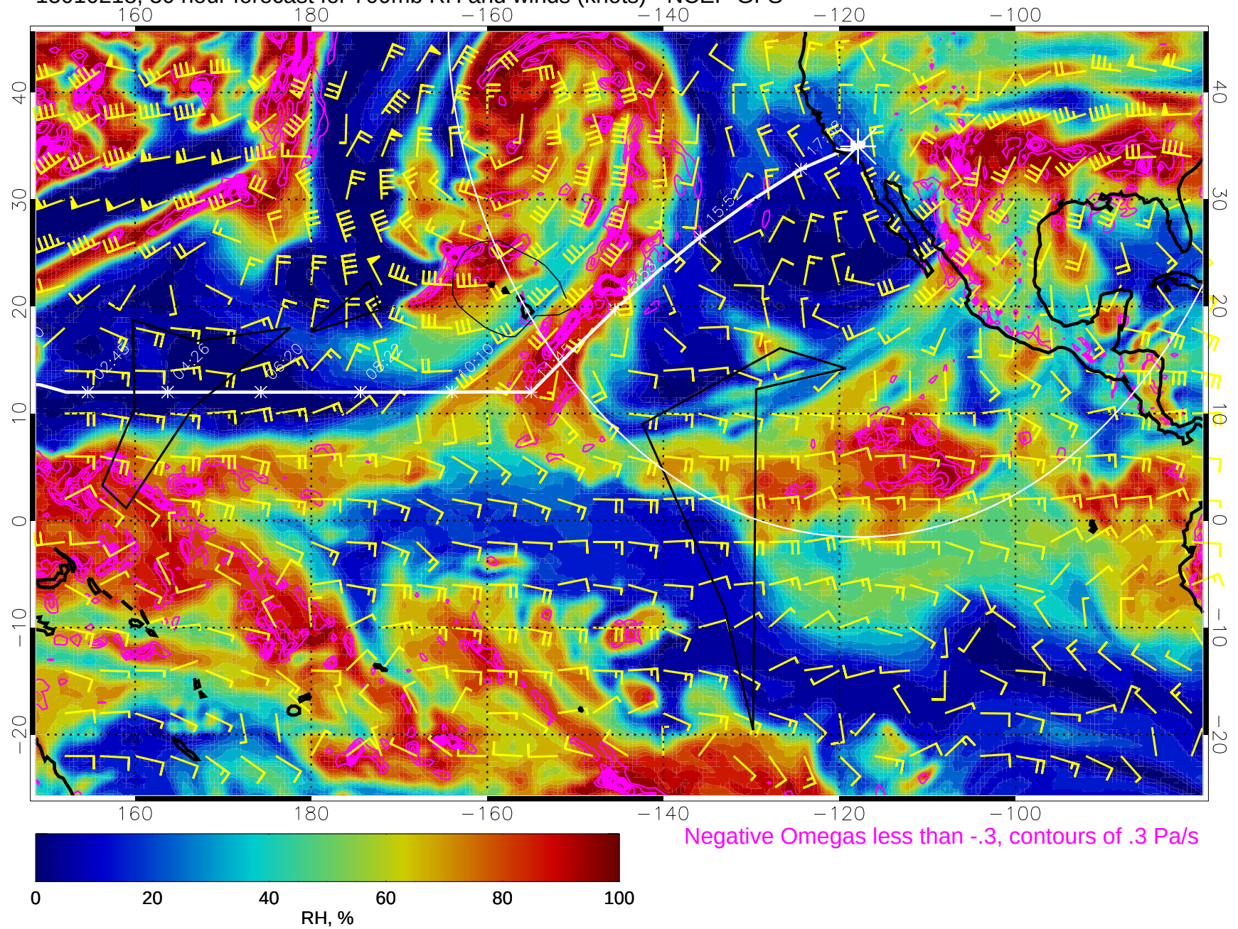
15010218, 30 hour forecast for 700mb RH and winds (knots) - NCEP GFS
