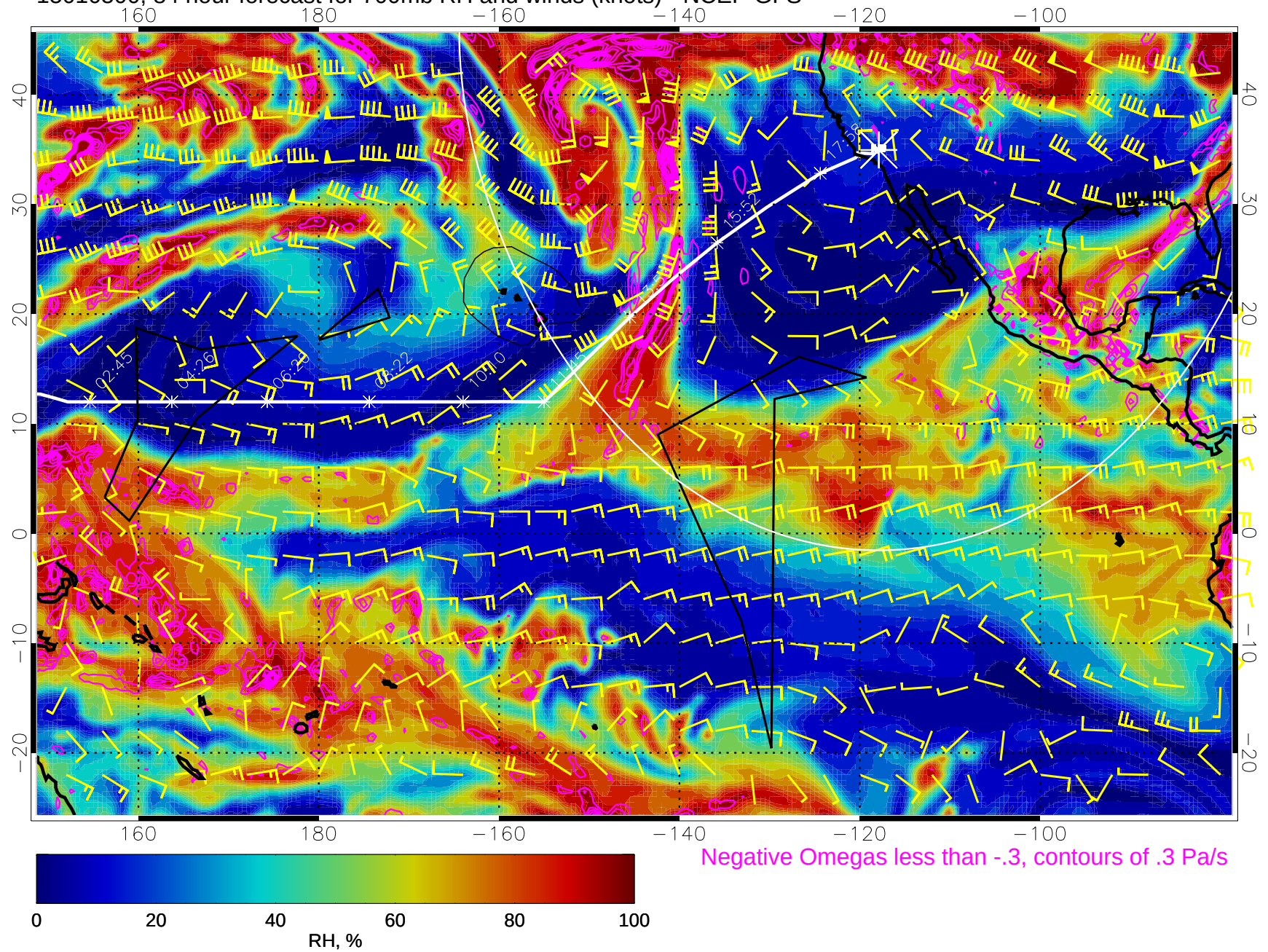
15010500, 84 hour forecast for 700mb RH and winds (knots) - NCEP GFS
