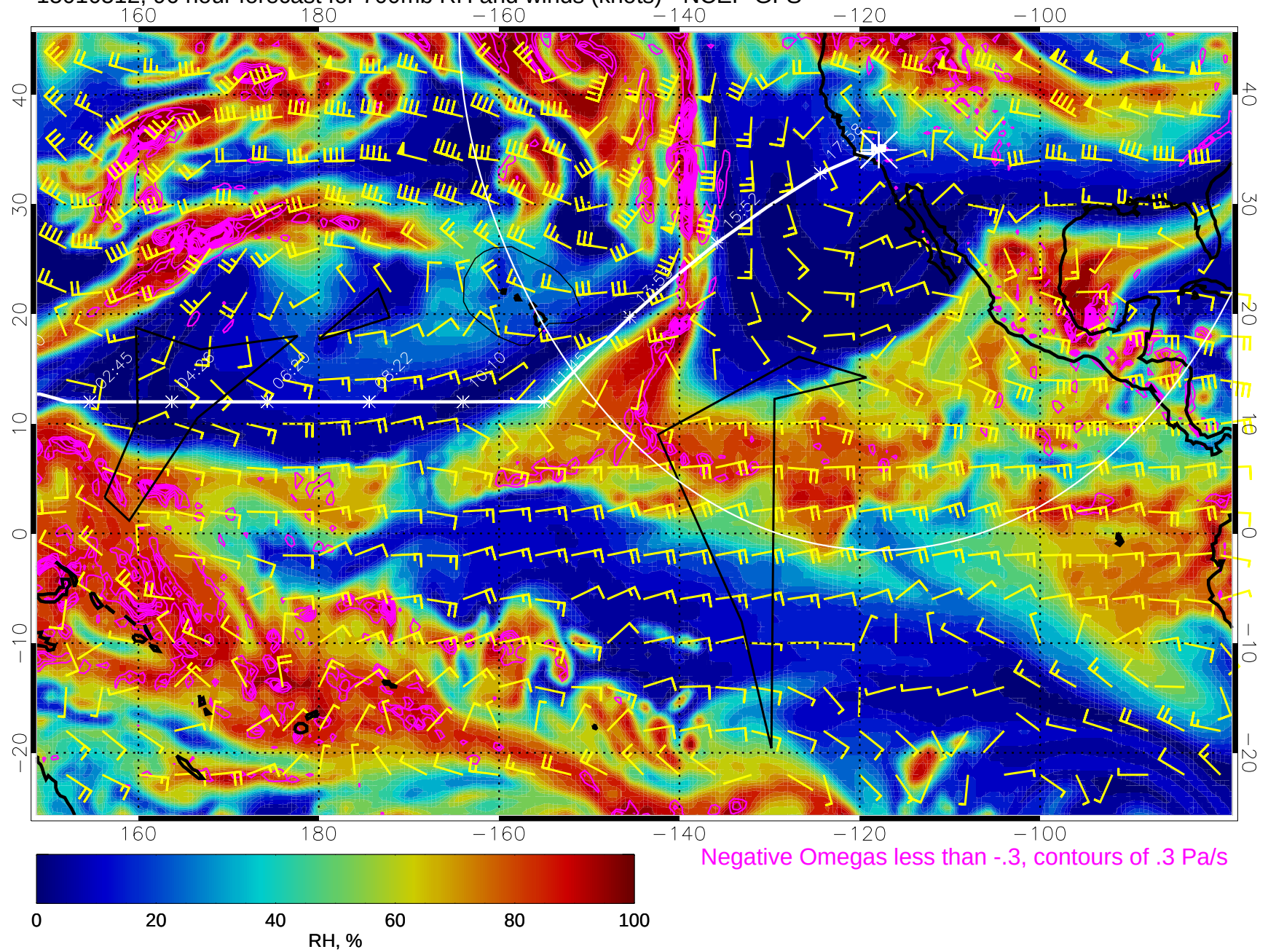
15010512, 96 hour forecast for 700mb RH and winds (knots) - NCEP GFS
