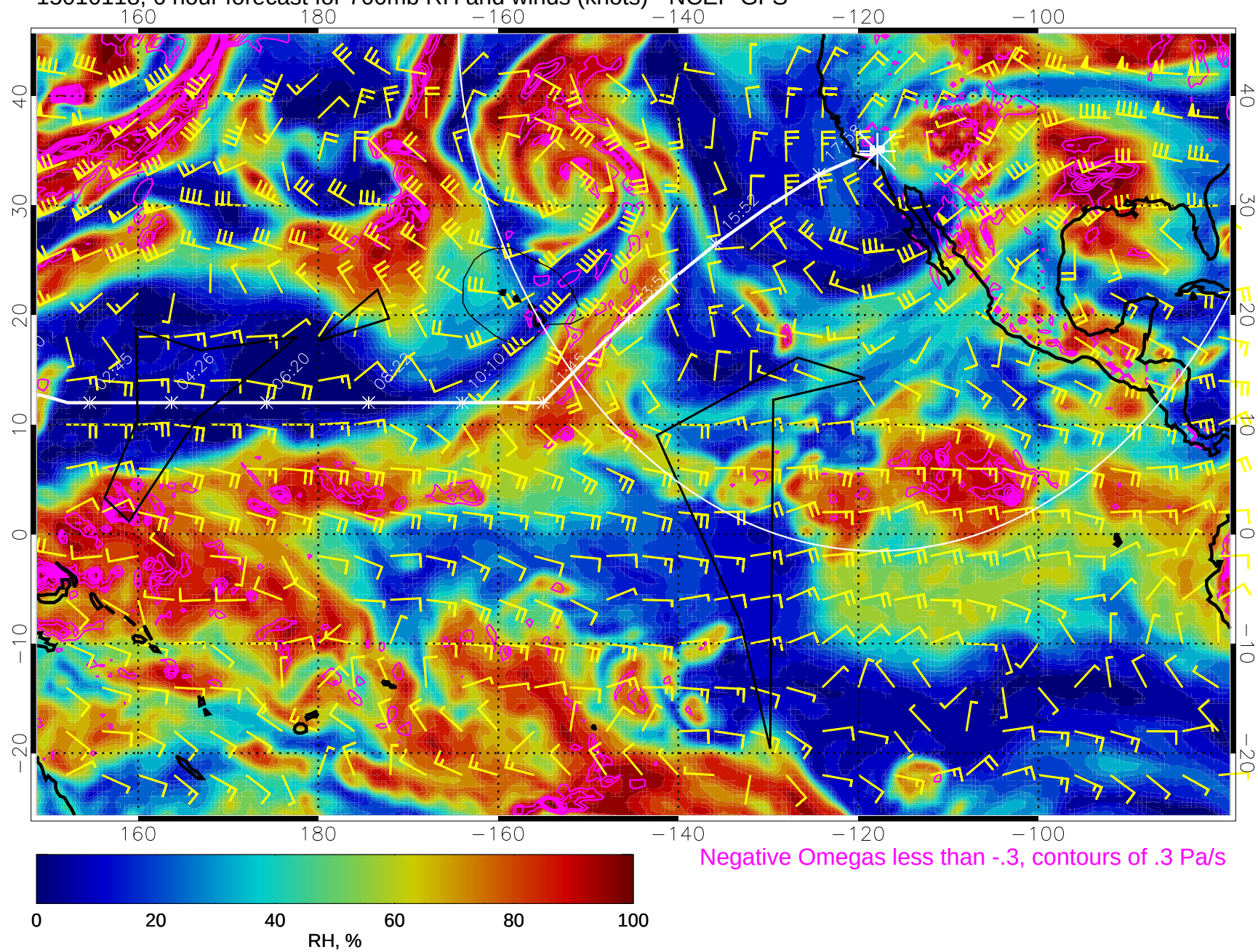
15010118, 6 hour forecast for 700mb RH and winds (knots) - NCEP GFS
