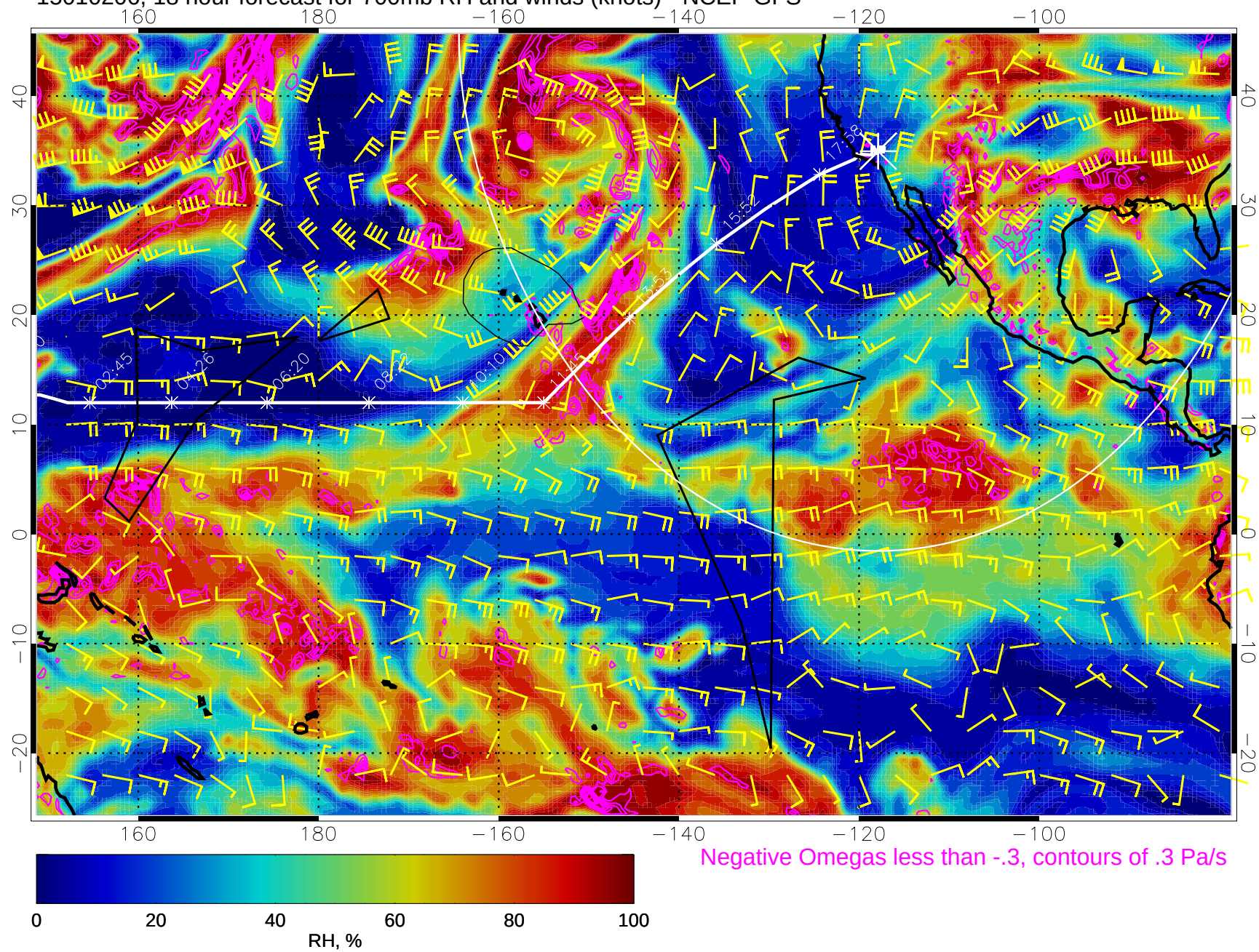
15010206, 18 hour forecast for 700mb RH and winds (knots) - NCEP GFS
