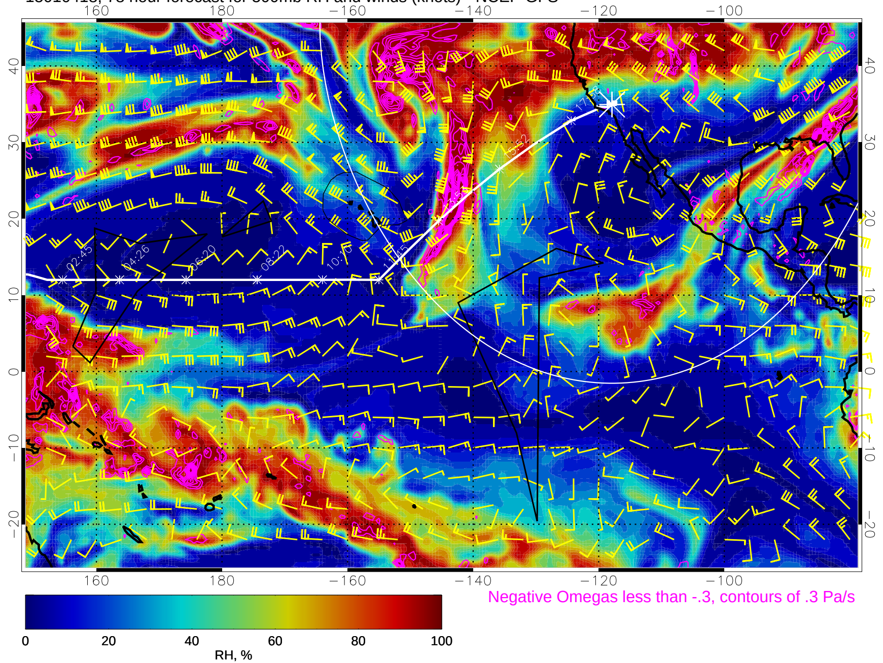
15010418, 78 hour forecast for 500mb RH and winds (knots) - NCEP GFS
