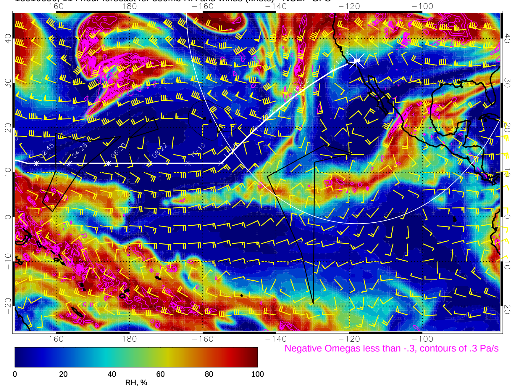
15010606, 114 hour forecast for 500mb RH and winds (knots) - NCEP GFS
