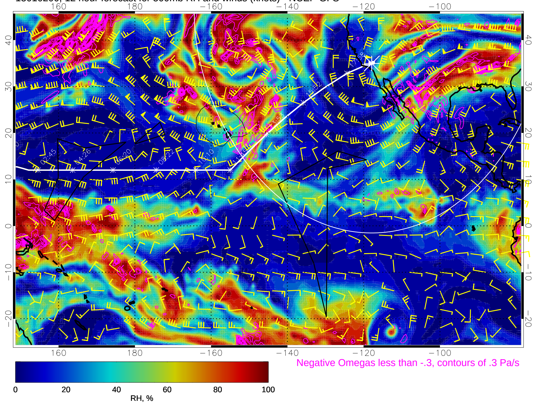
15010200, 12 hour forecast for 500mb RH and winds (knots) - NCEP GFS
