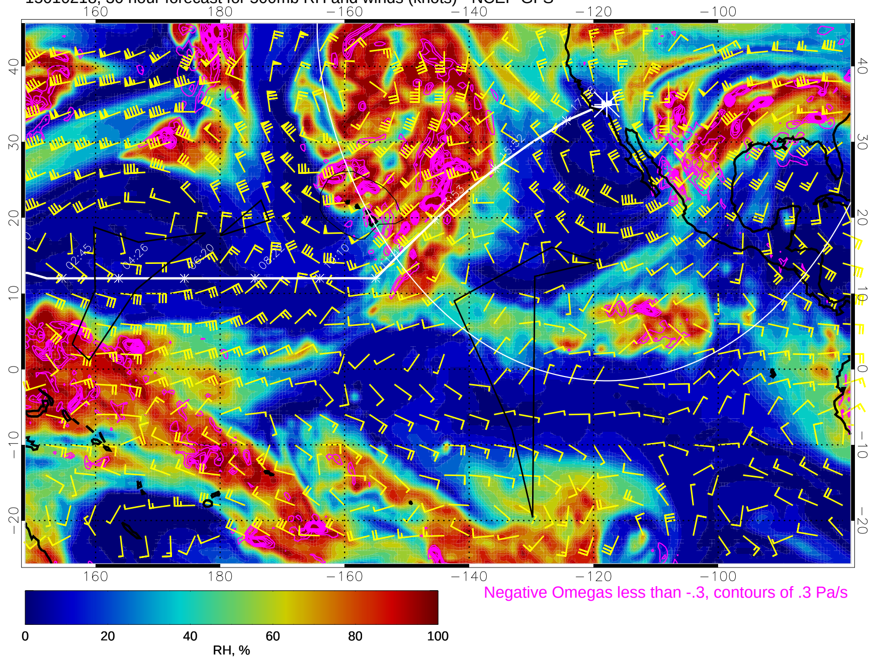
15010218, 30 hour forecast for 500mb RH and winds (knots) - NCEP GFS
