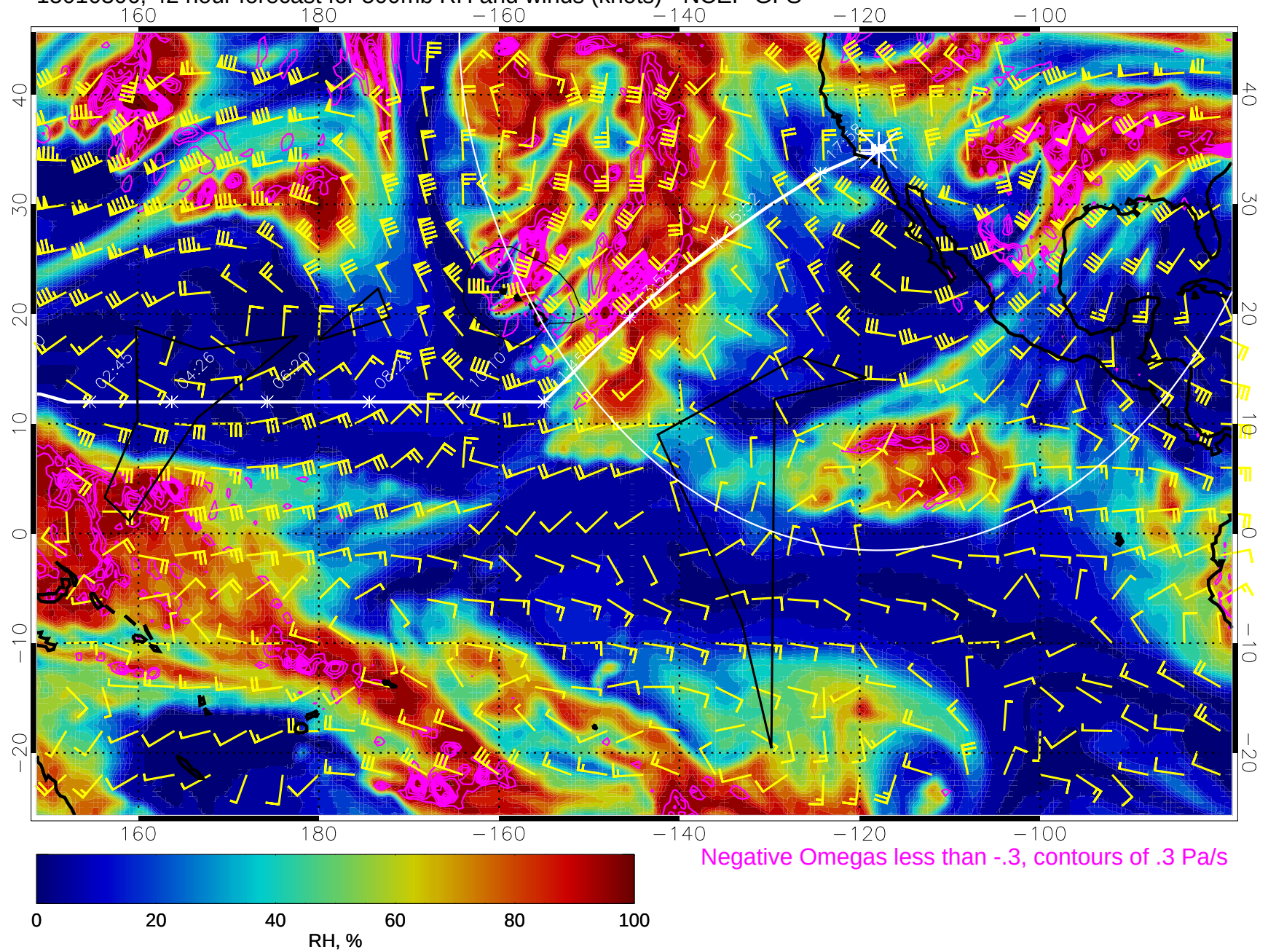
15010306, 42 hour forecast for 500mb RH and winds (knots) - NCEP GFS
