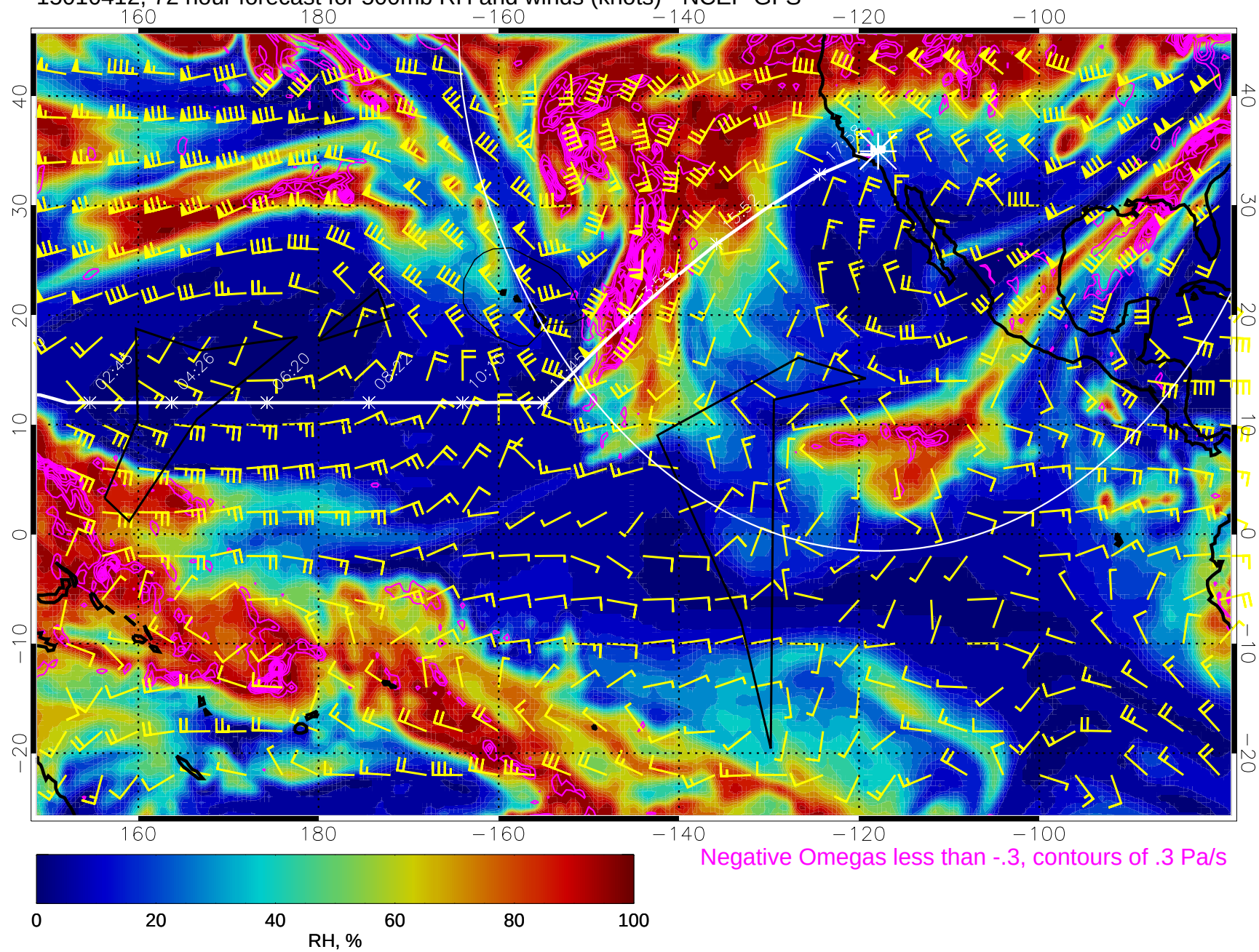
15010412, 72 hour forecast for 500mb RH and winds (knots) - NCEP GFS
