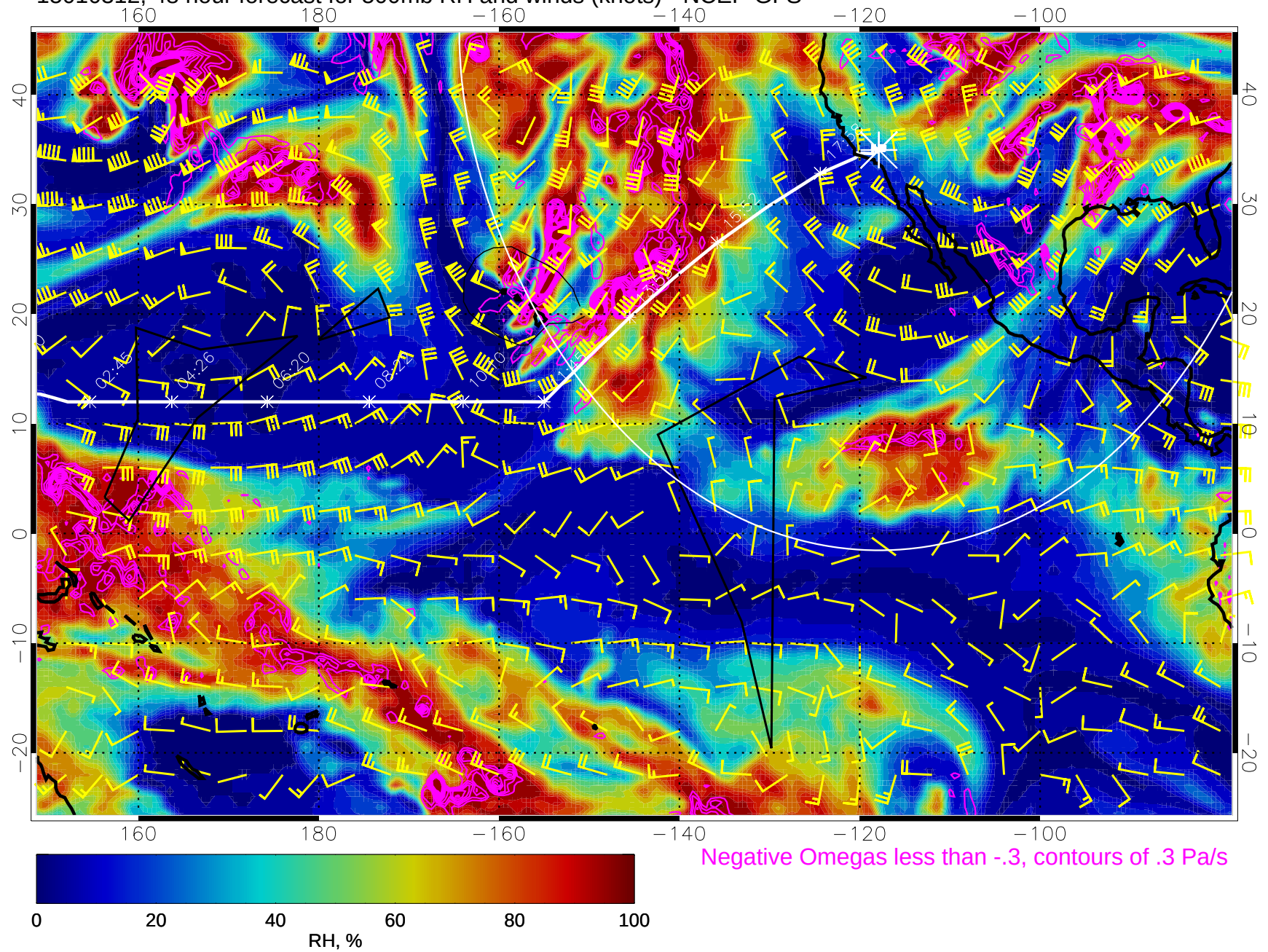
15010312, 48 hour forecast for 500mb RH and winds (knots) - NCEP GFS
