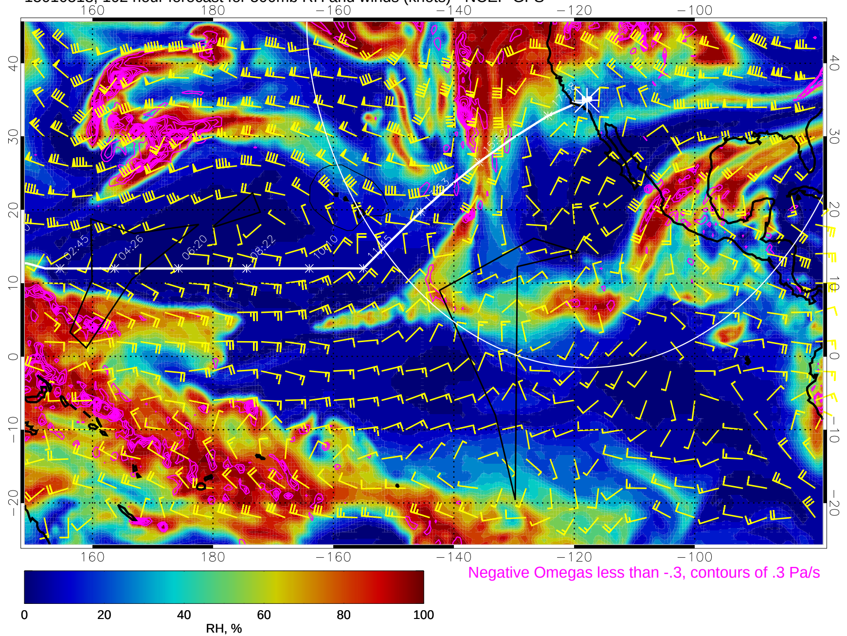
15010518, 102 hour forecast for 500mb RH and winds (knots) - NCEP GFS
