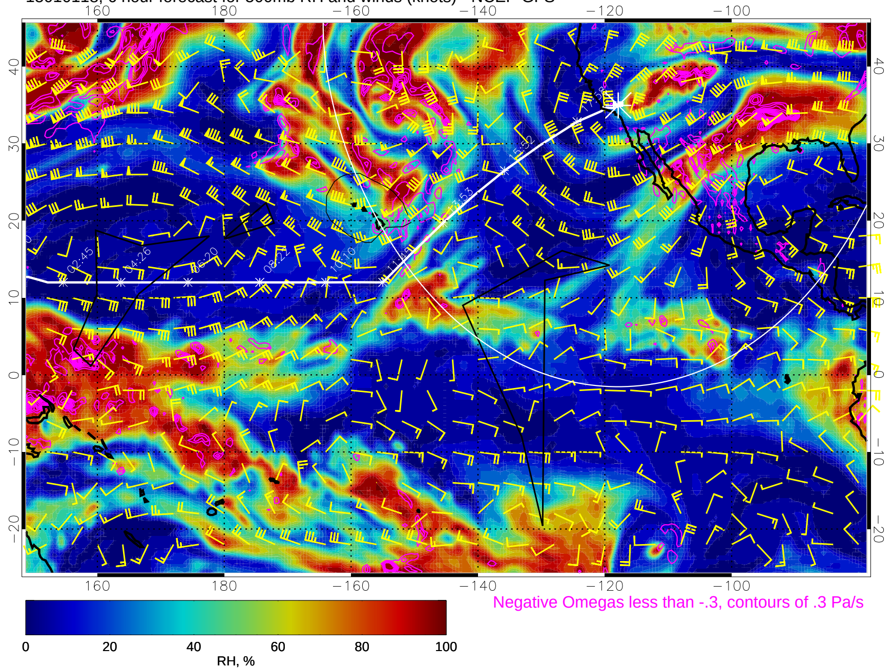
15010118, 6 hour forecast for 500mb RH and winds (knots) - NCEP GFS
