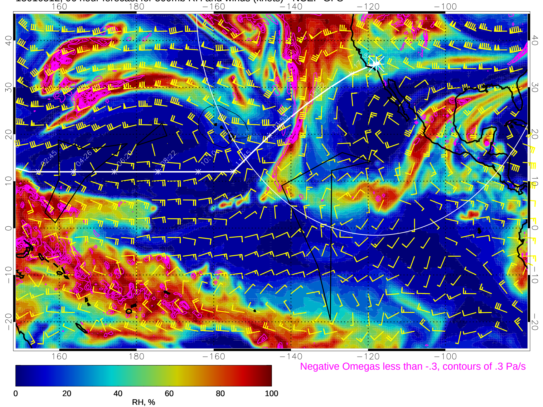
15010512, 96 hour forecast for 500mb RH and winds (knots) - NCEP GFS
