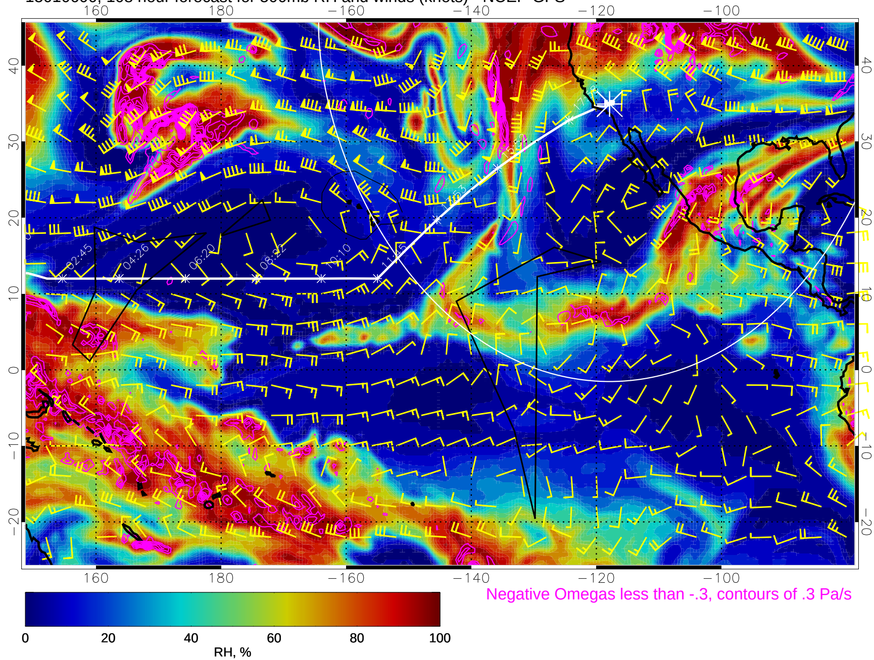
15010600, 108 hour forecast for 500mb RH and winds (knots) - NCEP GFS
