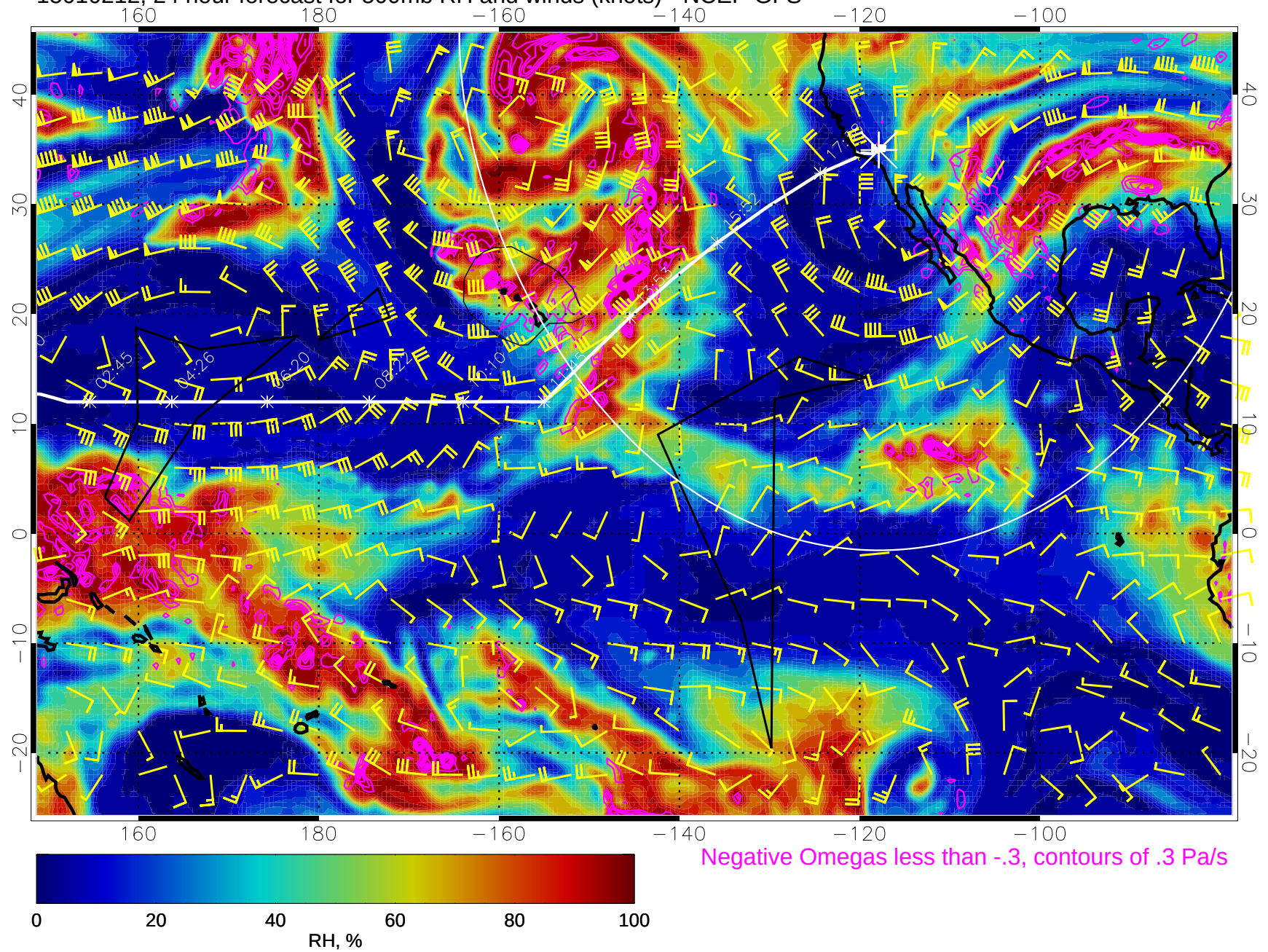
15010212, 24 hour forecast for 500mb RH and winds (knots) - NCEP GFS
