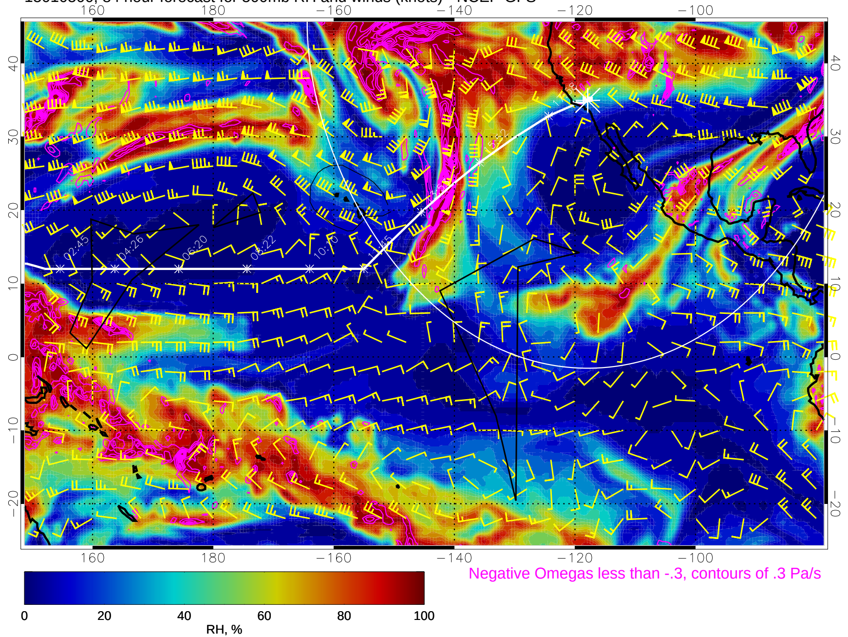
15010500, 84 hour forecast for 500mb RH and winds (knots) - NCEP GFS
