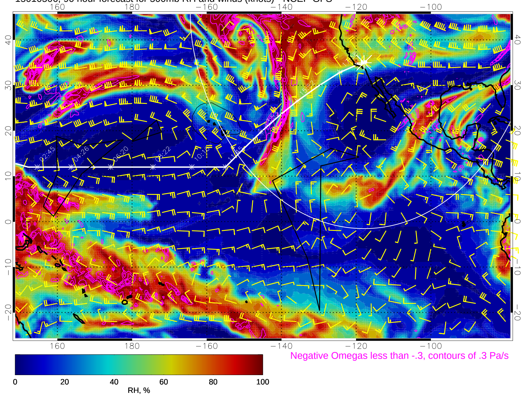
15010506, 90 hour forecast for 500mb RH and winds (knots) - NCEP GFS
