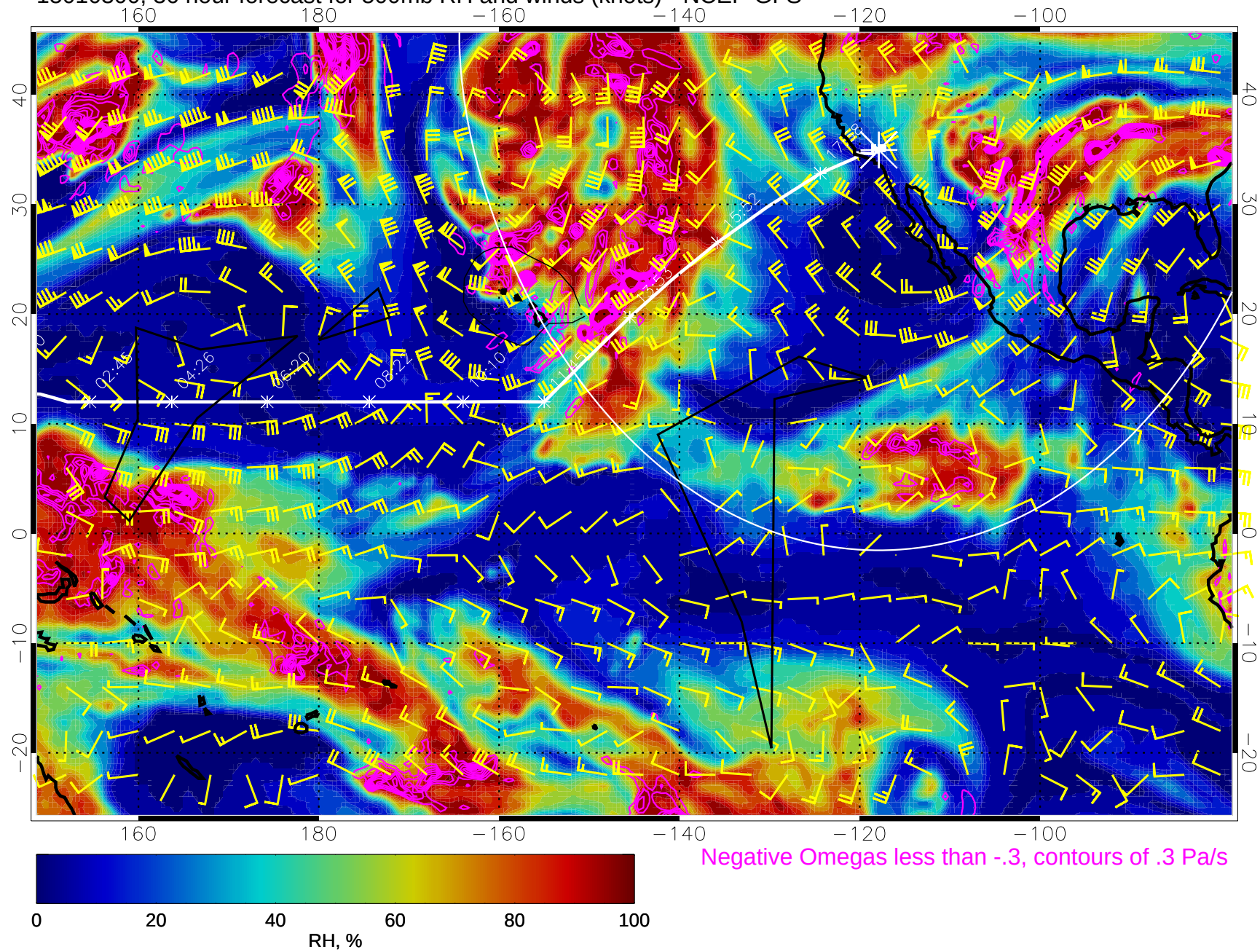
15010300, 36 hour forecast for 500mb RH and winds (knots) - NCEP GFS
