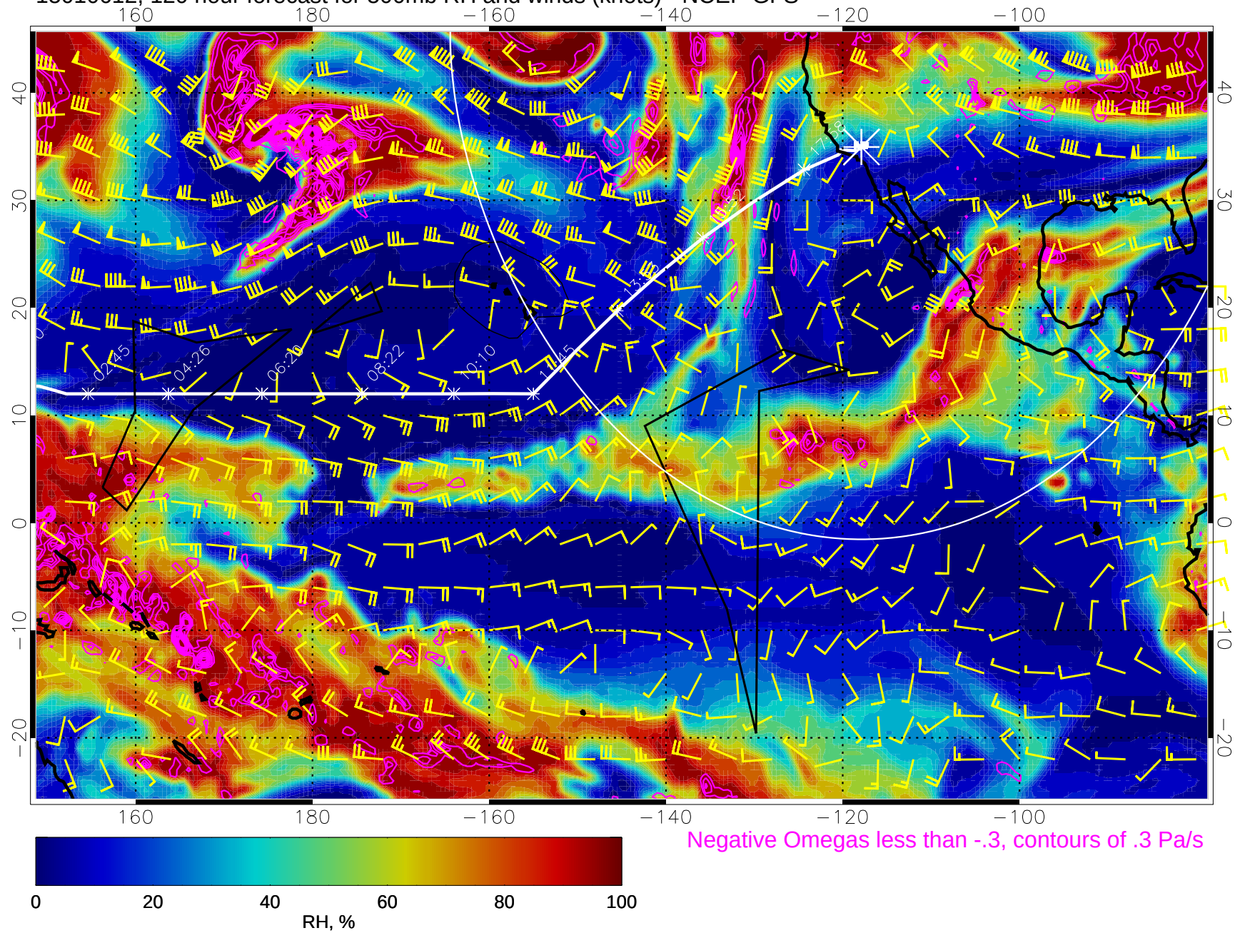
15010612, 120 hour forecast for 500mb RH and winds (knots) - NCEP GFS
