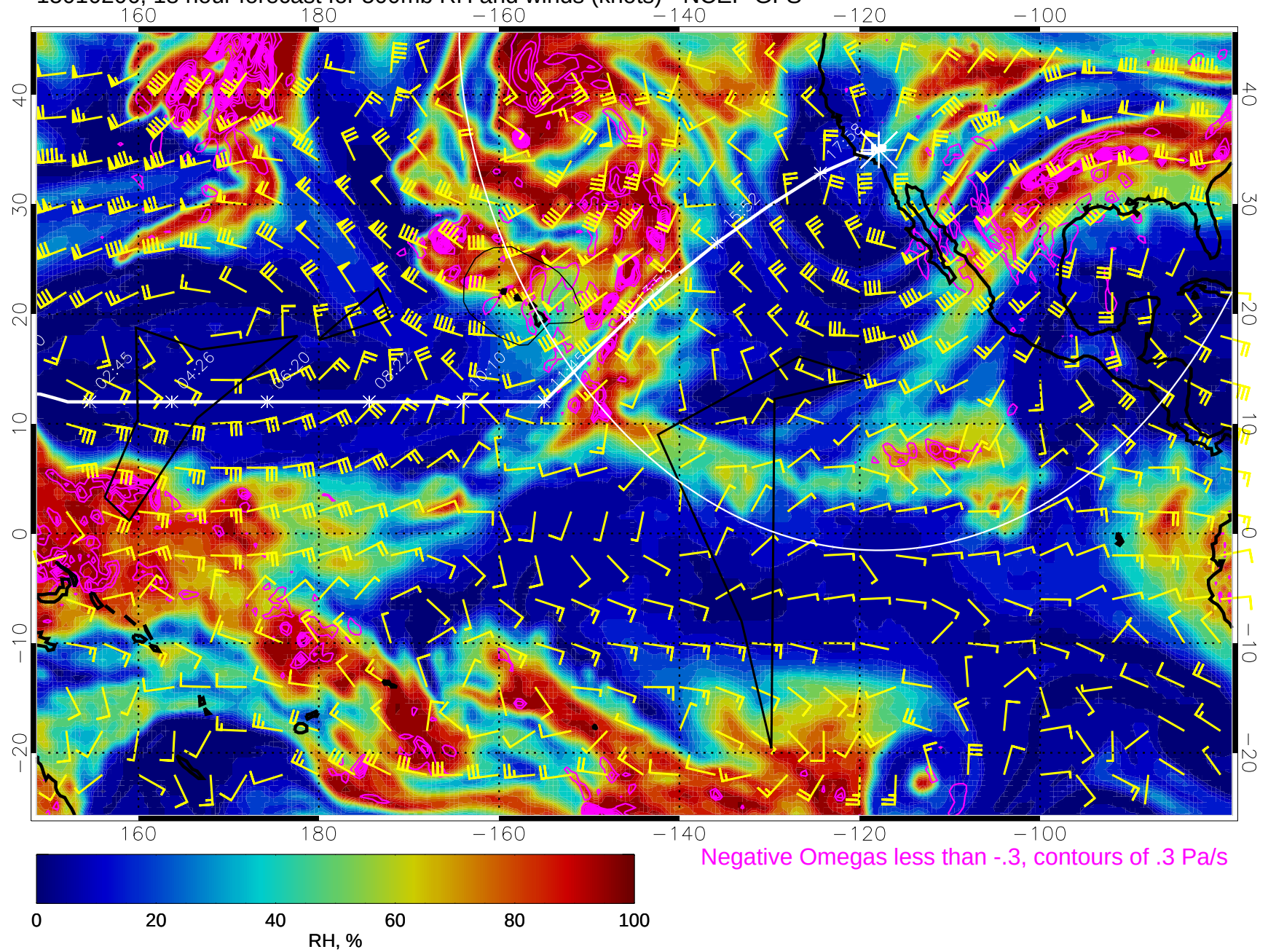
15010206, 18 hour forecast for 500mb RH and winds (knots) - NCEP GFS
