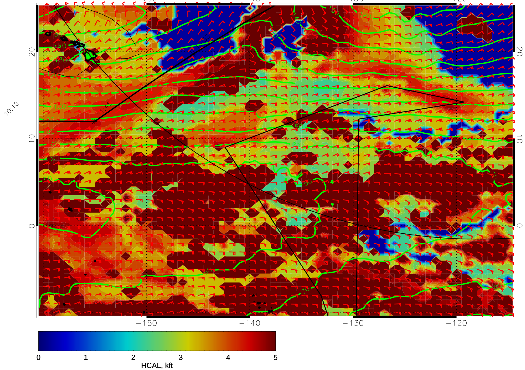
15010612, 120 hour forecast for HCAL, 1000mb Z, and winds (knots) -- NCEP GFS
