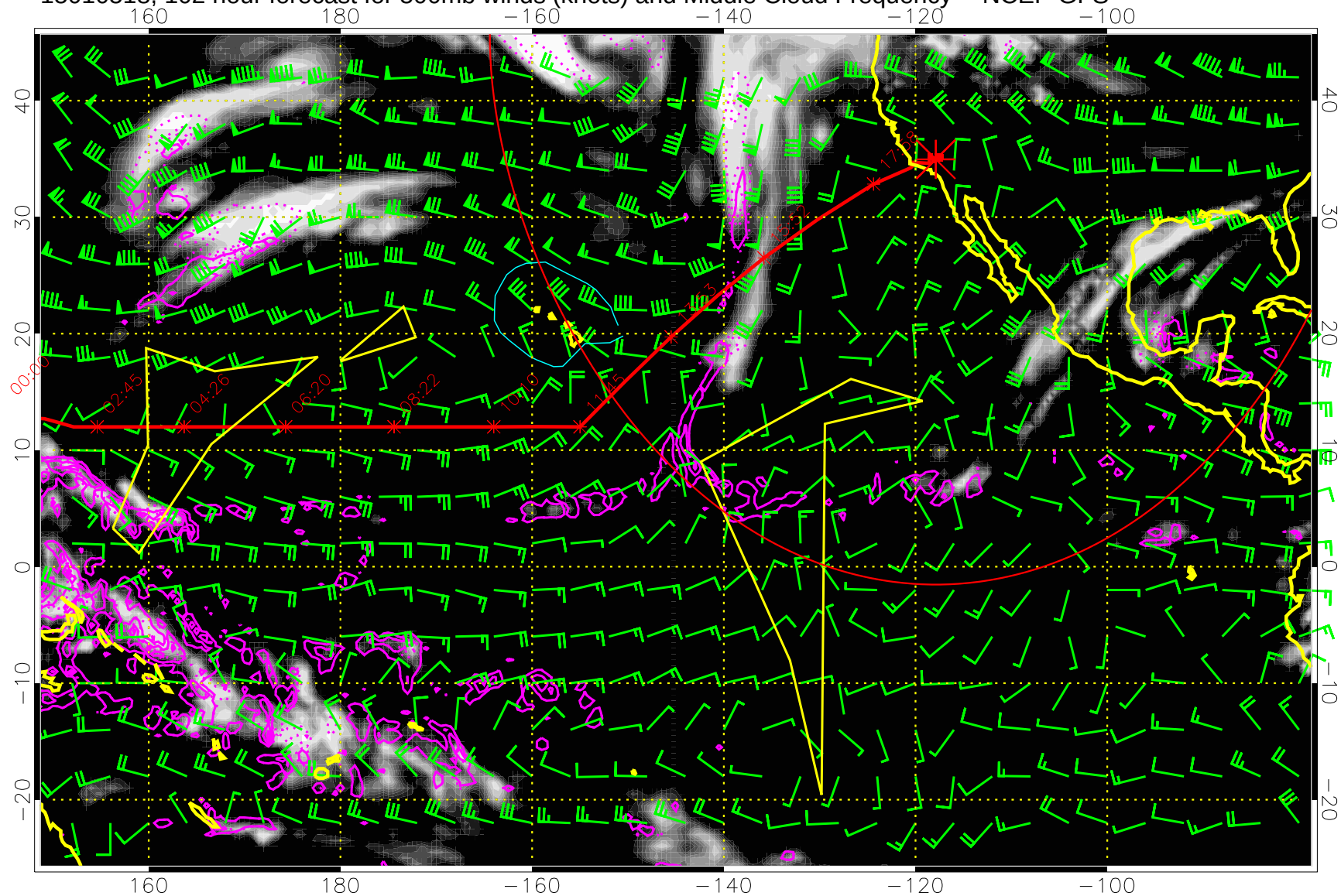
15010518, 102 hour forecast for 500mb winds (knots) and Middle Cloud Frequency -- NCEP GFS
