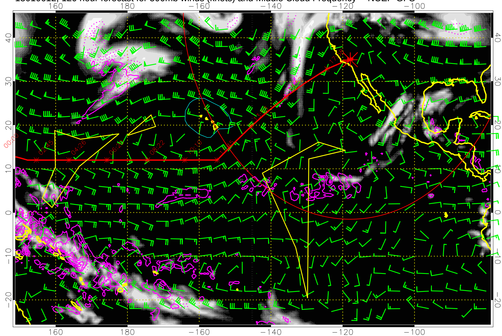
15010612, 120 hour forecast for 500mb winds (knots) and Middle Cloud Frequency -- NCEP GFS
