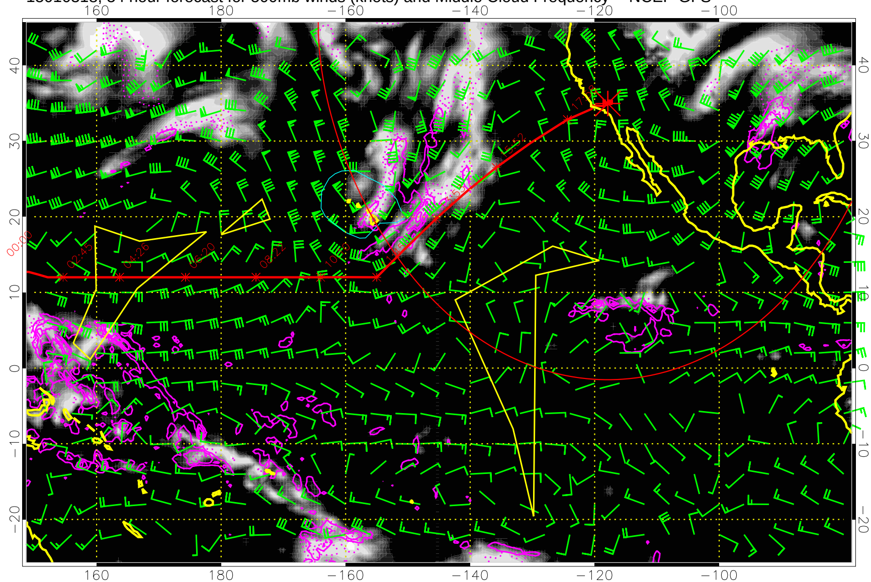
15010318, 54 hour forecast for 500mb winds (knots) and Middle Cloud Frequency -- NCEP GFS
