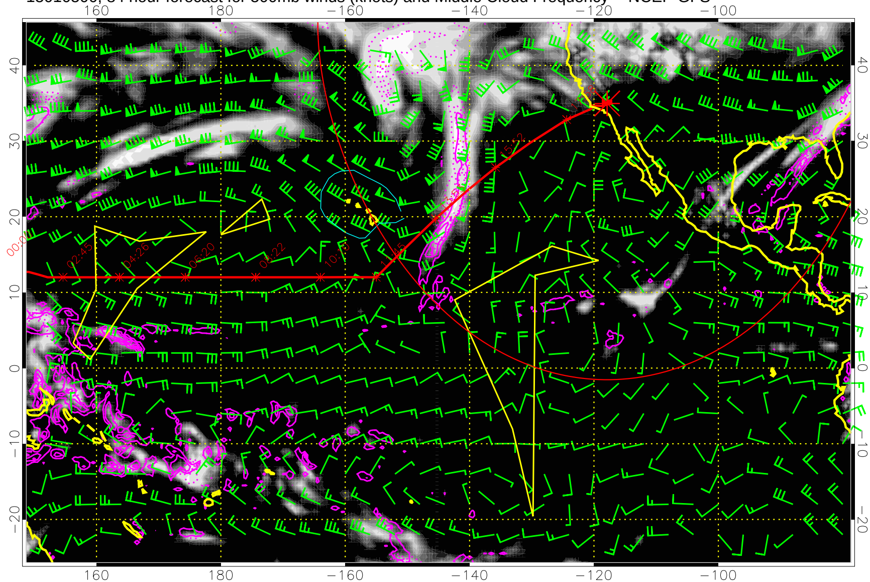
15010500, 84 hour forecast for 500mb winds (knots) and Middle Cloud Frequency -- NCEP GFS
