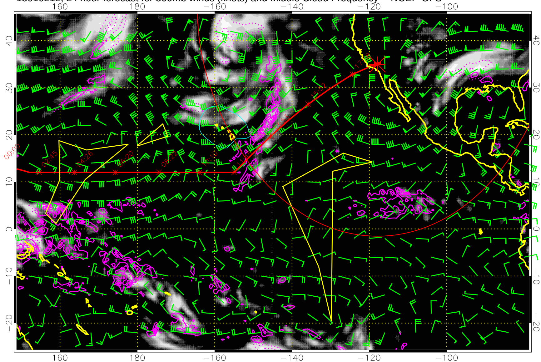
15010212, 24 hour forecast for 500mb winds (knots) and Middle Cloud Frequency -- NCEP GFS
