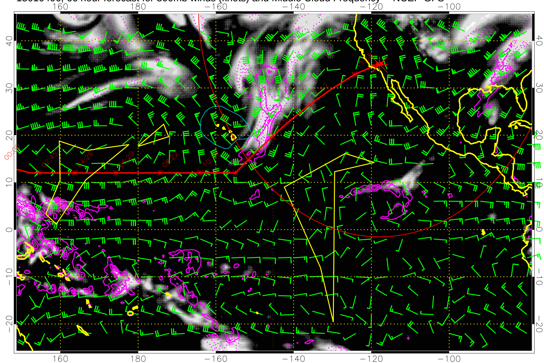
15010406, 66 hour forecast for 500mb winds (knots) and Middle Cloud Frequency -- NCEP GFS
