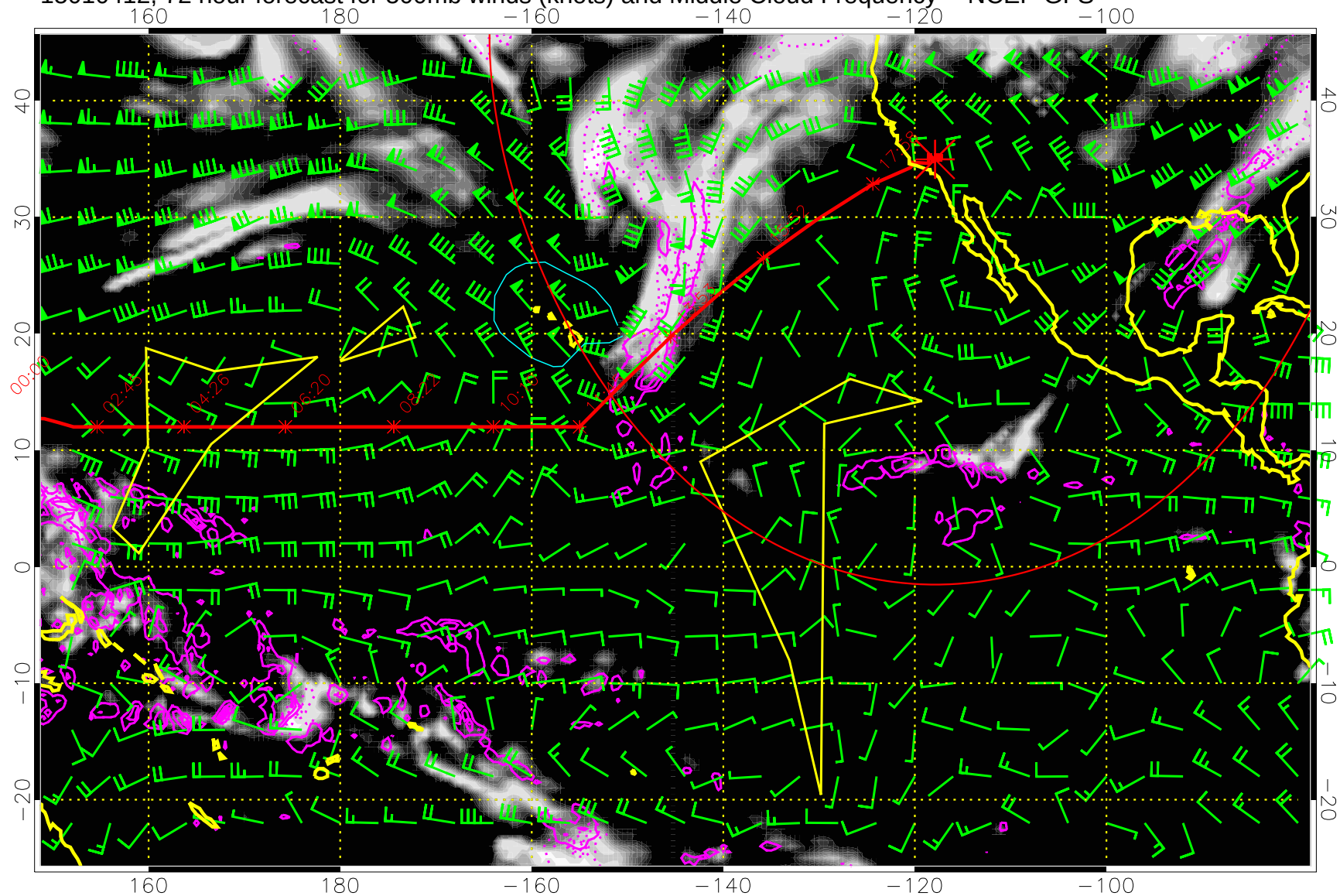
15010412, 72 hour forecast for 500mb winds (knots) and Middle Cloud Frequency -- NCEP GFS
