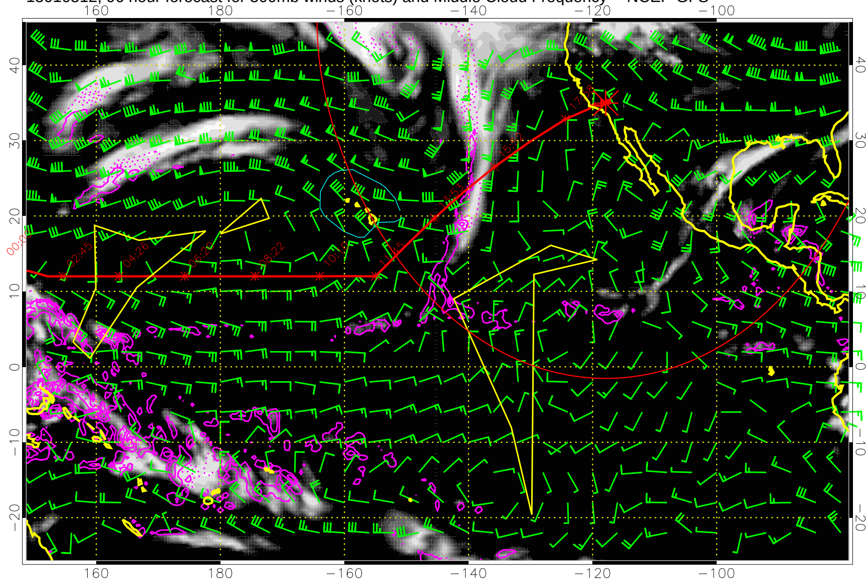
15010512, 96 hour forecast for 500mb winds (knots) and Middle Cloud Frequency -- NCEP GFS
