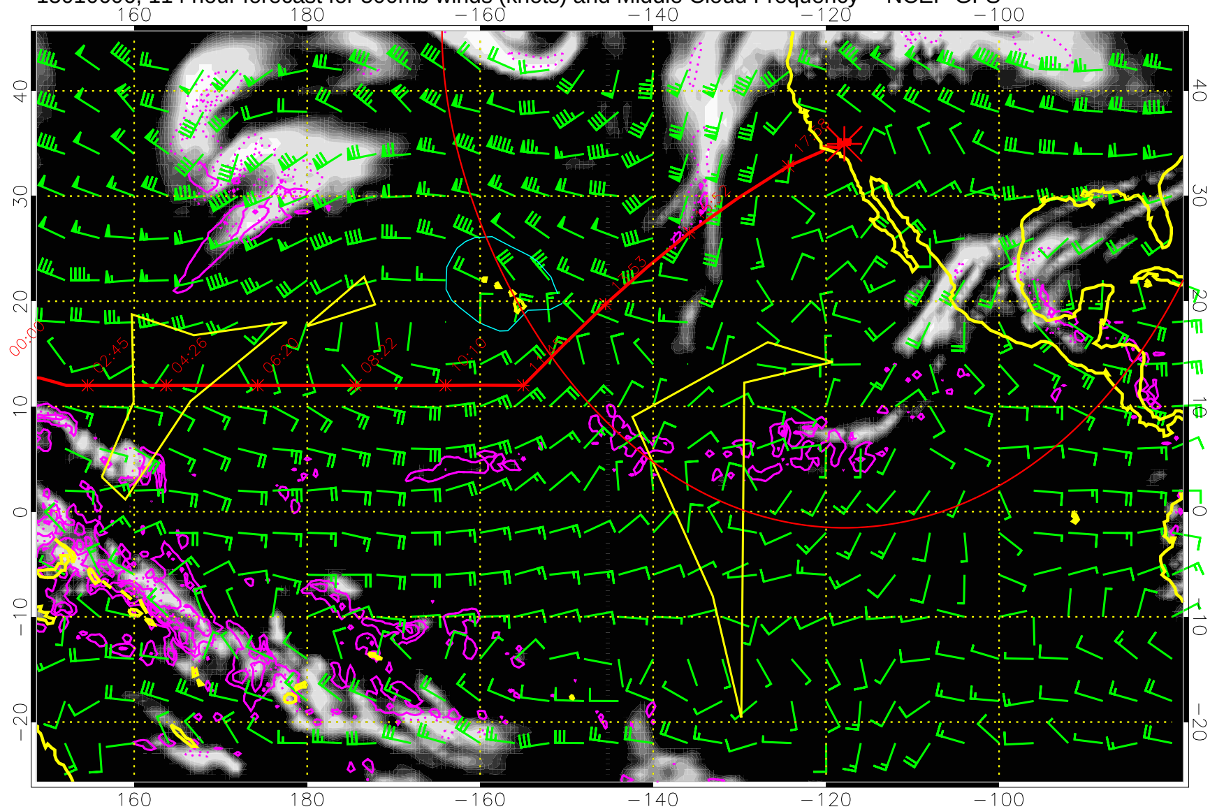
15010606, 114 hour forecast for 500mb winds (knots) and Middle Cloud Frequency -- NCEP GFS
