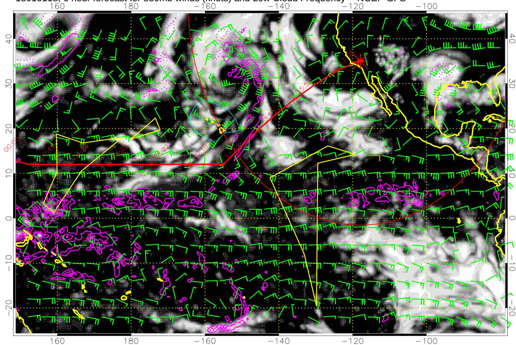
15010118, 6 hour forecast for 850mb winds (knots) and Low Cloud Frequency -- NCEP GFS
