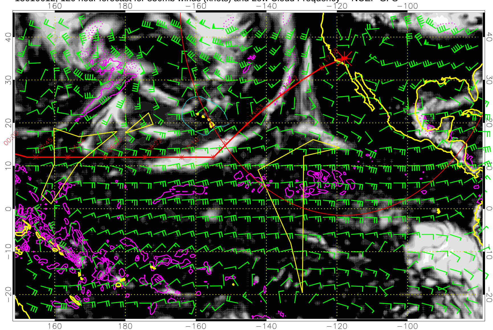
15010612, 120 hour forecast for 850mb winds (knots) and Low Cloud Frequency -- NCEP GFS
