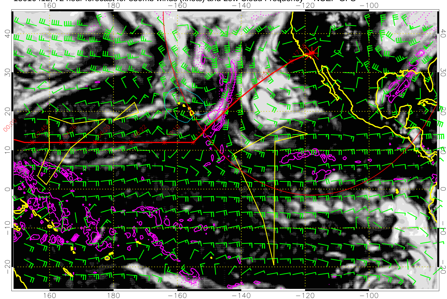
15010412, 72 hour forecast for 850mb winds (knots) and Low Cloud Frequency -- NCEP GFS
