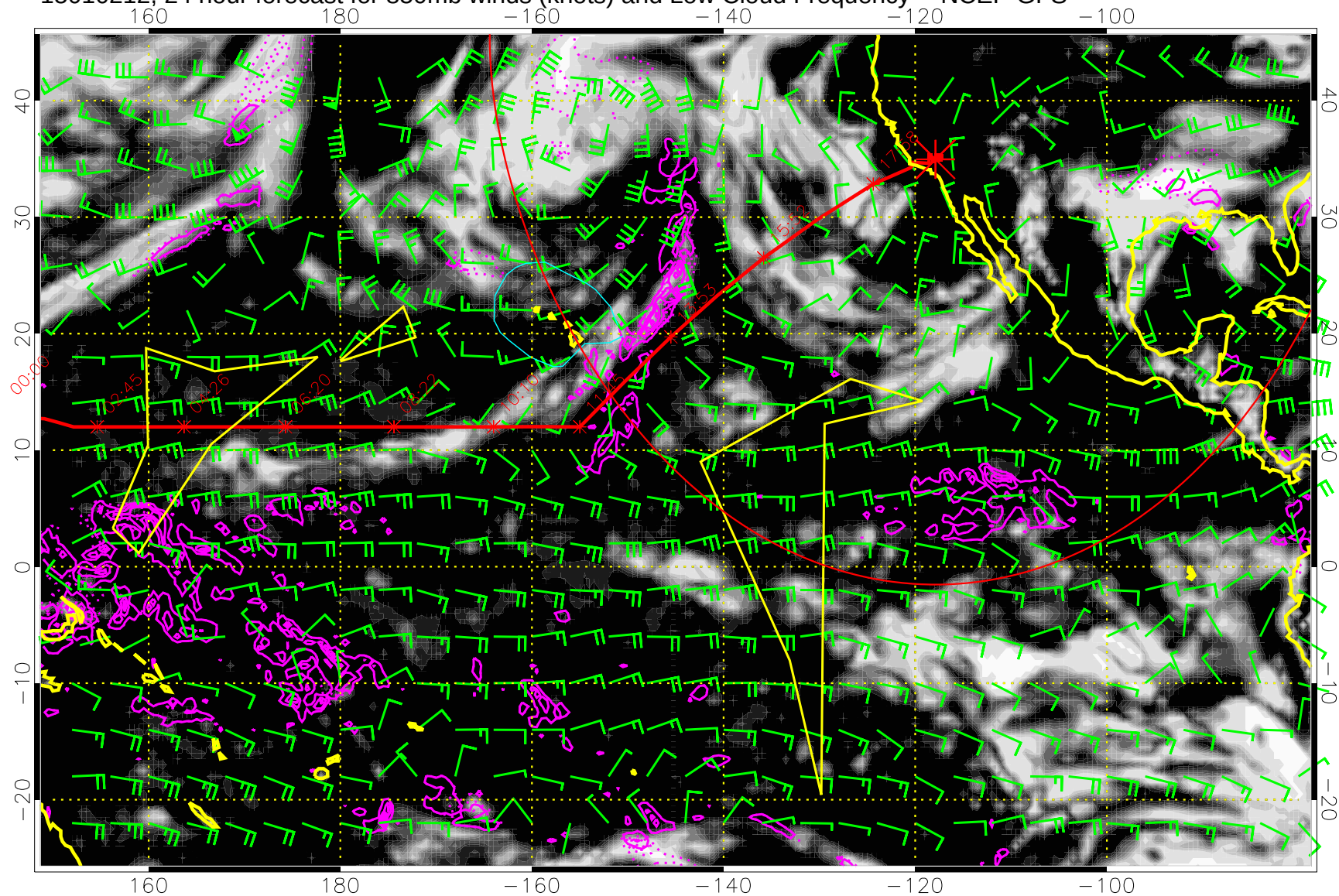
15010212, 24 hour forecast for 850mb winds (knots) and Low Cloud Frequency -- NCEP GFS
