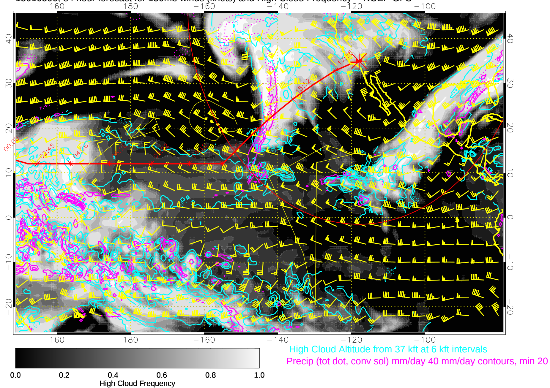
15010500, 84 hour forecast for 150mb winds (knots) and High Cloud Frequency -- NCEP GFS
