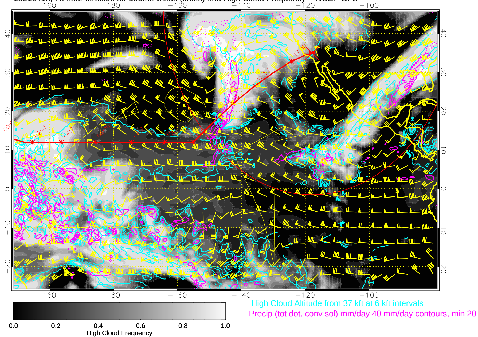
15010418, 78 hour forecast for 150mb winds (knots) and High Cloud Frequency -- NCEP GFS
