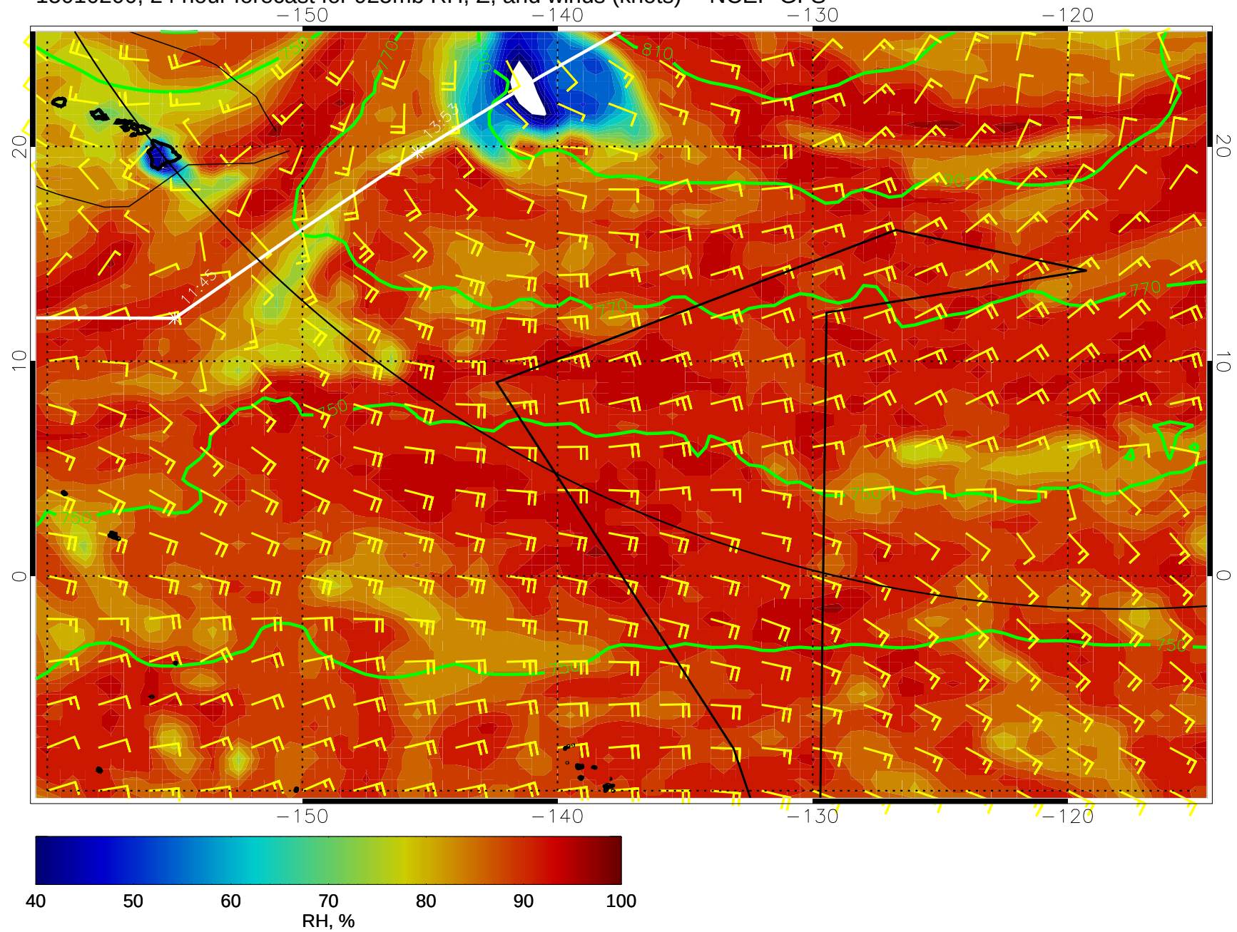
15010200, 24 hour forecast for 925mb RH, Z, and winds (knots) -- NCEP GFS
