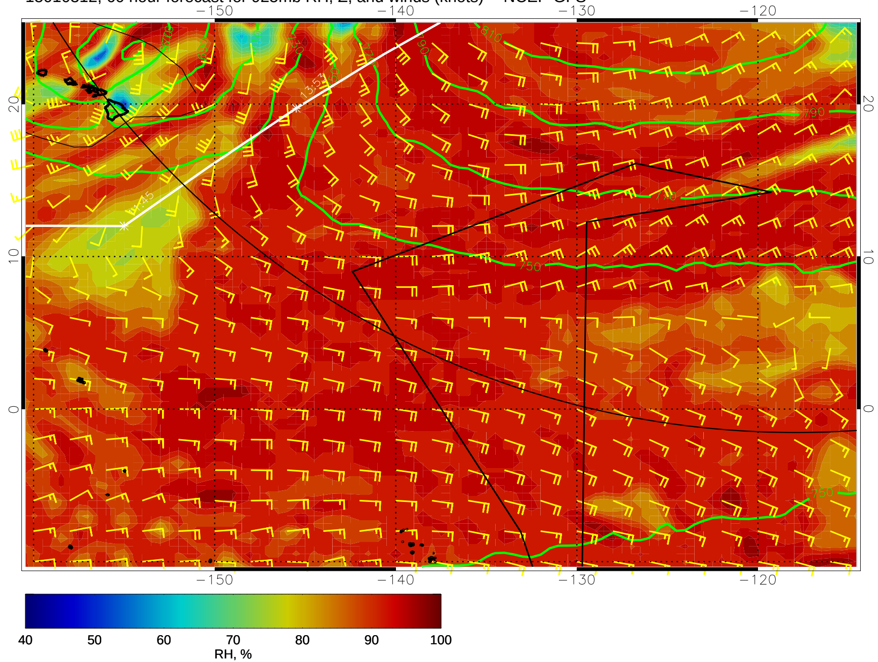
15010312, 60 hour forecast for 925mb RH, Z, and winds (knots) -- NCEP GFS
