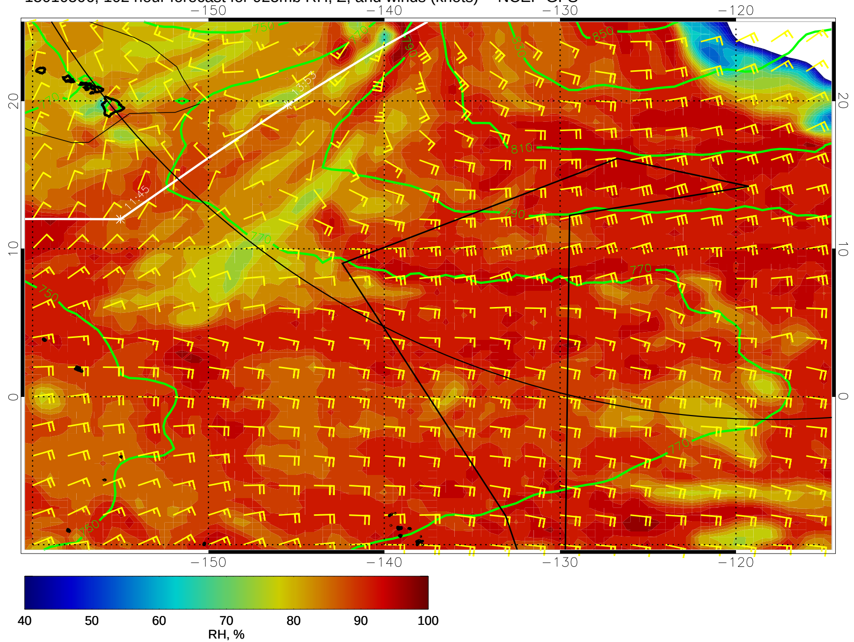
15010506, 102 hour forecast for 925mb RH, Z, and winds (knots) -- NCEP GFS
