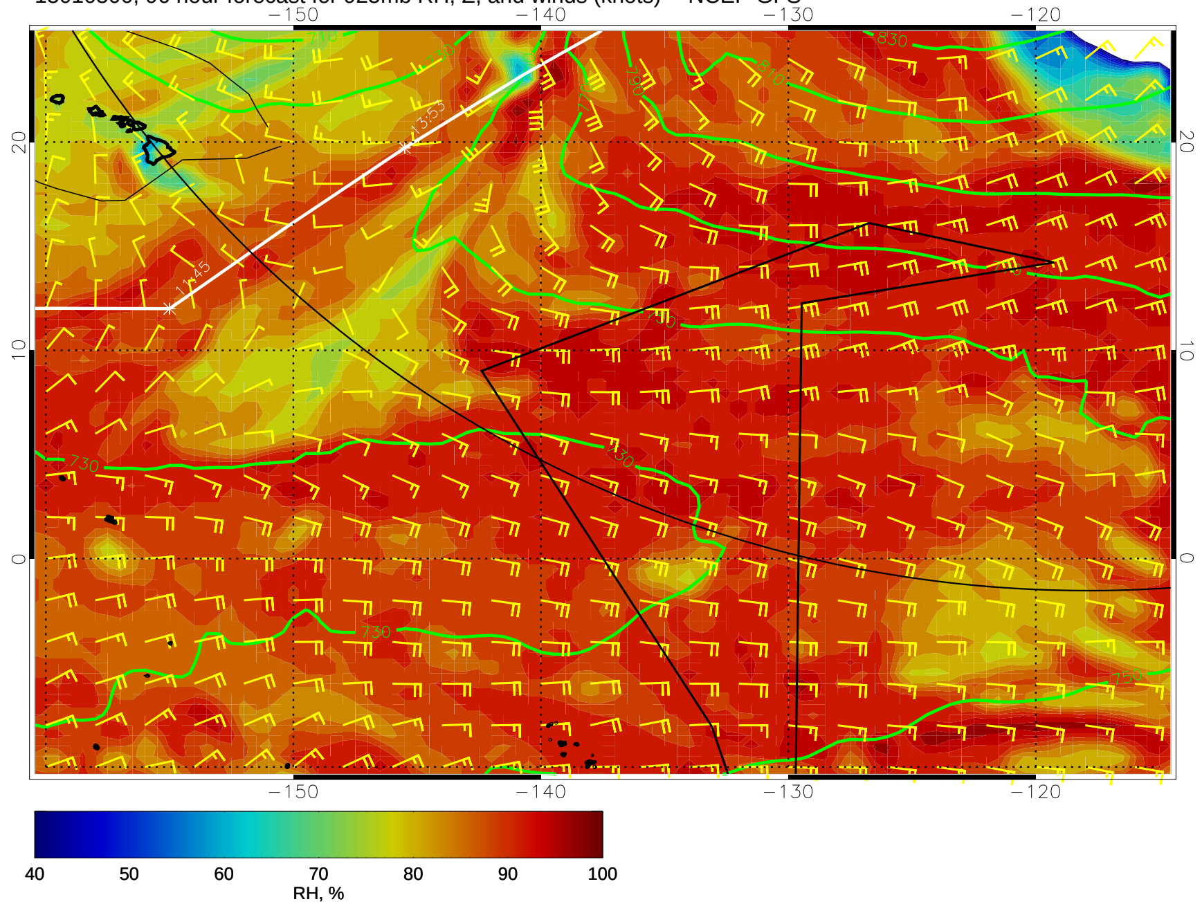
15010500, 96 hour forecast for 925mb RH, Z, and winds (knots) -- NCEP GFS
