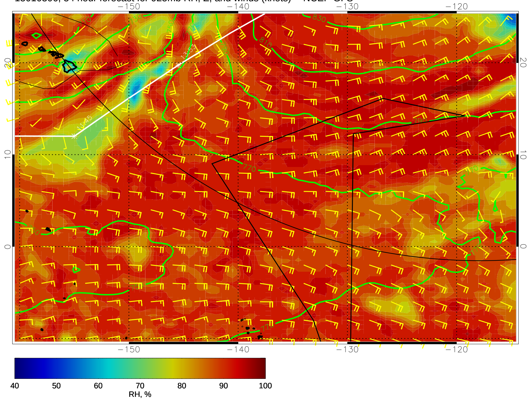
15010306, 54 hour forecast for 925mb RH, Z, and winds (knots) -- NCEP GFS
