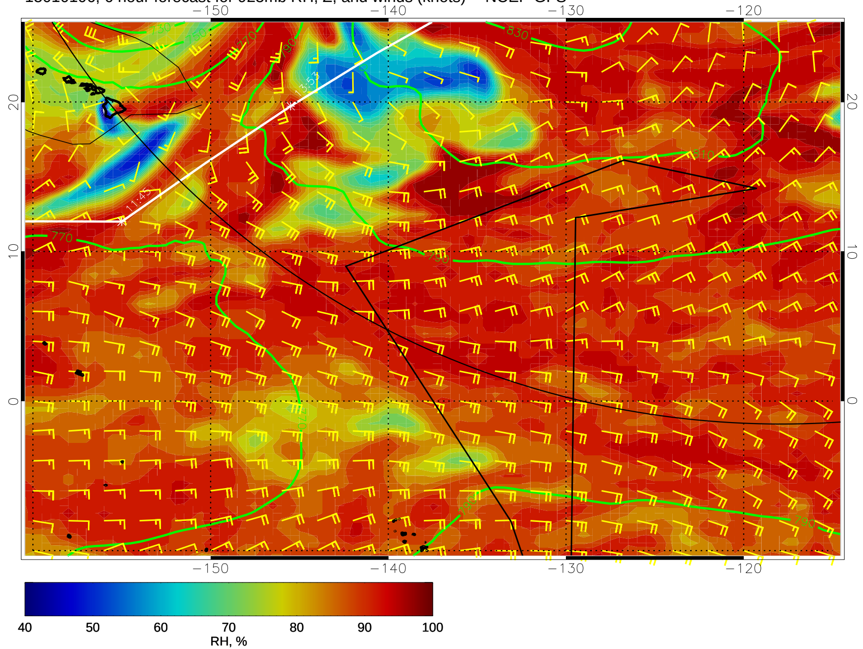
15010106, 6 hour forecast for 925mb RH, Z, and winds (knots) -- NCEP GFS
