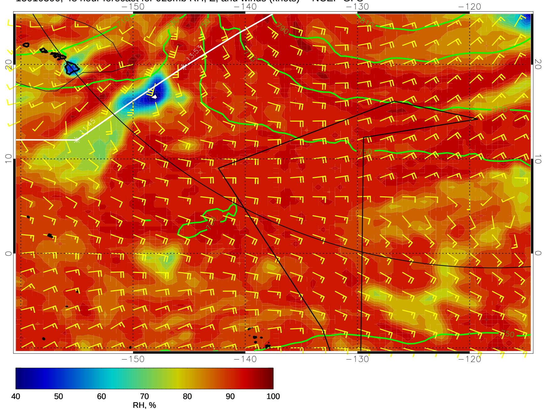
15010300, 48 hour forecast for 925mb RH, Z, and winds (knots) -- NCEP GFS
