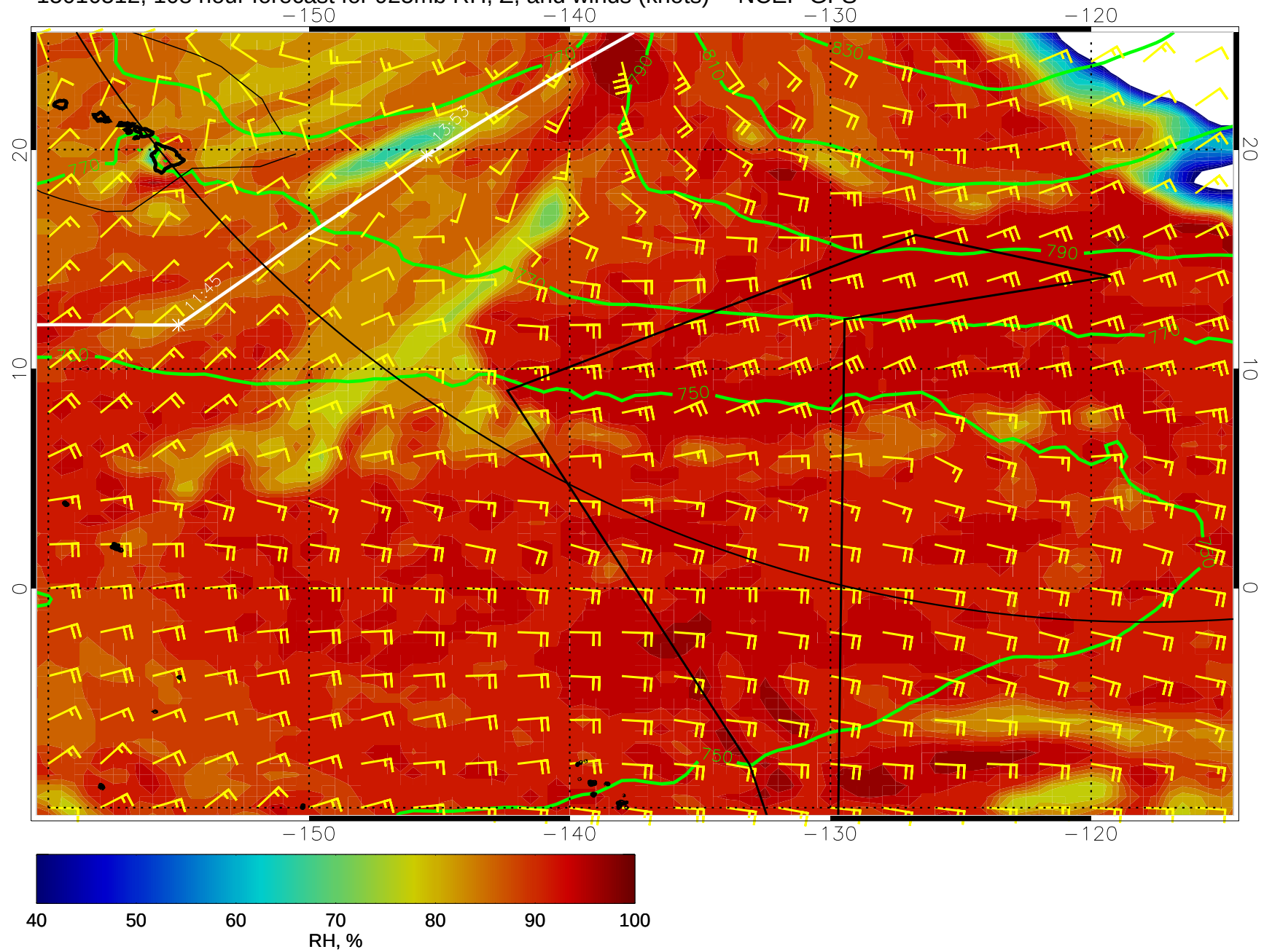
15010512, 108 hour forecast for 925mb RH, Z, and winds (knots) -- NCEP GFS
