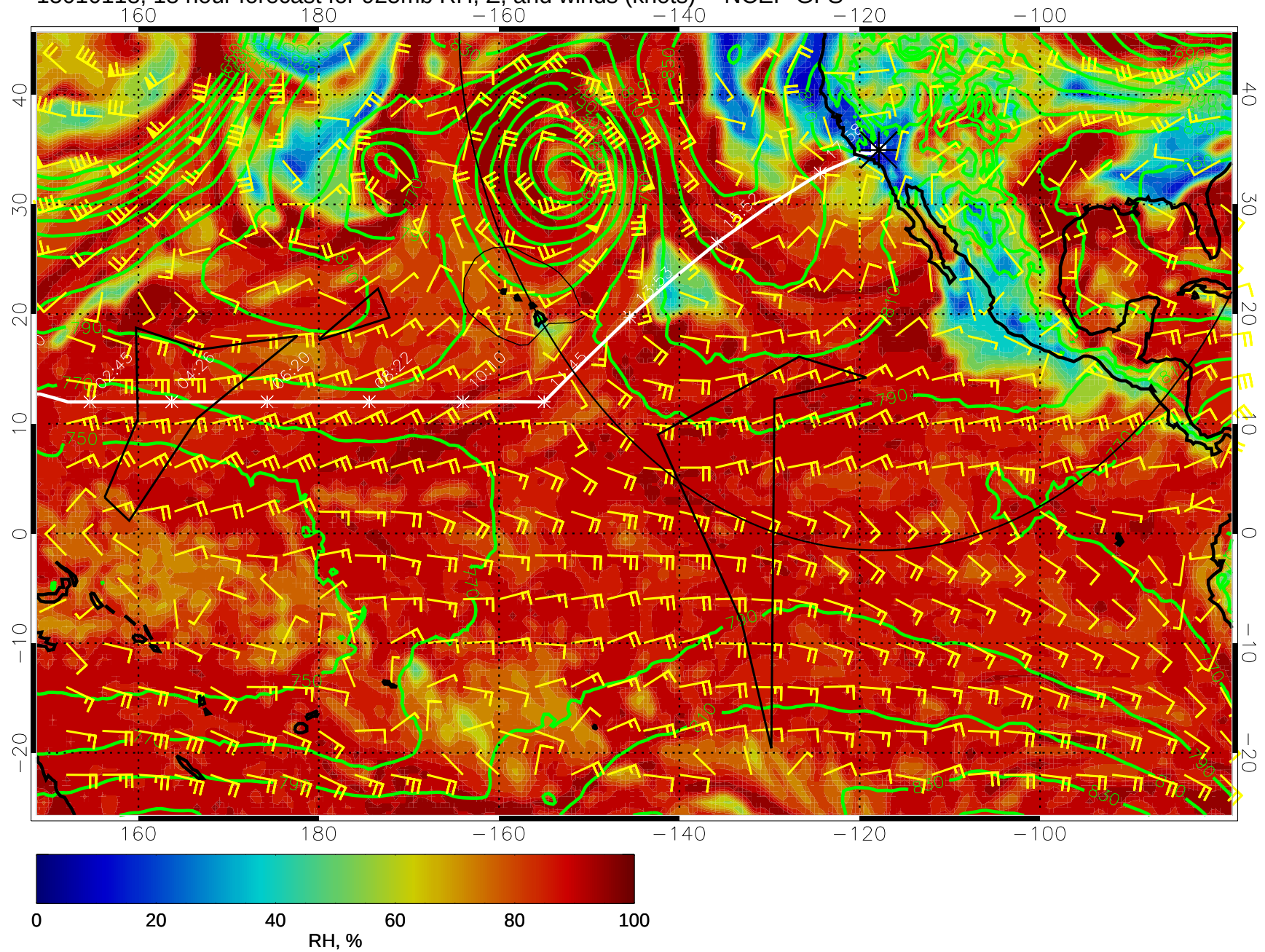
15010118, 18 hour forecast for 925mb RH, Z, and winds (knots) -- NCEP GFS
