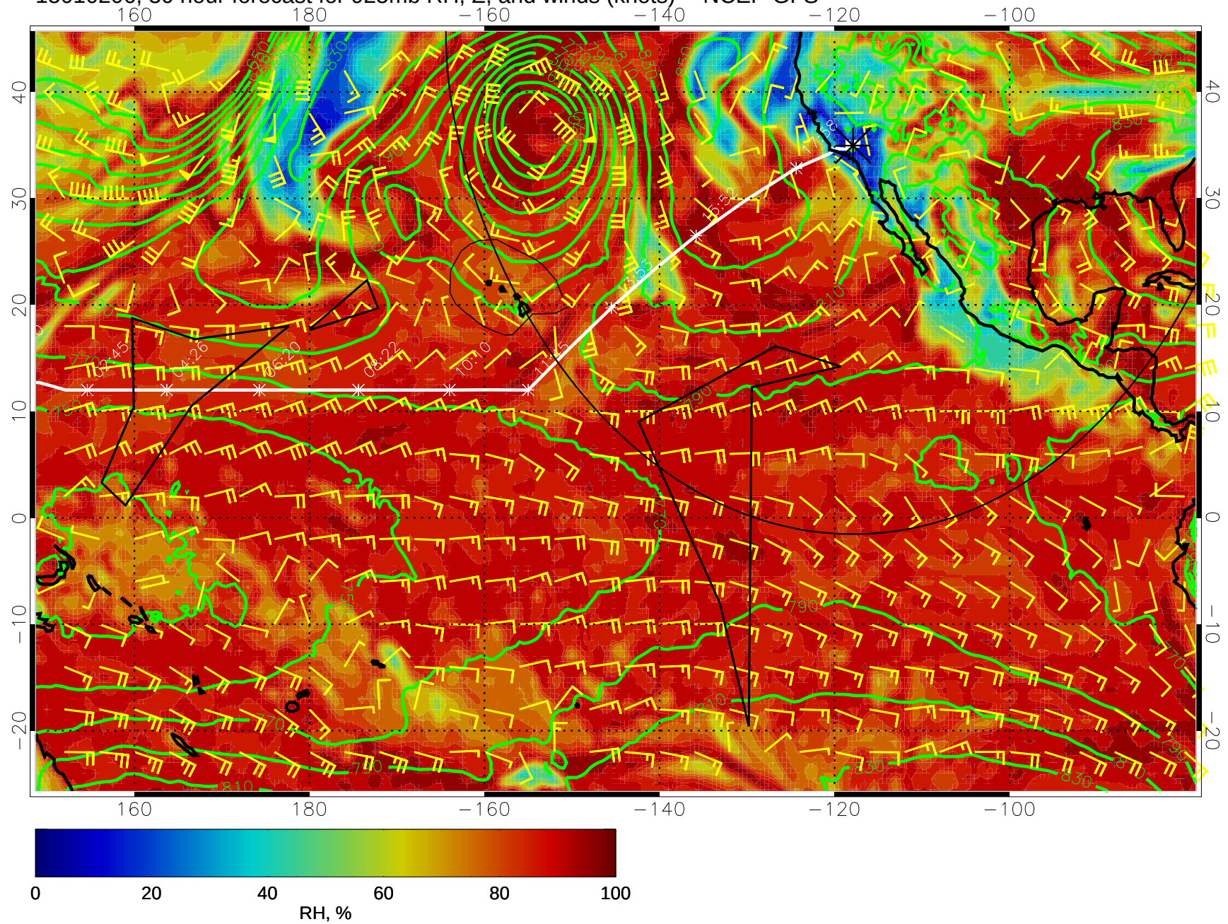
15010206, 30 hour forecast for 925mb RH, Z, and winds (knots) -- NCEP GFS
