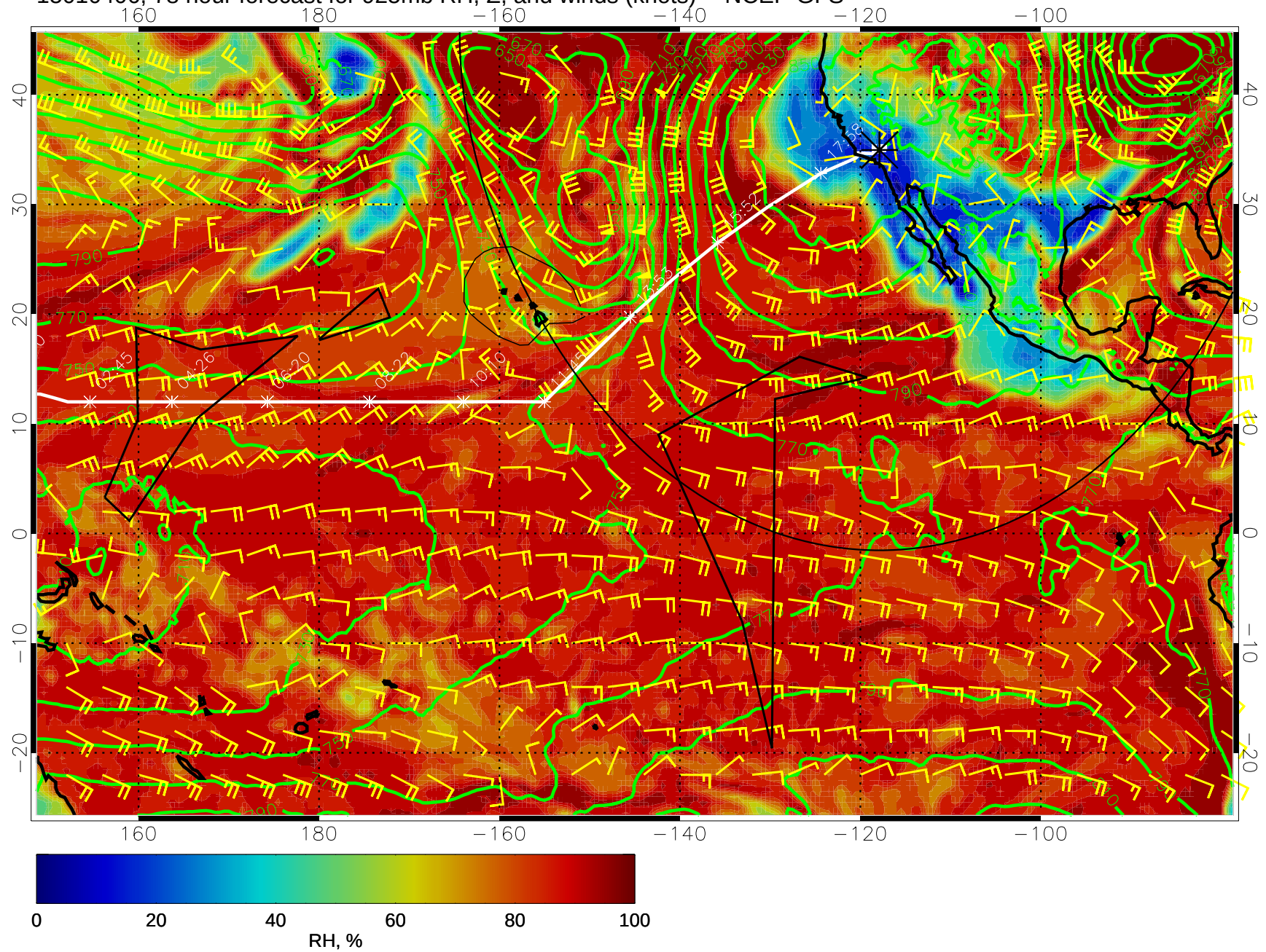
15010406, 78 hour forecast for 925mb RH, Z, and winds (knots) -- NCEP GFS
