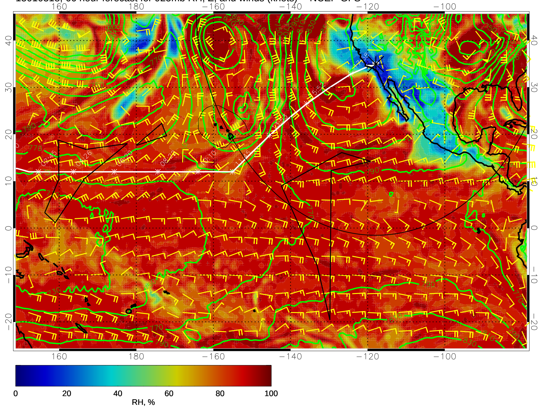
15010318, 66 hour forecast for 925mb RH, Z, and winds (knots) -- NCEP GFS
