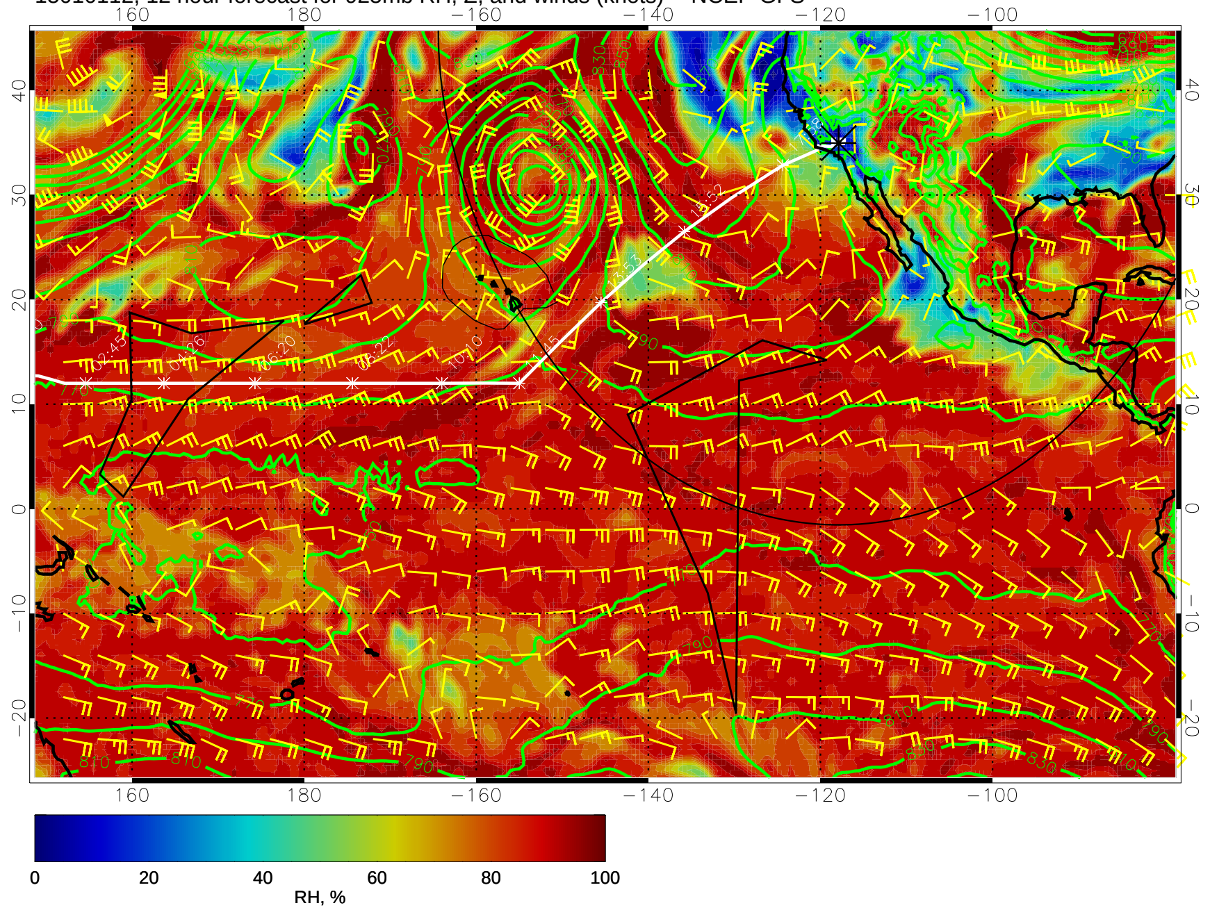
15010112, 12 hour forecast for 925mb RH, Z, and winds (knots) -- NCEP GFS
