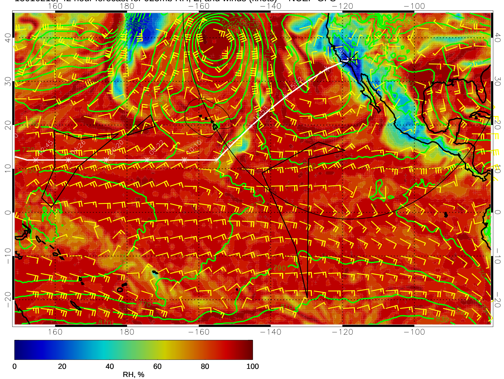
15010218, 42 hour forecast for 925mb RH, Z, and winds (knots) -- NCEP GFS
