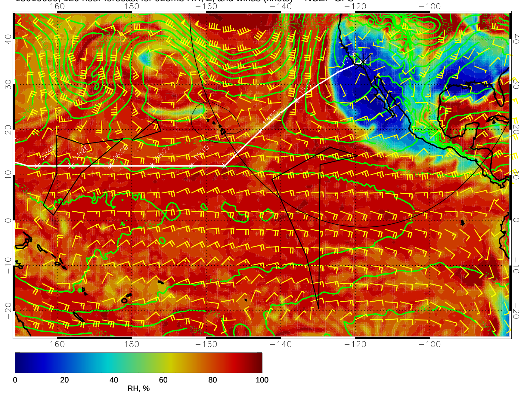
15010600, 120 hour forecast for 925mb RH, Z, and winds (knots) -- NCEP GFS
