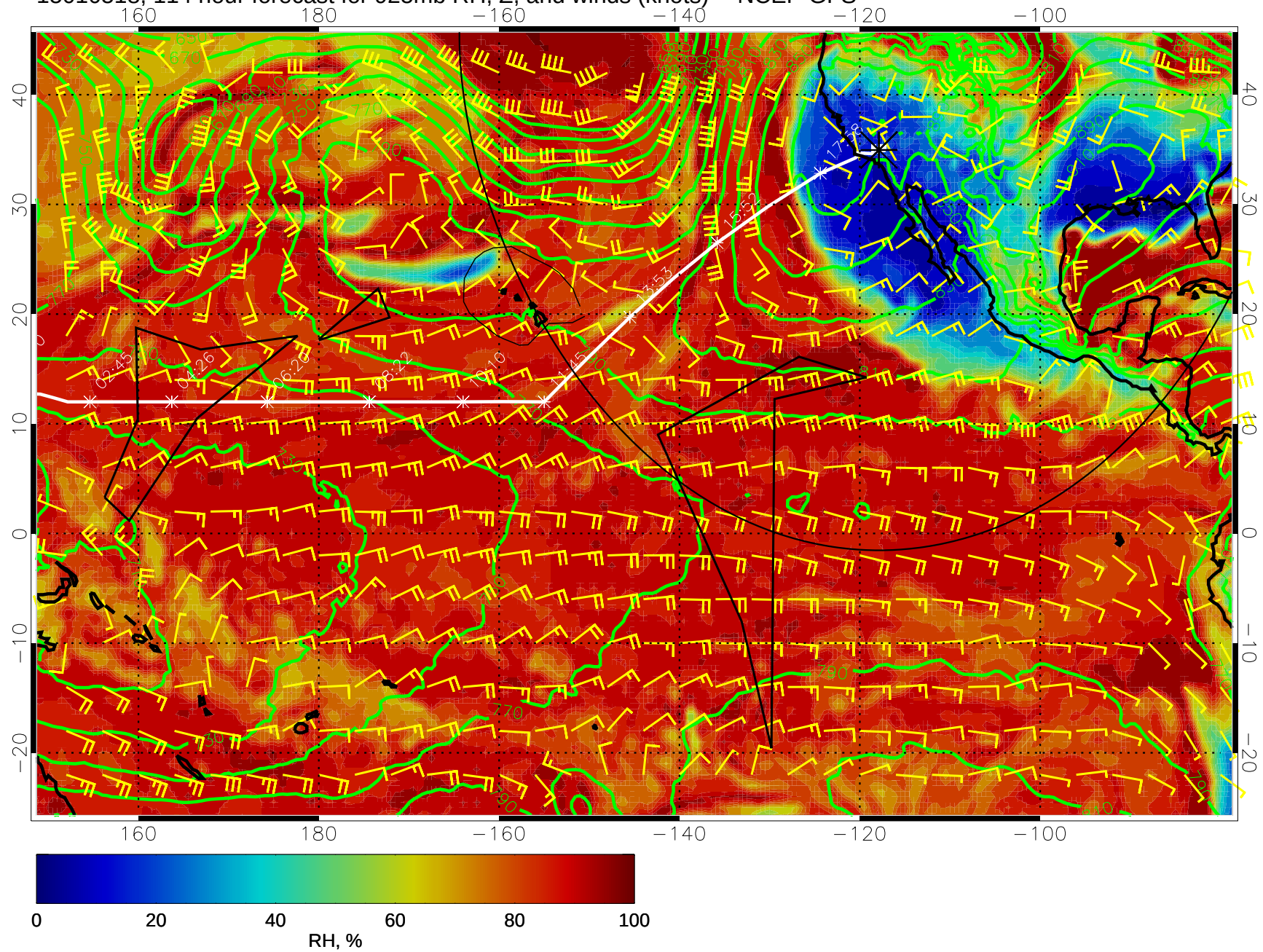
15010518, 114 hour forecast for 925mb RH, Z, and winds (knots) -- NCEP GFS
