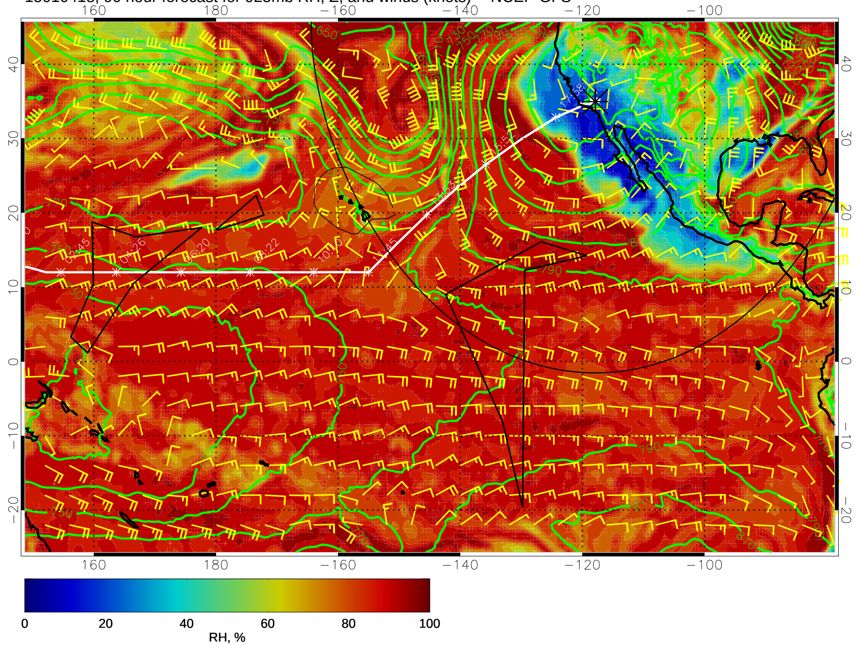
15010418, 90 hour forecast for 925mb RH, Z, and winds (knots) -- NCEP GFS
