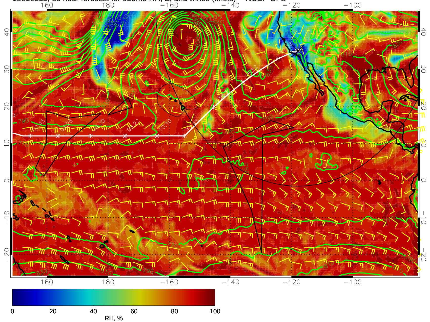
15010212, 36 hour forecast for 925mb RH, Z, and winds (knots) -- NCEP GFS
