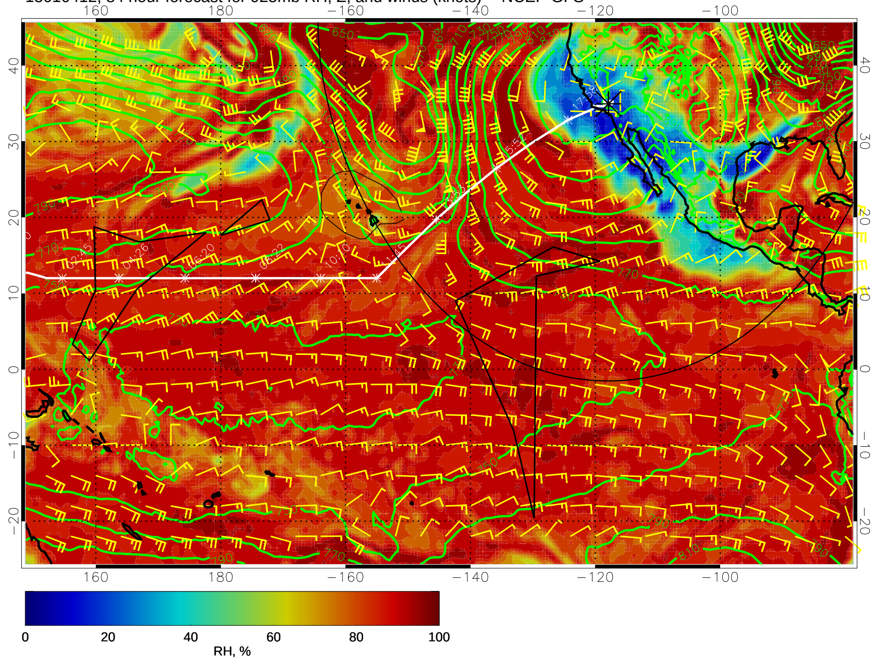
15010412, 84 hour forecast for 925mb RH, Z, and winds (knots) -- NCEP GFS
