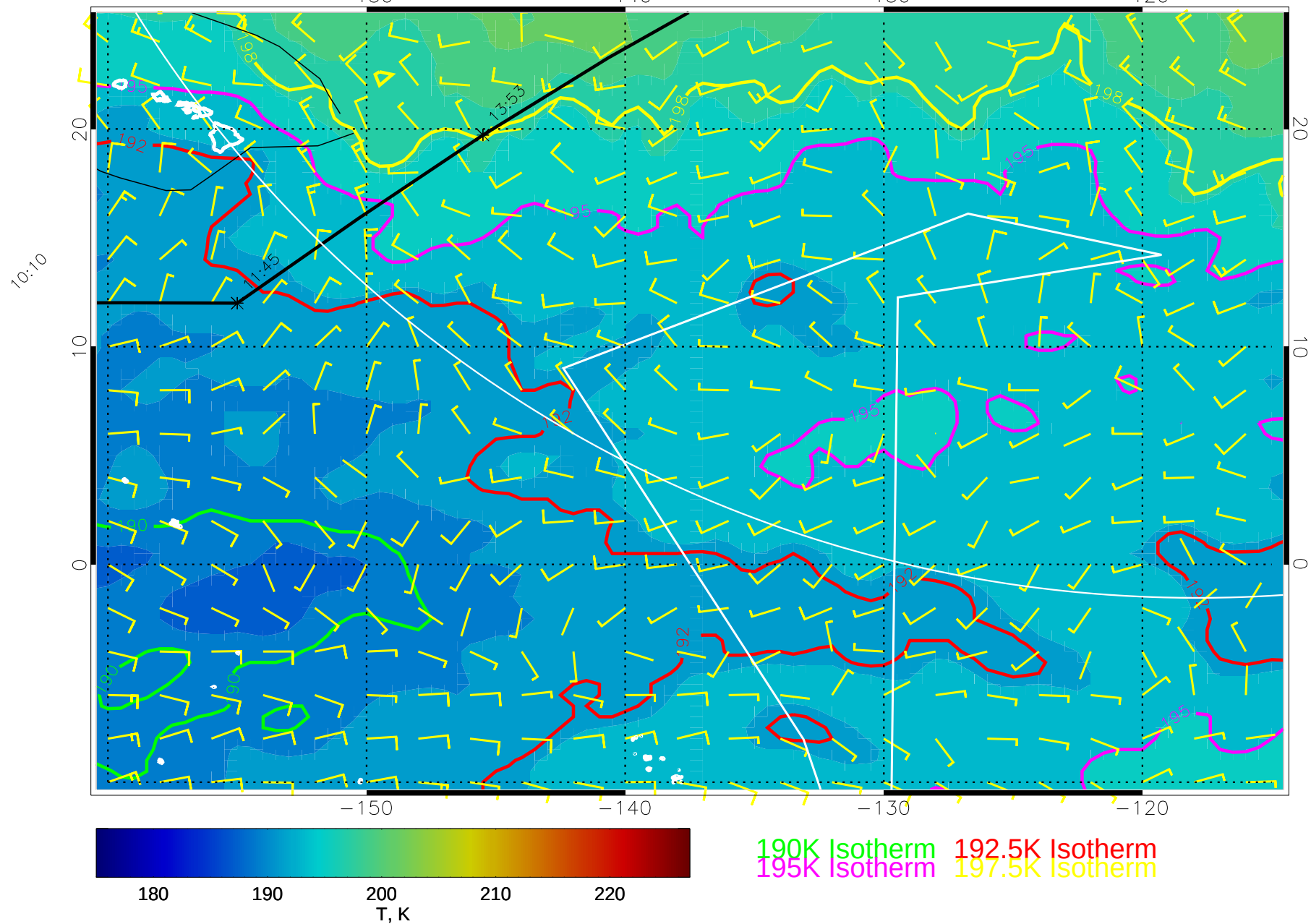
15010512, 108 hour forecast for 70mb T and winds (knots) -- NCEP GFS
