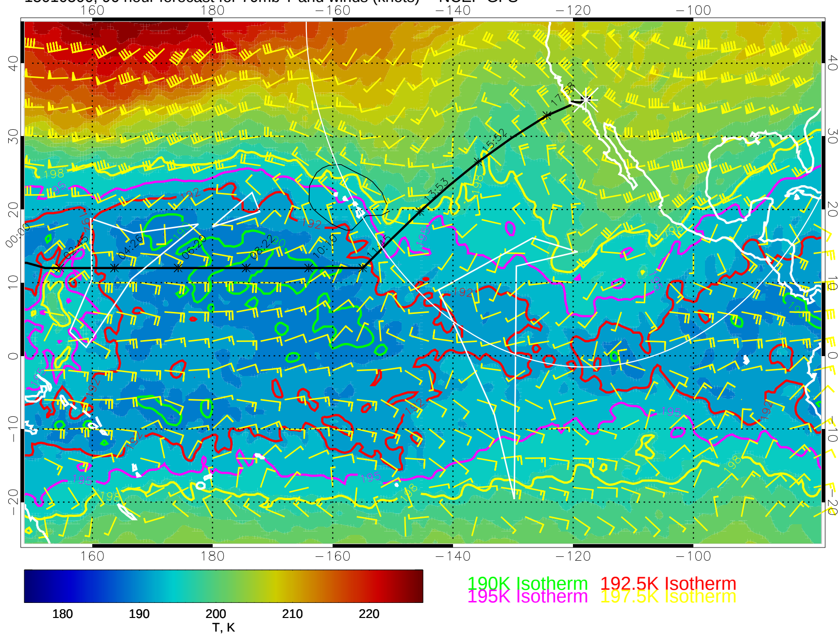
15010500, 96 hour forecast for 70mb T and winds (knots) -- NCEP GFS
