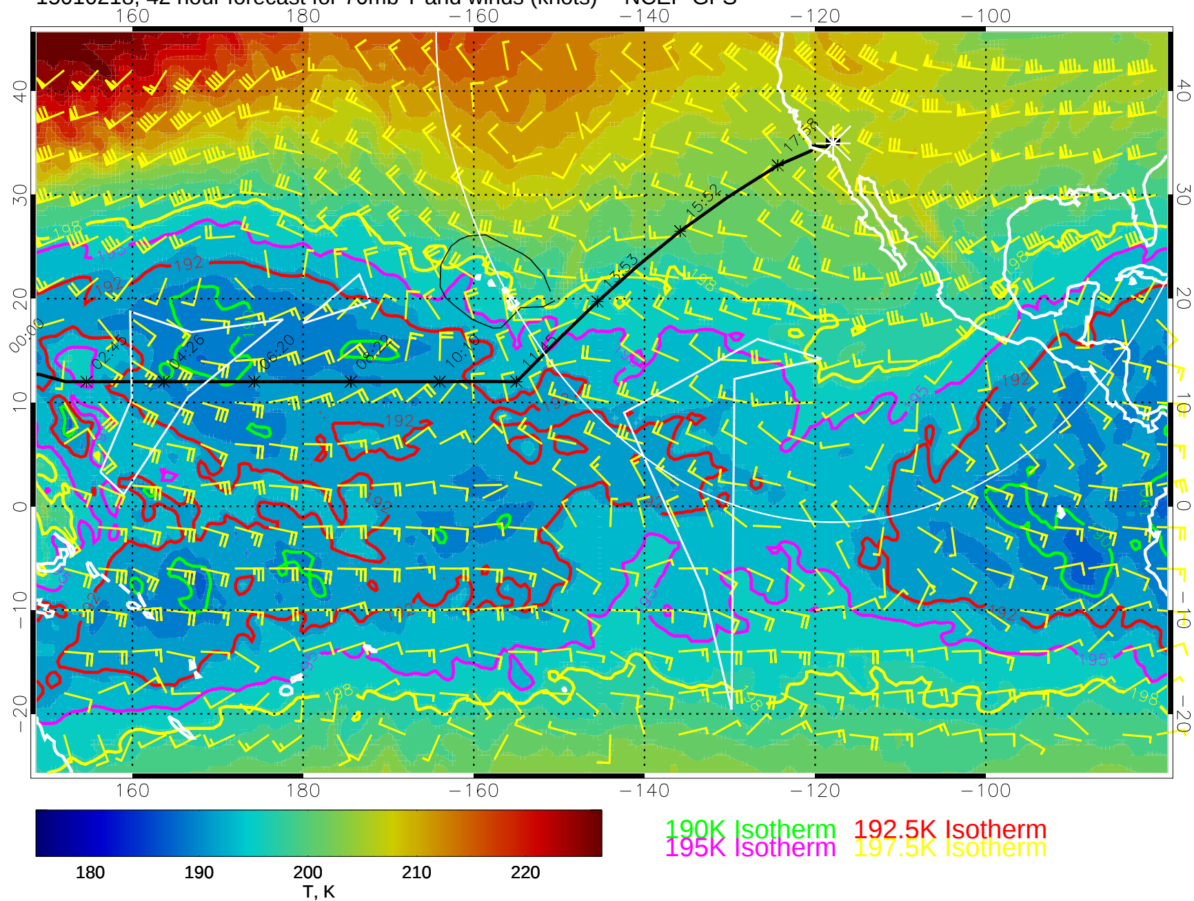
15010218, 42 hour forecast for 70mb T and winds (knots) -- NCEP GFS
