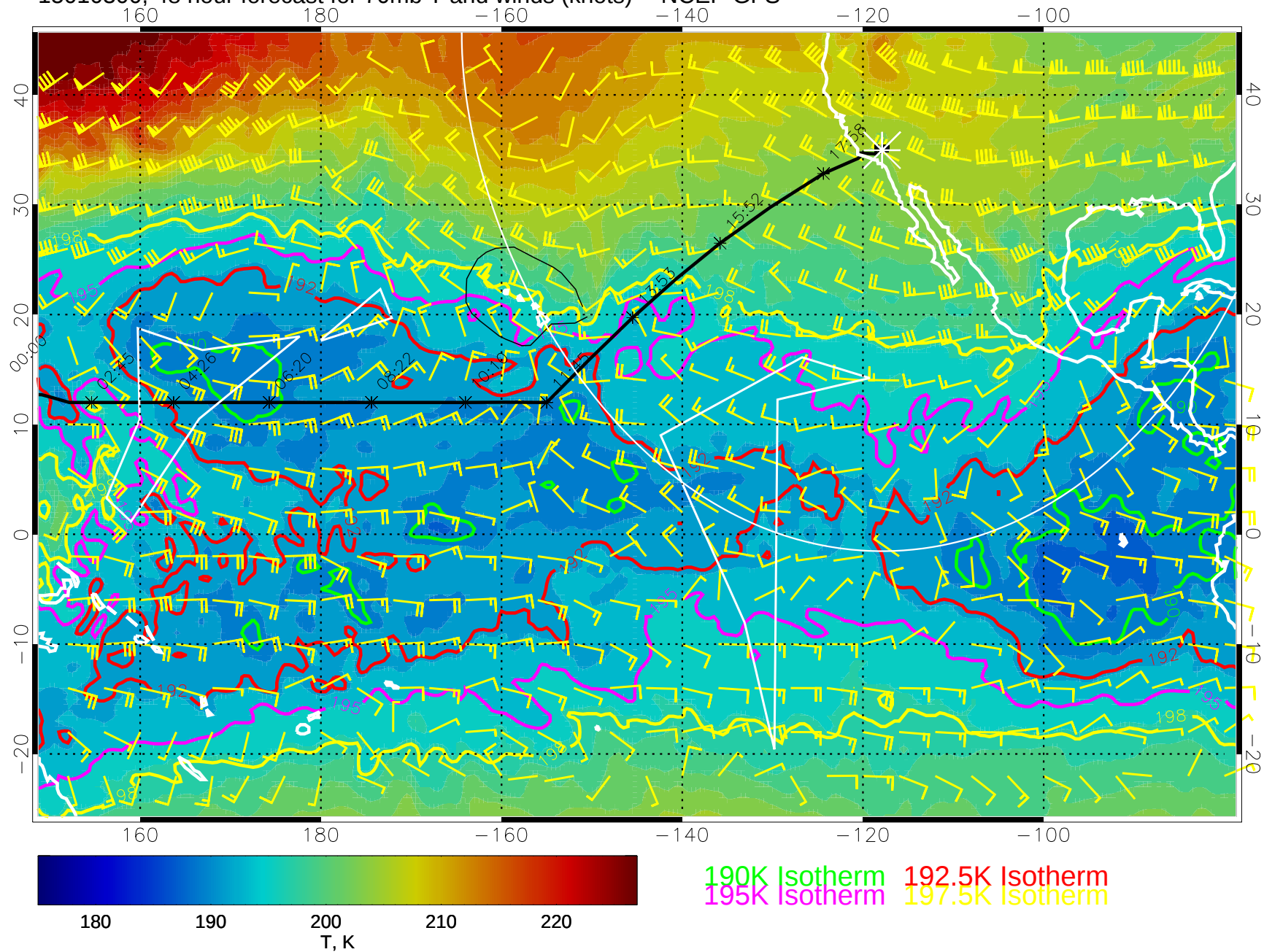
15010300, 48 hour forecast for 70mb T and winds (knots) -- NCEP GFS
