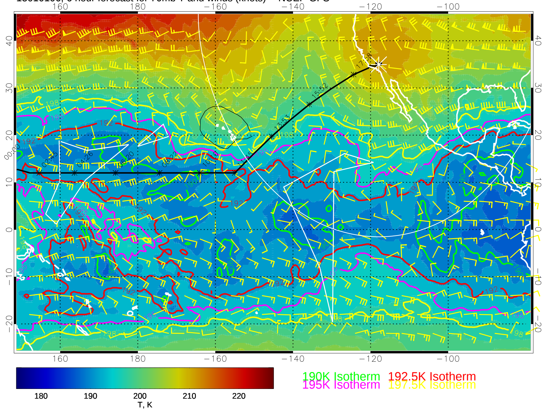
15010106, 6 hour forecast for 70mb T and winds (knots) -- NCEP GFS
