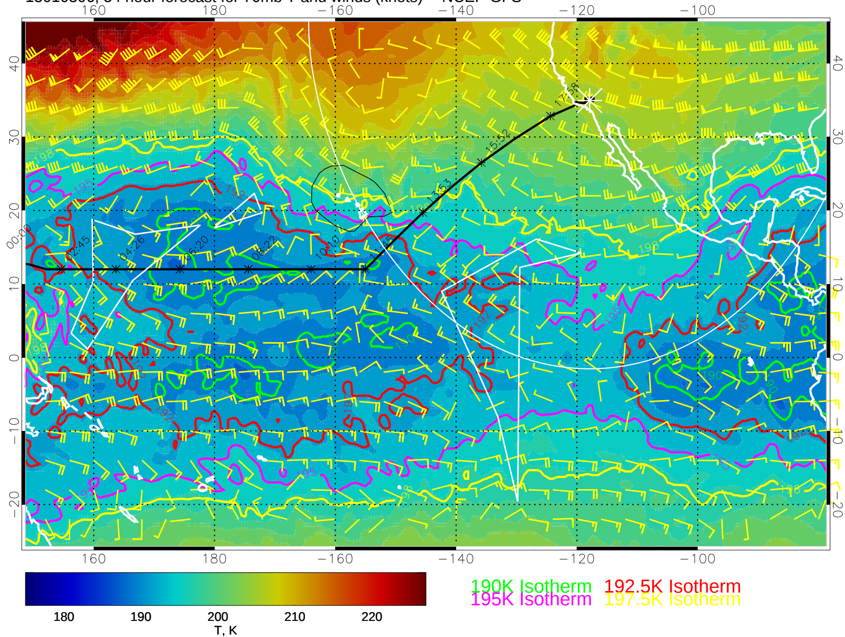
15010306, 54 hour forecast for 70mb T and winds (knots) -- NCEP GFS
