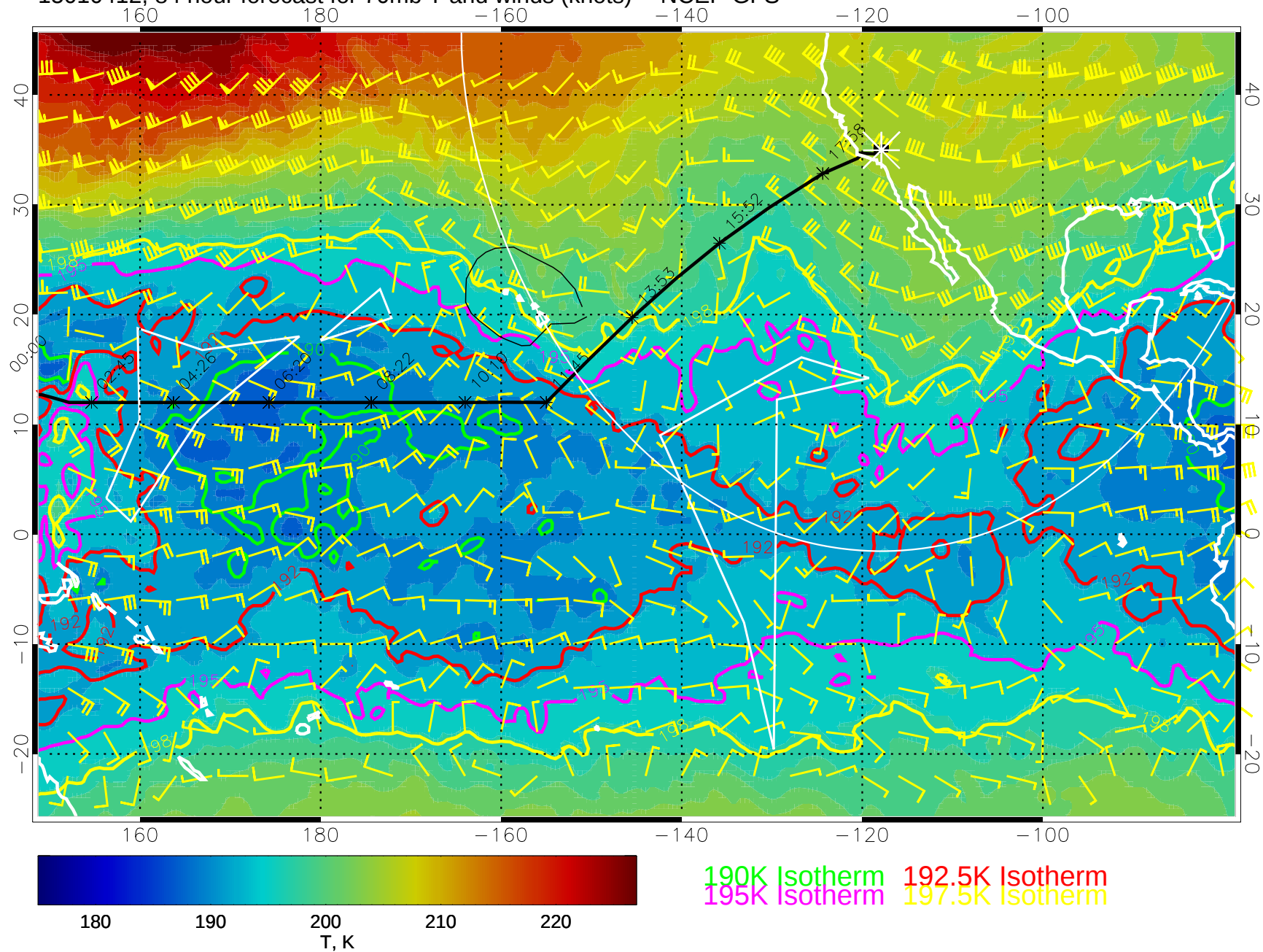
15010412, 84 hour forecast for 70mb T and winds (knots) -- NCEP GFS
