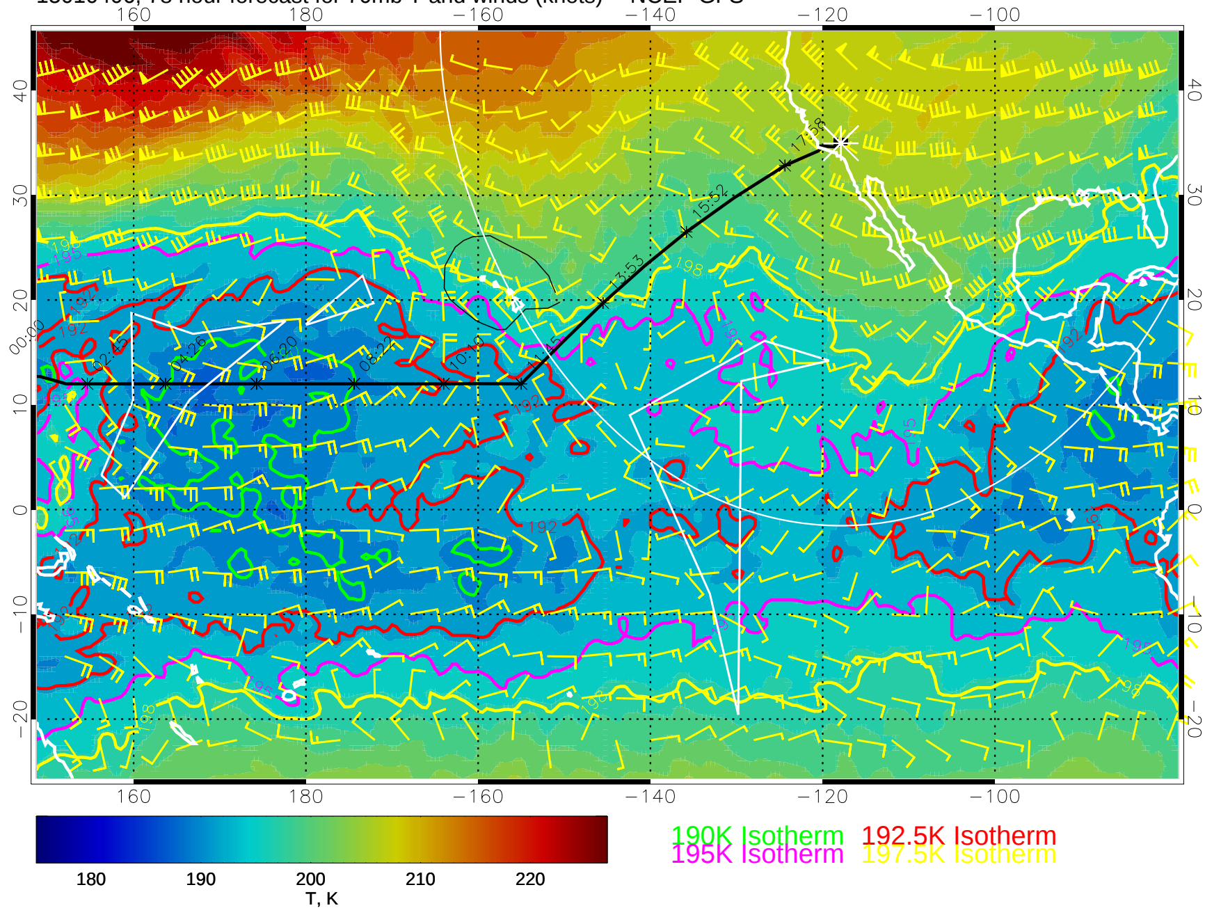
15010406, 78 hour forecast for 70mb T and winds (knots) -- NCEP GFS
