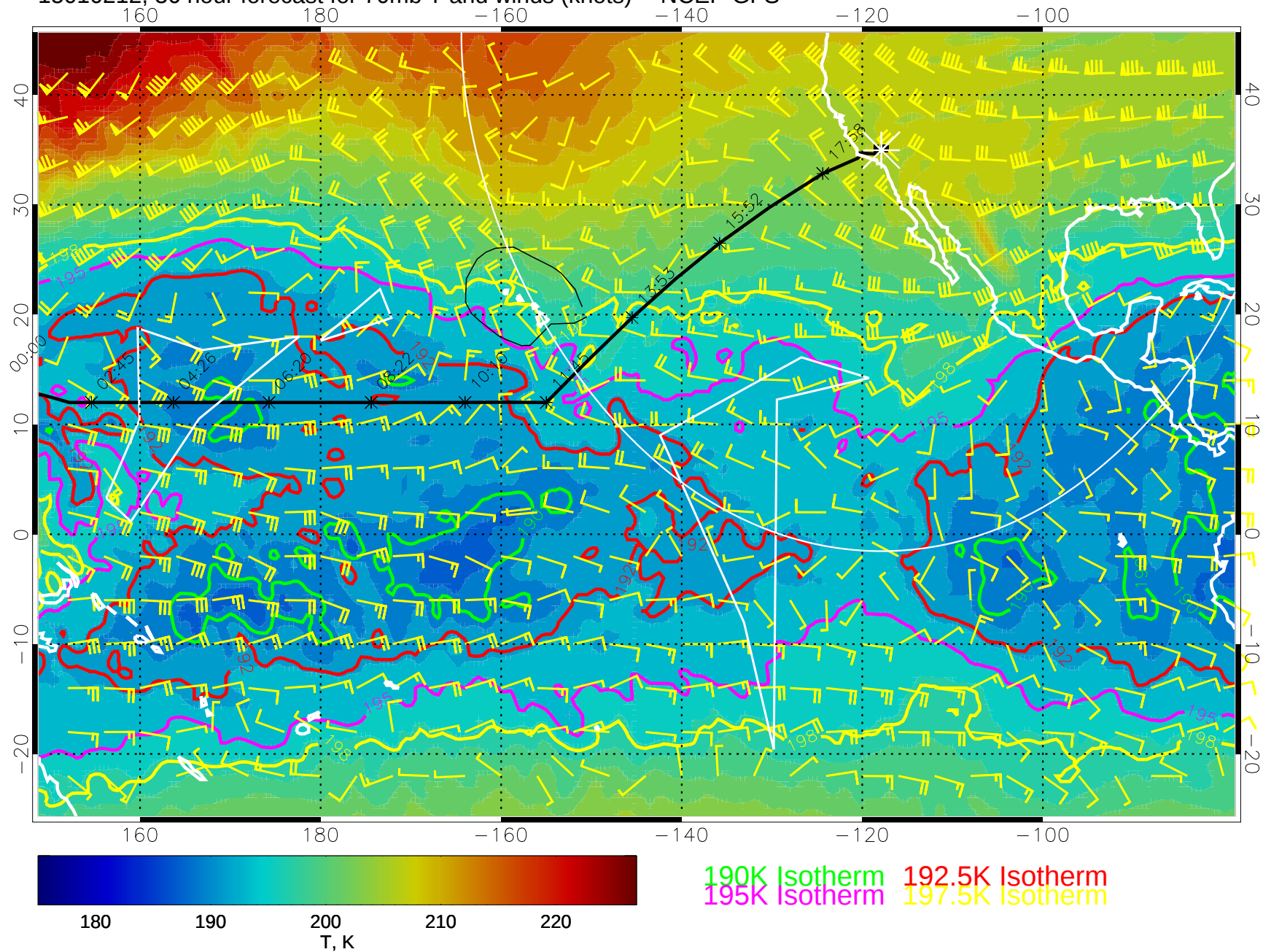
15010212, 36 hour forecast for 70mb T and winds (knots) -- NCEP GFS
