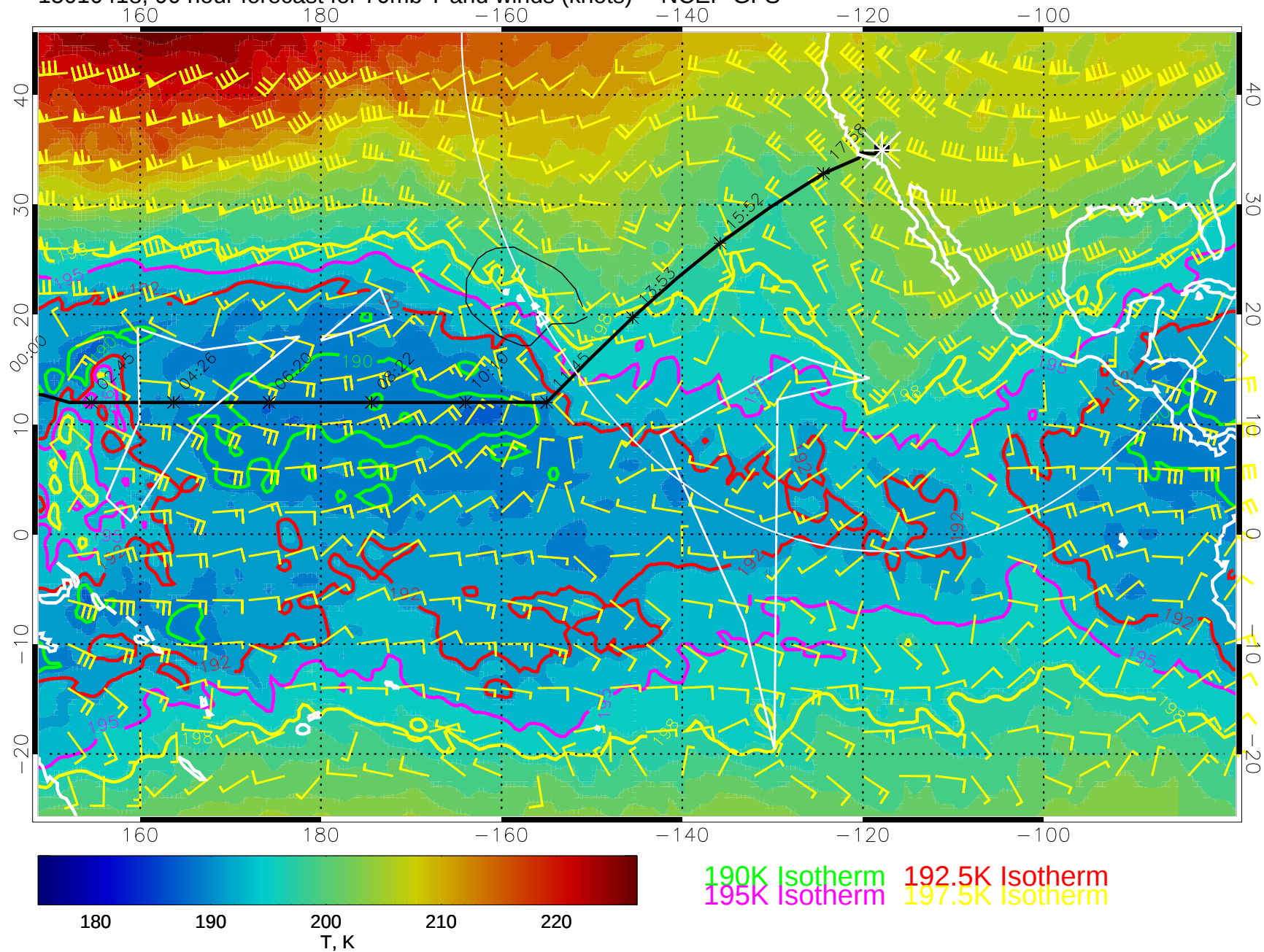
15010418, 90 hour forecast for 70mb T and winds (knots) -- NCEP GFS
