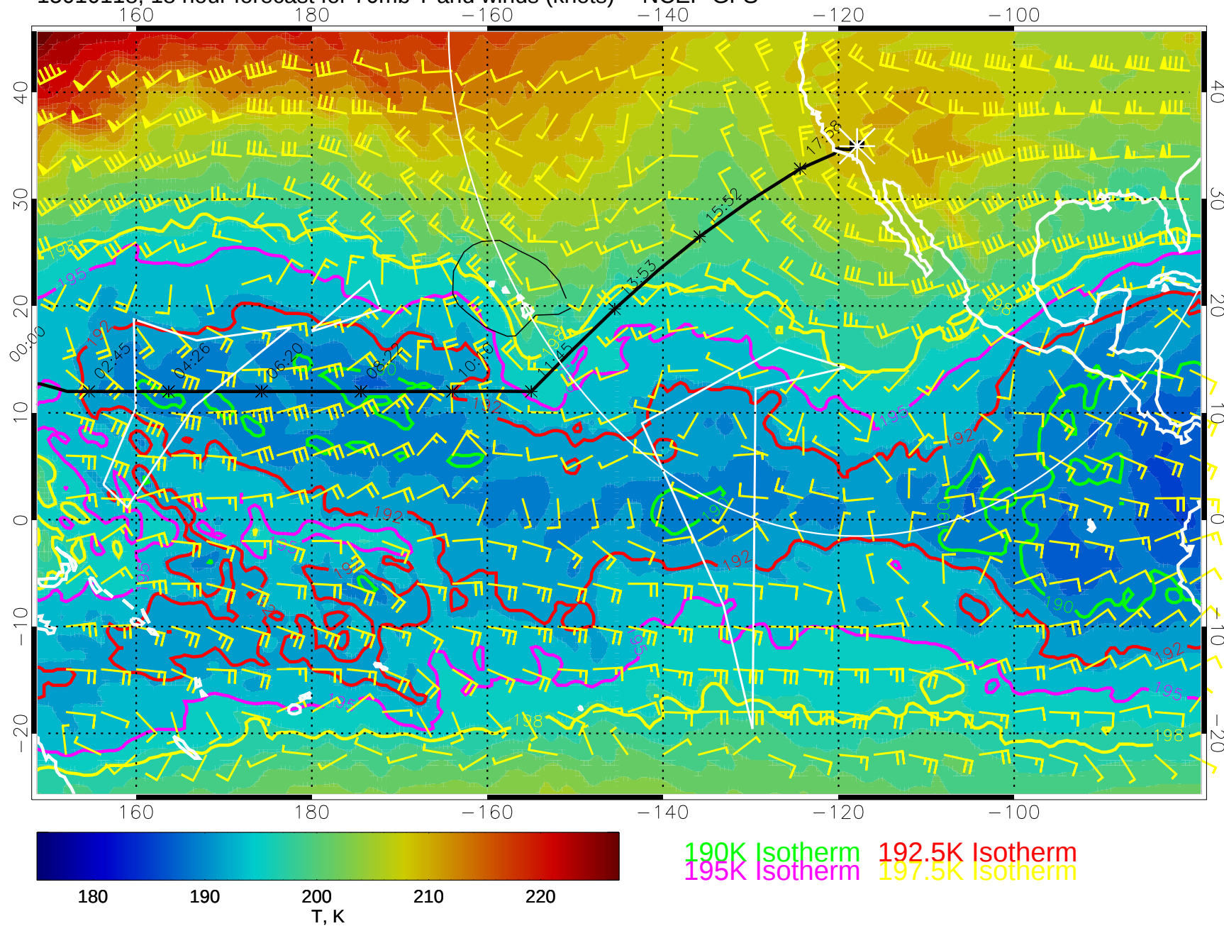
15010118, 18 hour forecast for 70mb T and winds (knots) -- NCEP GFS
