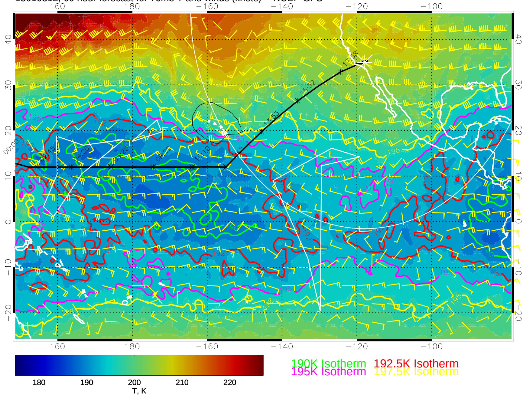
15010312, 60 hour forecast for 70mb T and winds (knots) -- NCEP GFS
