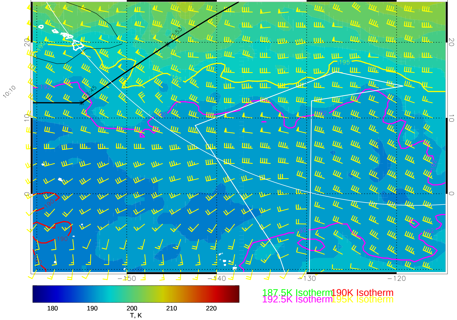
15010218, 42 hour forecast for 100mb T and winds (knots) -- NCEP GFS
