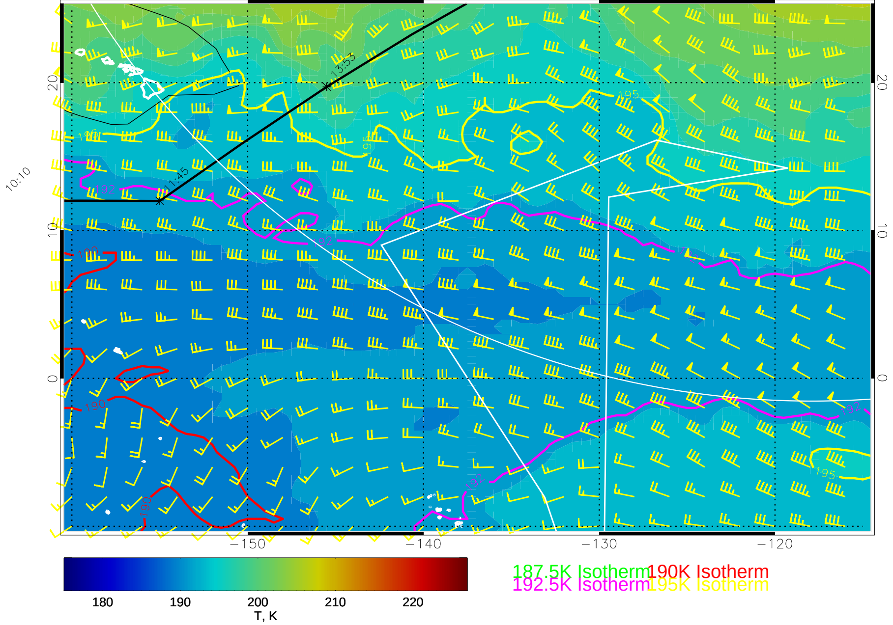
15010312, 60 hour forecast for 100mb T and winds (knots) -- NCEP GFS
