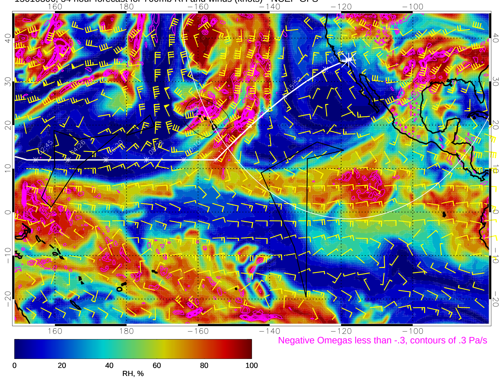
15010306, 54 hour forecast for 700mb RH and winds (knots) - NCEP GFS
