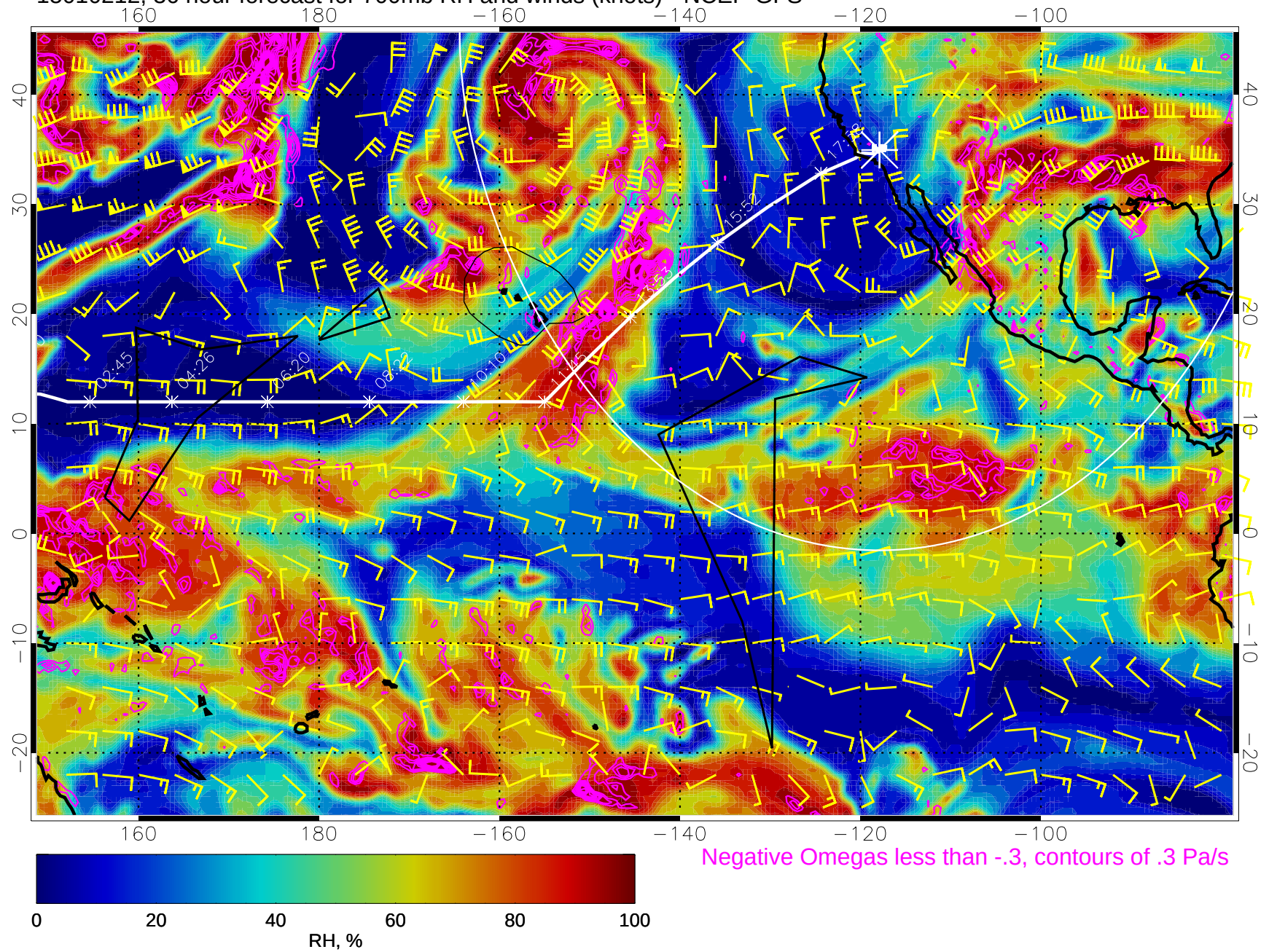
15010212, 36 hour forecast for 700mb RH and winds (knots) - NCEP GFS
