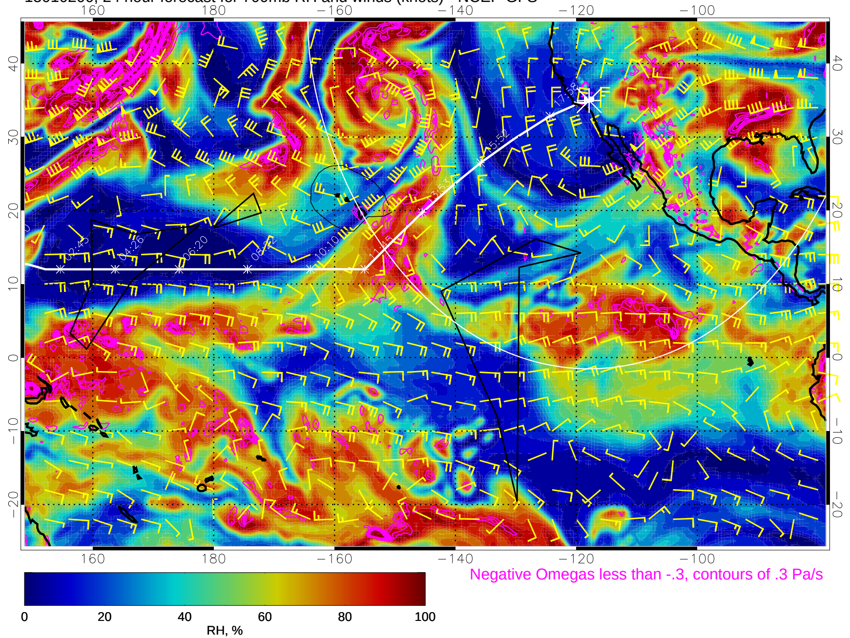
15010200, 24 hour forecast for 700mb RH and winds (knots) - NCEP GFS
