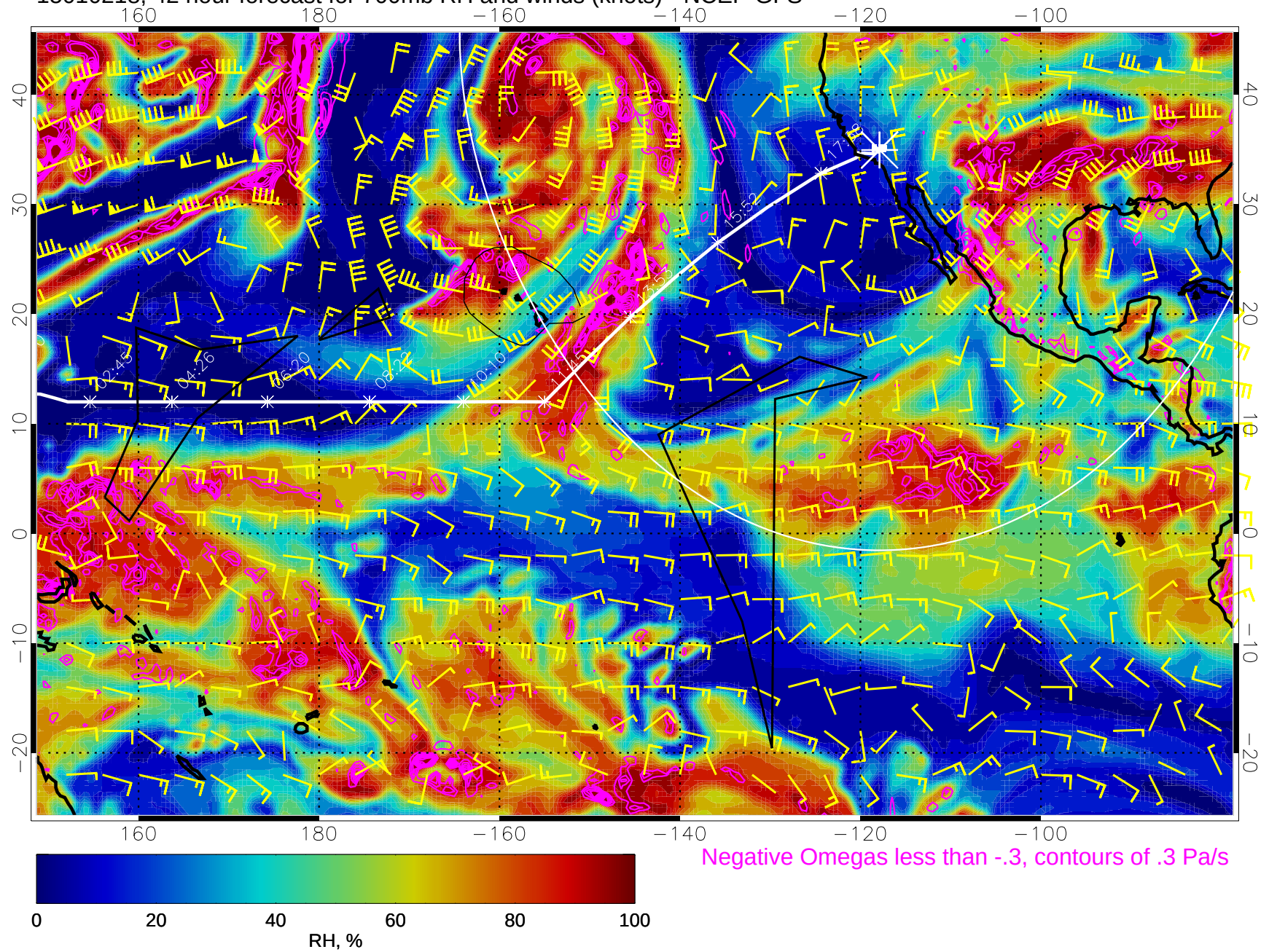
15010218, 42 hour forecast for 700mb RH and winds (knots) - NCEP GFS
