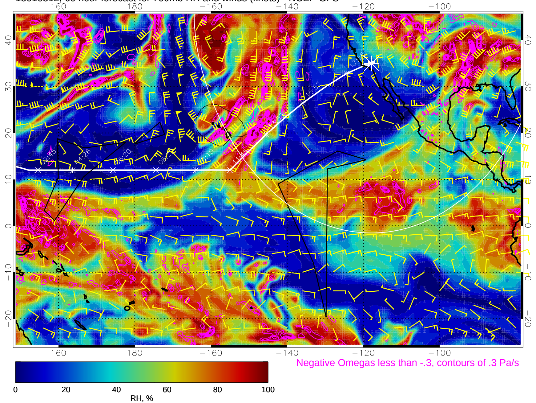
15010312, 60 hour forecast for 700mb RH and winds (knots) - NCEP GFS
