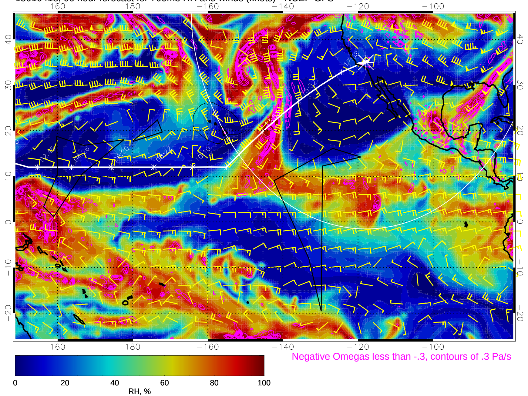
15010418, 90 hour forecast for 700mb RH and winds (knots) - NCEP GFS
