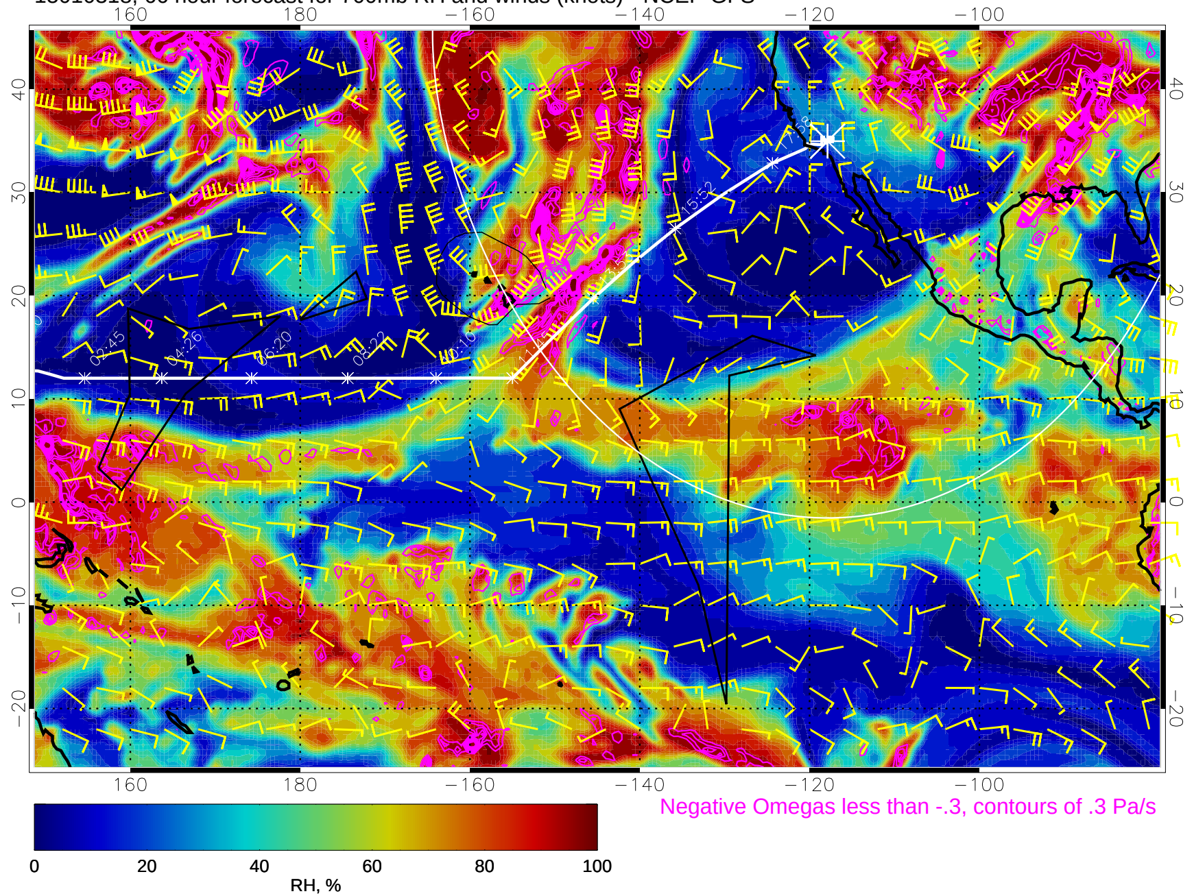
15010318, 66 hour forecast for 700mb RH and winds (knots) - NCEP GFS
