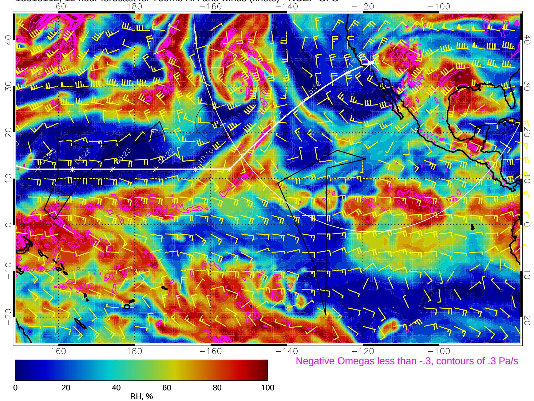
15010112, 12 hour forecast for 700mb RH and winds (knots) - NCEP GFS
