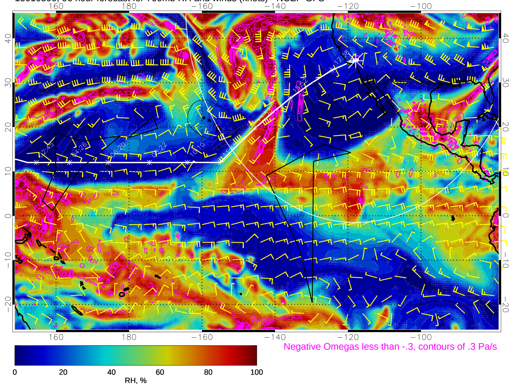
15010500, 96 hour forecast for 700mb RH and winds (knots) - NCEP GFS
