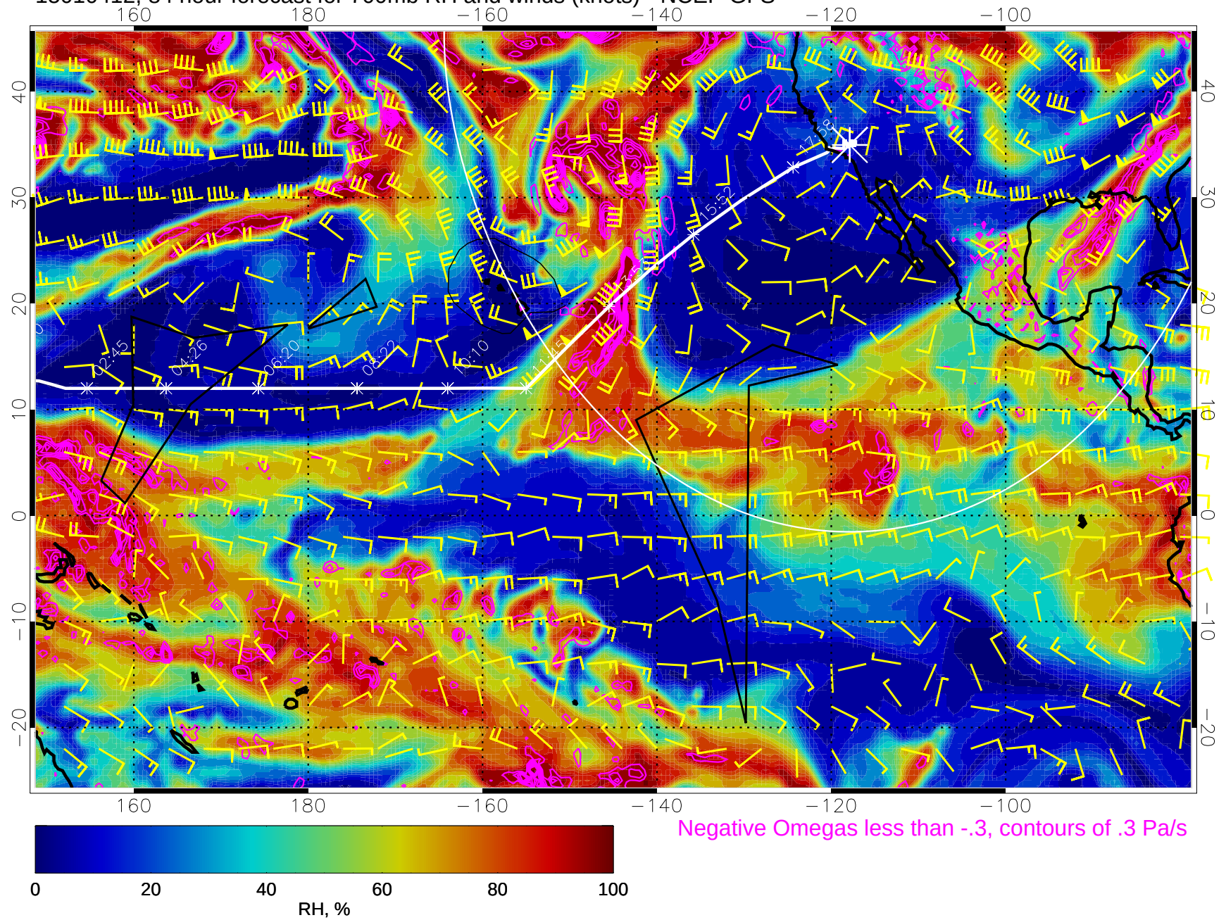
15010412, 84 hour forecast for 700mb RH and winds (knots) - NCEP GFS
