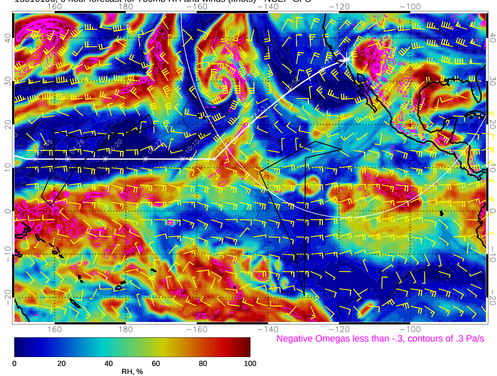
15010106, 6 hour forecast for 700mb RH and winds (knots) - NCEP GFS
