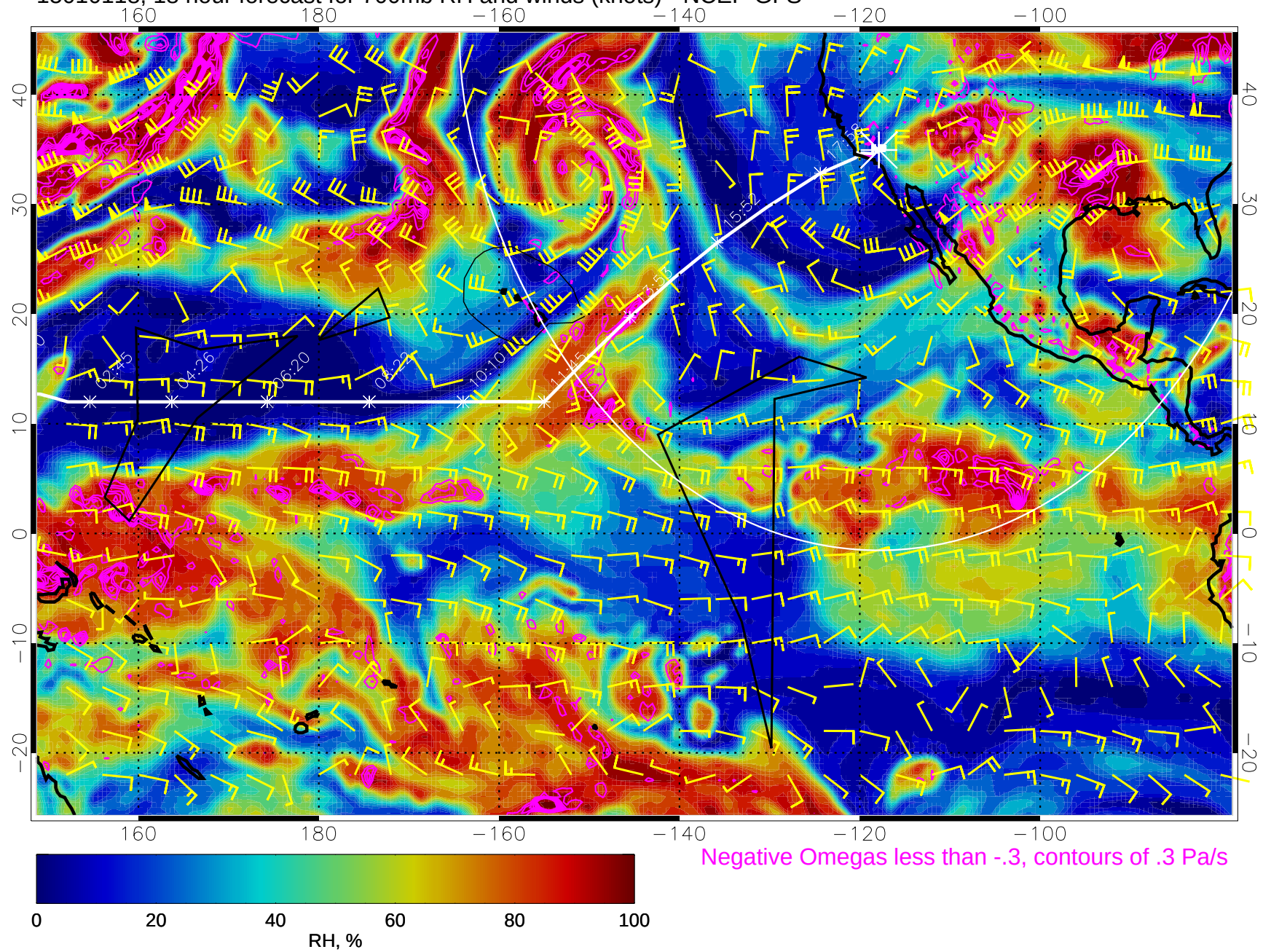
15010118, 18 hour forecast for 700mb RH and winds (knots) - NCEP GFS
