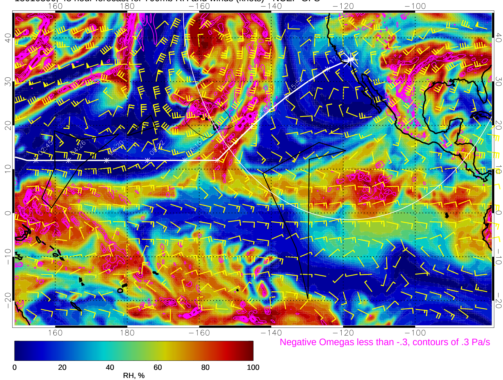
15010300, 48 hour forecast for 700mb RH and winds (knots) - NCEP GFS
