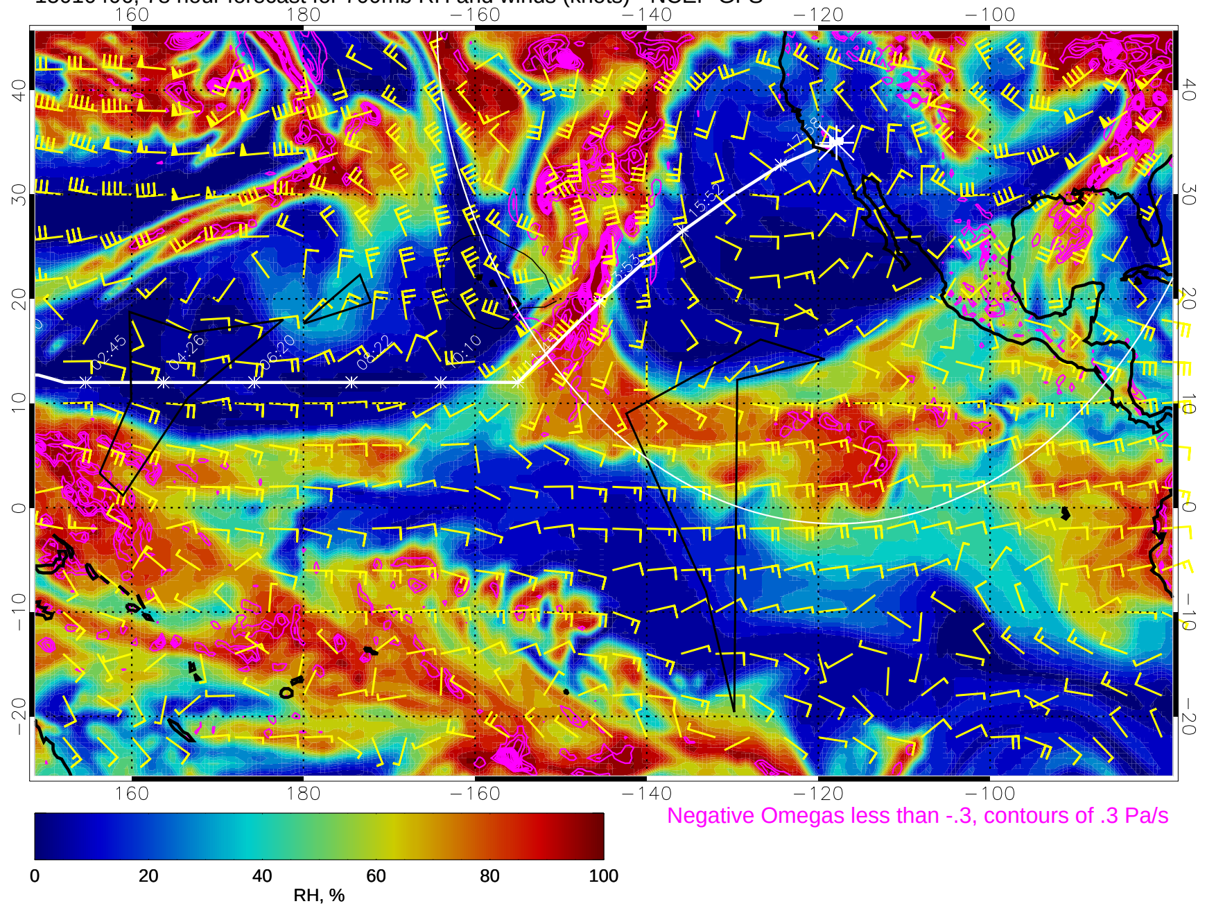
15010406, 78 hour forecast for 700mb RH and winds (knots) - NCEP GFS
