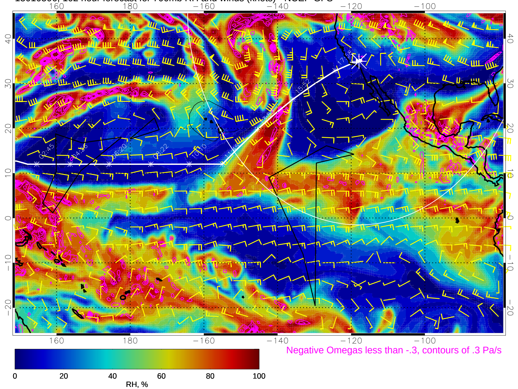
15010506, 102 hour forecast for 700mb RH and winds (knots) - NCEP GFS
