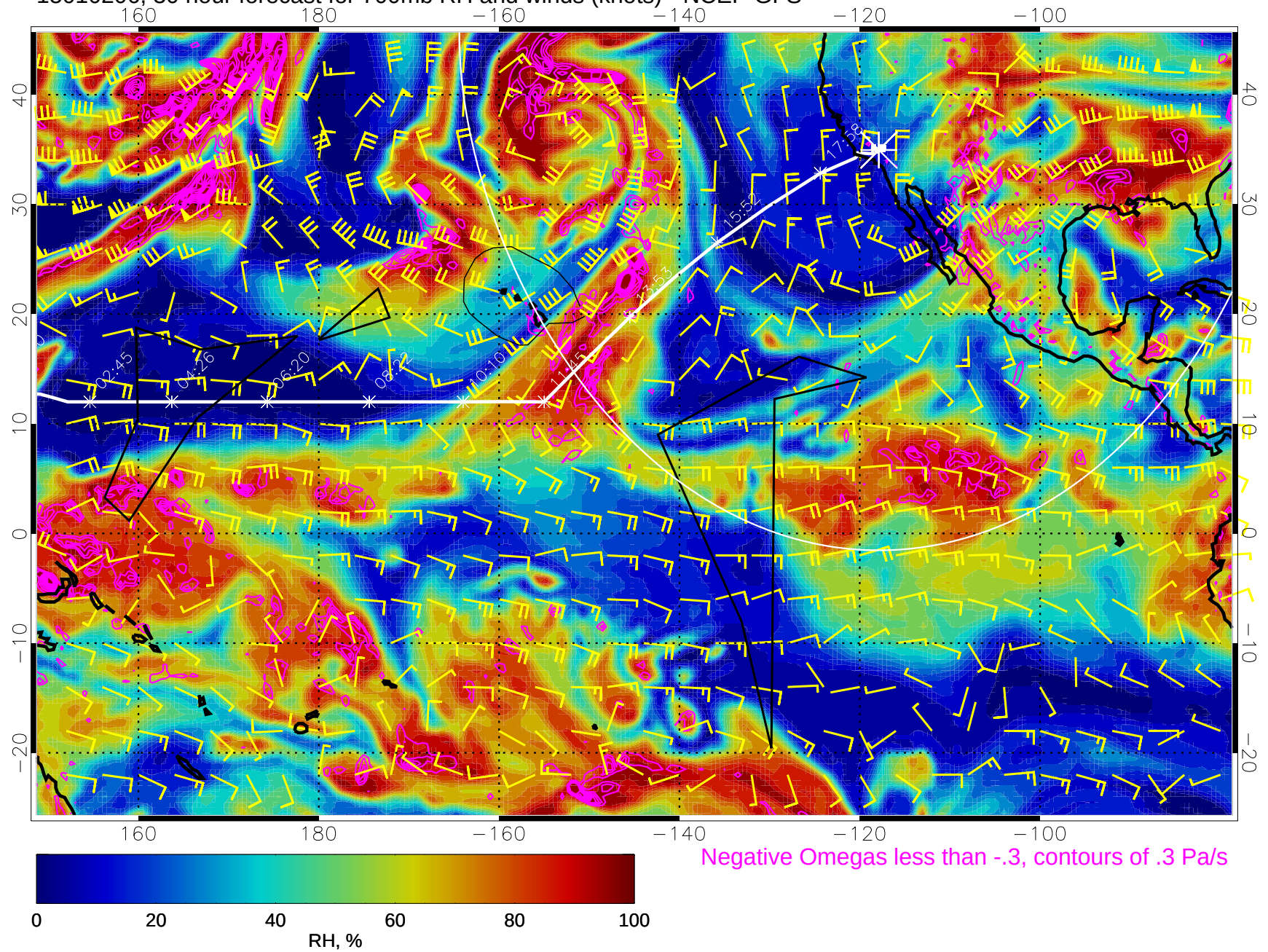
15010206, 30 hour forecast for 700mb RH and winds (knots) - NCEP GFS
