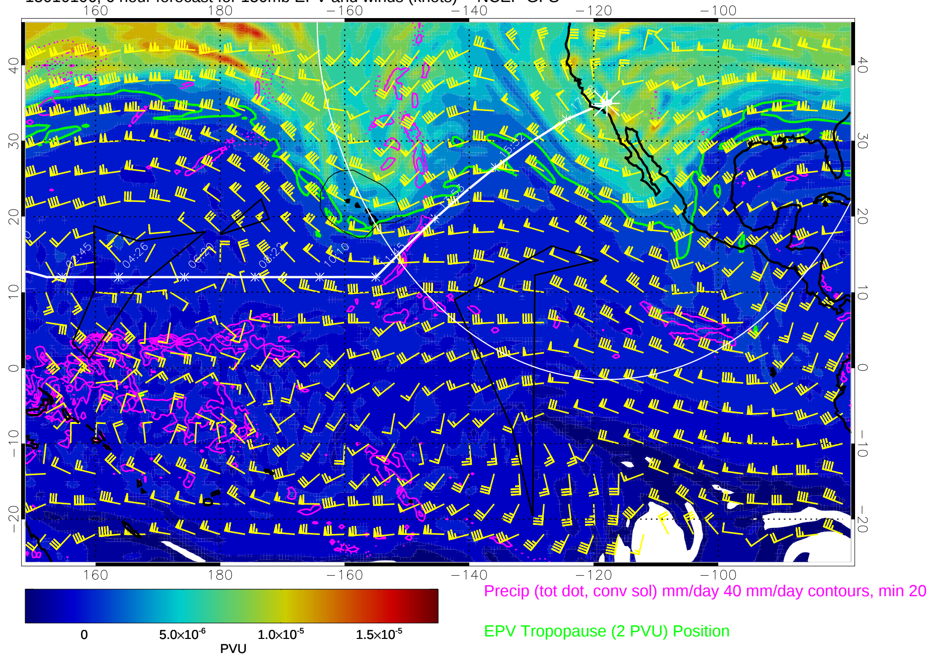
15010106, 6 hour forecast for 150mb EPV and winds (knots) -- NCEP GFS
