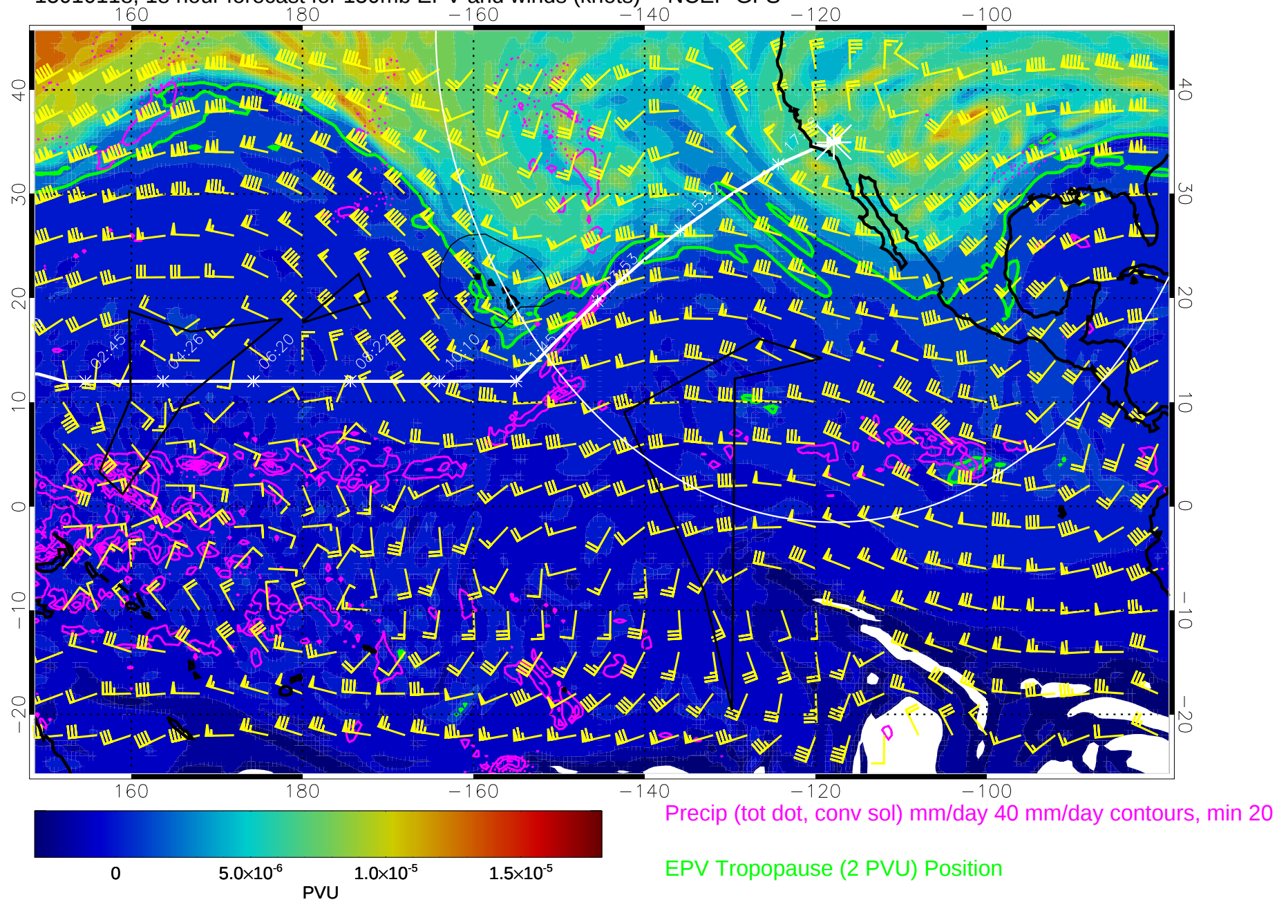
15010118, 18 hour forecast for 150mb EPV and winds (knots) -- NCEP GFS
