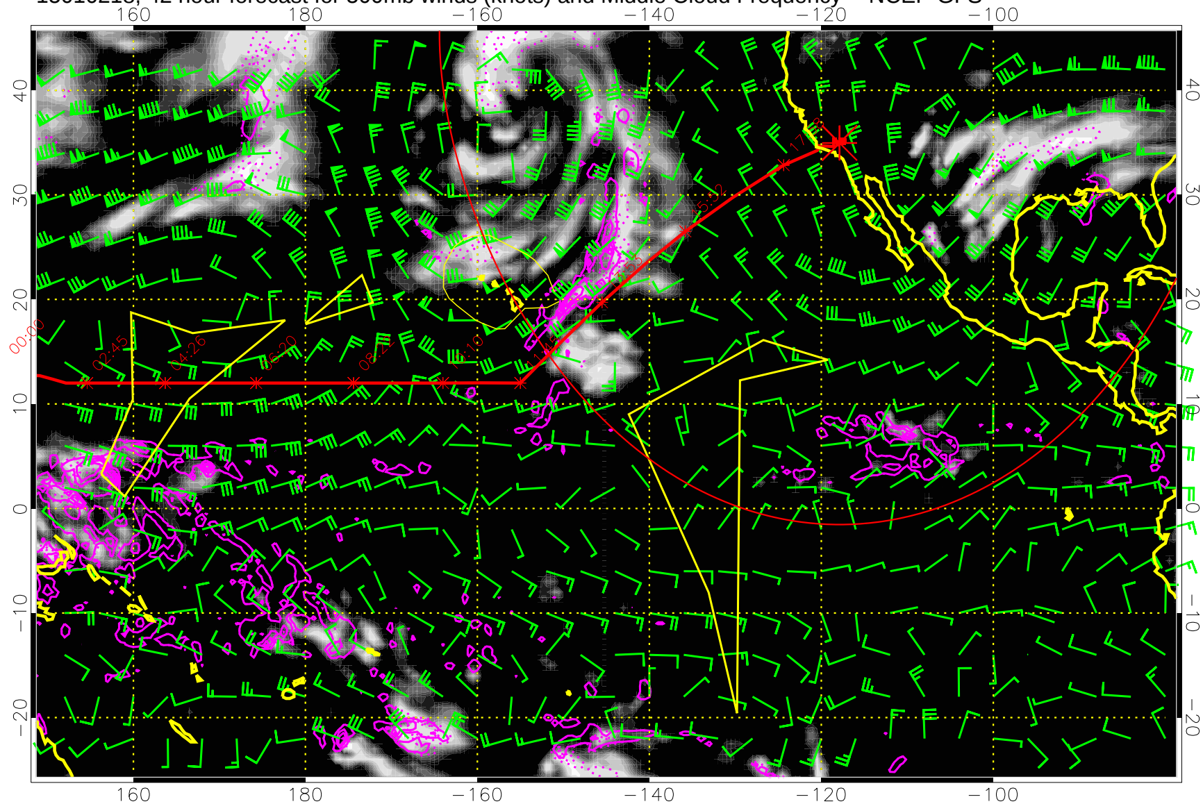
15010218, 42 hour forecast for 500mb winds (knots) and Middle Cloud Frequency -- NCEP GFS
