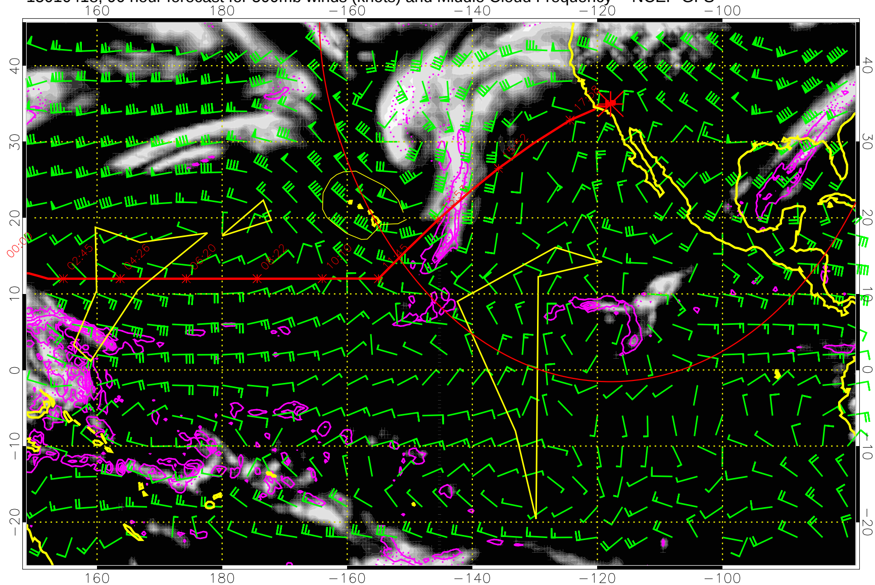
15010418, 90 hour forecast for 500mb winds (knots) and Middle Cloud Frequency -- NCEP GFS
