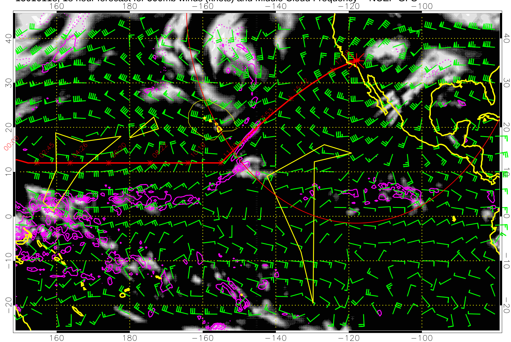
15010118, 18 hour forecast for 500mb winds (knots) and Middle Cloud Frequency -- NCEP GFS
