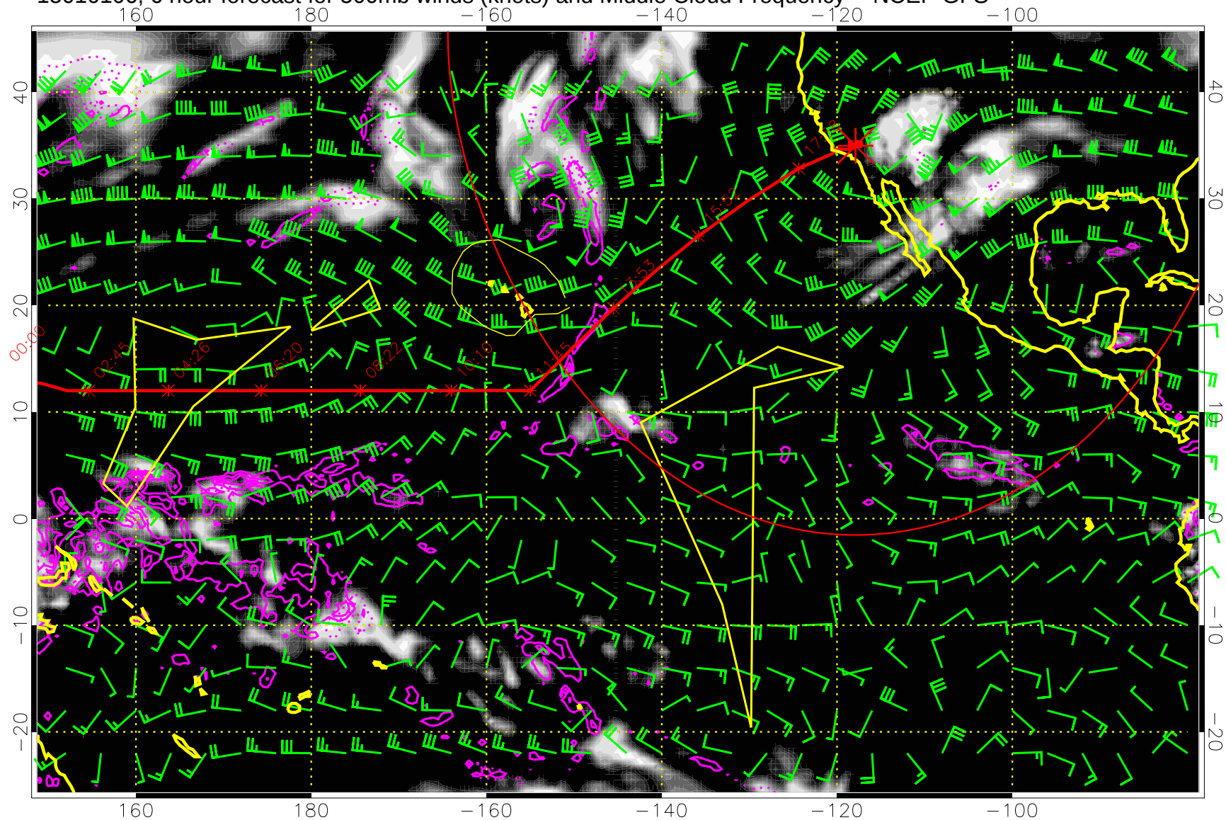
15010106, 6 hour forecast for 500mb winds (knots) and Middle Cloud Frequency -- NCEP GFS
