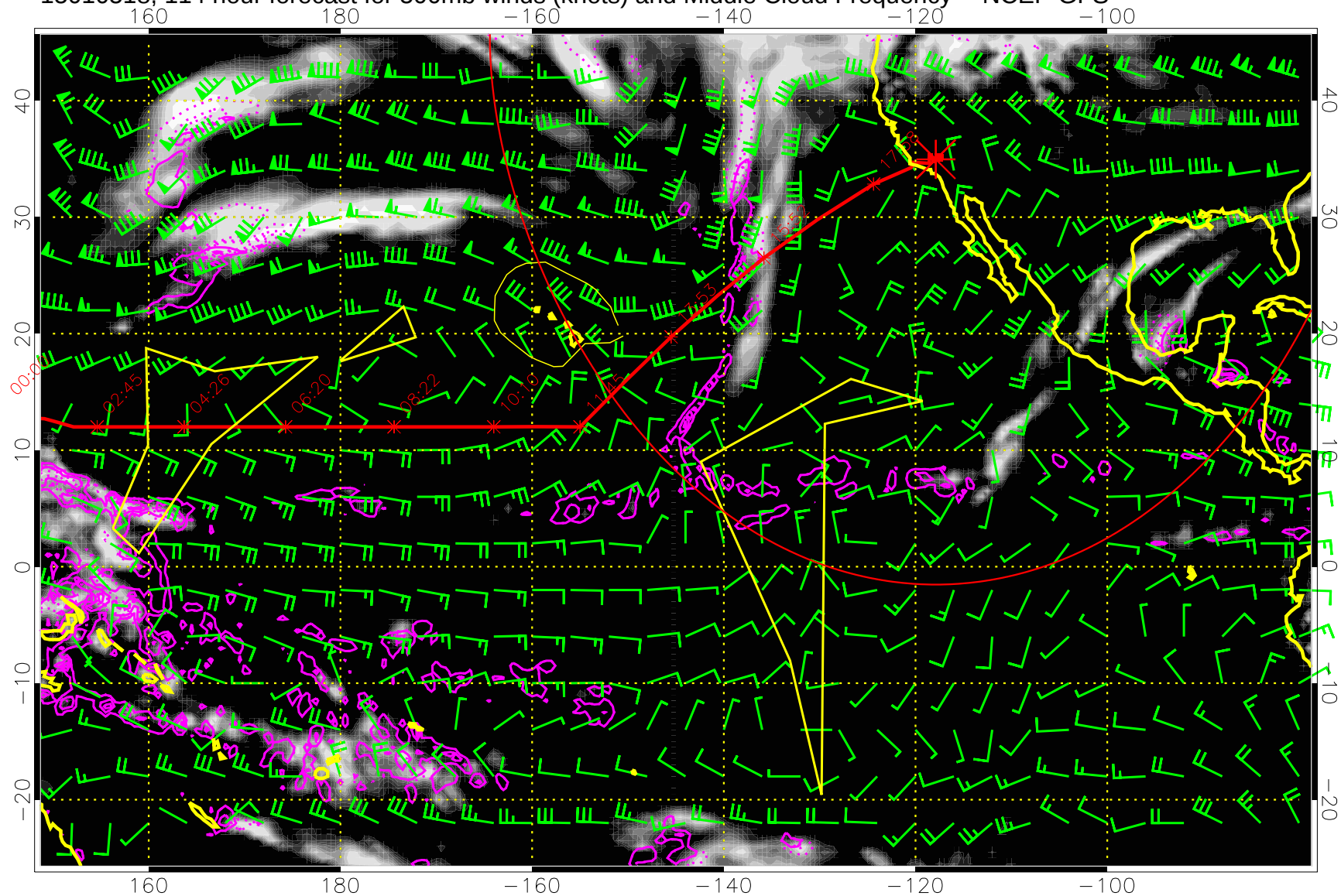
15010518, 114 hour forecast for 500mb winds (knots) and Middle Cloud Frequency -- NCEP GFS
