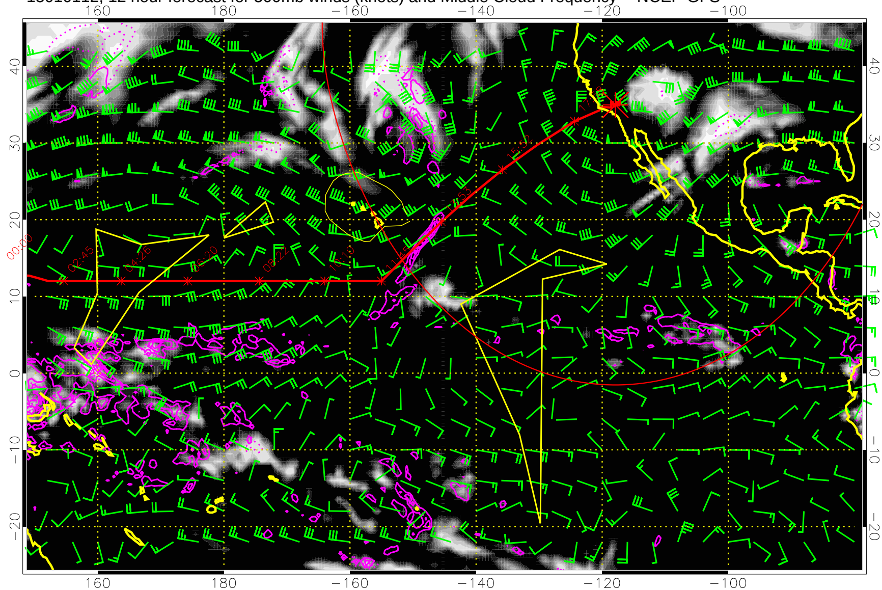
15010112, 12 hour forecast for 500mb winds (knots) and Middle Cloud Frequency -- NCEP GFS
