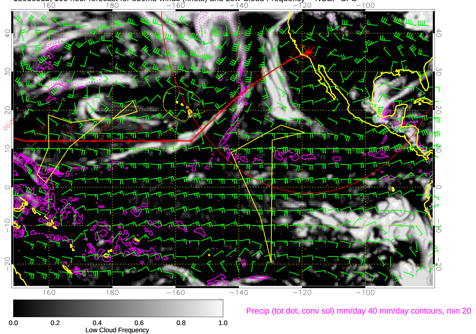
15010512, 108 hour forecast for 850mb winds (knots) and Low Cloud Frequency -- NCEP GFS
