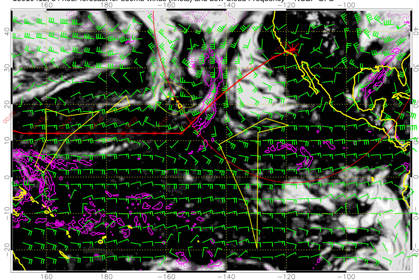
15010412, 84 hour forecast for 850mb winds (knots) and Low Cloud Frequency -- NCEP GFS
