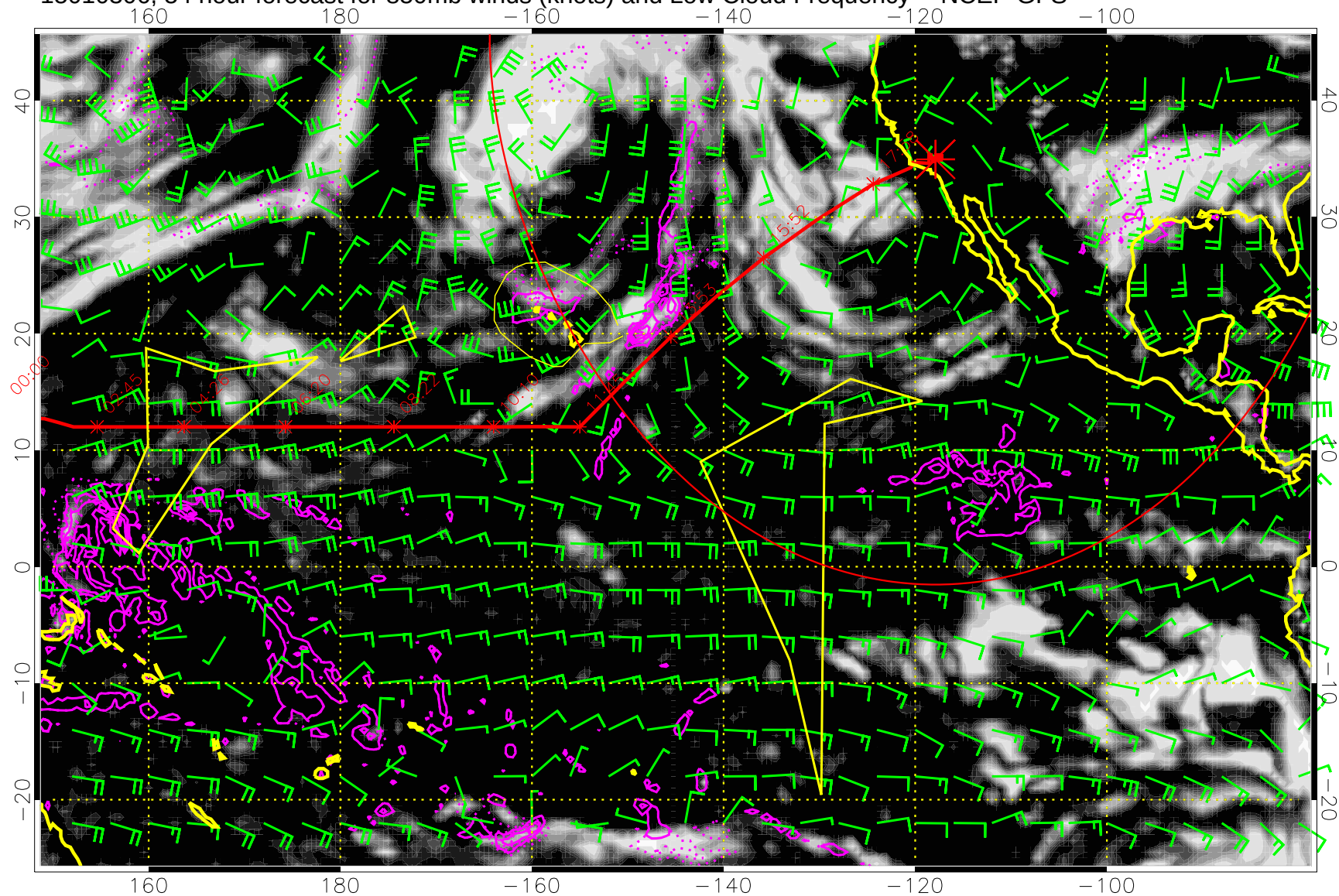
15010306, 54 hour forecast for 850mb winds (knots) and Low Cloud Frequency -- NCEP GFS
