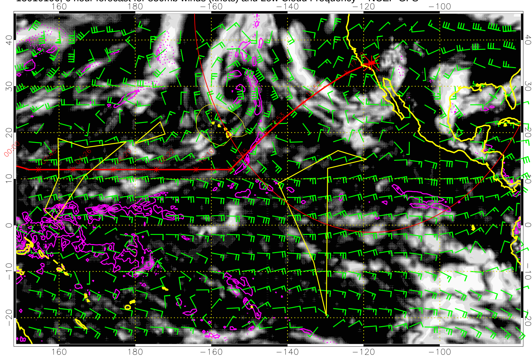
15010106, 6 hour forecast for 850mb winds (knots) and Low Cloud Frequency -- NCEP GFS
