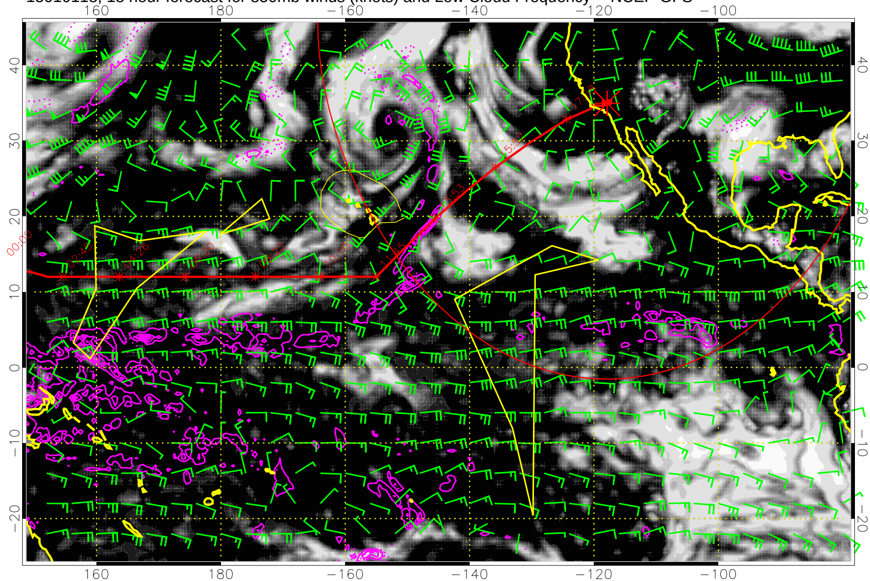
15010118, 18 hour forecast for 850mb winds (knots) and Low Cloud Frequency -- NCEP GFS
