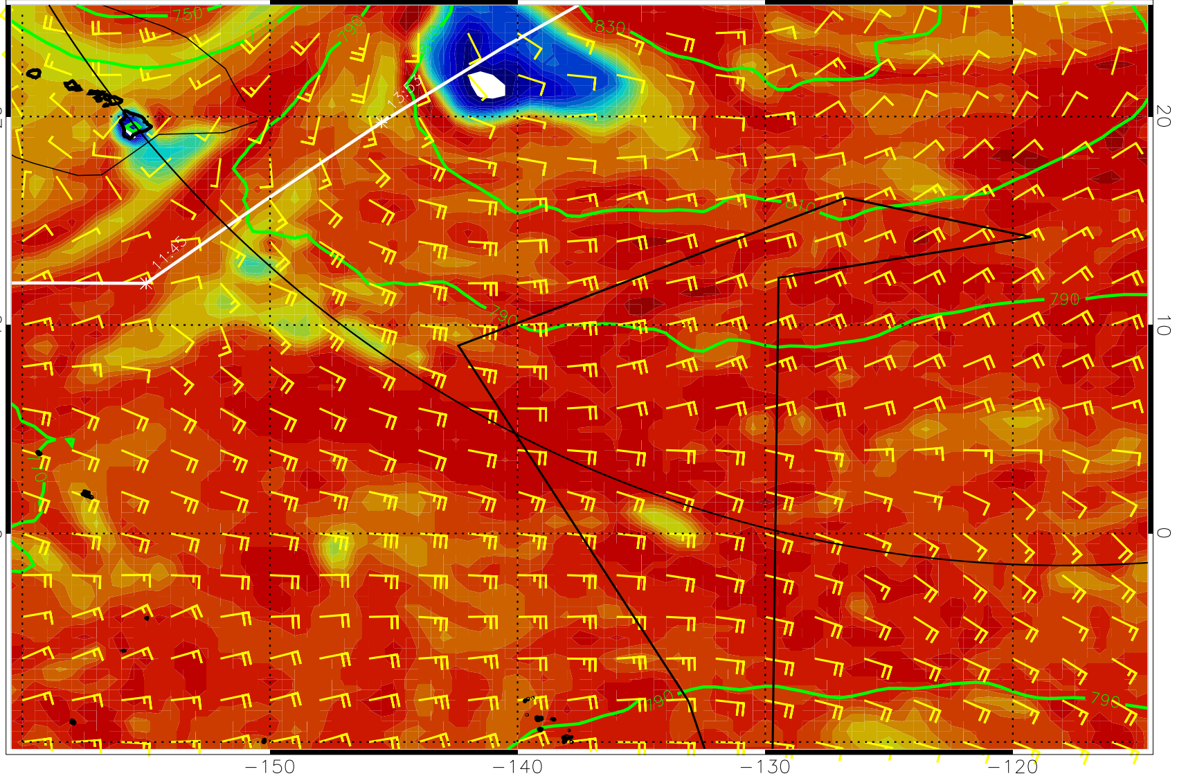
20020215, 00 local forecast for elements T1H, L, and winds (knots) 20020215 20020215 20020215 20020215 -150 -140 -130 -120
