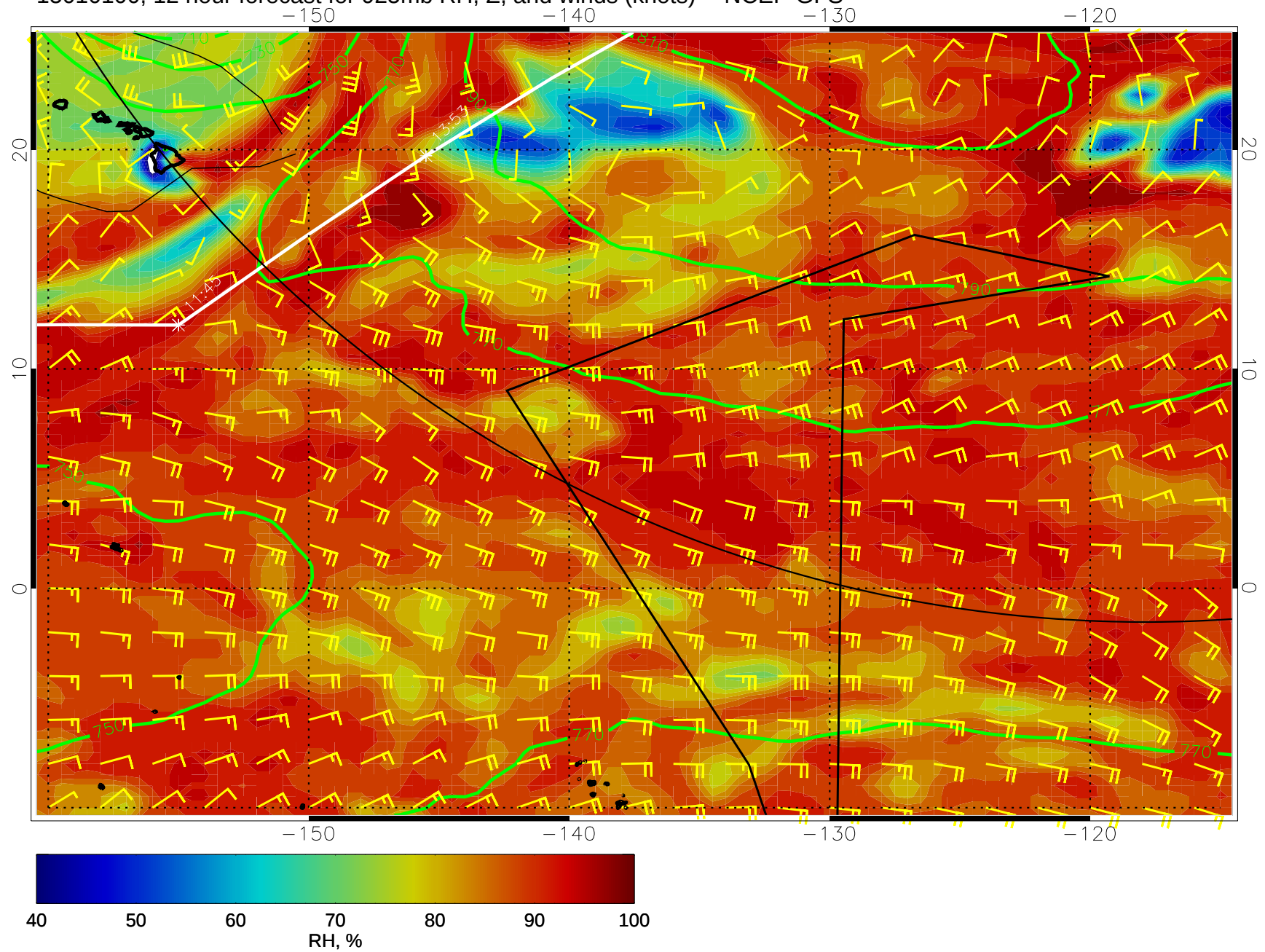
15010100, 12 hour forecast for 925mb RH, Z, and winds (knots) -- NCEP GFS
