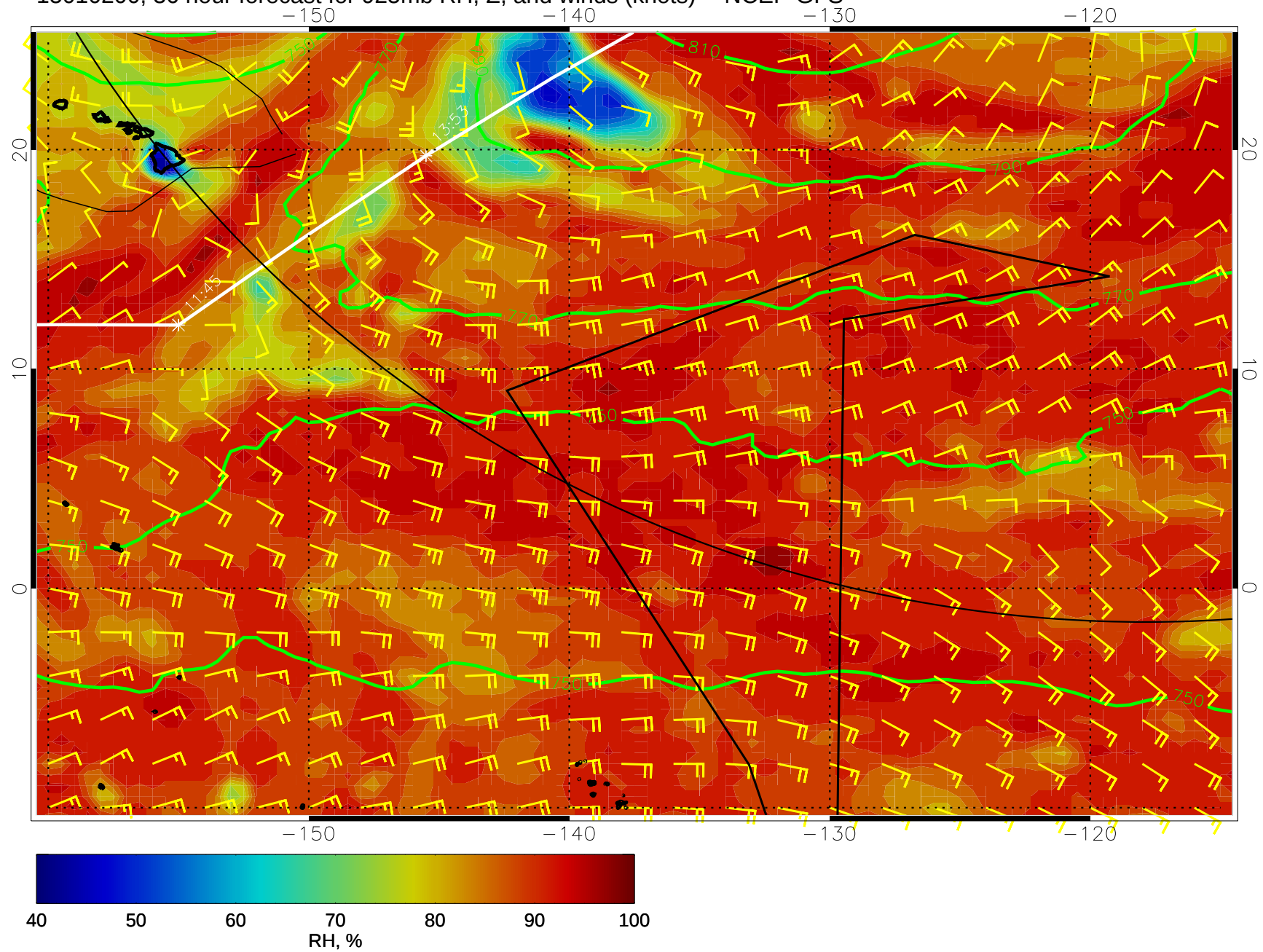
15010200, 36 hour forecast for 925mb RH, Z, and winds (knots) -- NCEP GFS
