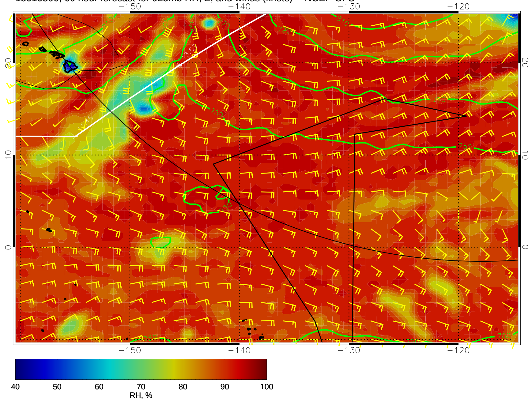
15010300, 60 hour forecast for 925mb RH, Z, and winds (knots) -- NCEP GFS
