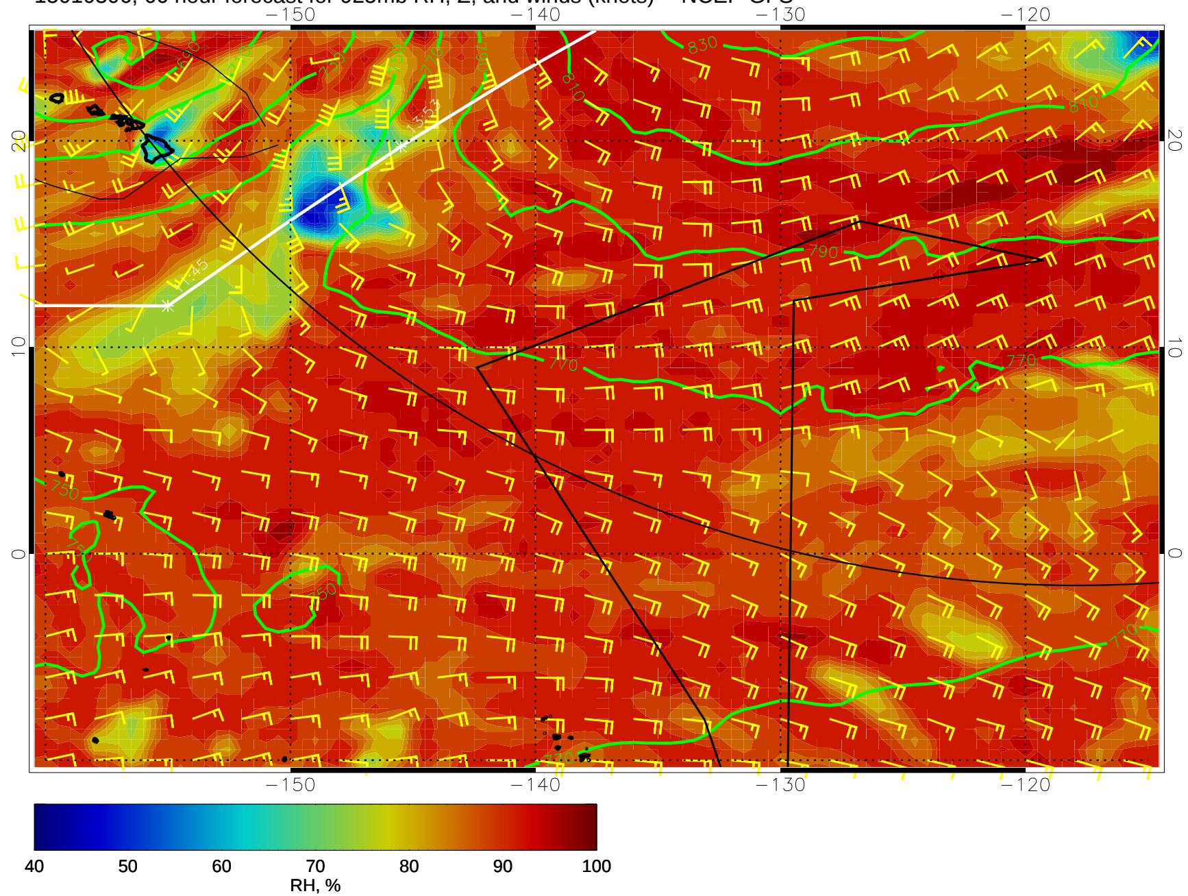
15010306, 66 hour forecast for 925mb RH, Z, and winds (knots) -- NCEP GFS
