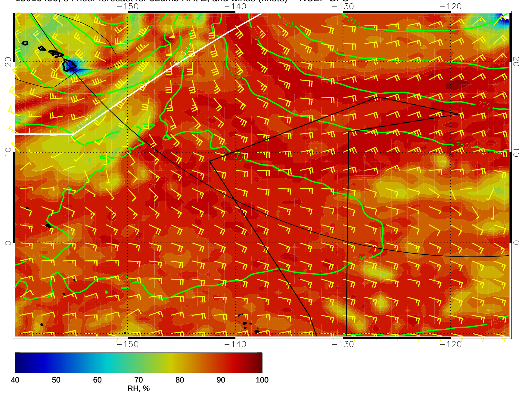
15010400, 84 hour forecast for 925mb RH, Z, and winds (knots) -- NCEP GFS
