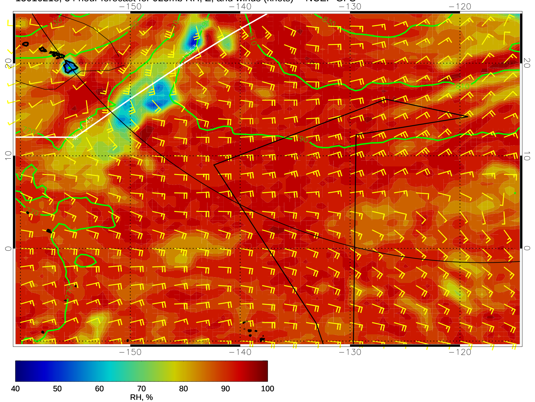
15010218, 54 hour forecast for 925mb RH, Z, and winds (knots) -- NCEP GFS
