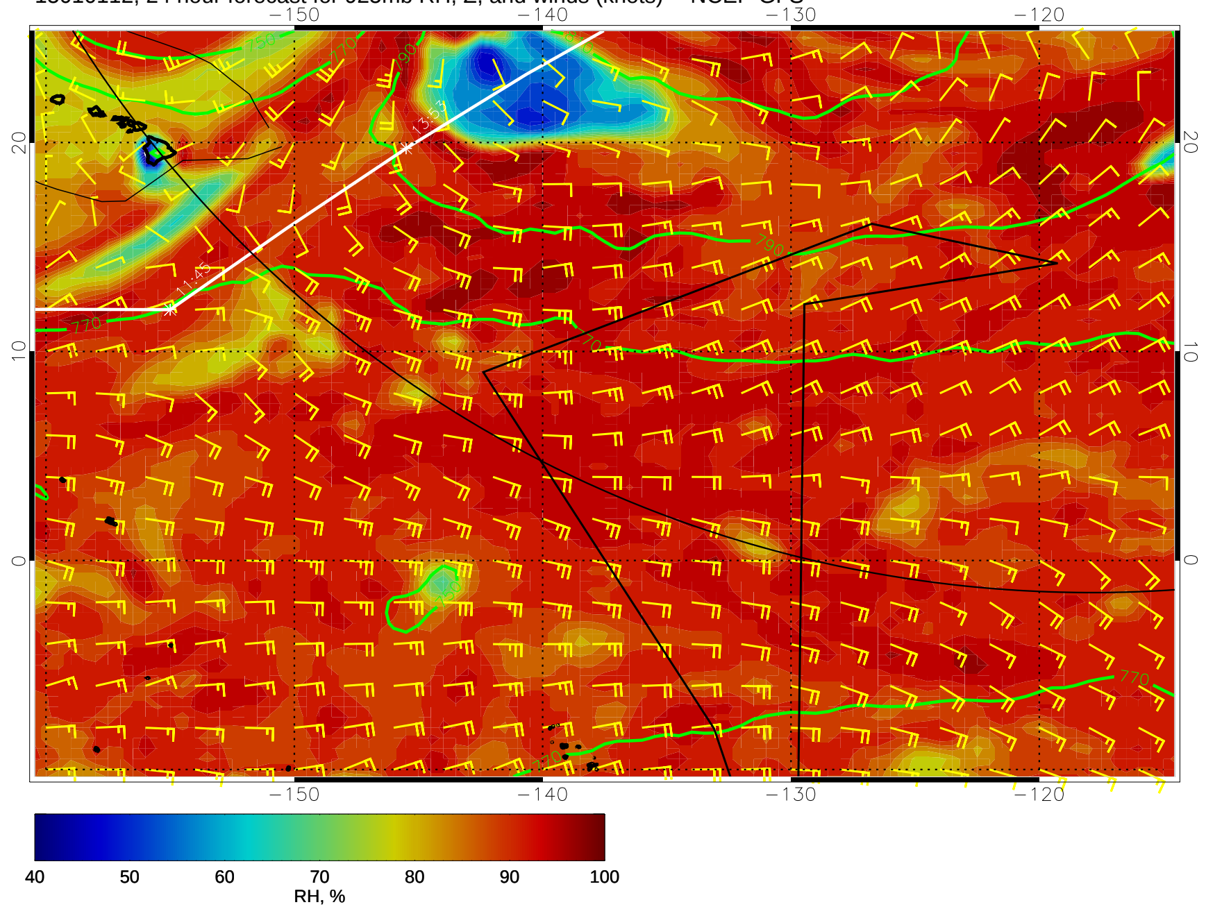
15010112, 24 hour forecast for 925mb RH, Z, and winds (knots) -- NCEP GFS
