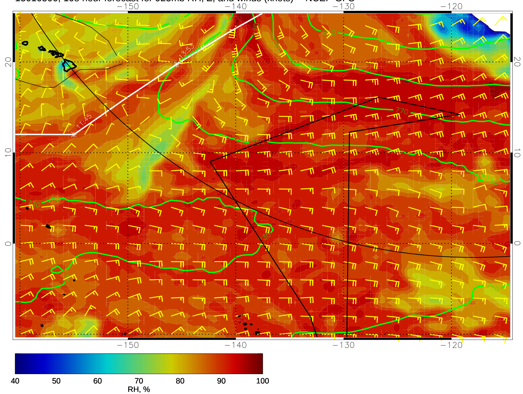
15010500, 108 hour forecast for 925mb RH, Z, and winds (knots) -- NCEP GFS
