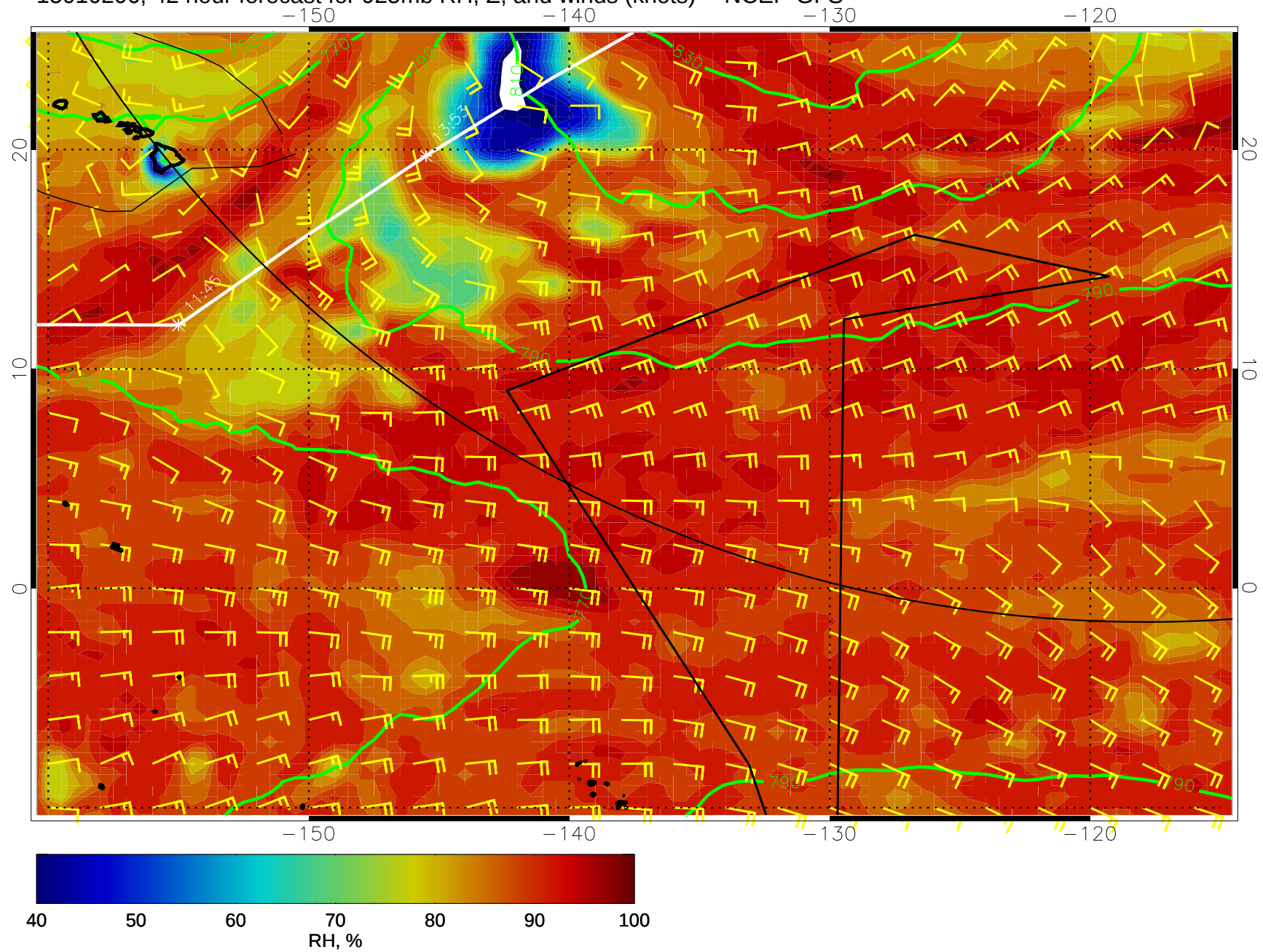
15010206, 42 hour forecast for 925mb RH, Z, and winds (knots) -- NCEP GFS
