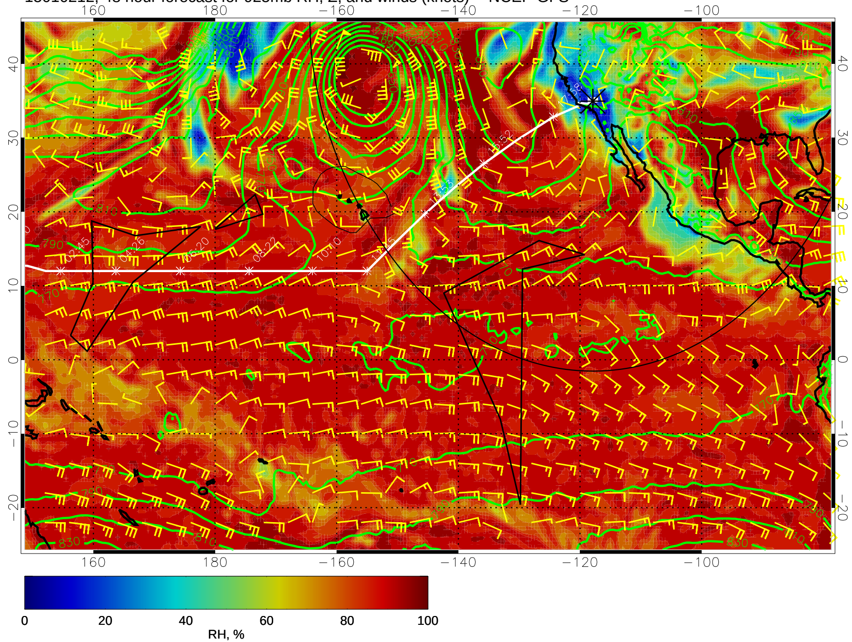
15010212, 48 hour forecast for 925mb RH, Z, and winds (knots) -- NCEP GFS
