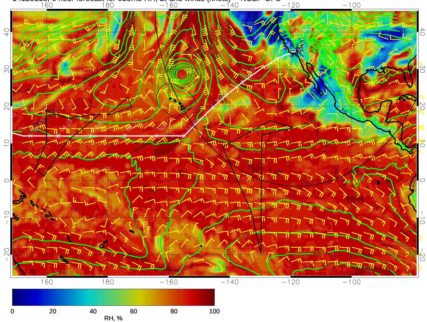
14123118, 6 hour forecast for 925mb RH, Z, and winds (knots) -- NCEP GFS
