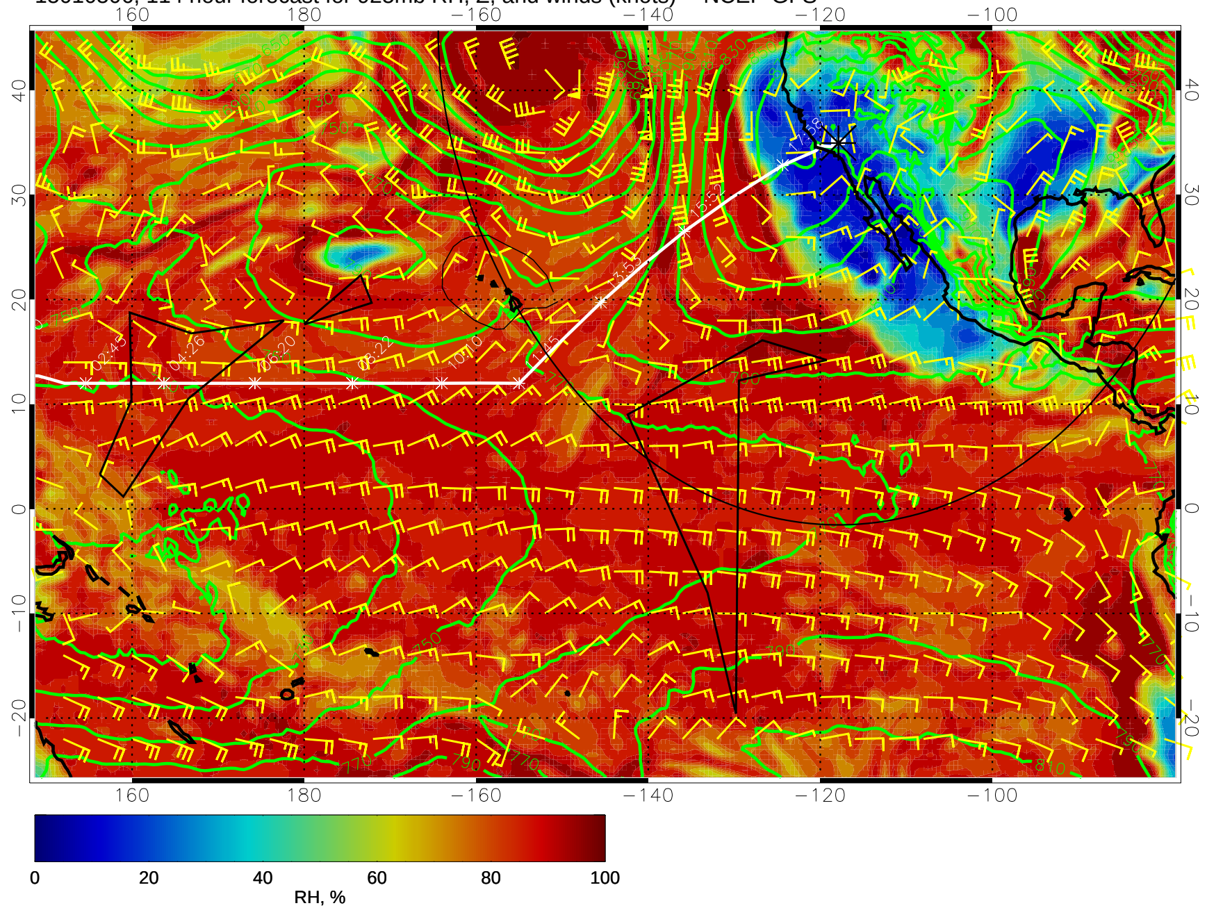
15010506, 114 hour forecast for 925mb RH, Z, and winds (knots) -- NCEP GFS
