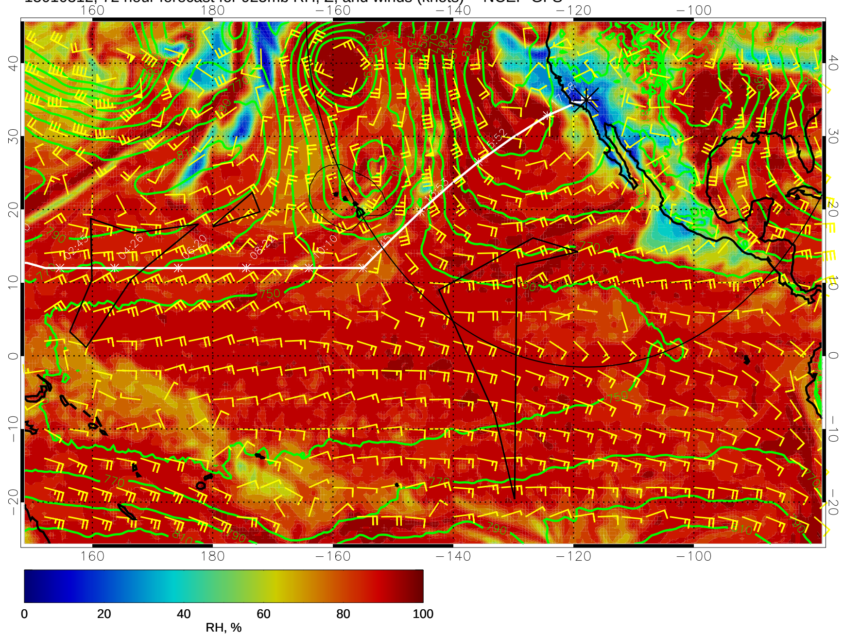
15010312, 72 hour forecast for 925mb RH, Z, and winds (knots) -- NCEP GFS
