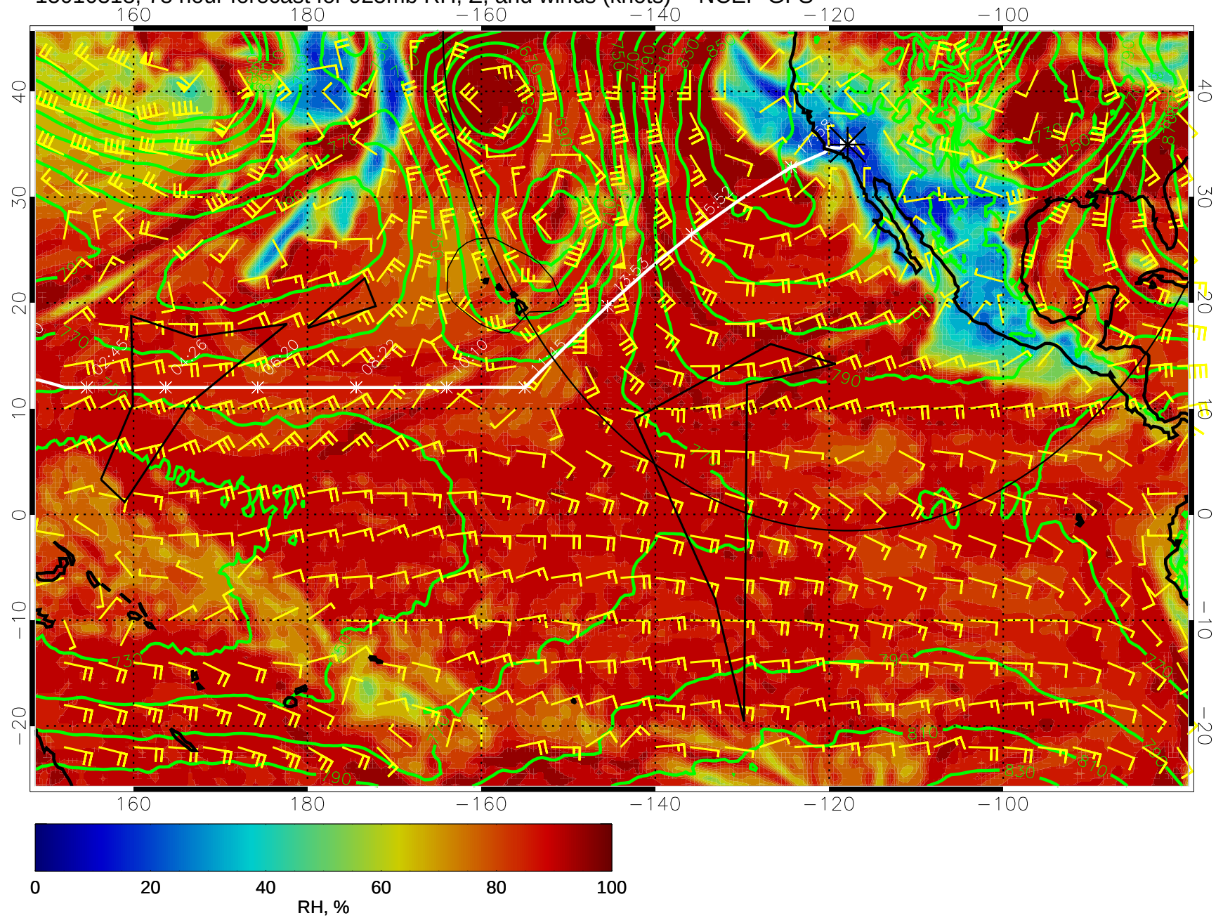
15010318, 78 hour forecast for 925mb RH, Z, and winds (knots) -- NCEP GFS
