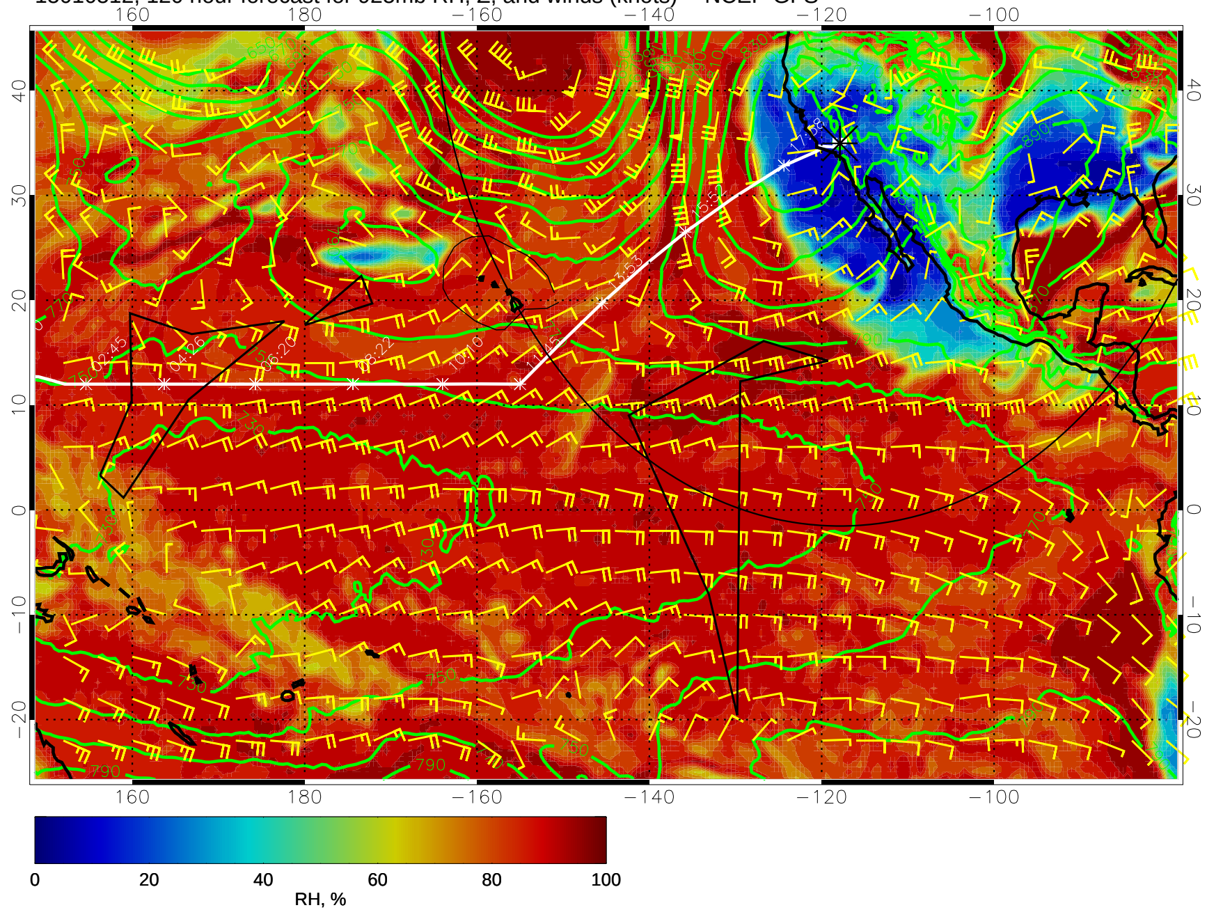
15010512, 120 hour forecast for 925mb RH, Z, and winds (knots) -- NCEP GFS
