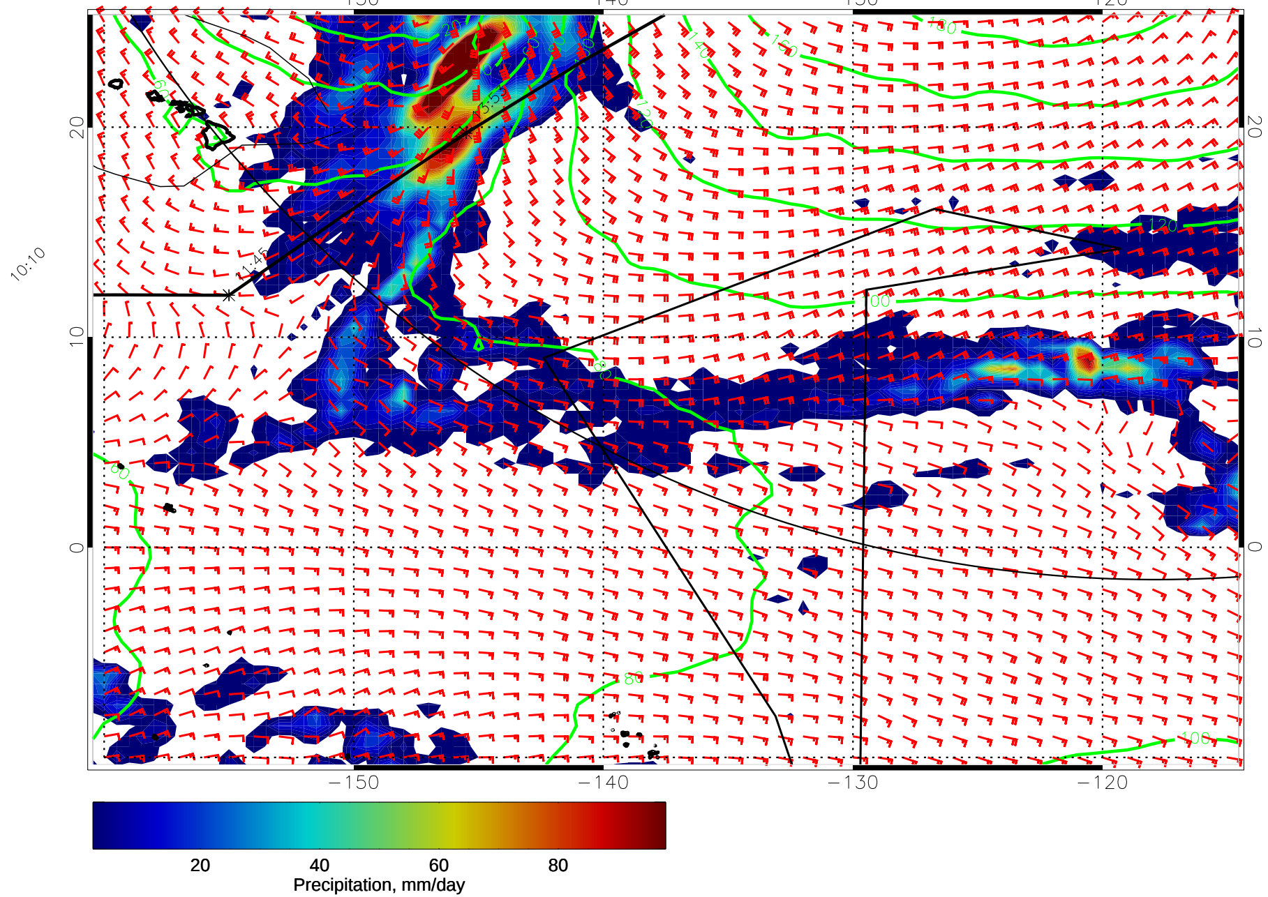
15010406, 90 hour forecast for precip, 1000mb Z, and winds (knots) -- NCEP GFS
