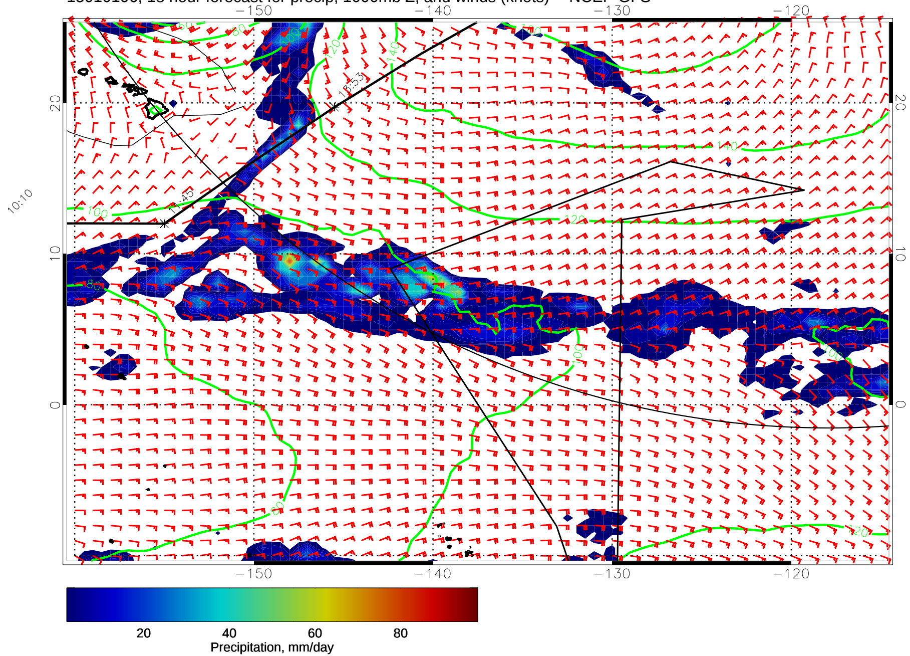
15010106, 18 hour forecast for precip, 1000mb Z, and winds (knots) -- NCEP GFS
