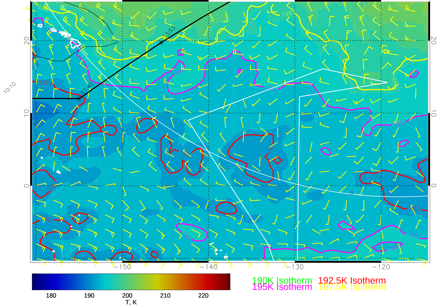
15010500, 108 hour forecast for 70mb T and winds (knots) -- NCEP GFS
