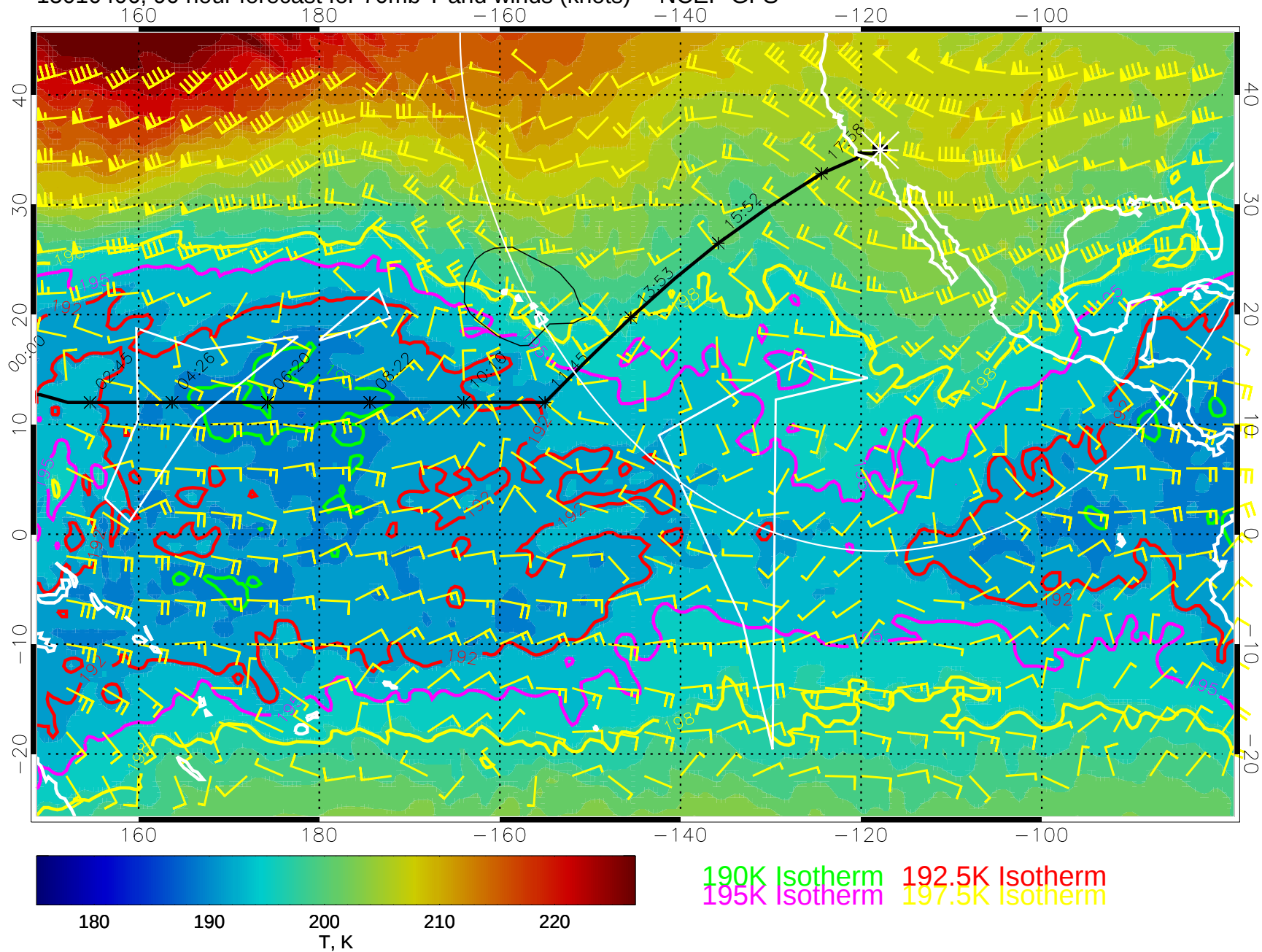
15010406, 90 hour forecast for 70mb T and winds (knots) -- NCEP GFS
