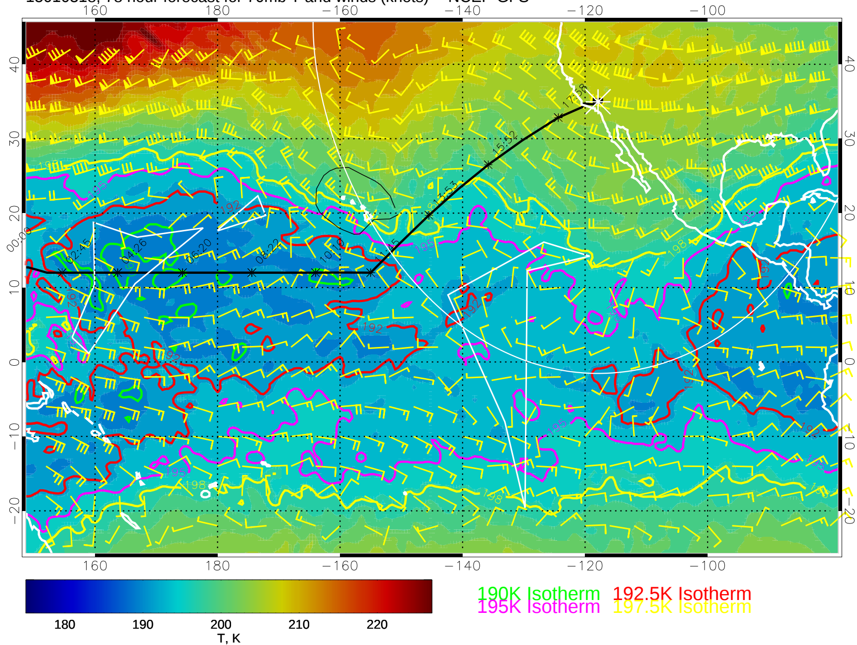
15010318, 78 hour forecast for 70mb T and winds (knots) -- NCEP GFS
