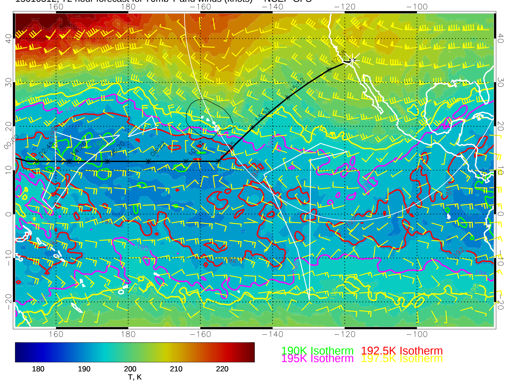
15010312, 72 hour forecast for 70mb T and winds (knots) -- NCEP GFS
