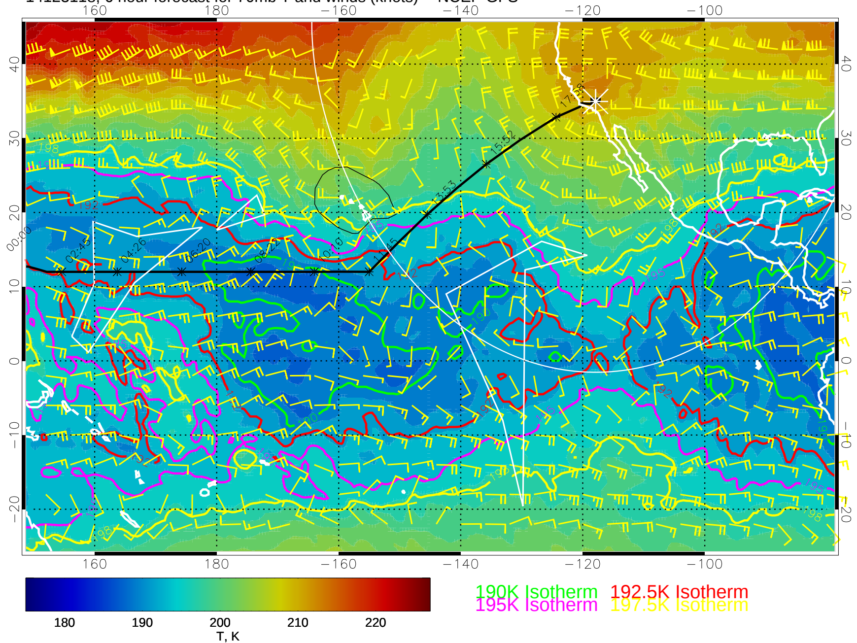
14123118, 6 hour forecast for 70mb T and winds (knots) -- NCEP GFS
