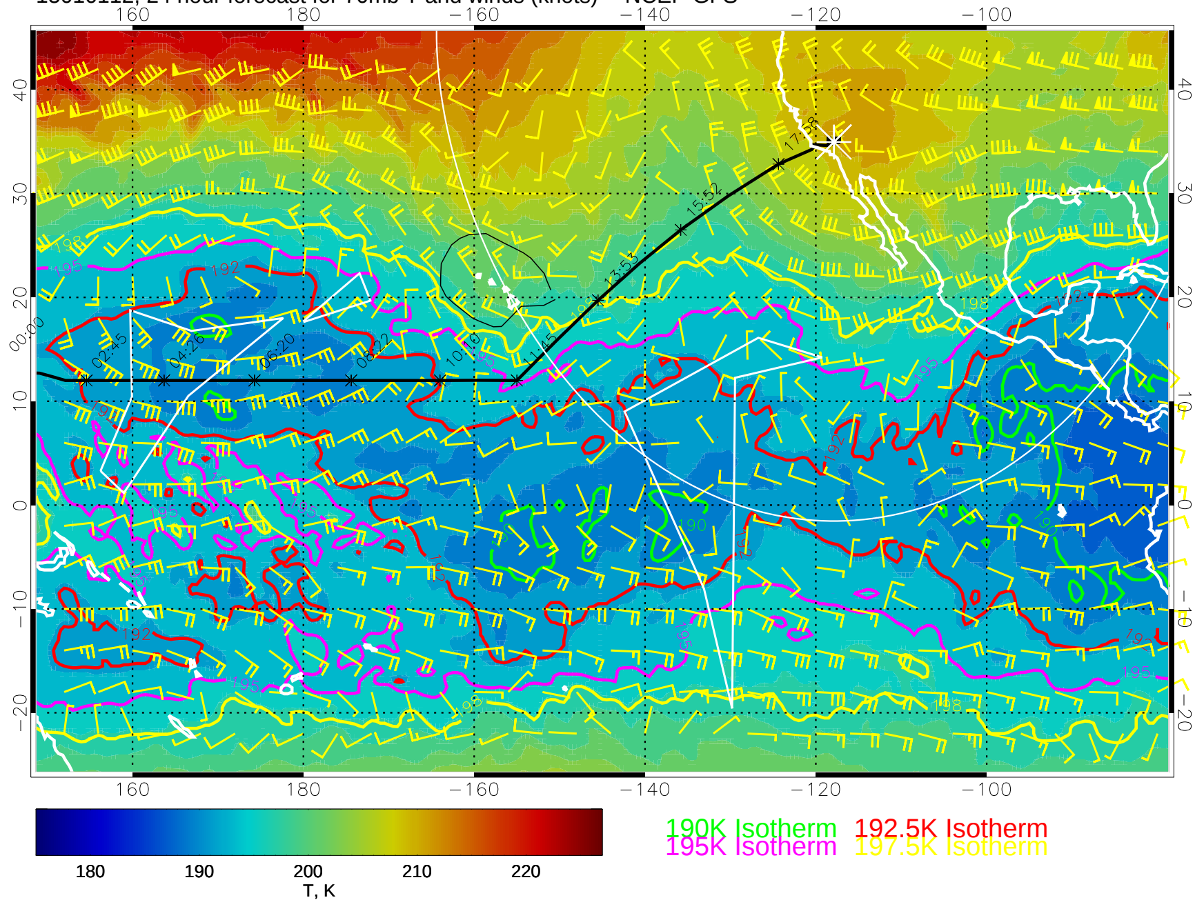
15010112, 24 hour forecast for 70mb T and winds (knots) -- NCEP GFS
