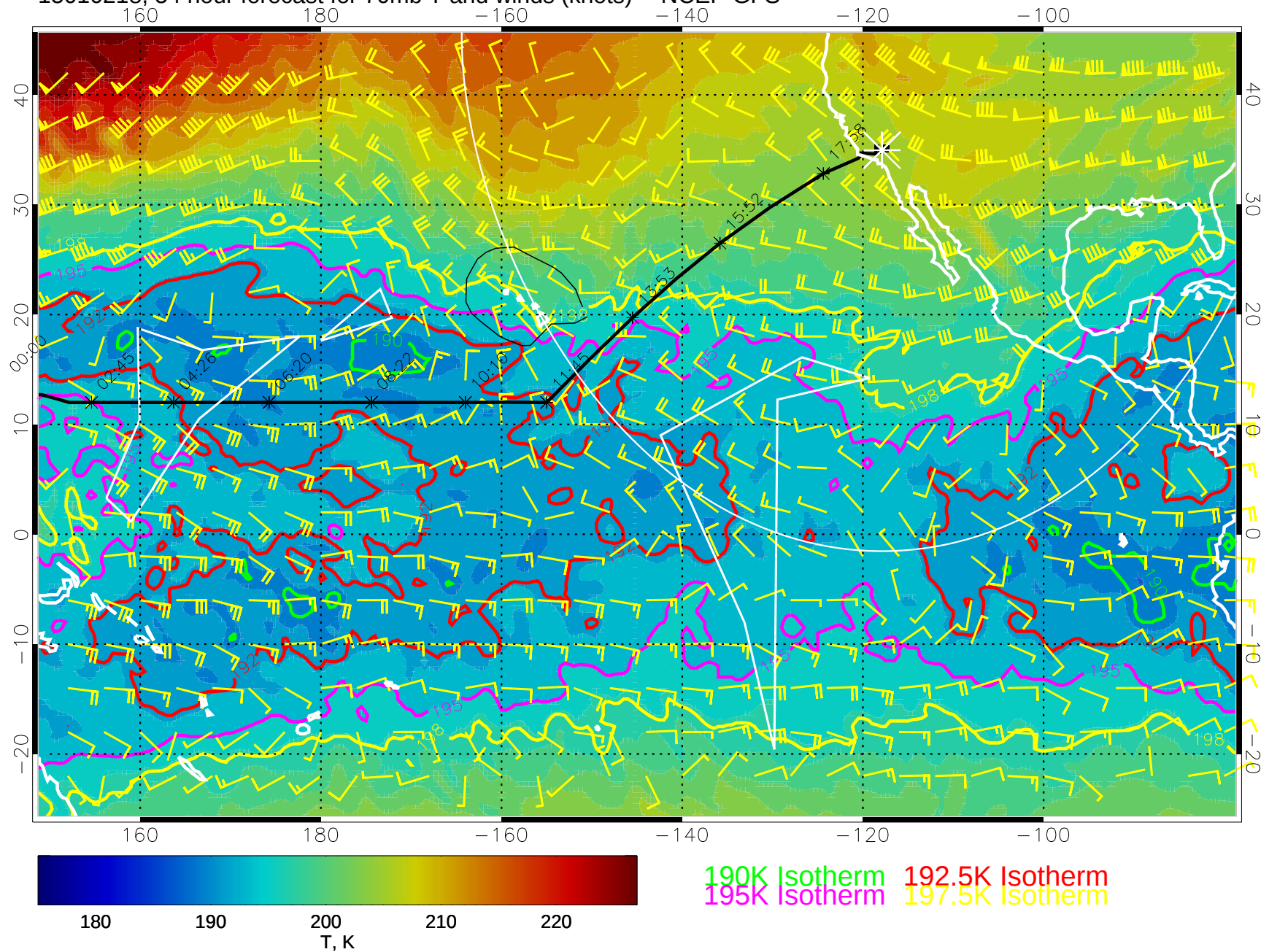
15010218, 54 hour forecast for 70mb T and winds (knots) -- NCEP GFS
