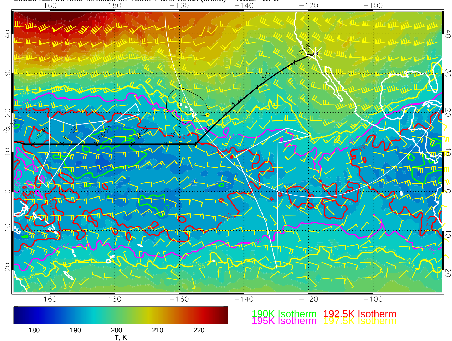
15010412, 96 hour forecast for 70mb T and winds (knots) -- NCEP GFS
