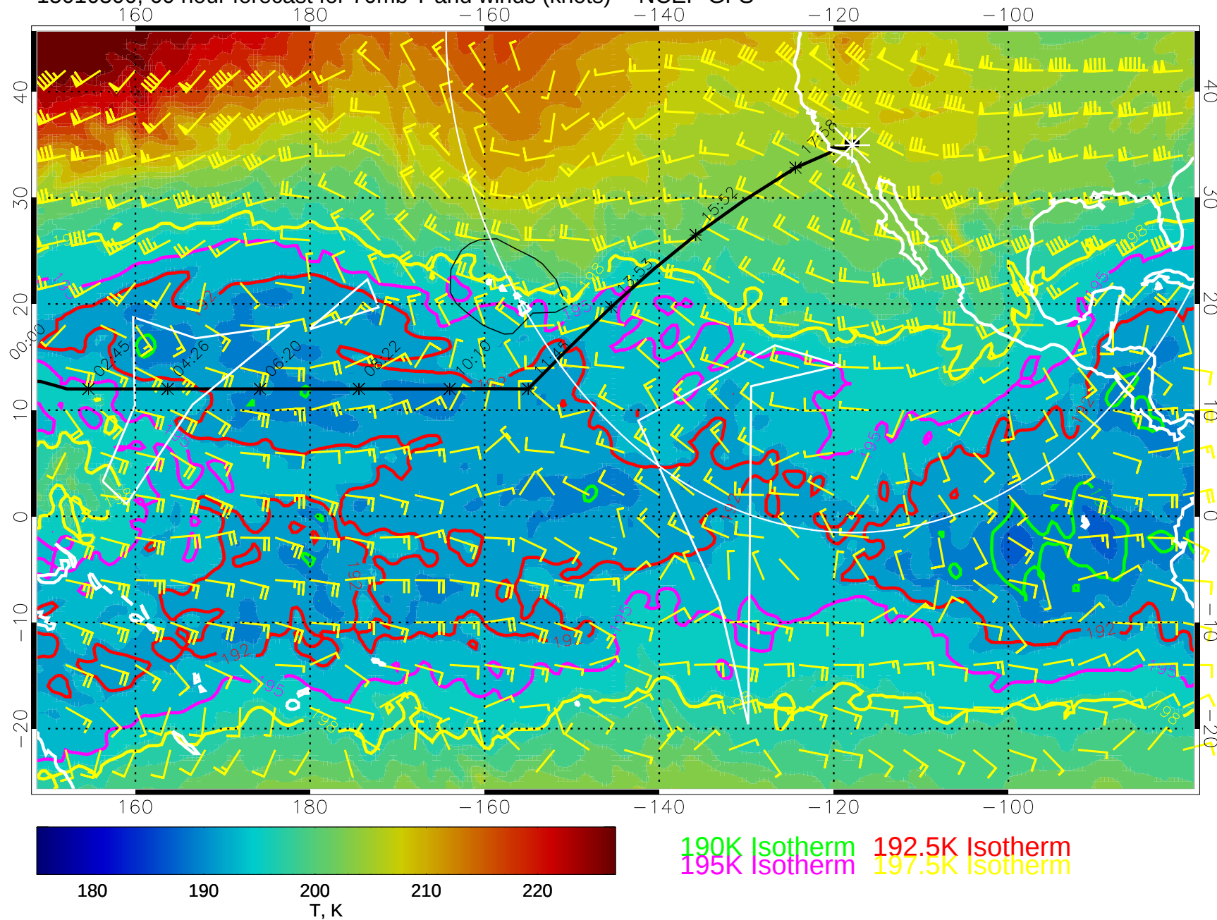
15010300, 60 hour forecast for 70mb T and winds (knots) -- NCEP GFS
