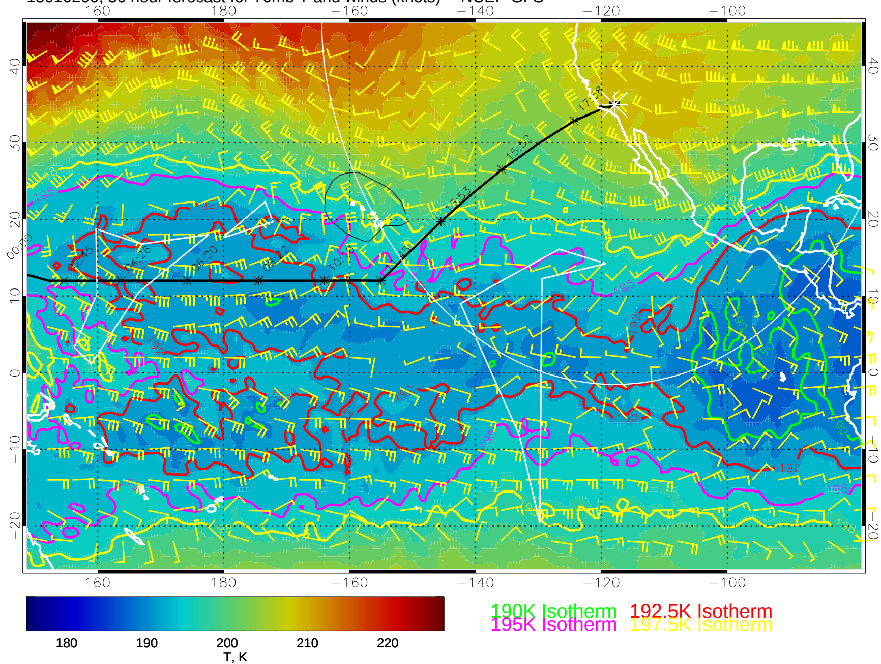
15010200, 36 hour forecast for 70mb T and winds (knots) -- NCEP GFS
