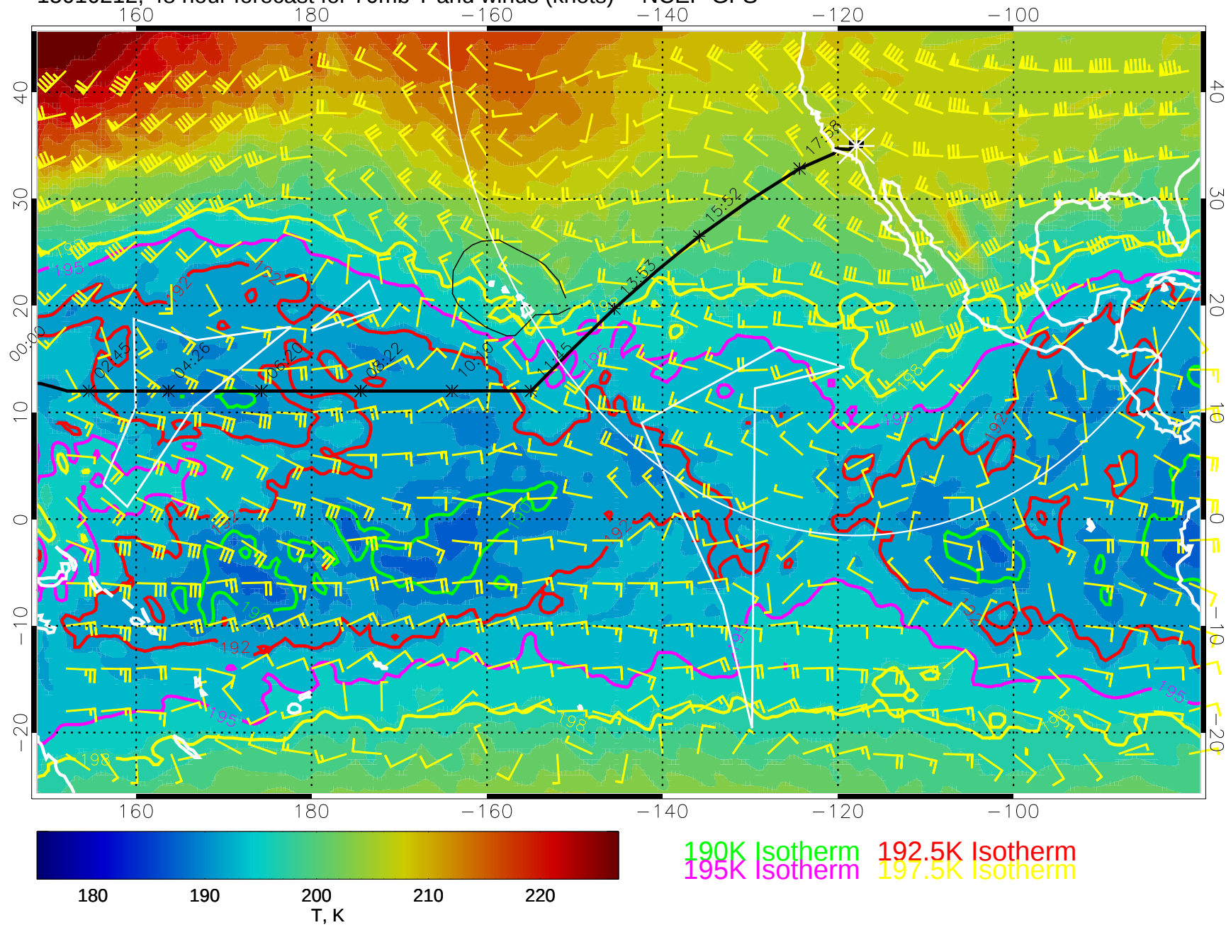
15010212, 48 hour forecast for 70mb T and winds (knots) -- NCEP GFS
