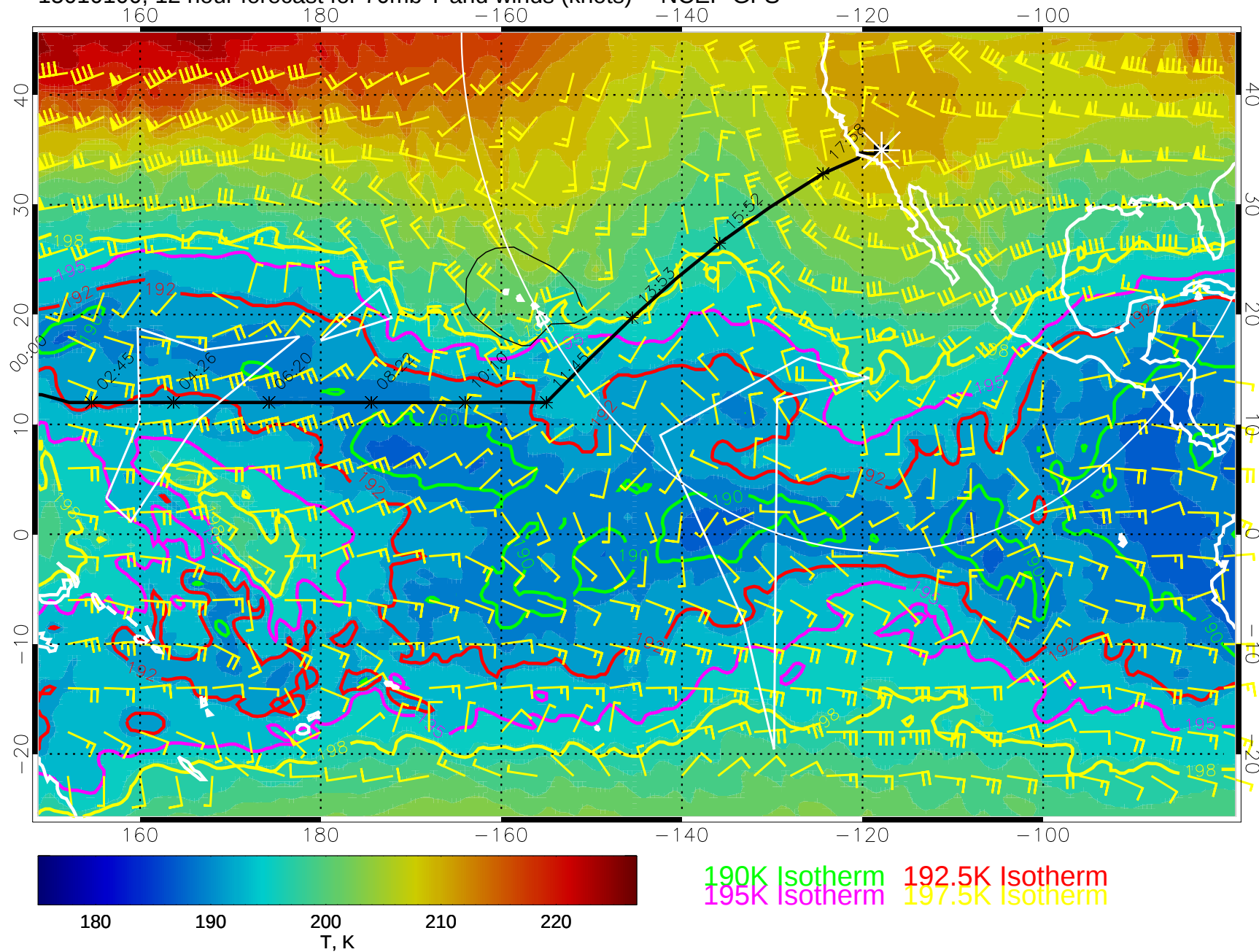
15010100, 12 hour forecast for 70mb T and winds (knots) -- NCEP GFS
