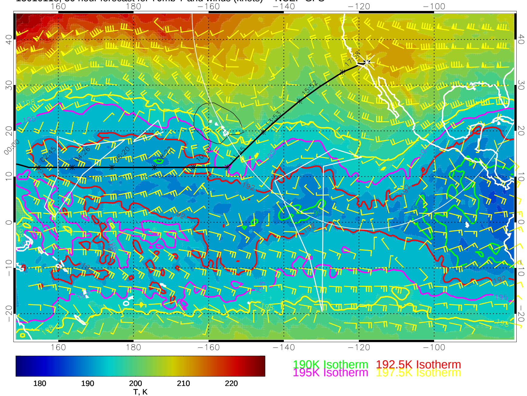
15010118, 30 hour forecast for 70mb T and winds (knots) -- NCEP GFS
