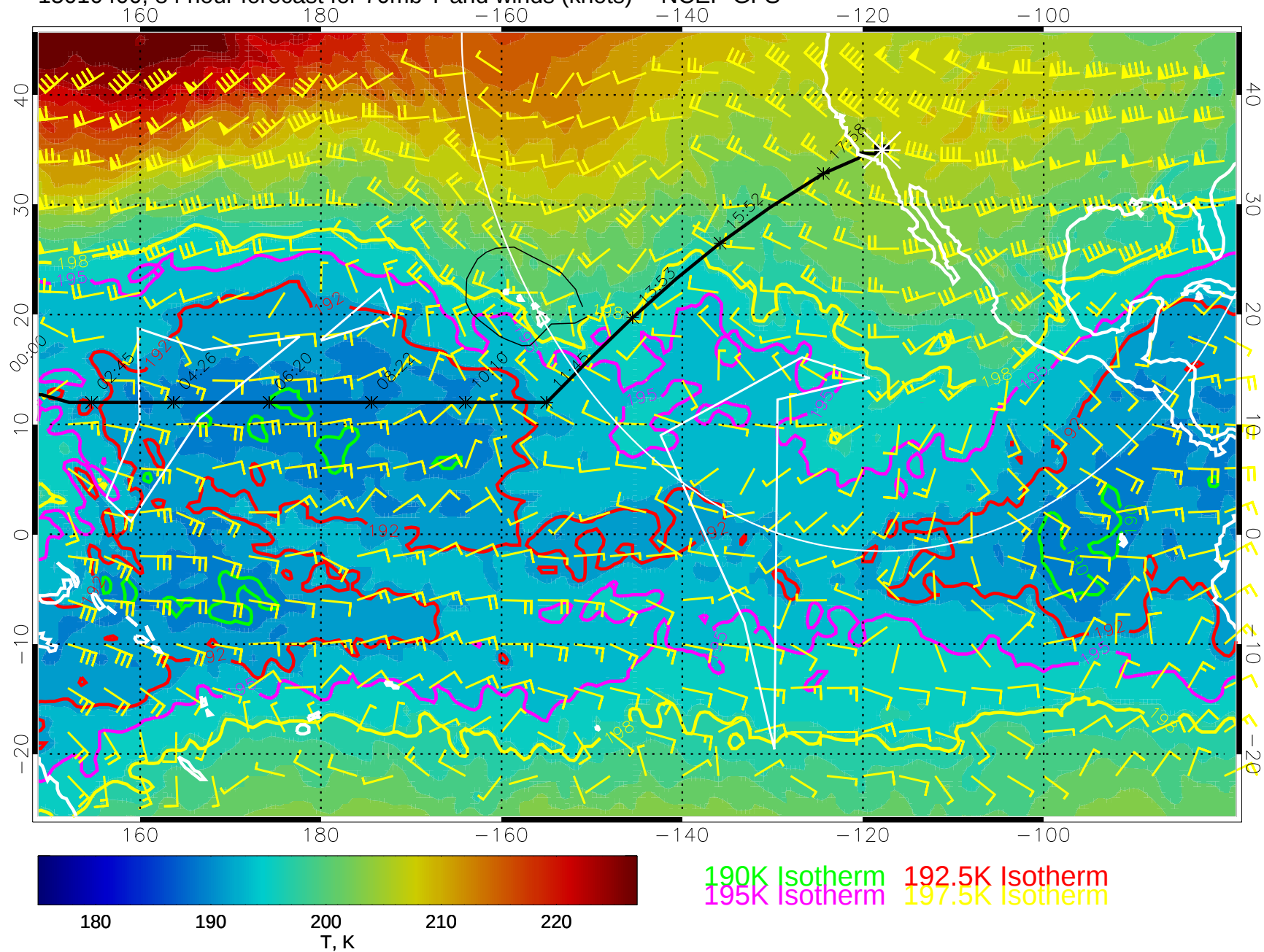
15010400, 84 hour forecast for 70mb T and winds (knots) -- NCEP GFS
