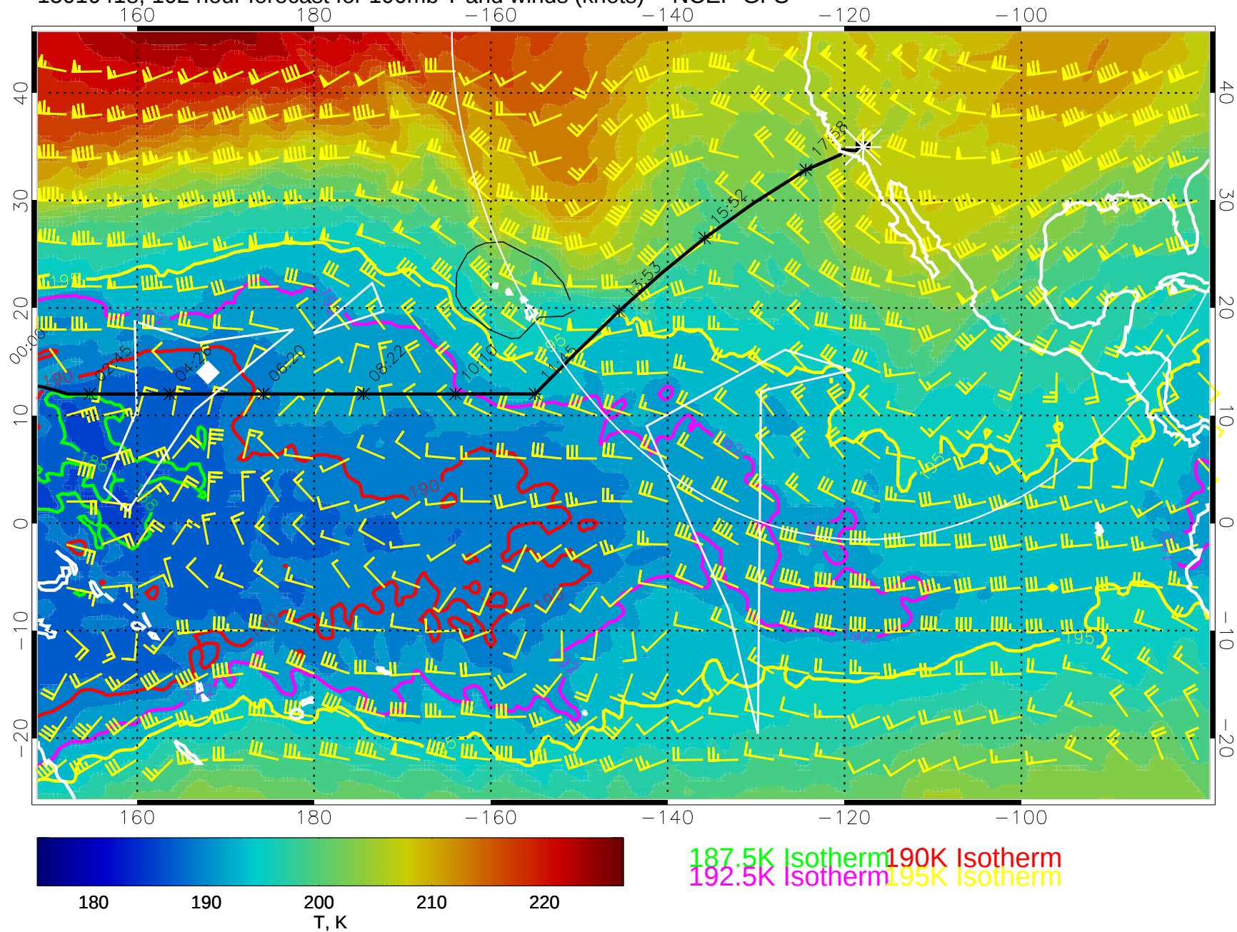
15010418, 102 hour forecast for 100mb T and winds (knots) -- NCEP GFS
