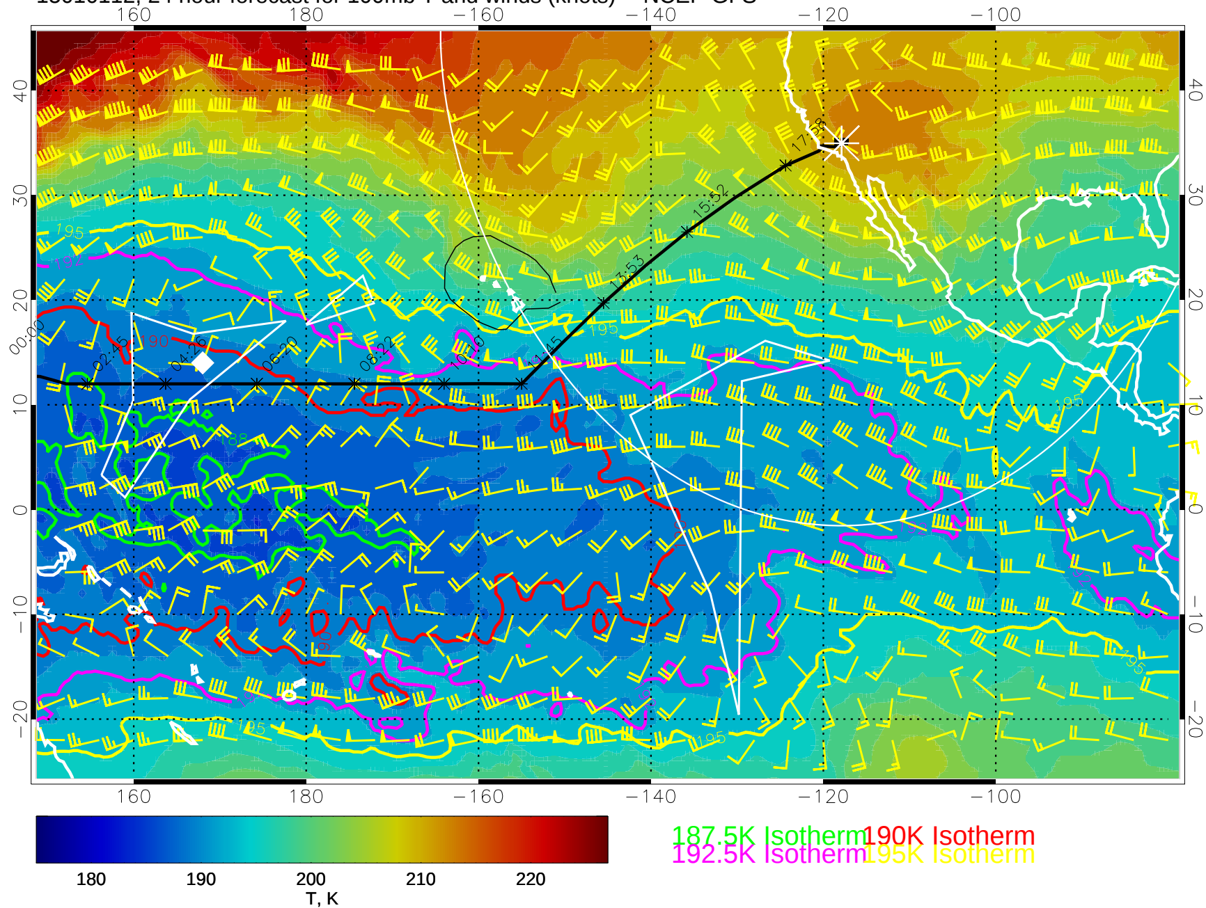
15010112, 24 hour forecast for 100mb T and winds (knots) -- NCEP GFS
