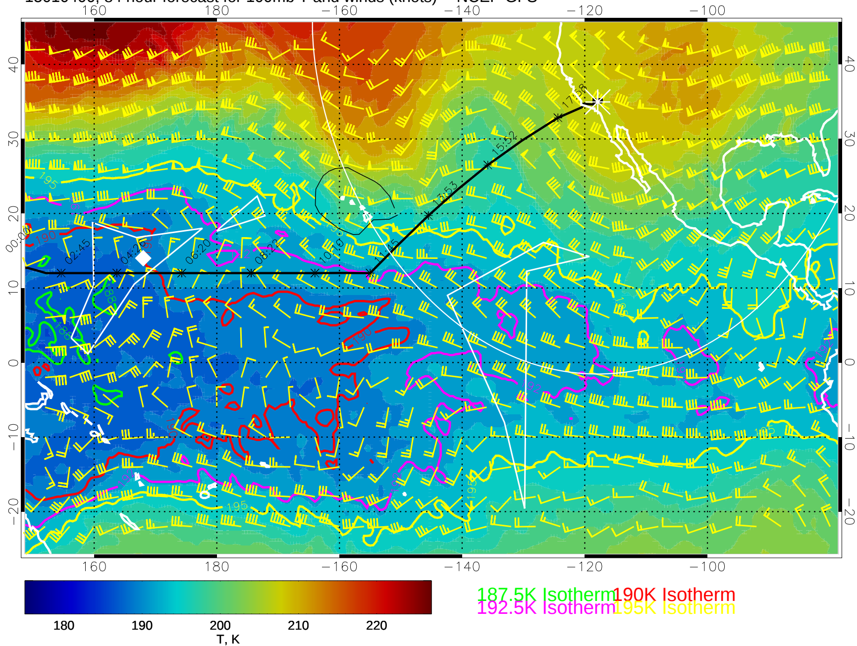
15010400, 84 hour forecast for 100mb T and winds (knots) -- NCEP GFS
