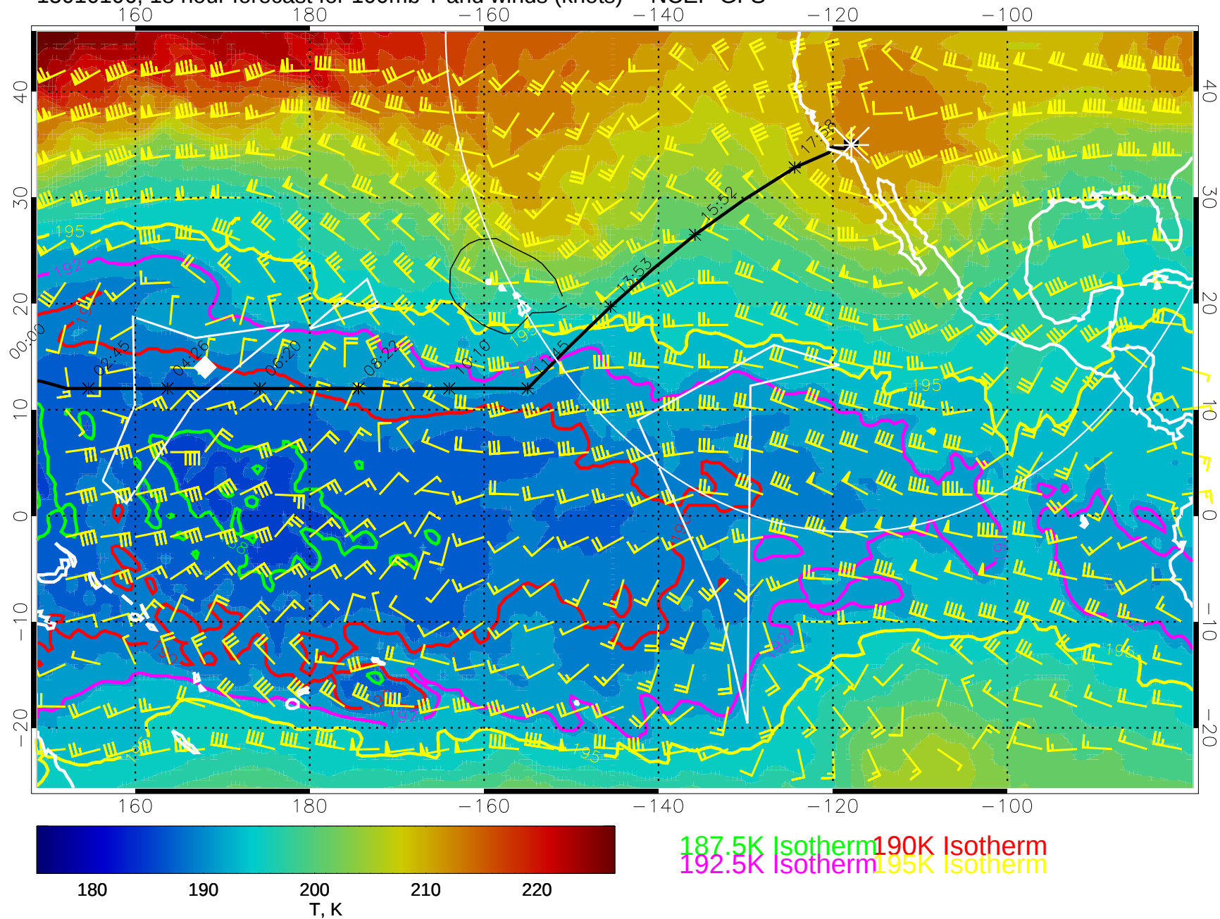
15010106, 18 hour forecast for 100mb T and winds (knots) -- NCEP GFS
