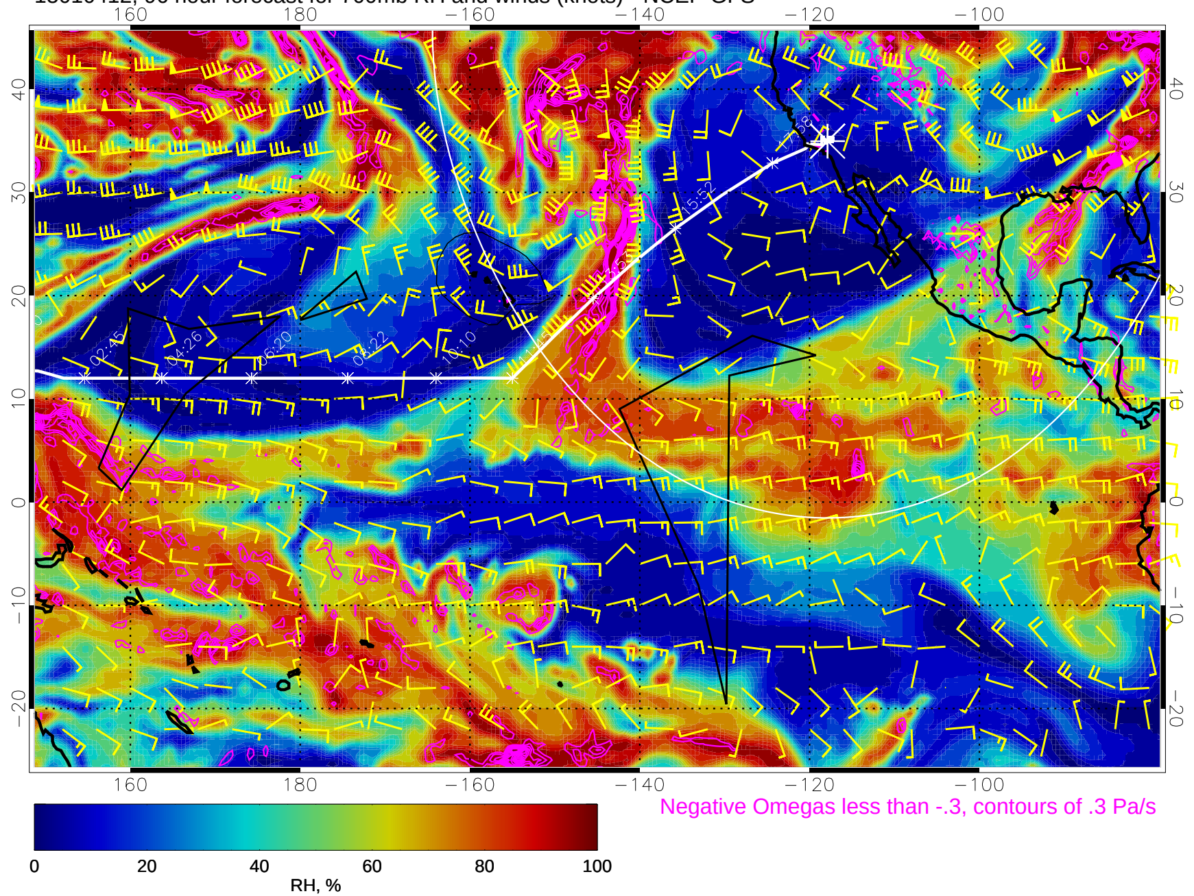
15010412, 96 hour forecast for 700mb RH and winds (knots) - NCEP GFS
