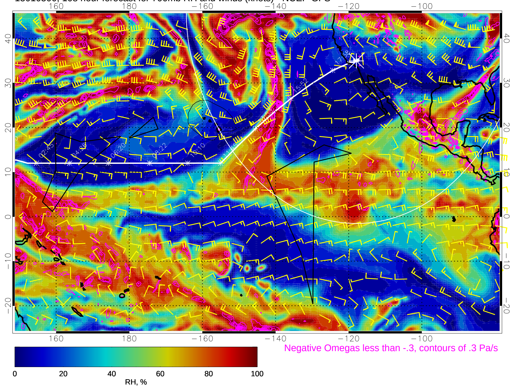
15010500, 108 hour forecast for 700mb RH and winds (knots) - NCEP GFS
