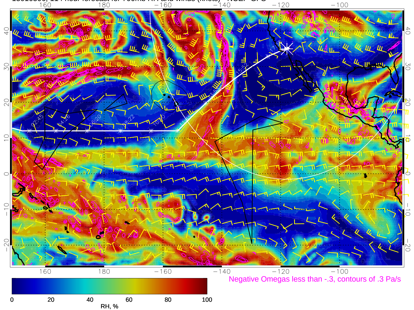
15010506, 114 hour forecast for 700mb RH and winds (knots) - NCEP GFS
