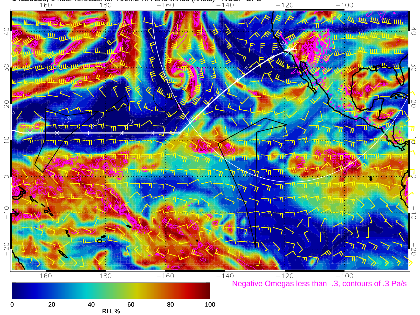
14123118, 6 hour forecast for 700mb RH and winds (knots) - NCEP GFS
