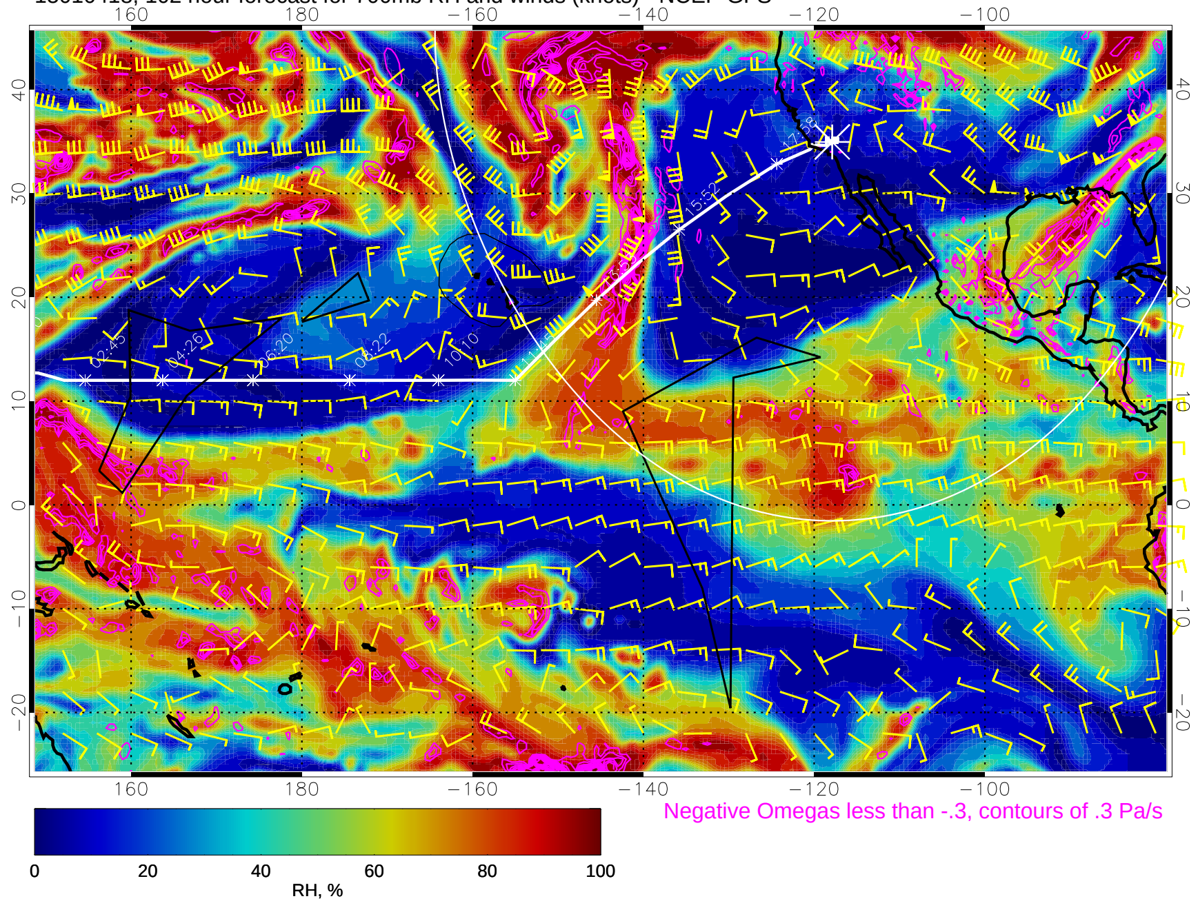
15010418, 102 hour forecast for 700mb RH and winds (knots) - NCEP GFS
