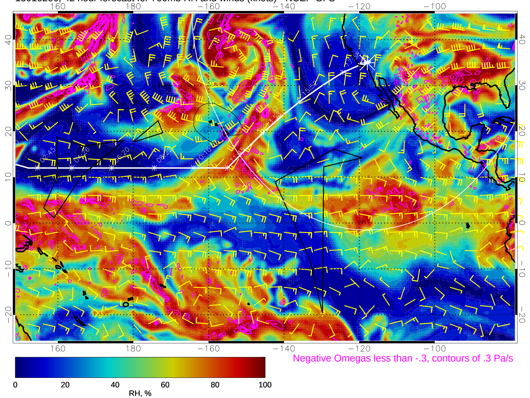
15010206, 42 hour forecast for 700mb RH and winds (knots) - NCEP GFS
