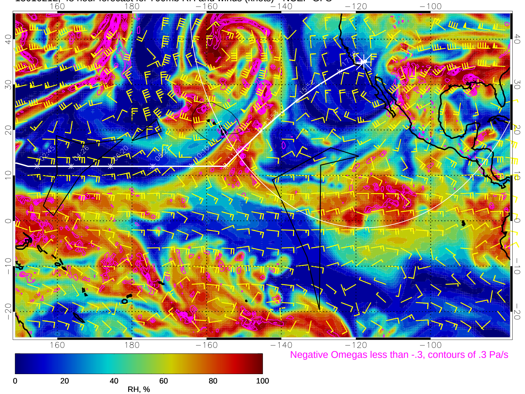
15010212, 48 hour forecast for 700mb RH and winds (knots) - NCEP GFS
