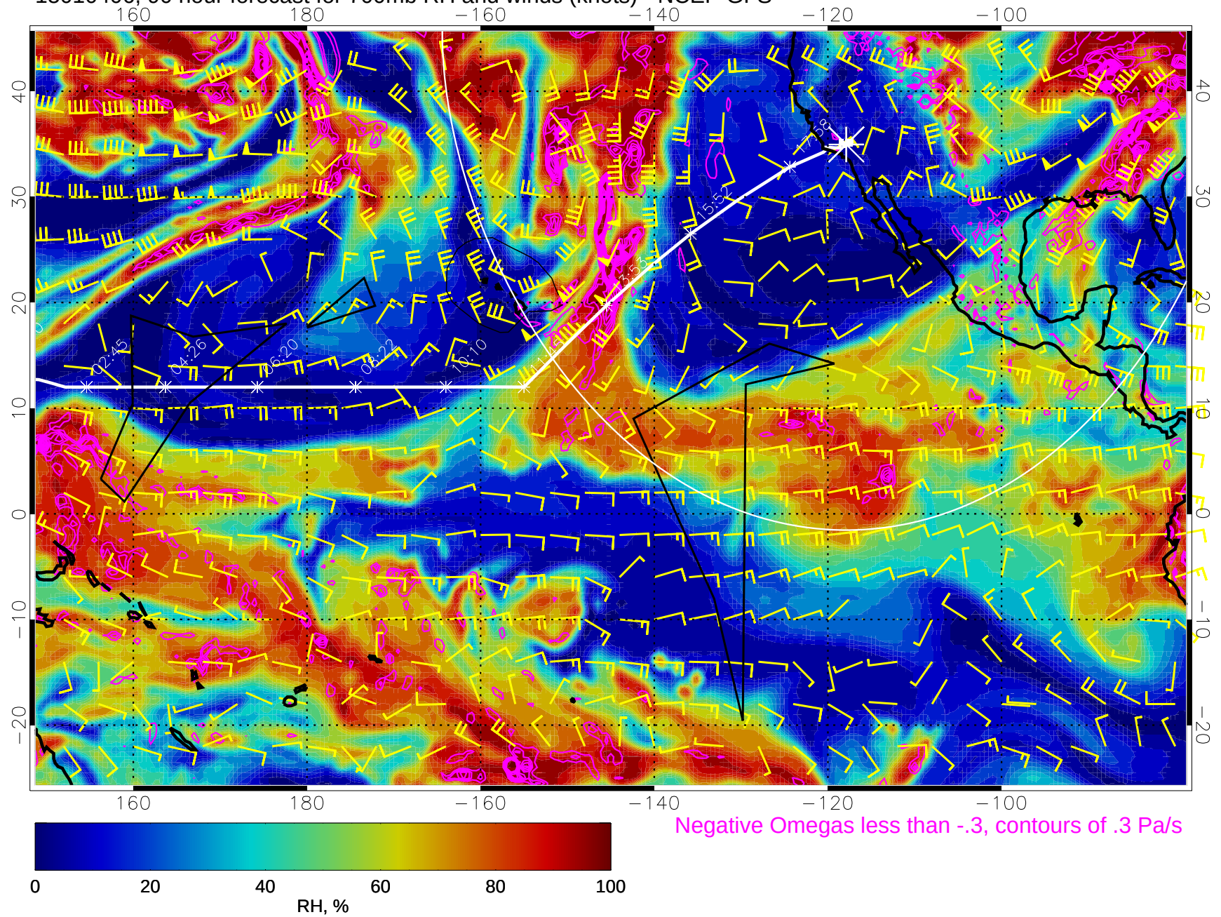
15010406, 90 hour forecast for 700mb RH and winds (knots) - NCEP GFS
