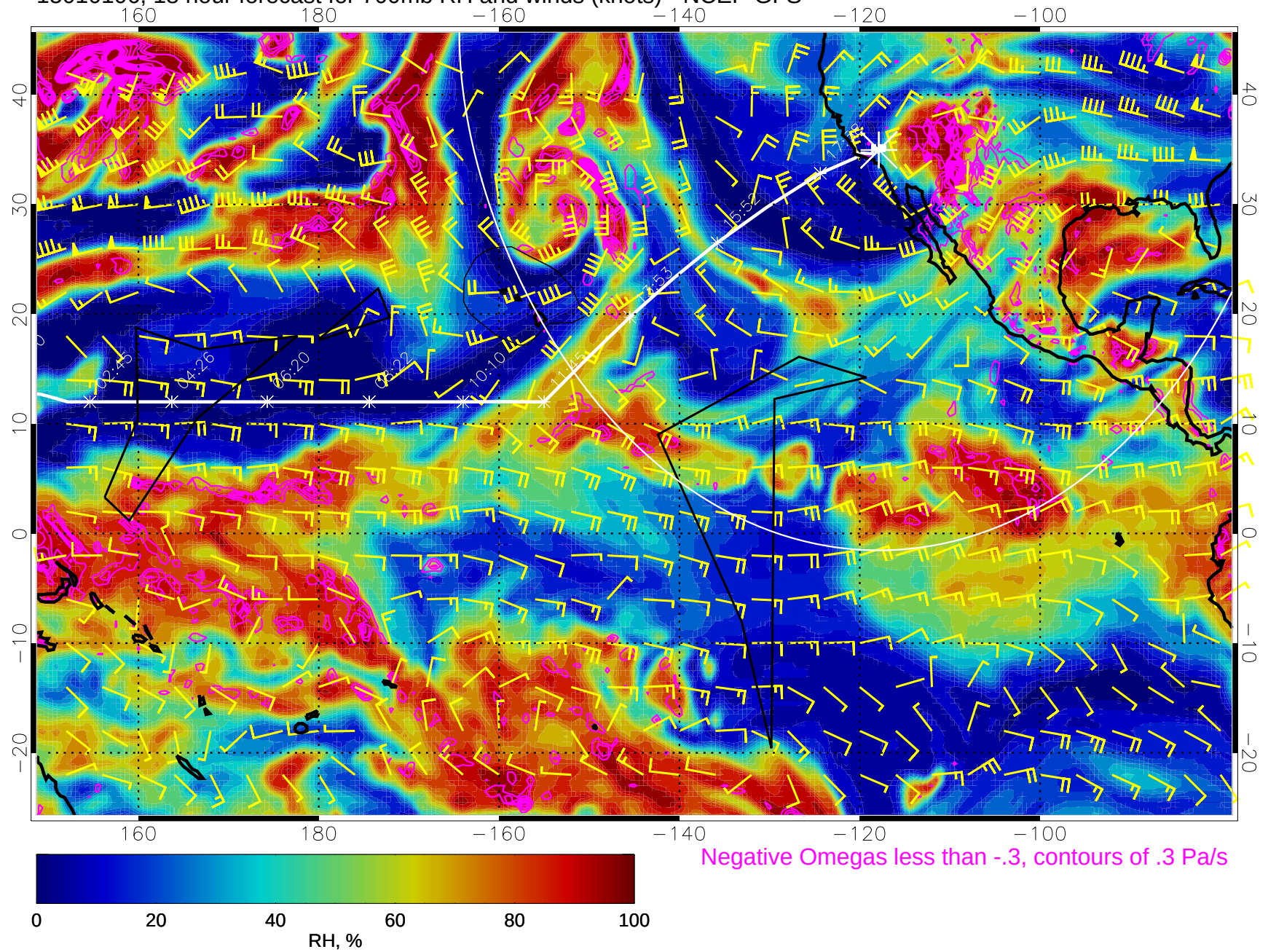
15010106, 18 hour forecast for 700mb RH and winds (knots) - NCEP GFS
