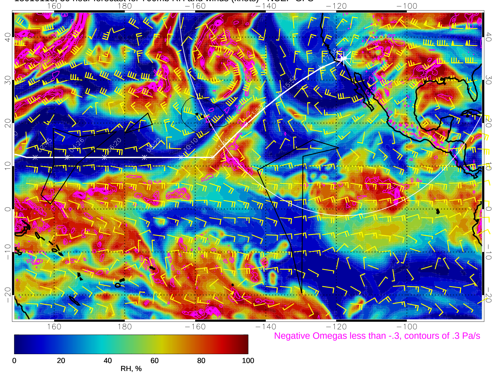
15010118, 30 hour forecast for 700mb RH and winds (knots) - NCEP GFS
