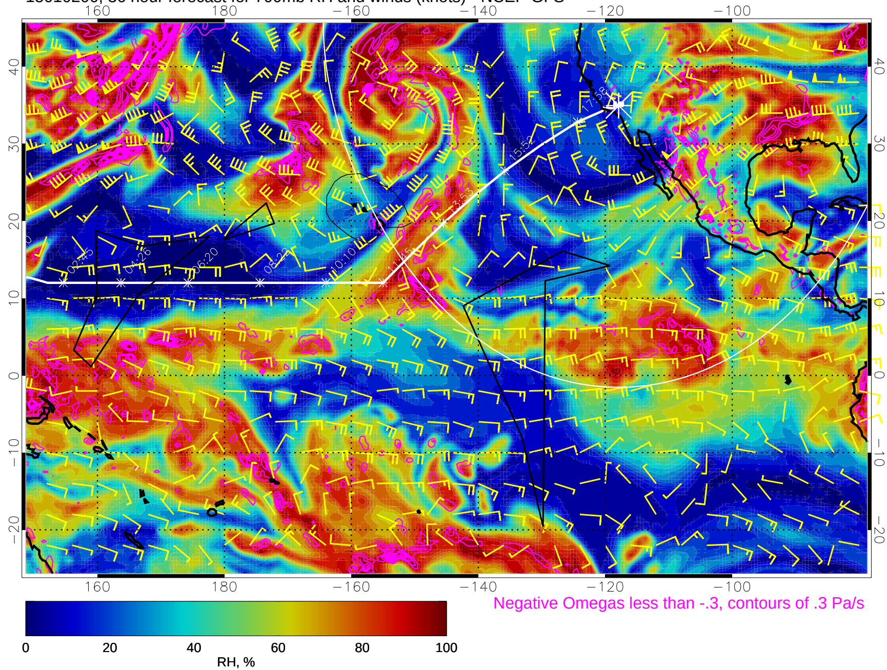
15010200, 36 hour forecast for 700mb RH and winds (knots) - NCEP GFS
