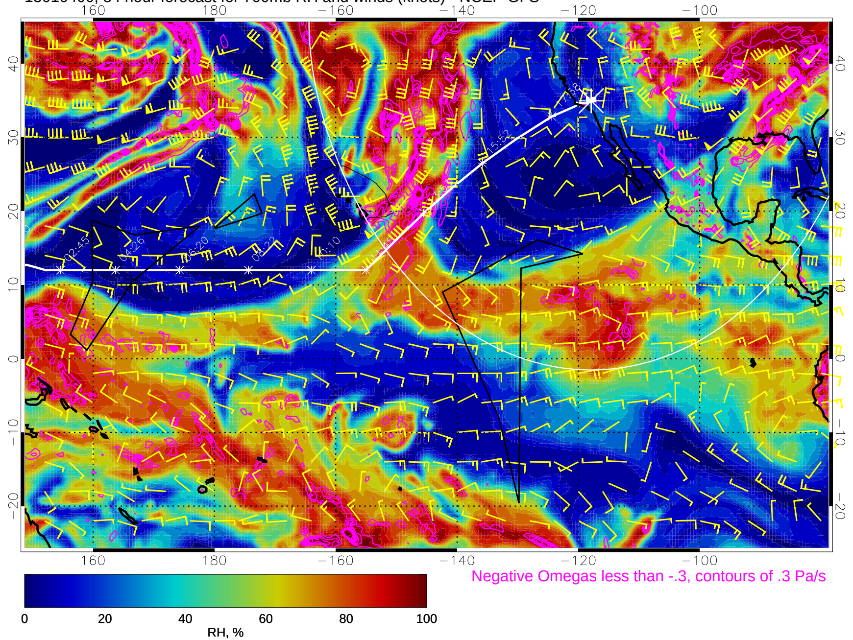
15010400, 84 hour forecast for 700mb RH and winds (knots) - NCEP GFS
