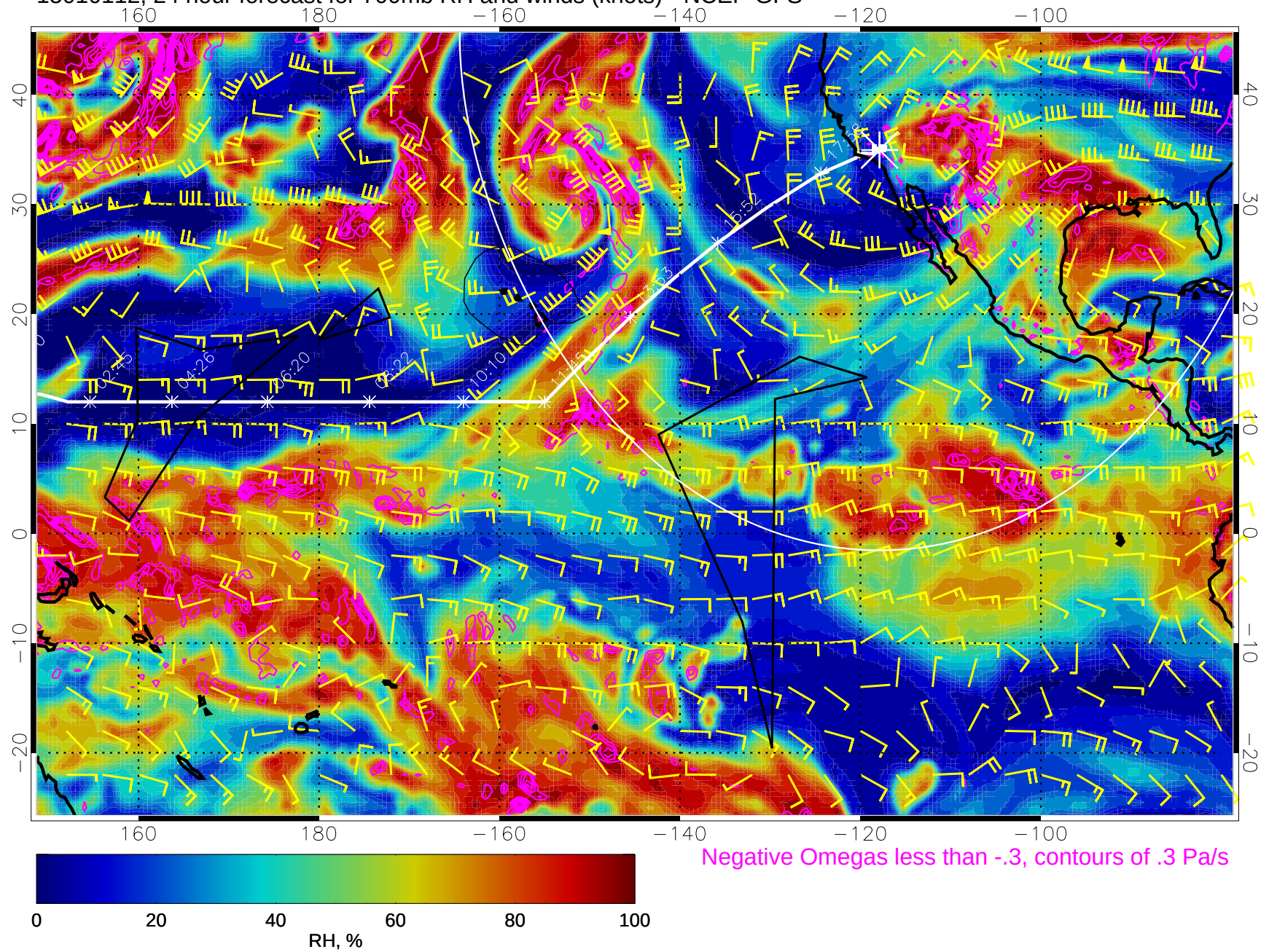
15010112, 24 hour forecast for 700mb RH and winds (knots) - NCEP GFS
