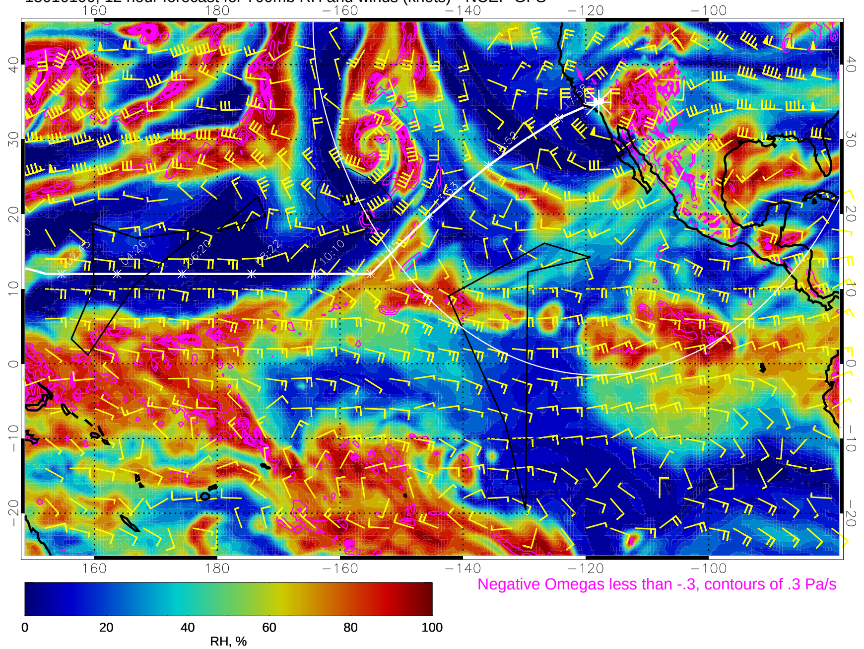
15010100, 12 hour forecast for 700mb RH and winds (knots) - NCEP GFS
