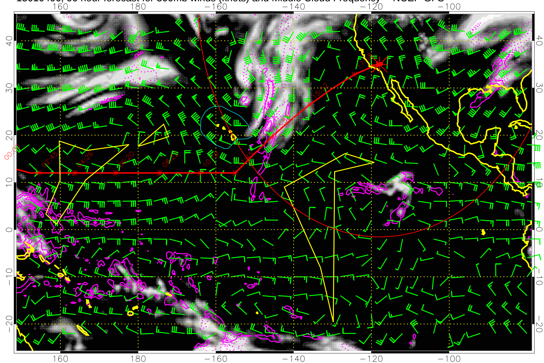
15010406, 90 hour forecast for 500mb winds (knots) and Middle Cloud Frequency -- NCEP GFS
