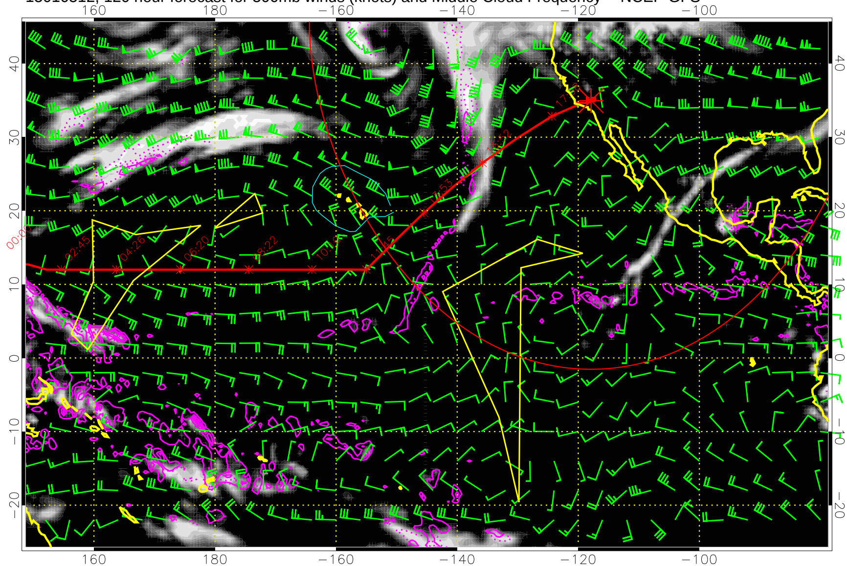
15010512, 120 hour forecast for 500mb winds (knots) and Middle Cloud Frequency -- NCEP GFS
