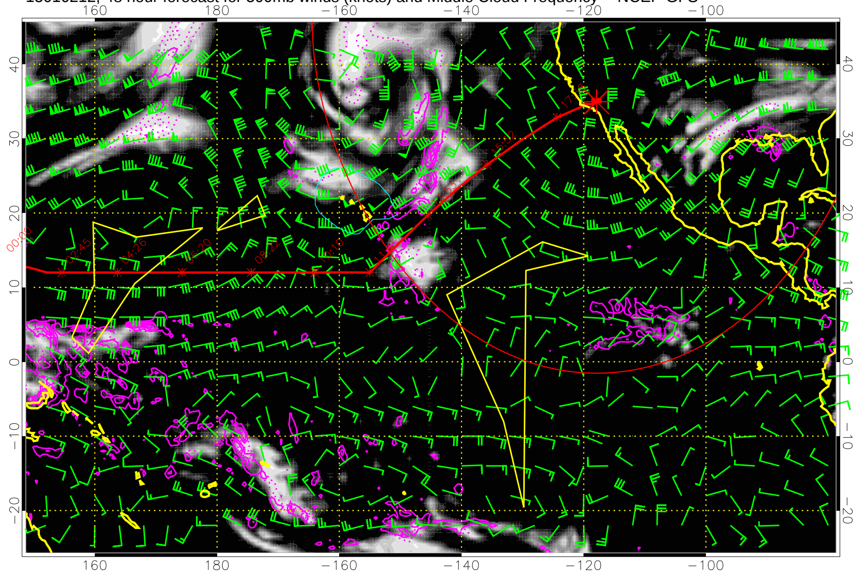
15010212, 48 hour forecast for 500mb winds (knots) and Middle Cloud Frequency -- NCEP GFS
