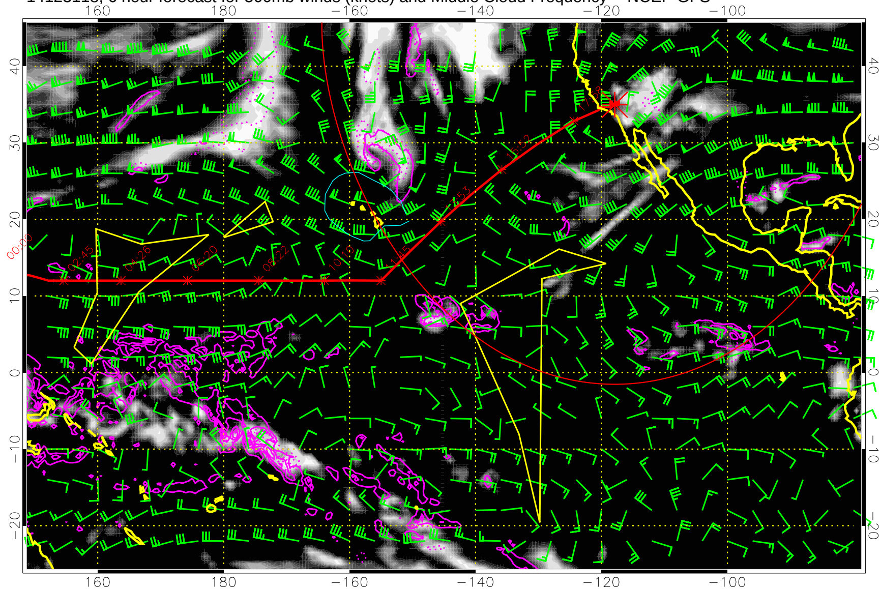
14123118, 6 hour forecast for 500mb winds (knots) and Middle Cloud Frequency -- NCEP GFS
