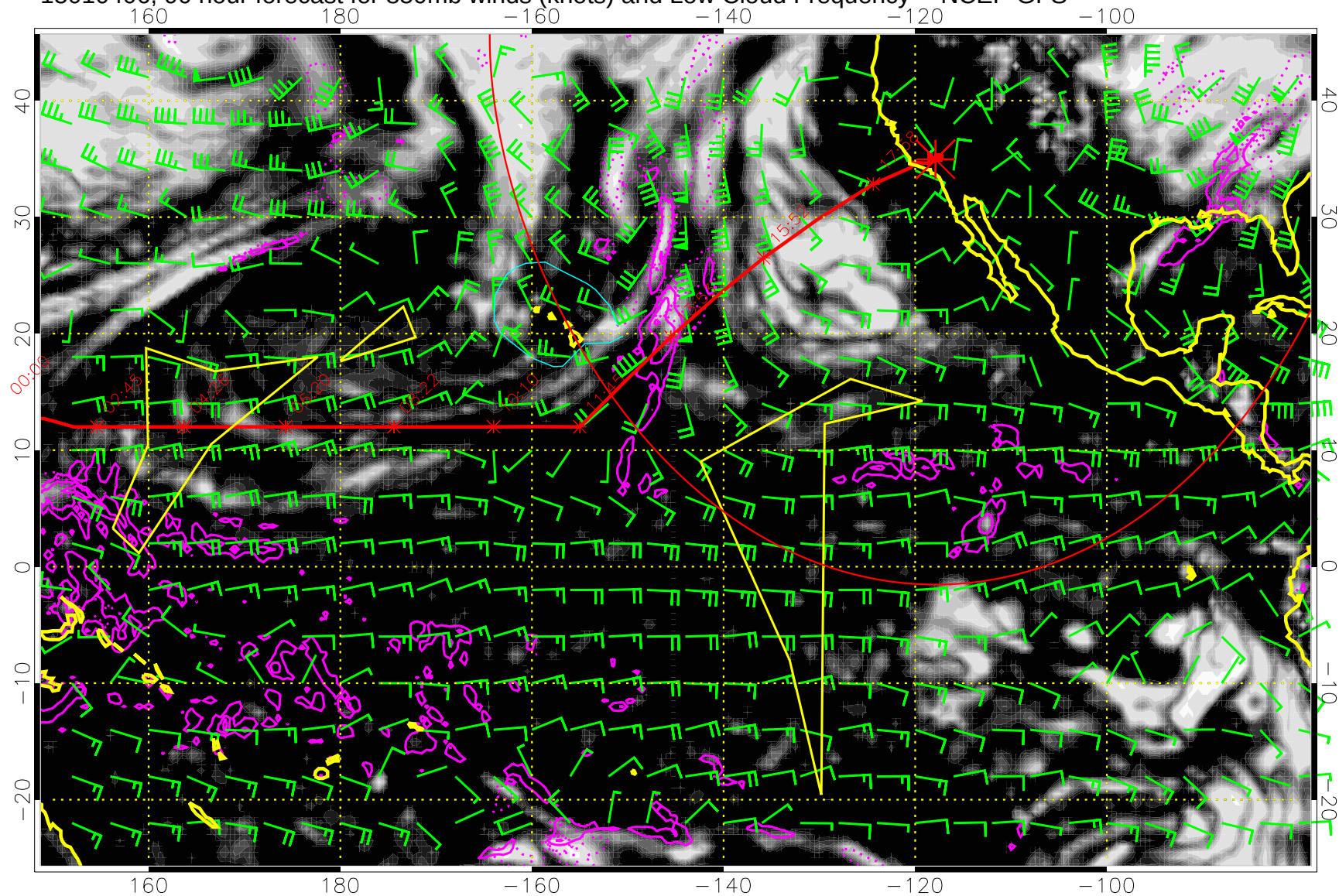
15010406, 90 hour forecast for 850mb winds (knots) and Low Cloud Frequency -- NCEP GFS
