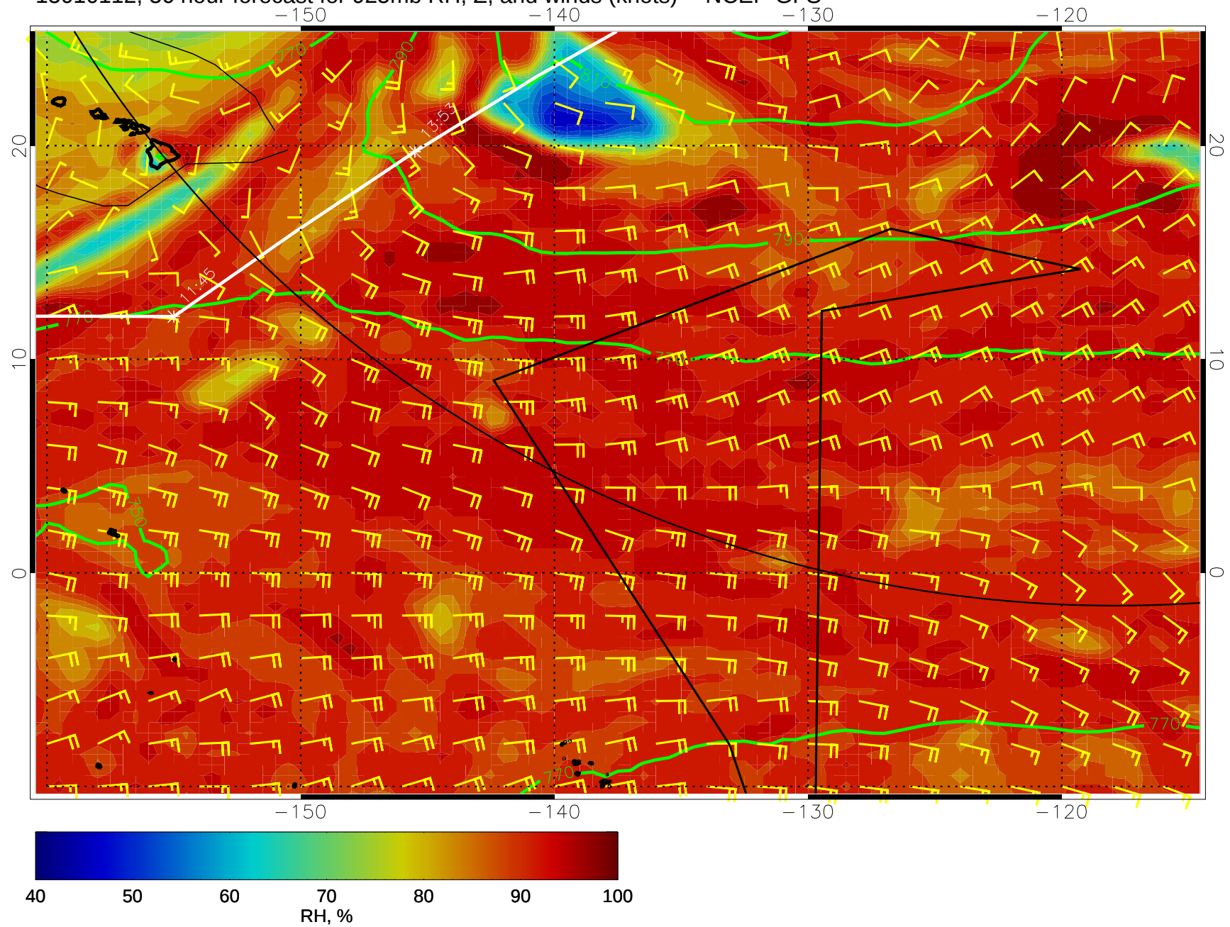
15010112, 36 hour forecast for 925mb RH, Z, and winds (knots) -- NCEP GFS
