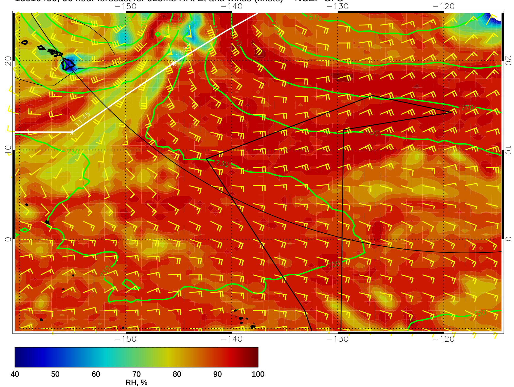
15010400, 96 hour forecast for 925mb RH, Z, and winds (knots) -- NCEP GFS
