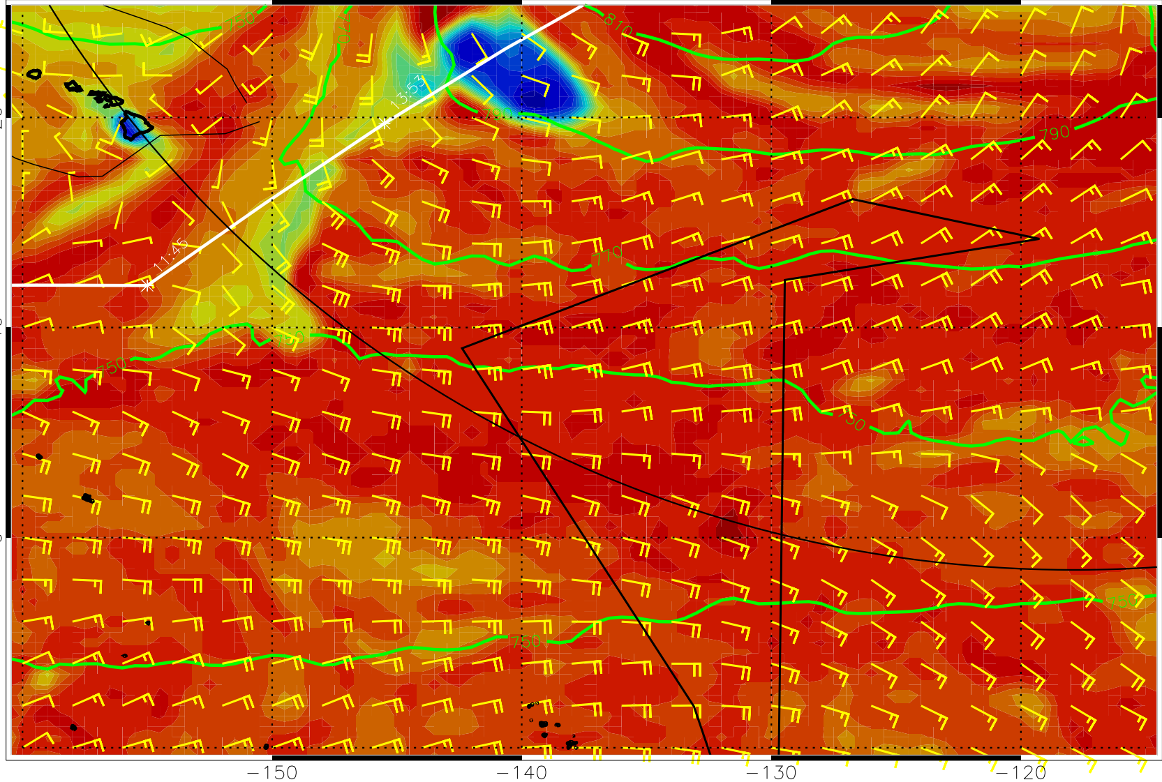
East for clouds (km, \pm , and winds (km/s) 100% 0% 100% 0% 100% 0%
