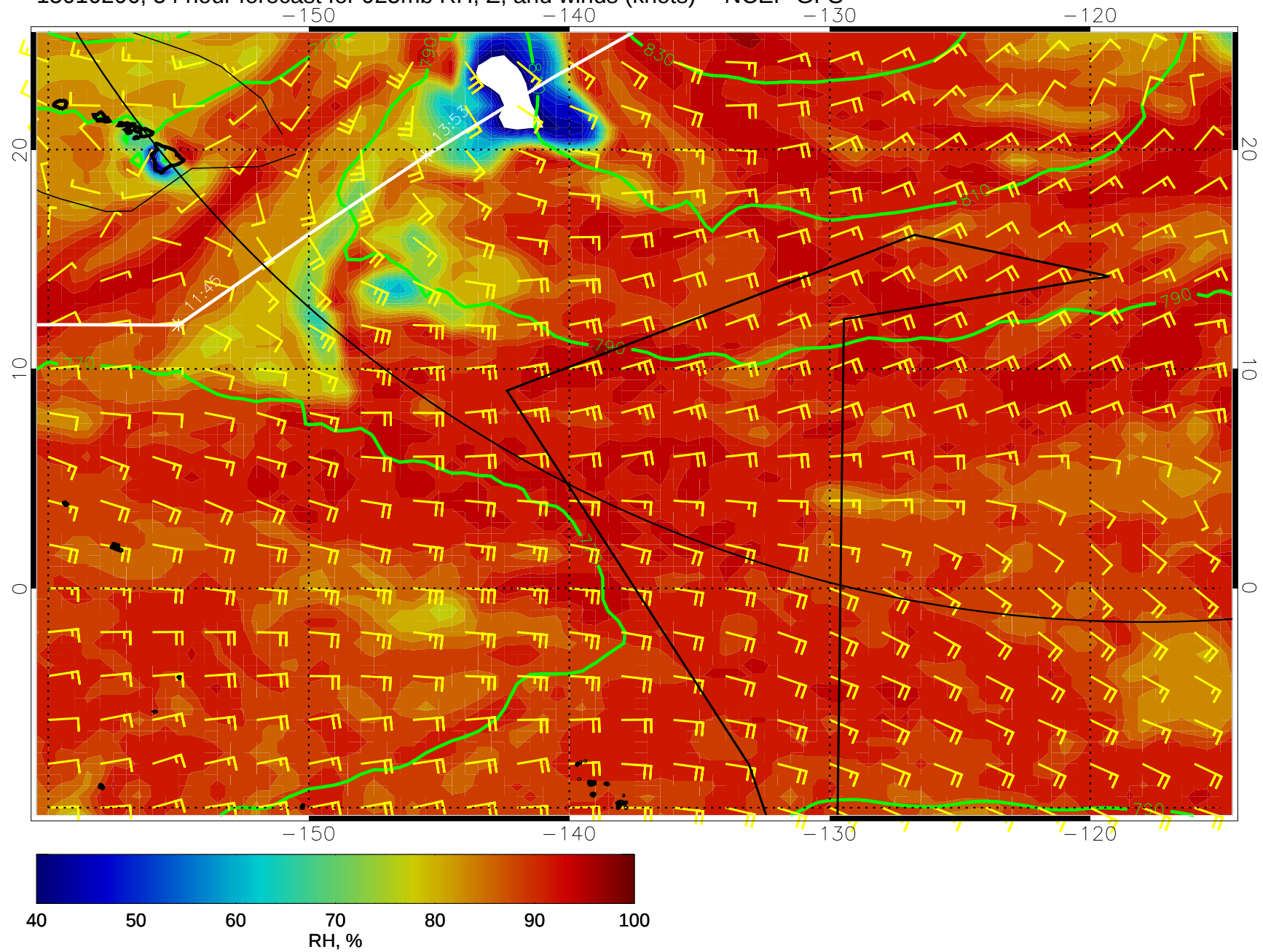
15010206, 54 hour forecast for 925mb RH, Z, and winds (knots) -- NCEP GFS
